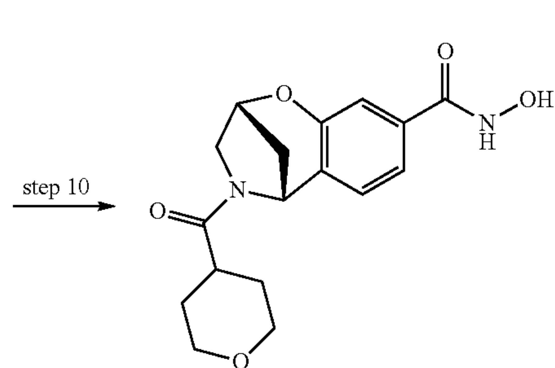
Step-3: 7-Hydroxy-4-oxochroman-2-carboxylic acid
