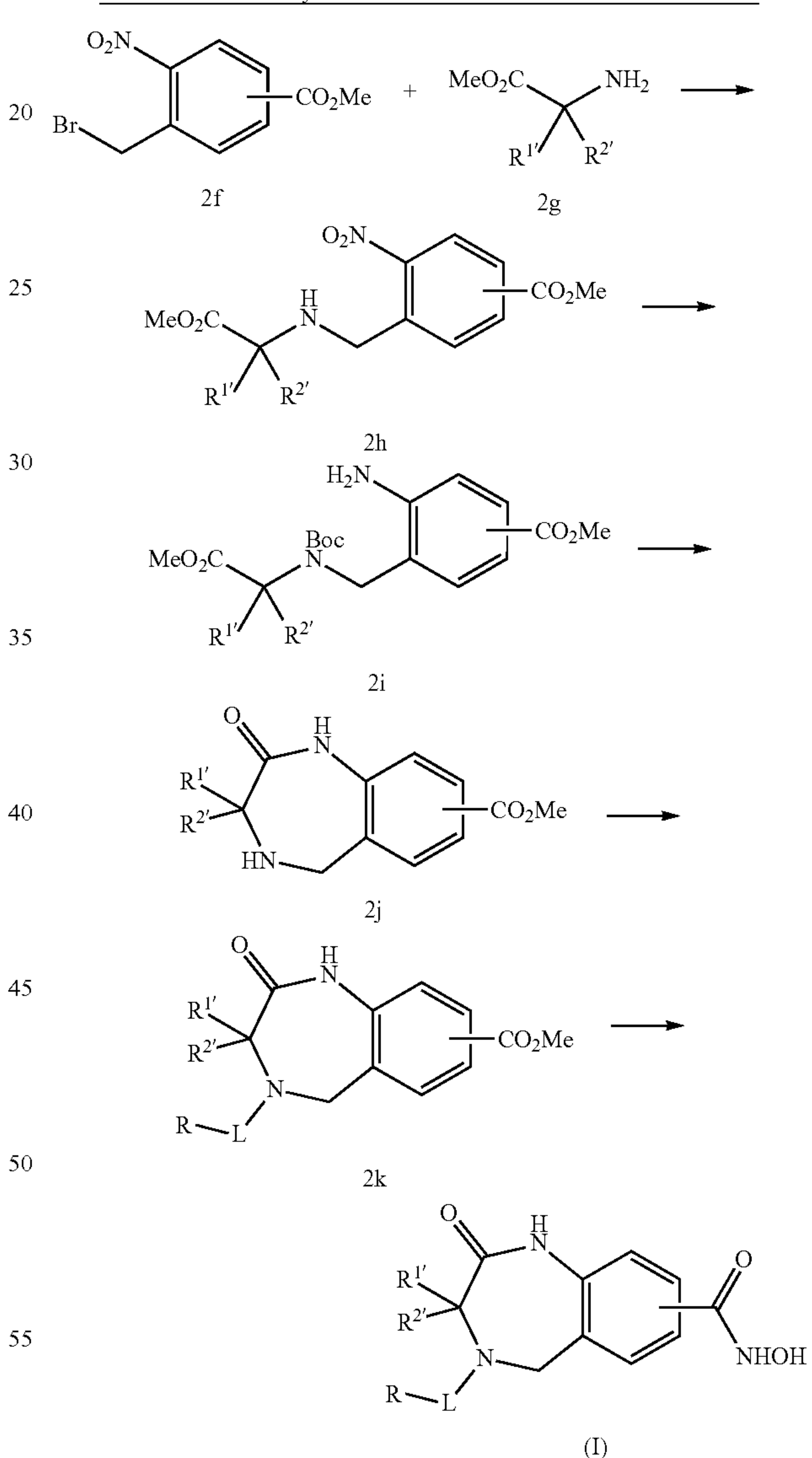
Scheme 2. General synthesis of amides described in the disclosure.
