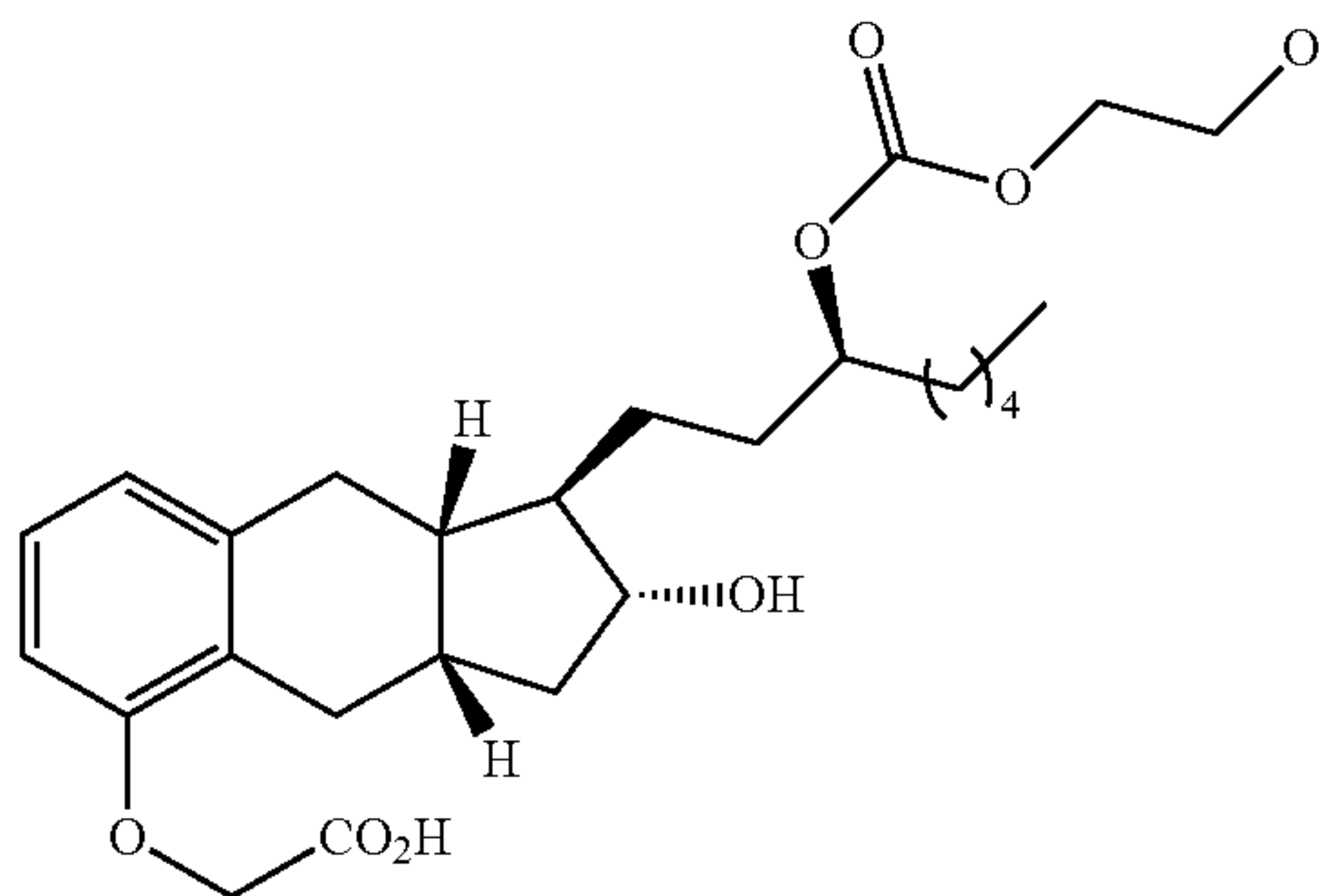
Compound Ib-15
