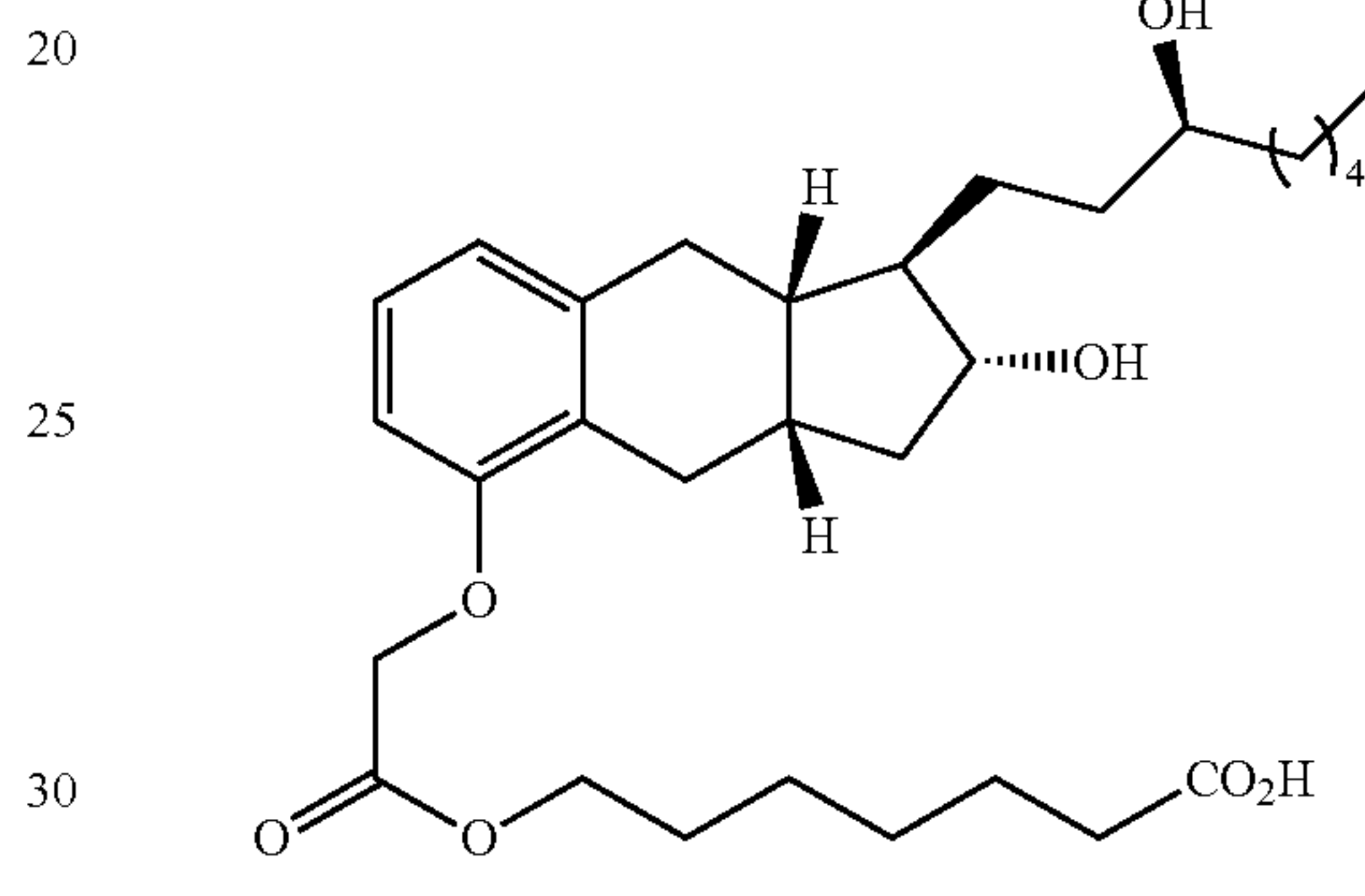
Compound II-11
