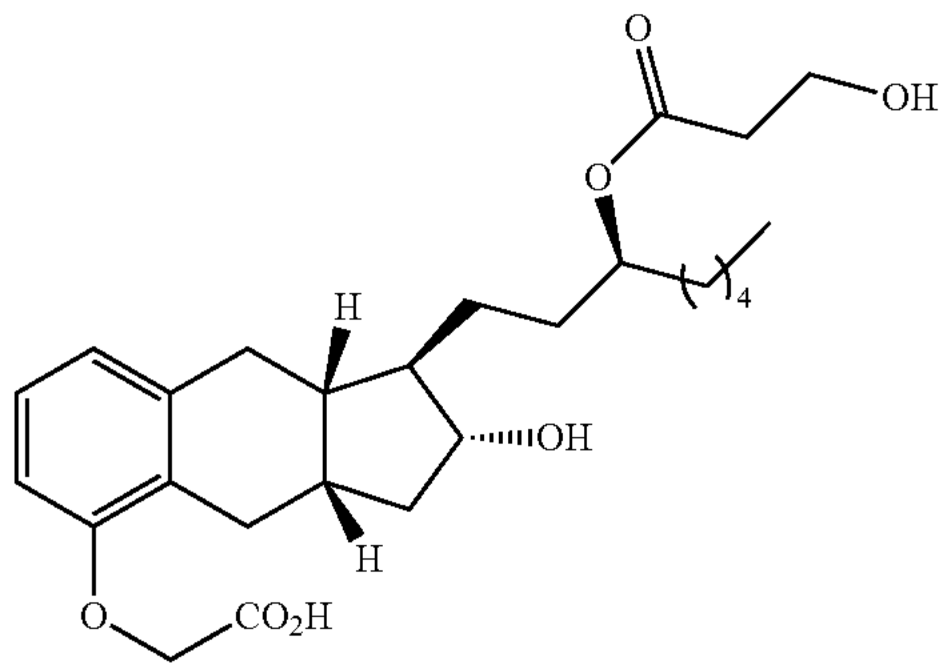
Compound Ib-5
