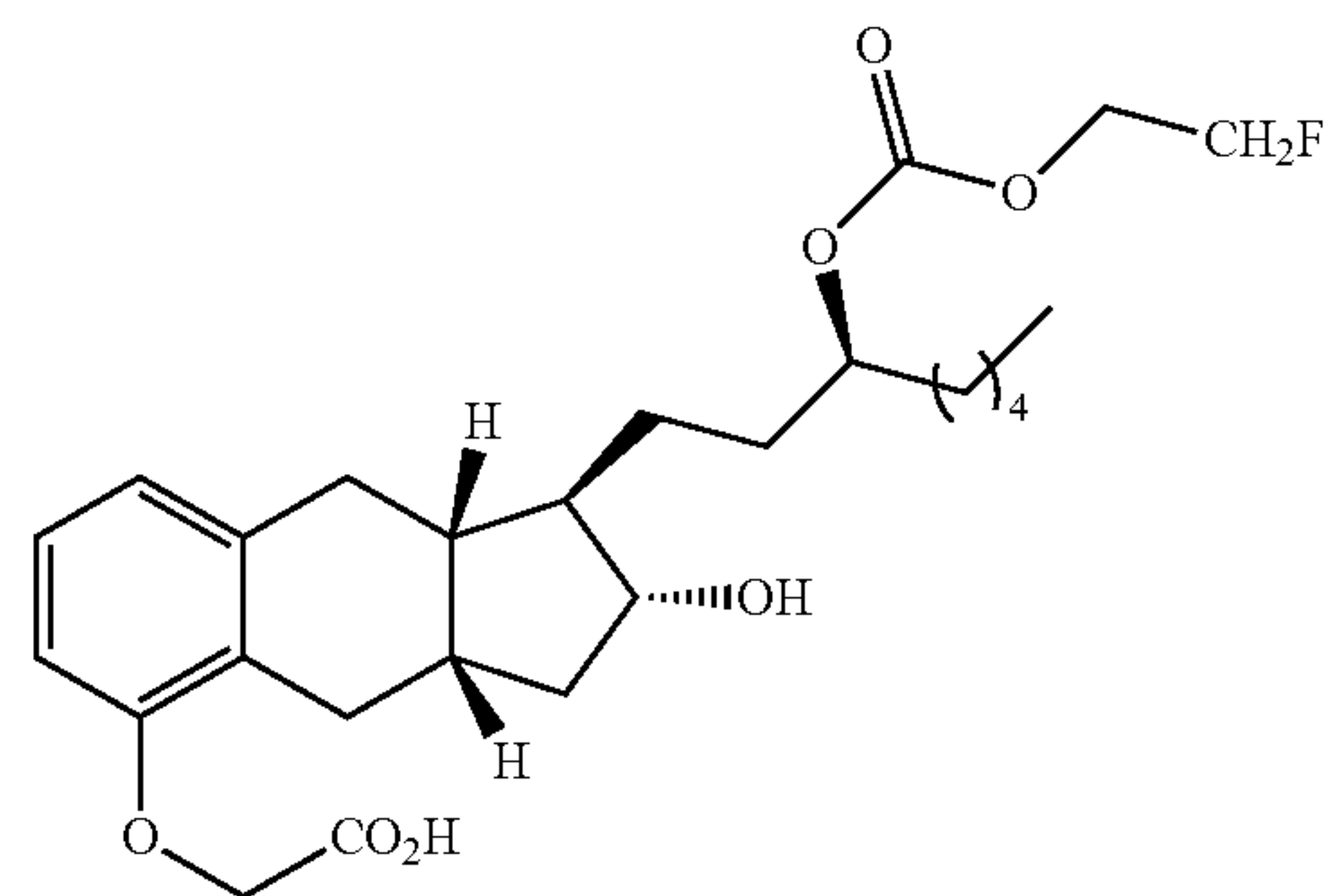
Compound Ib-12
