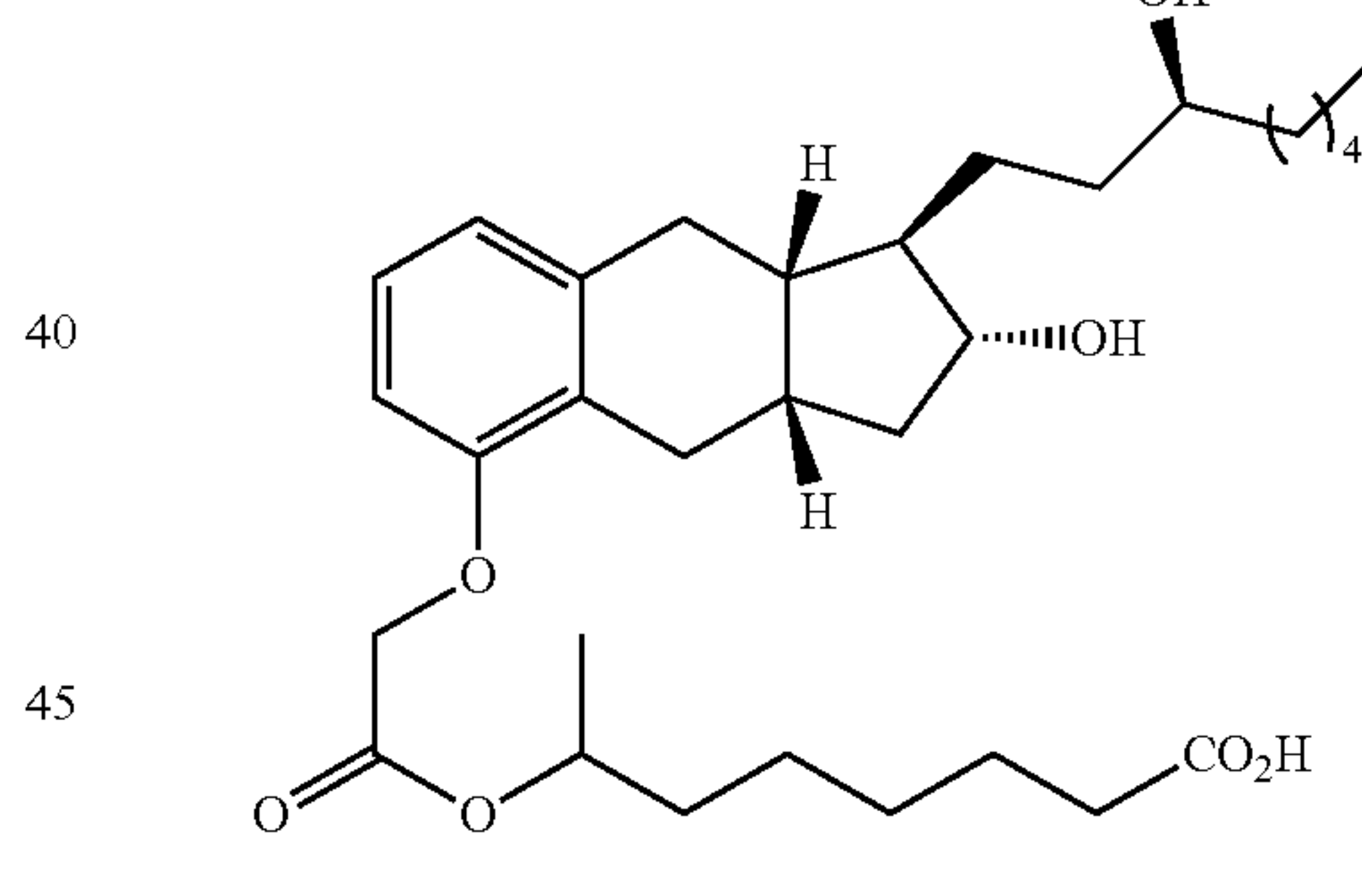
Compound II-12
