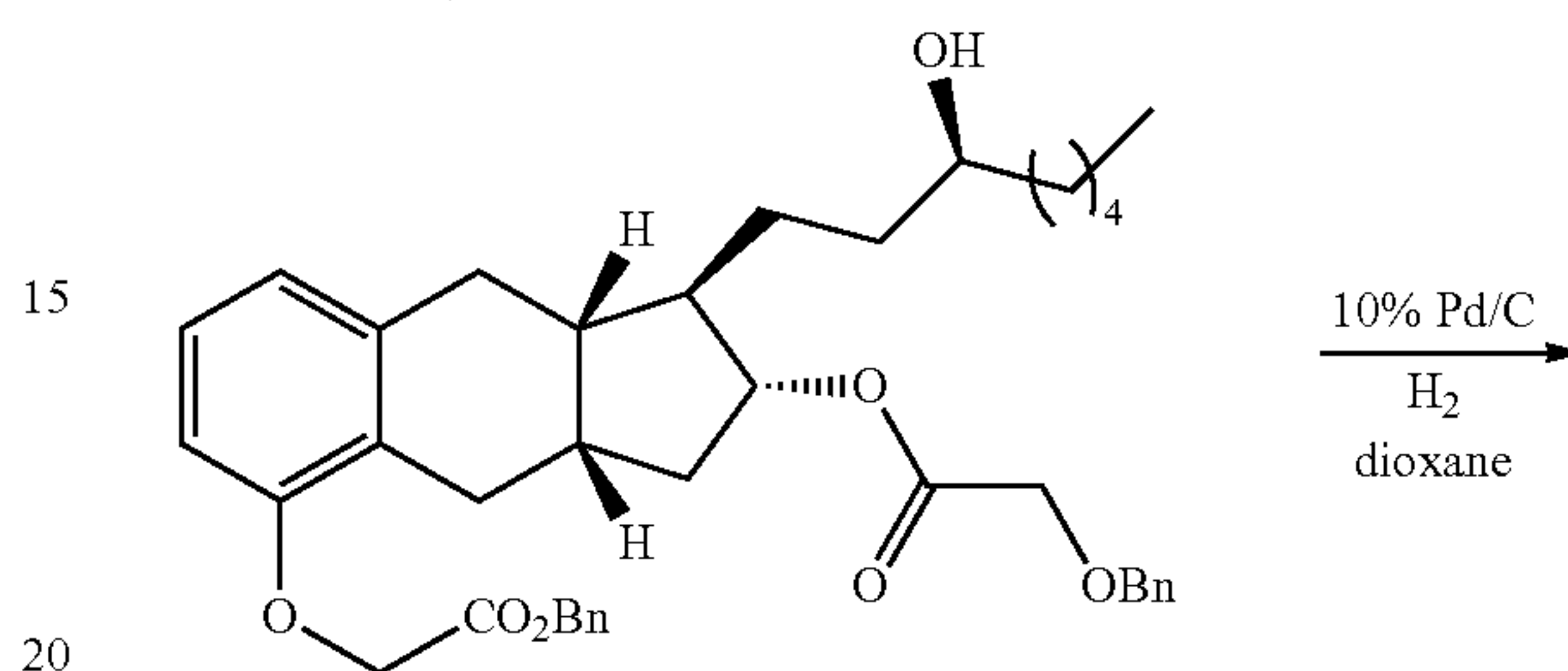
Compound Ia-3
