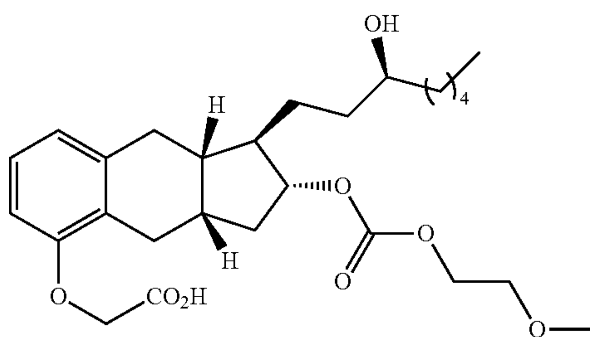
Compound Ia-15
