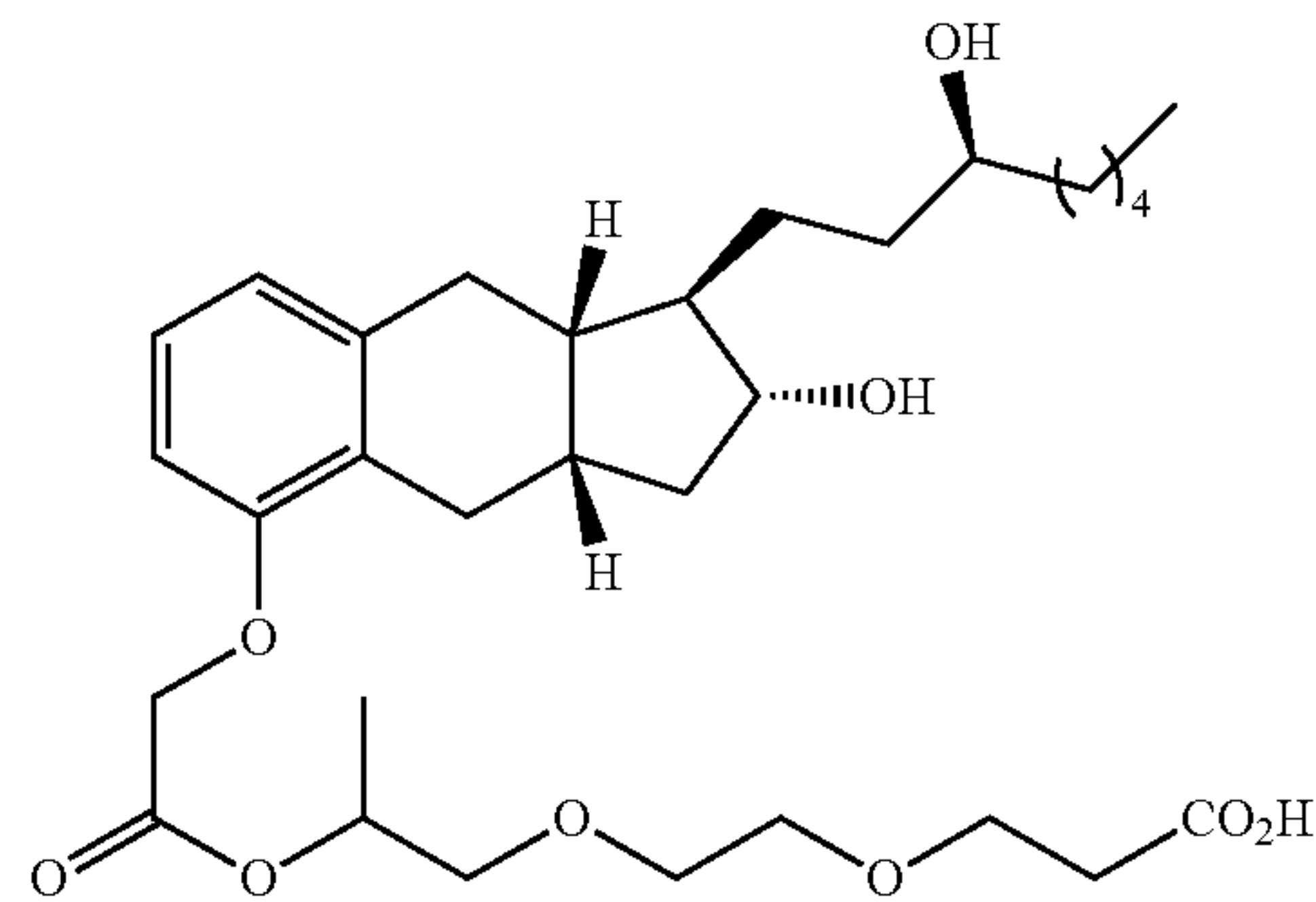
Compound II-20
