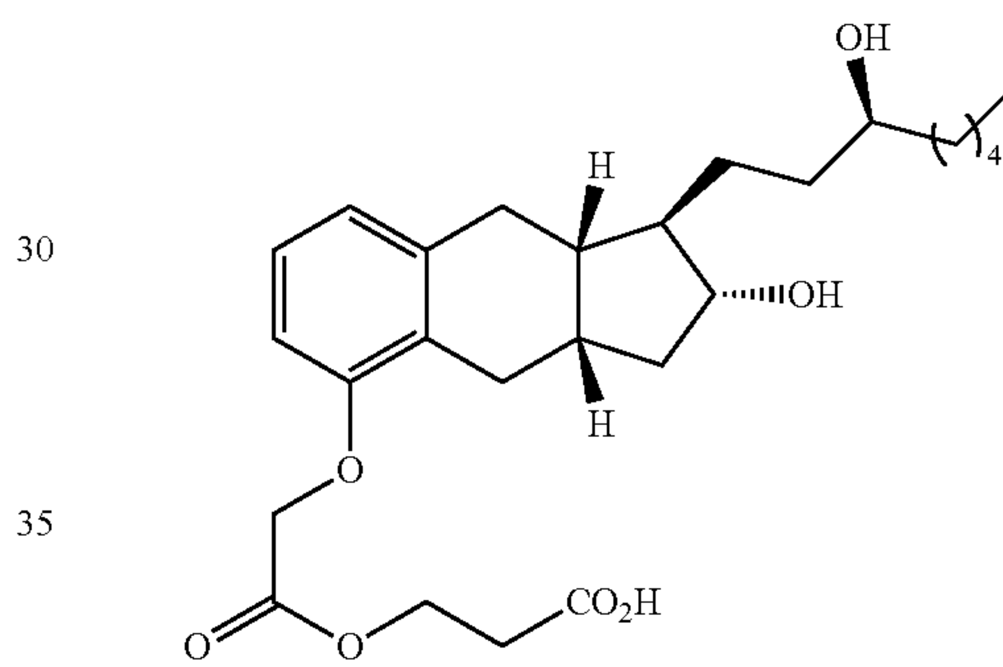
Compound II-24
