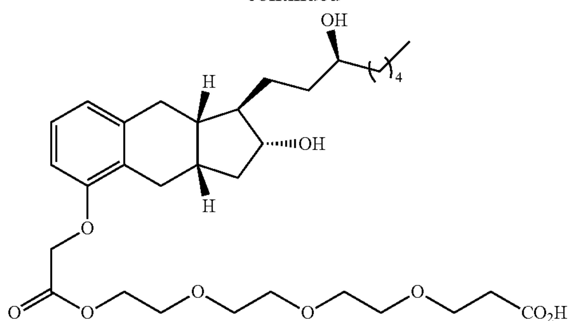
Compound II-18
