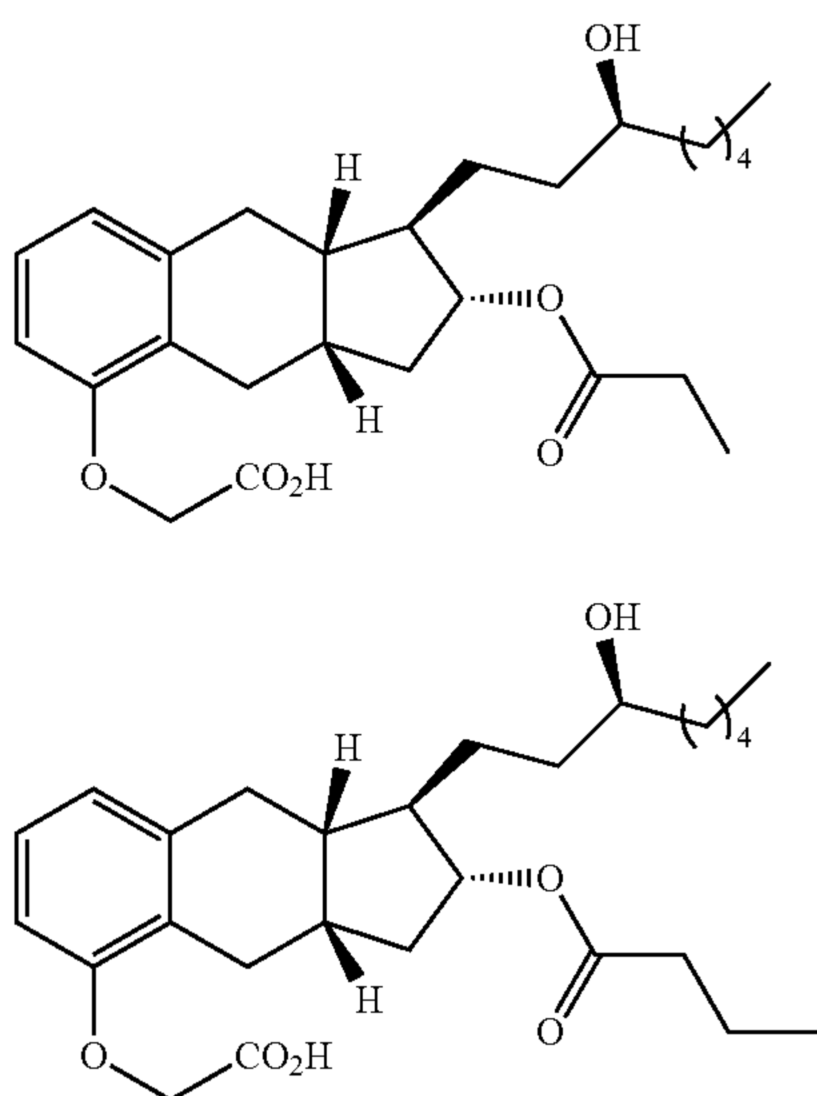
Compound Ia-2
