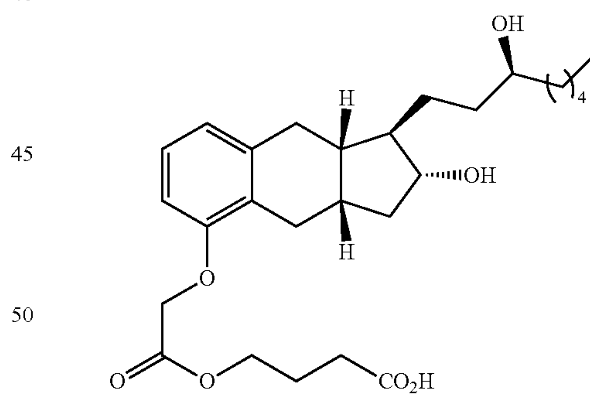
Compound II-25
