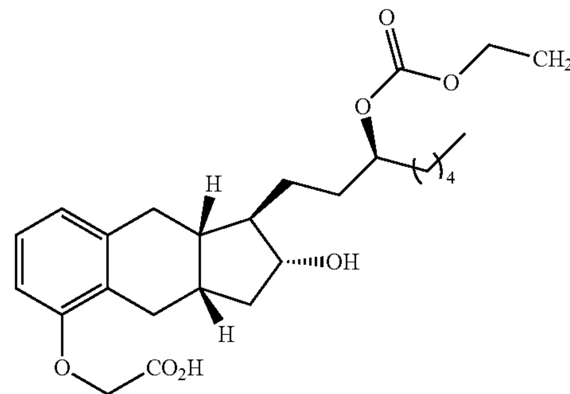
Compound Ib-12
