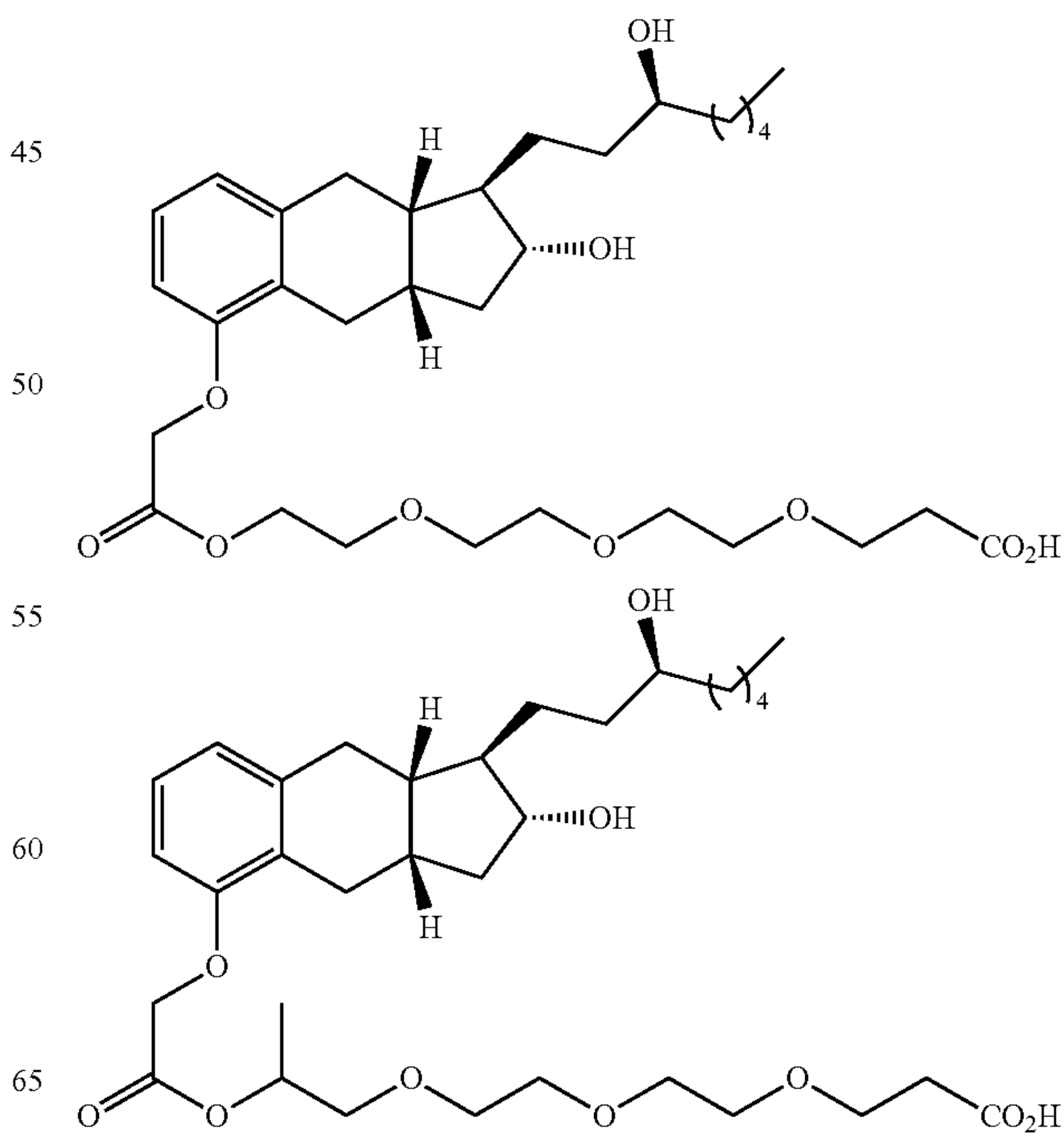
Compound II-19
