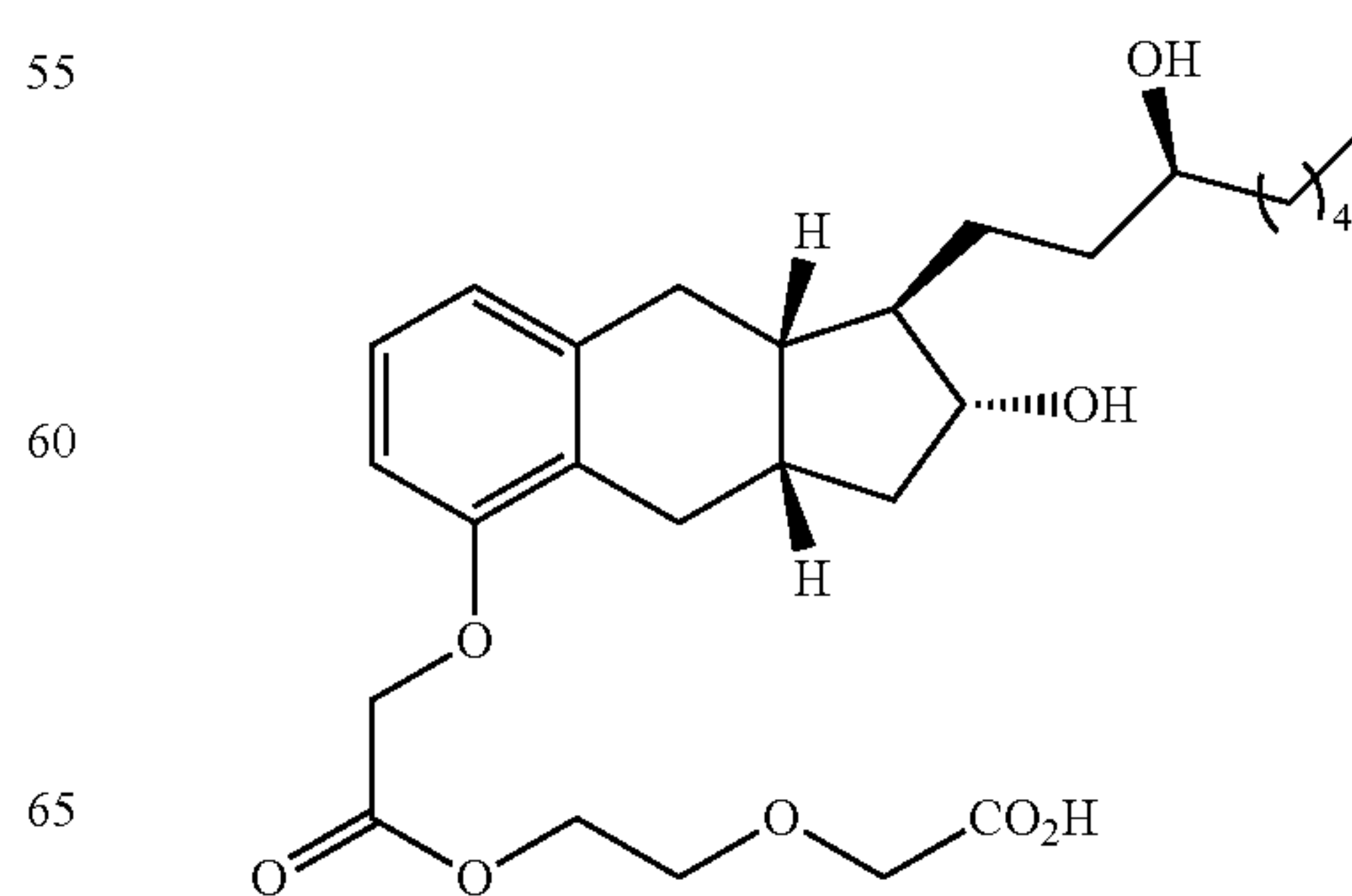
Compound II-13
