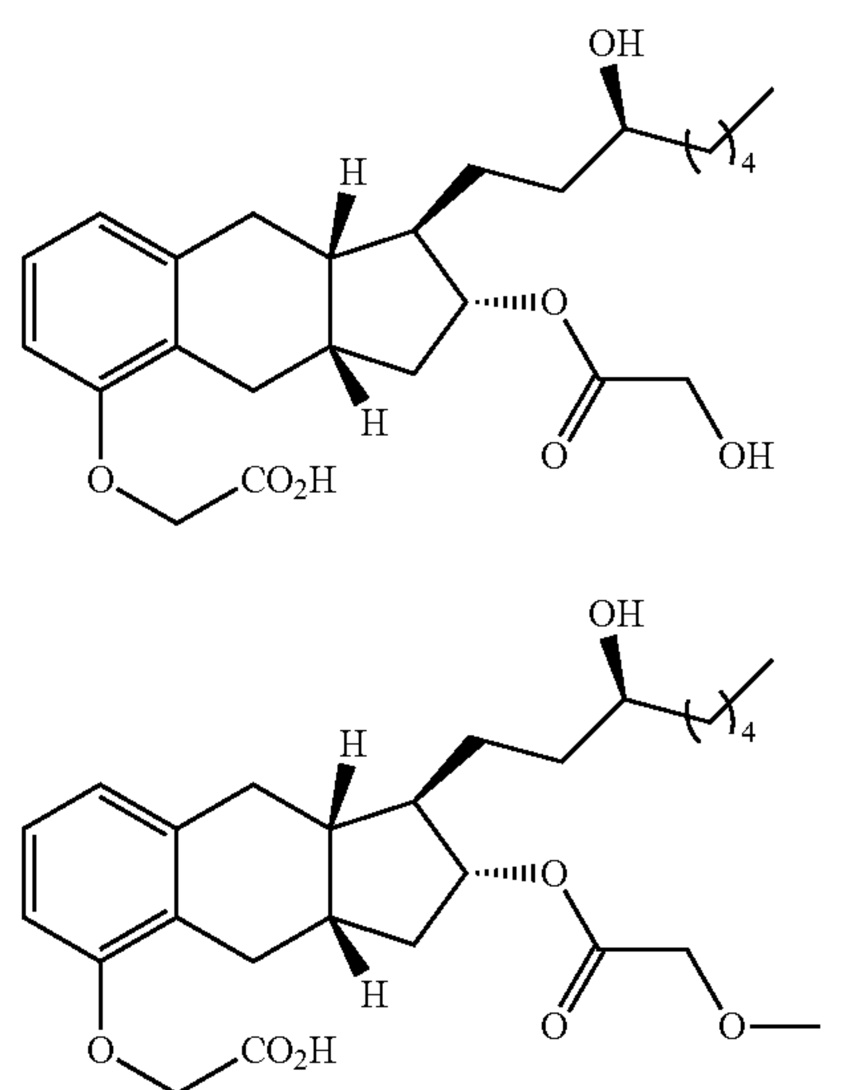
Compound Ia-8
