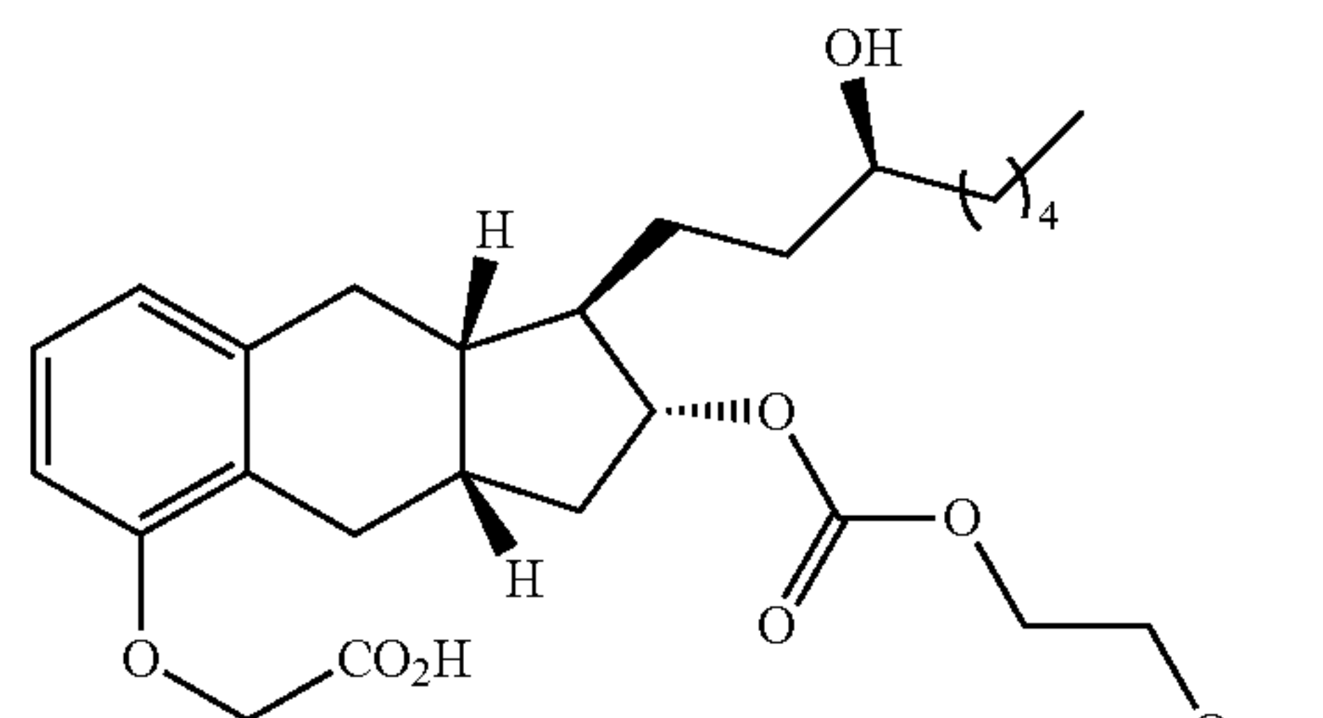
Compound Ib-1
