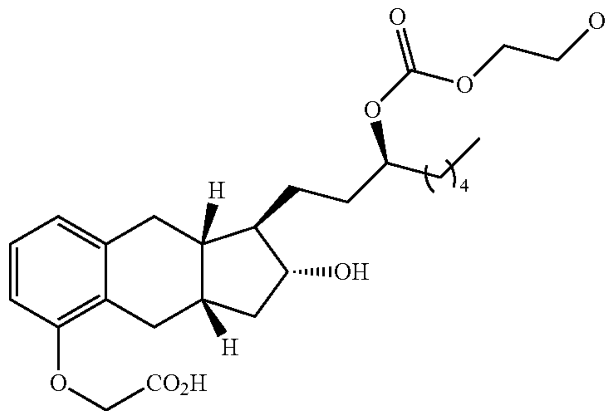
Compound Ib-14
