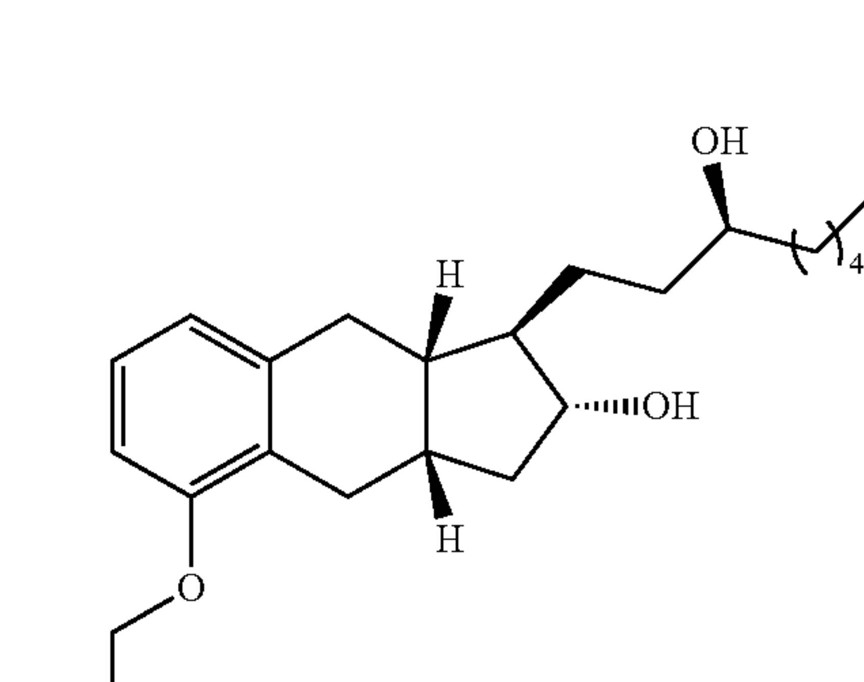
Compound II-4
