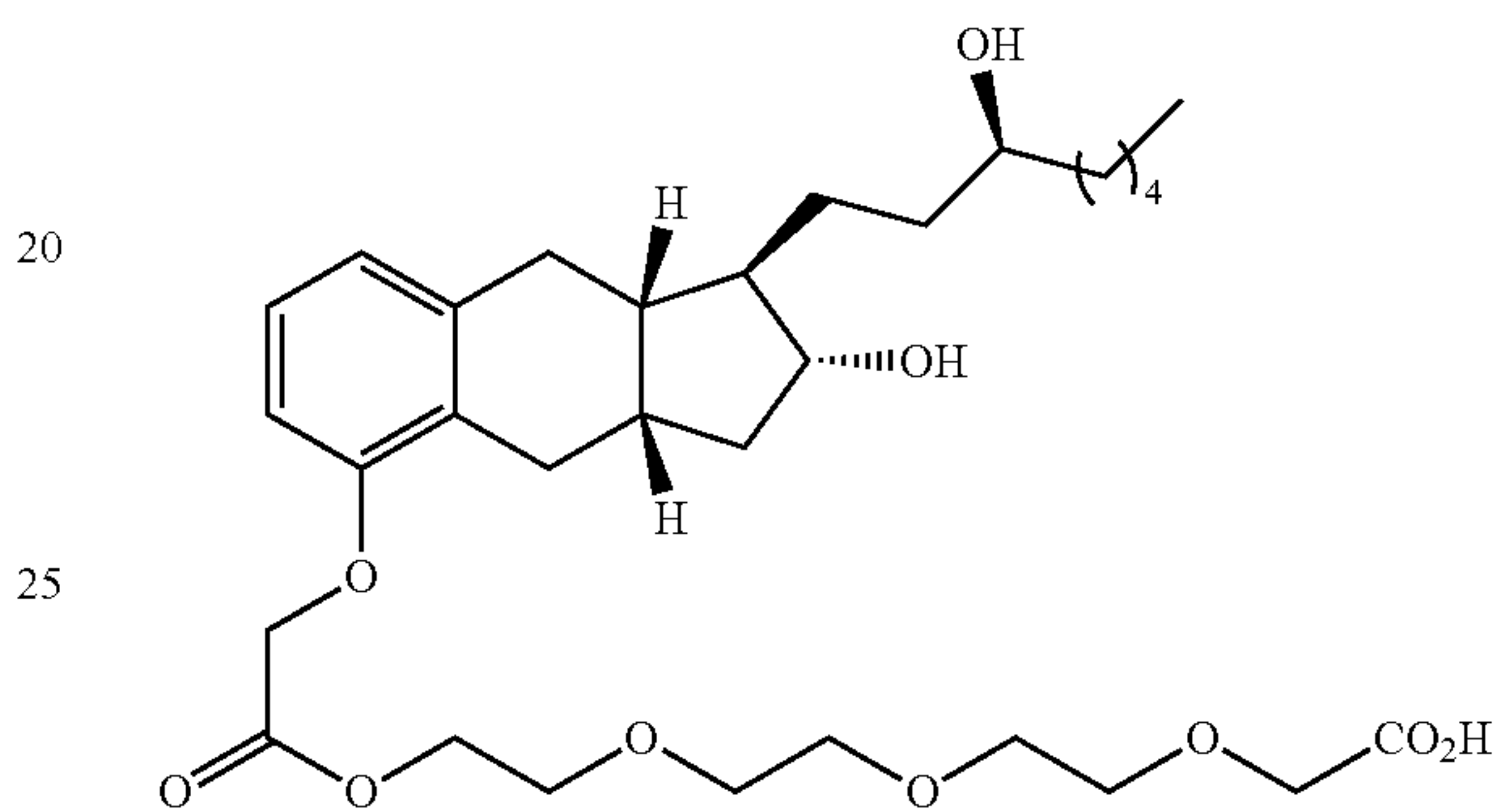
Compound II-17
