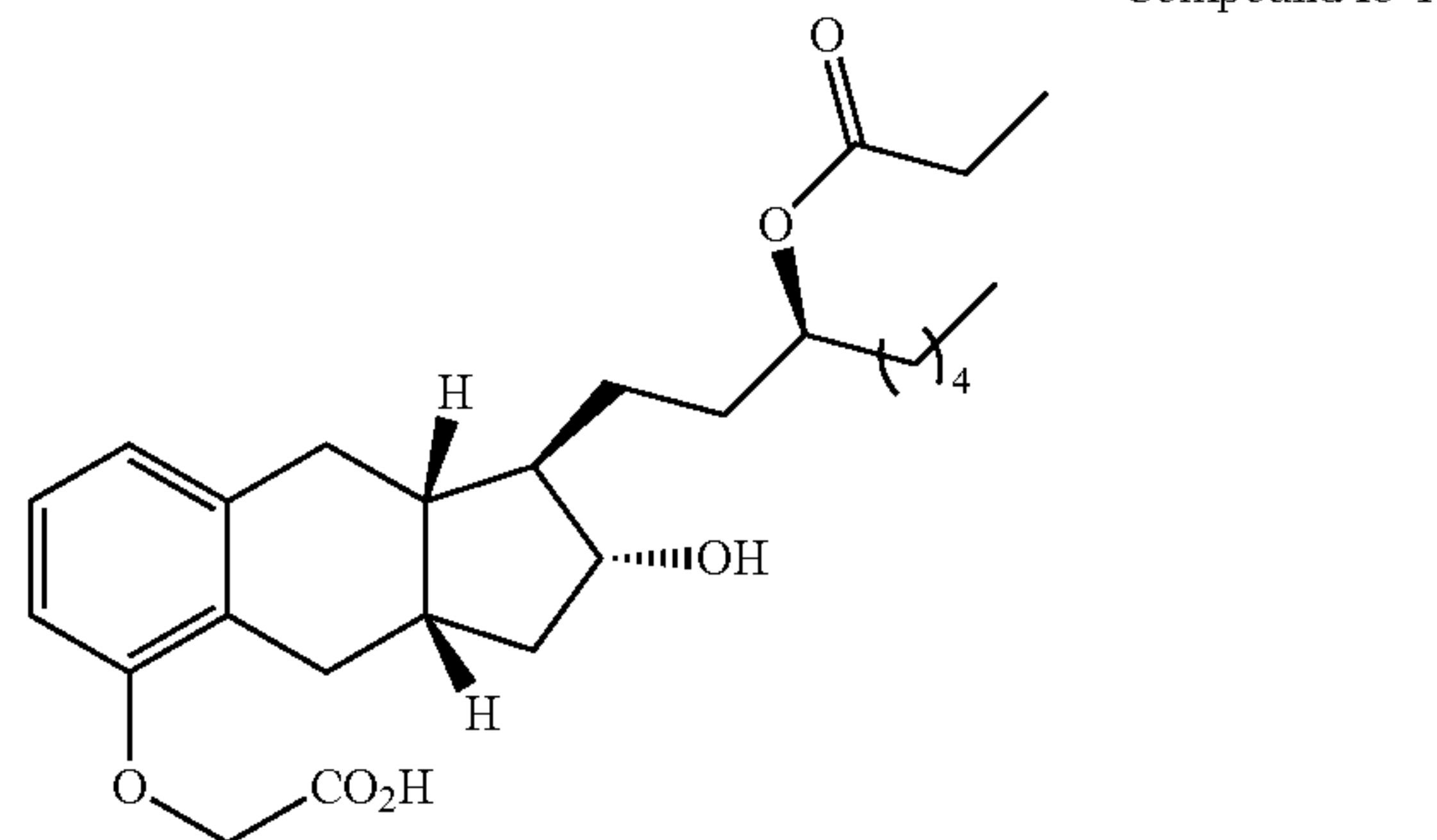
Compound Ib-2
