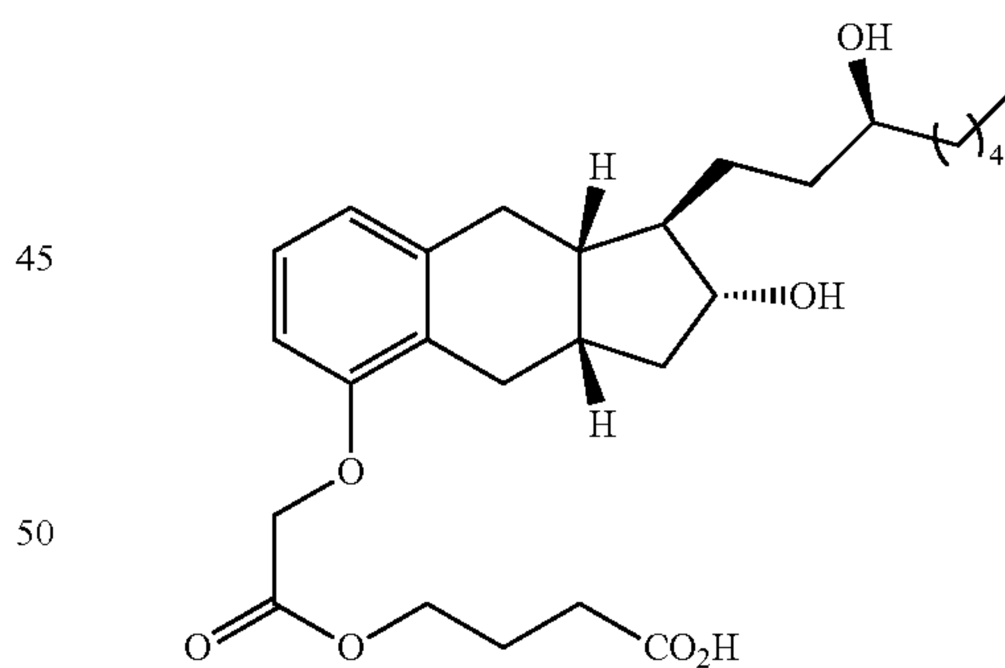
Compound II-25
