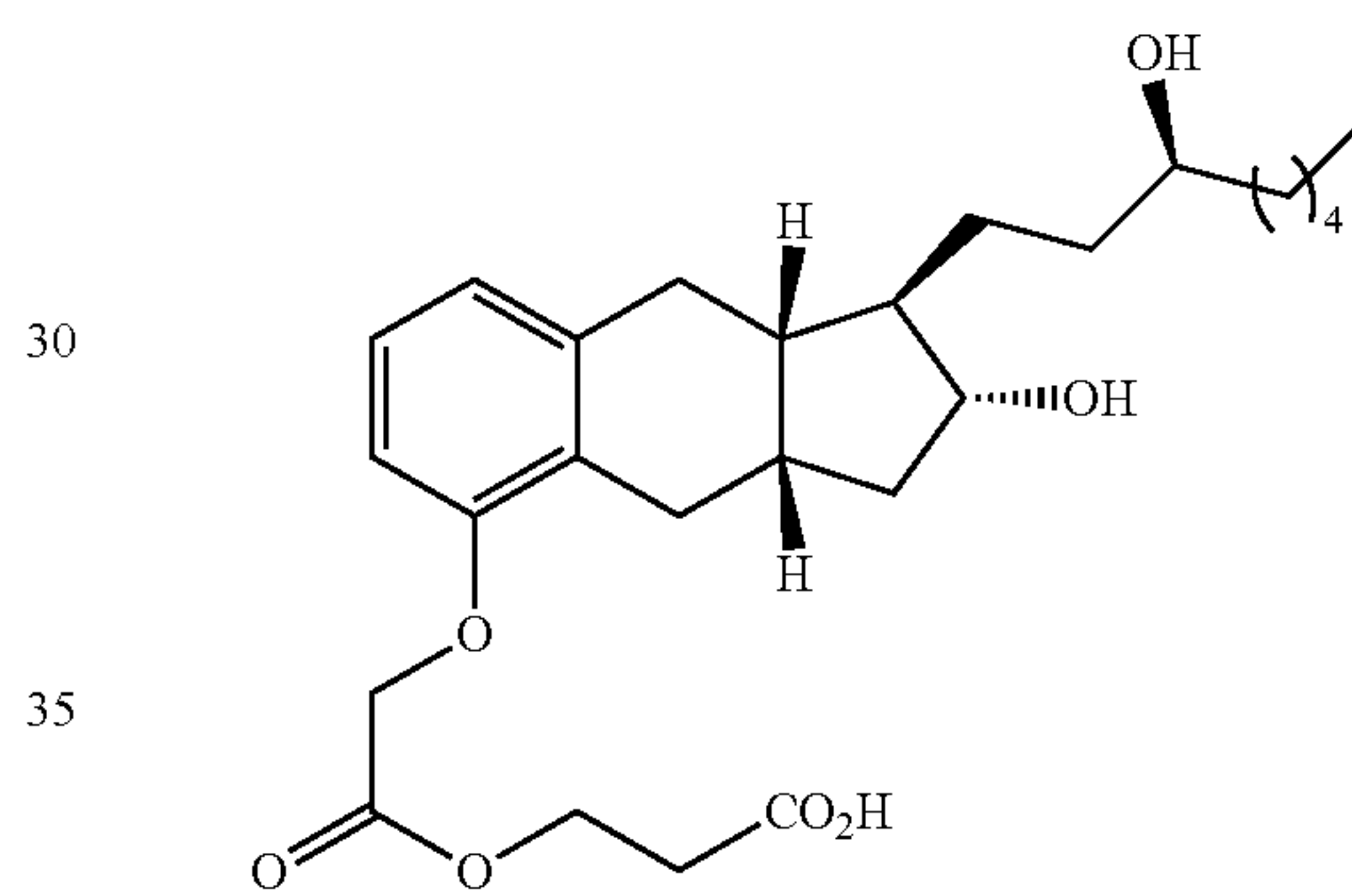
Compound II-24
