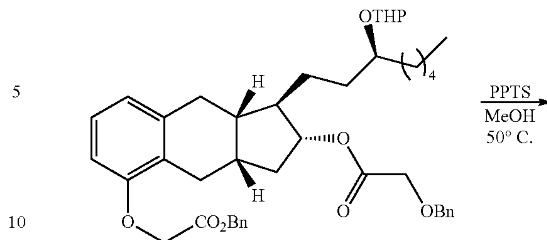
Compound Ia-2
