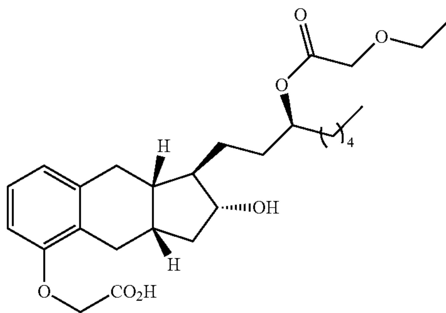
Compound Ib-6
