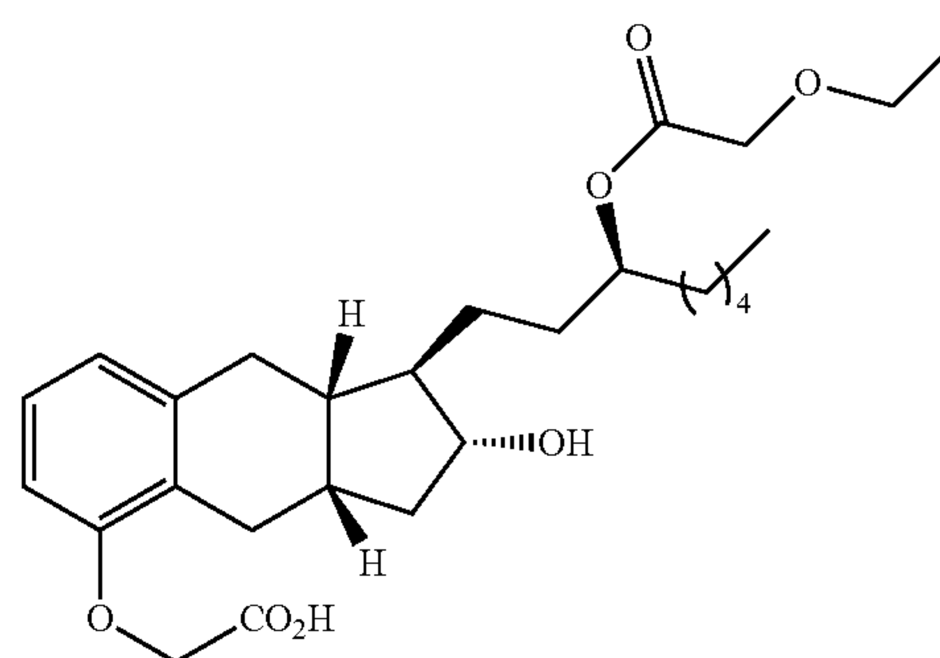
Compound Ib-9
