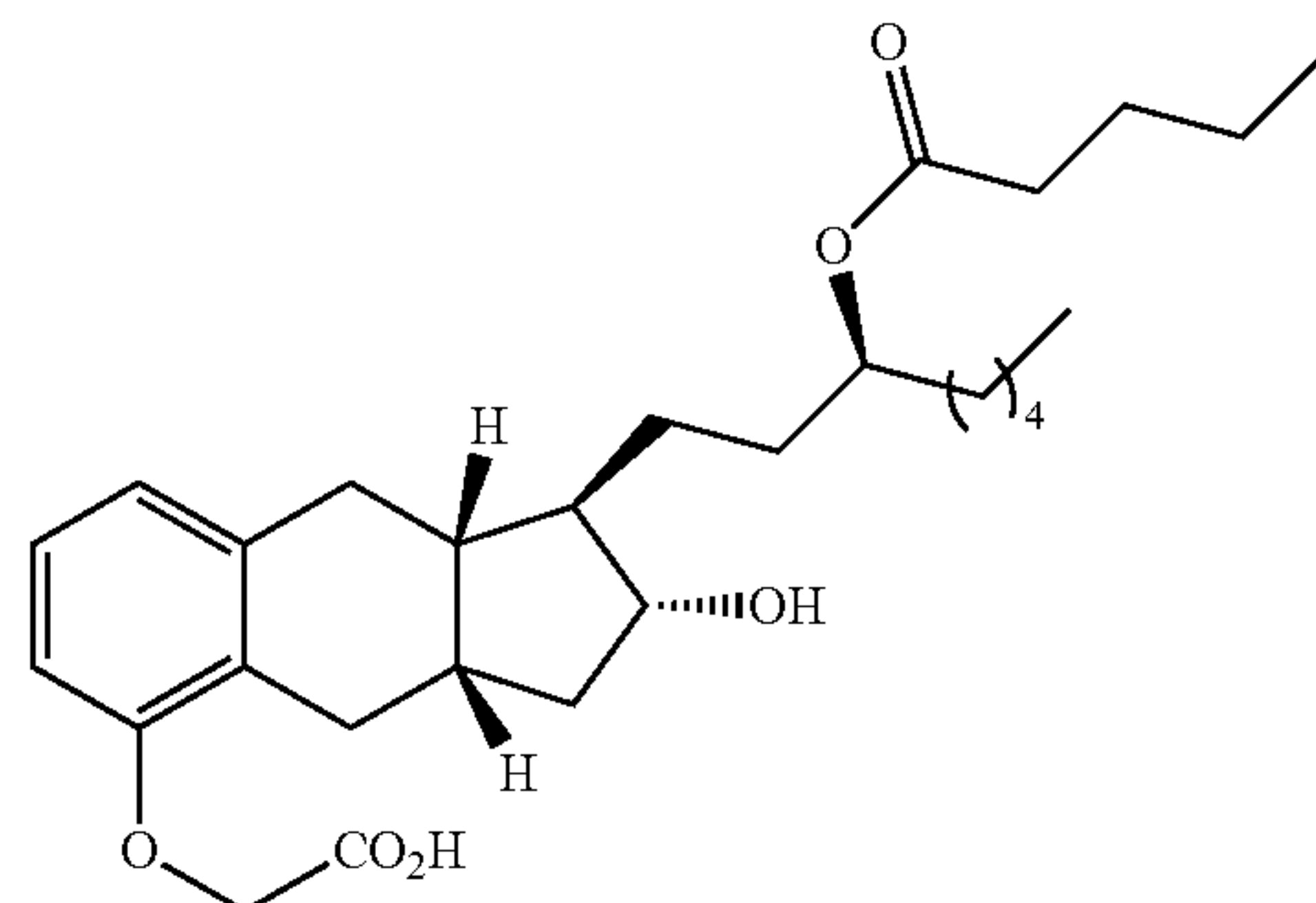
Compound Ib-3
