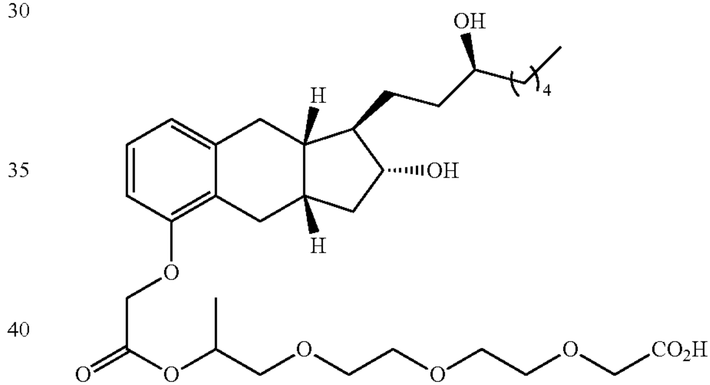
Compound II-18
