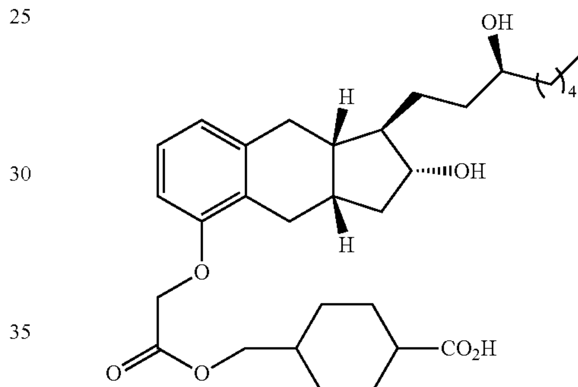
Compound II-23
