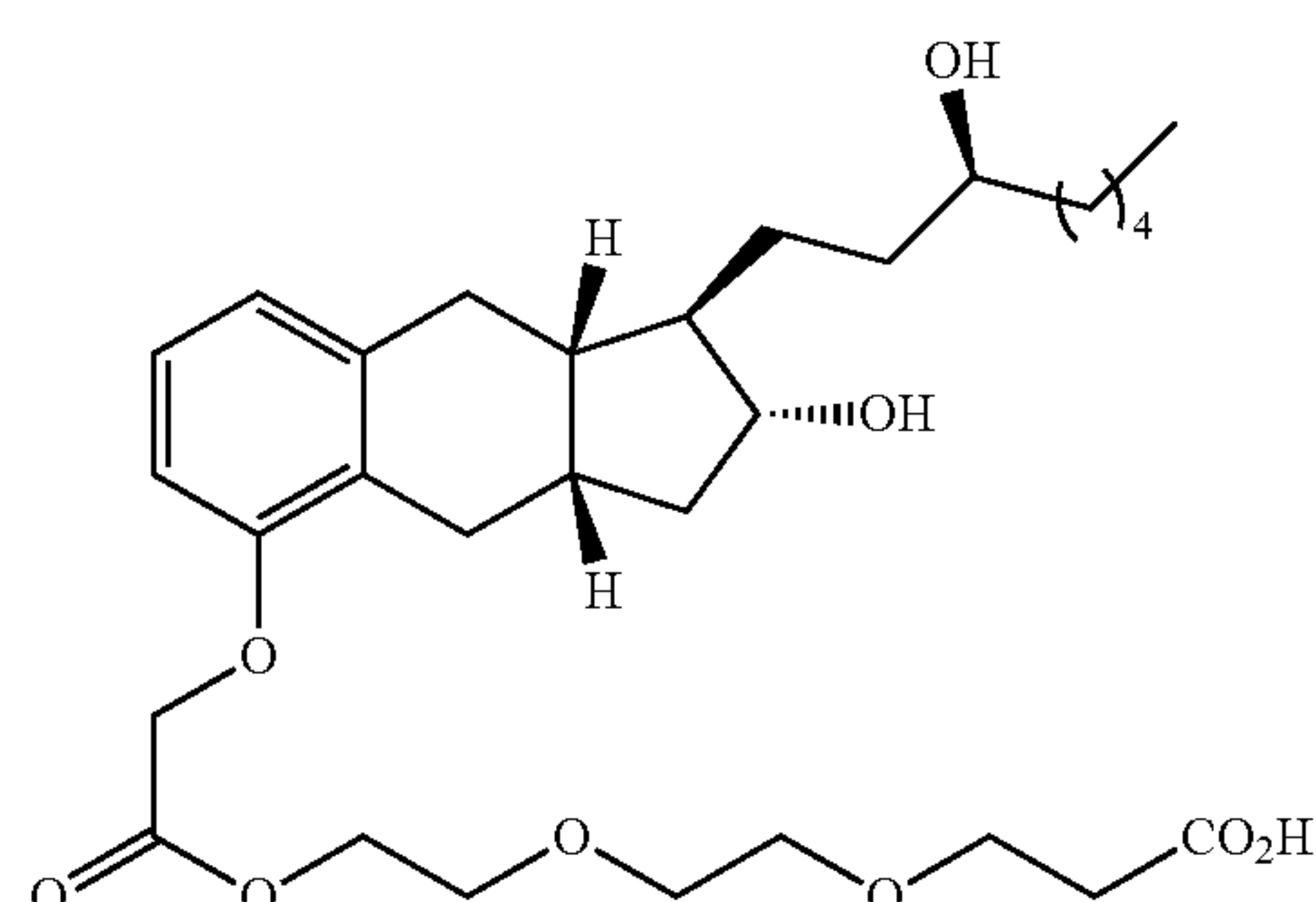
Compound II-19
