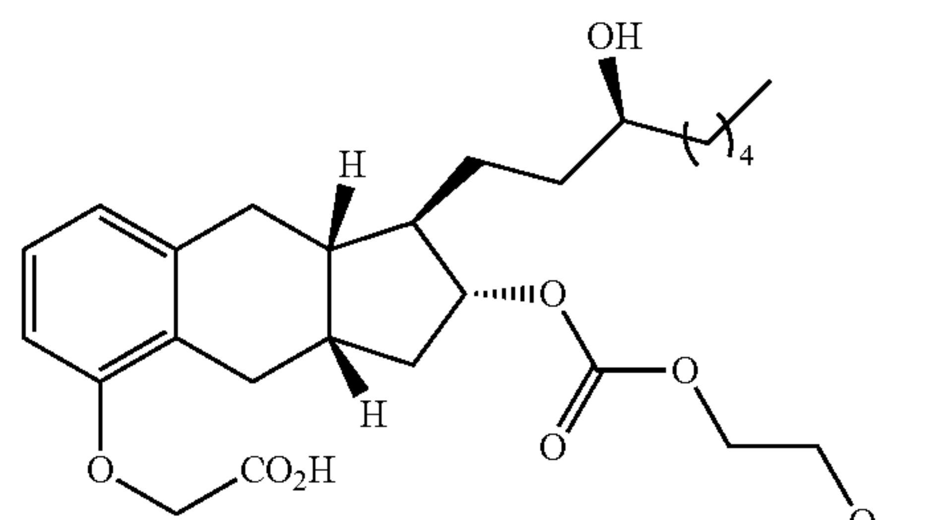
Compound Ib-1
