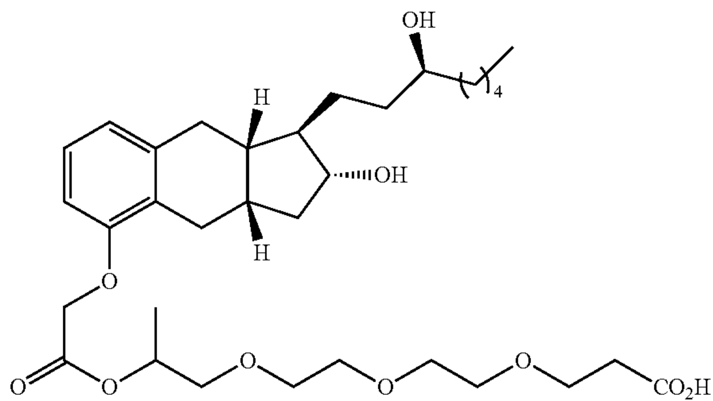
Compound II-20
