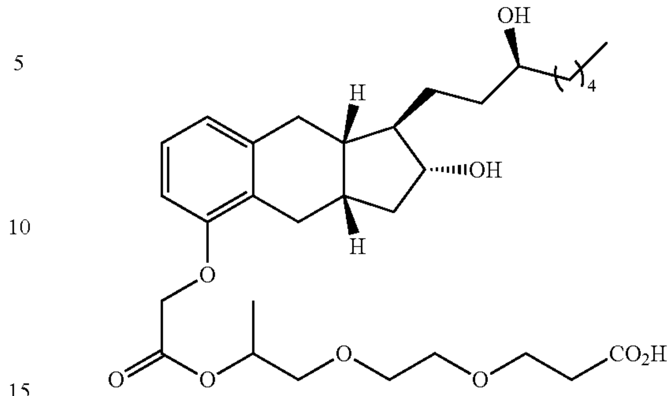
Compound II-20
