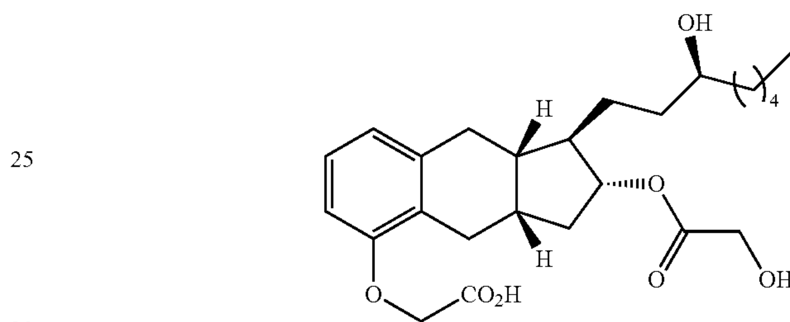
Compound Ia-9
