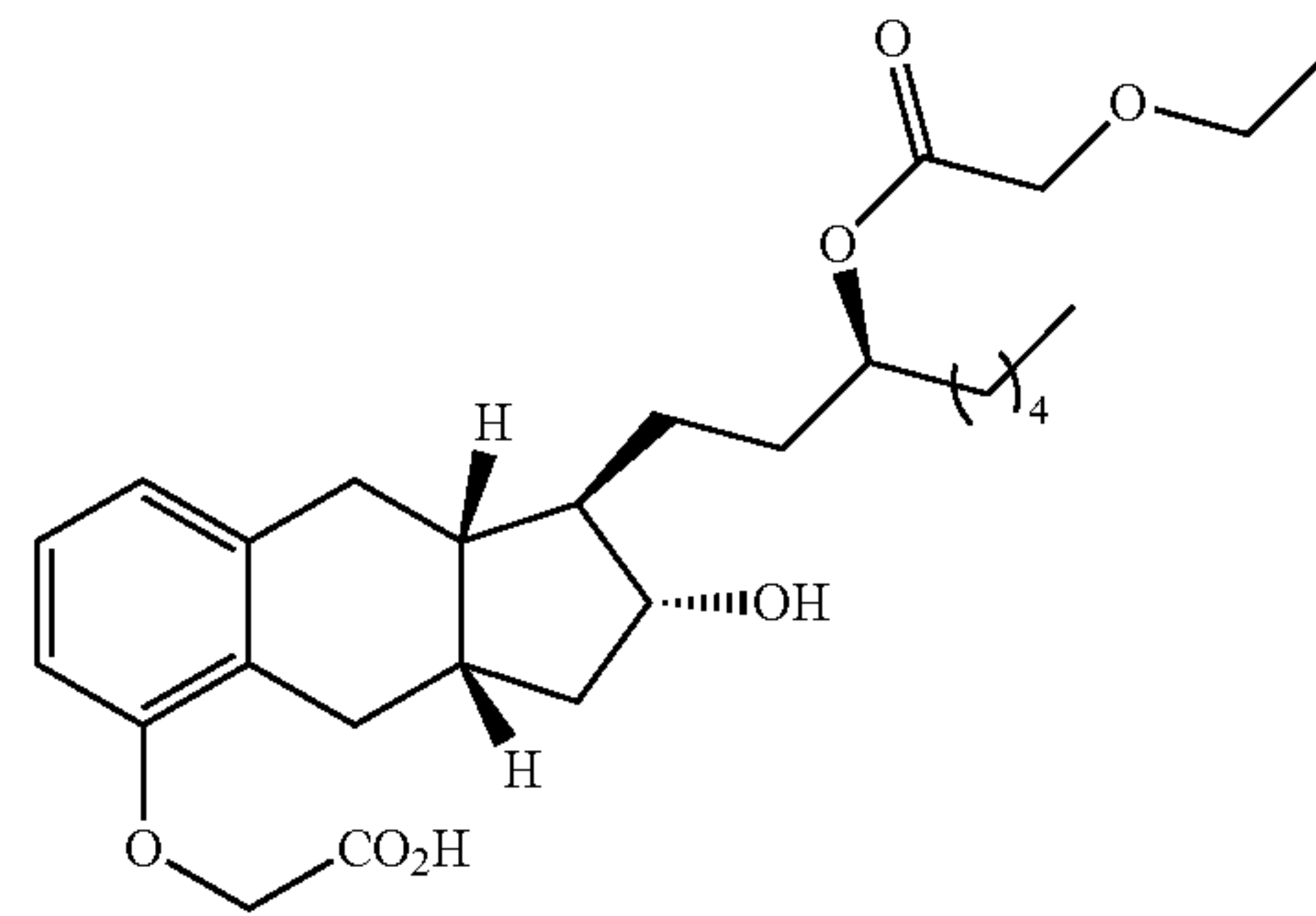
Compound Ib-9
