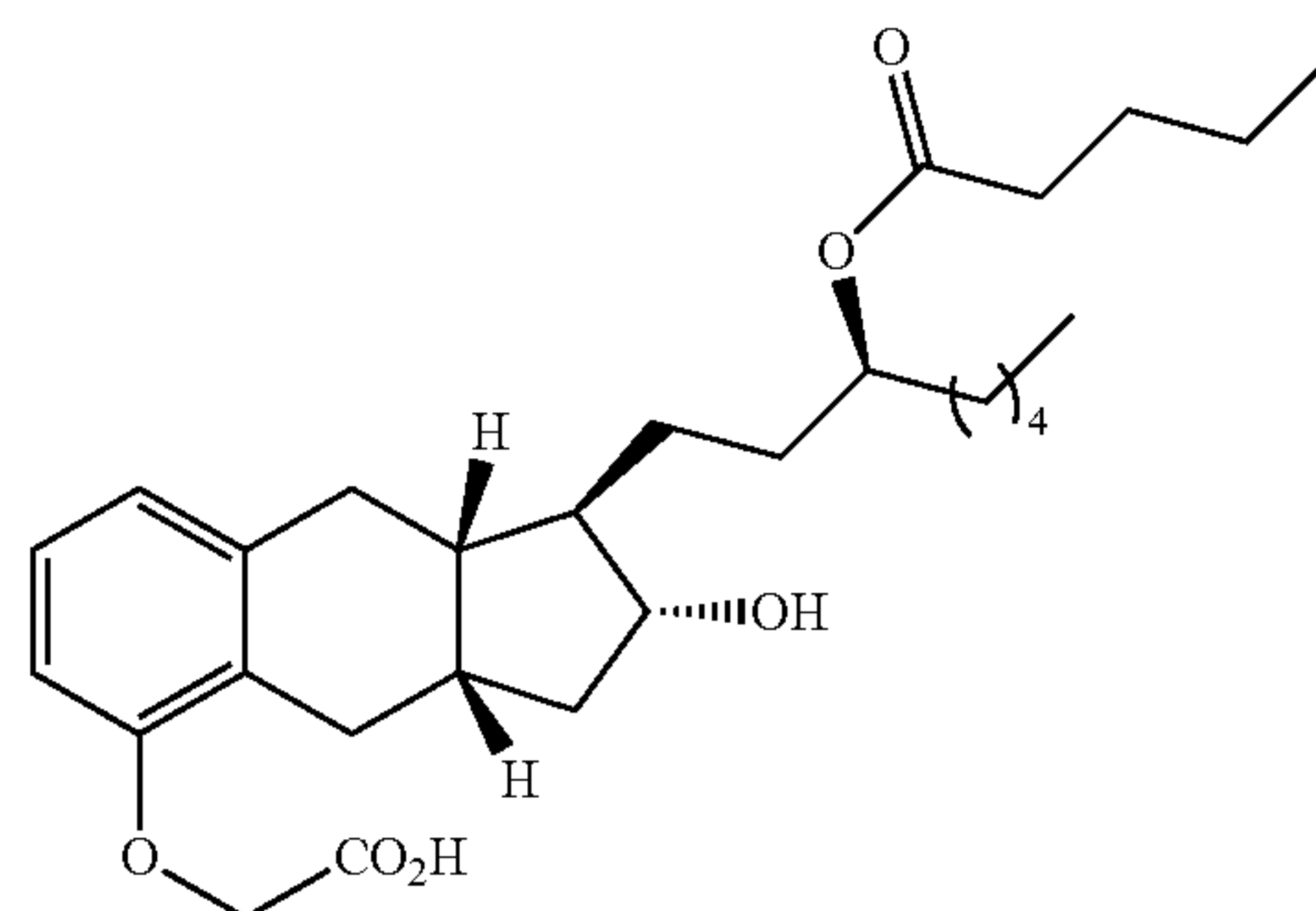
Compound Ib-4
