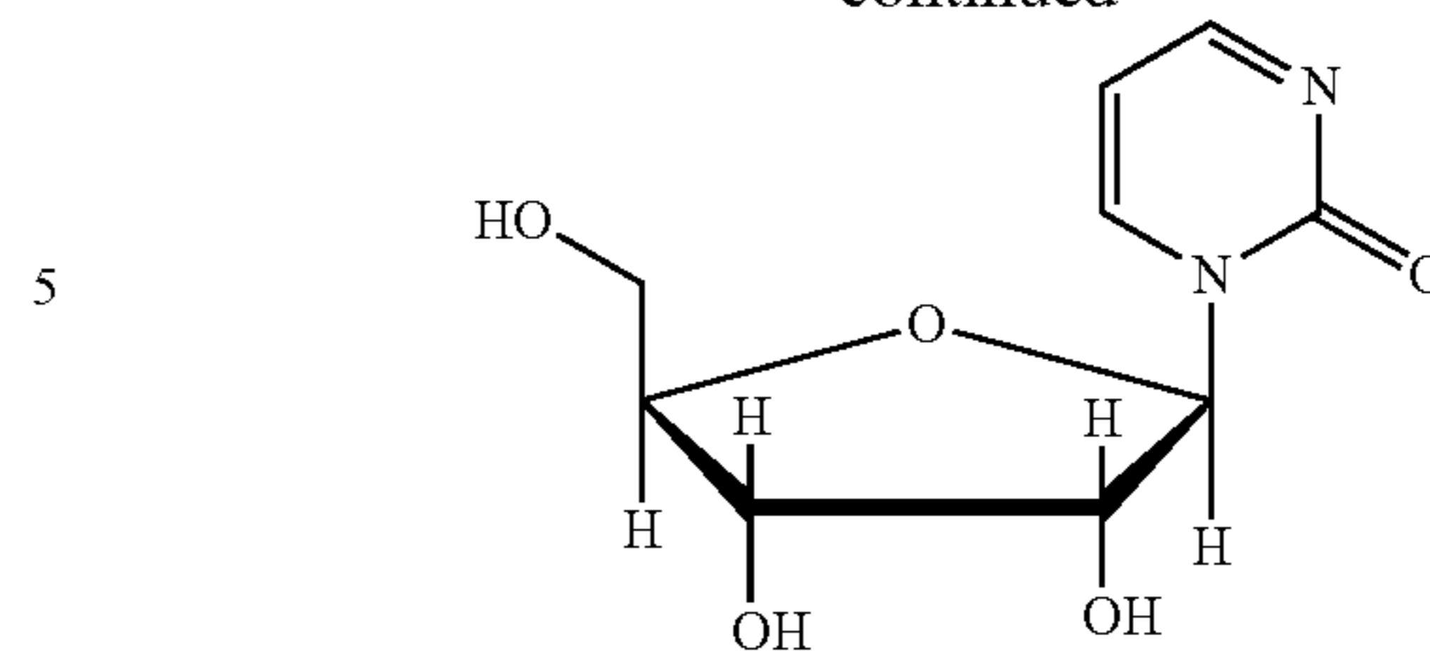
Zebularine
