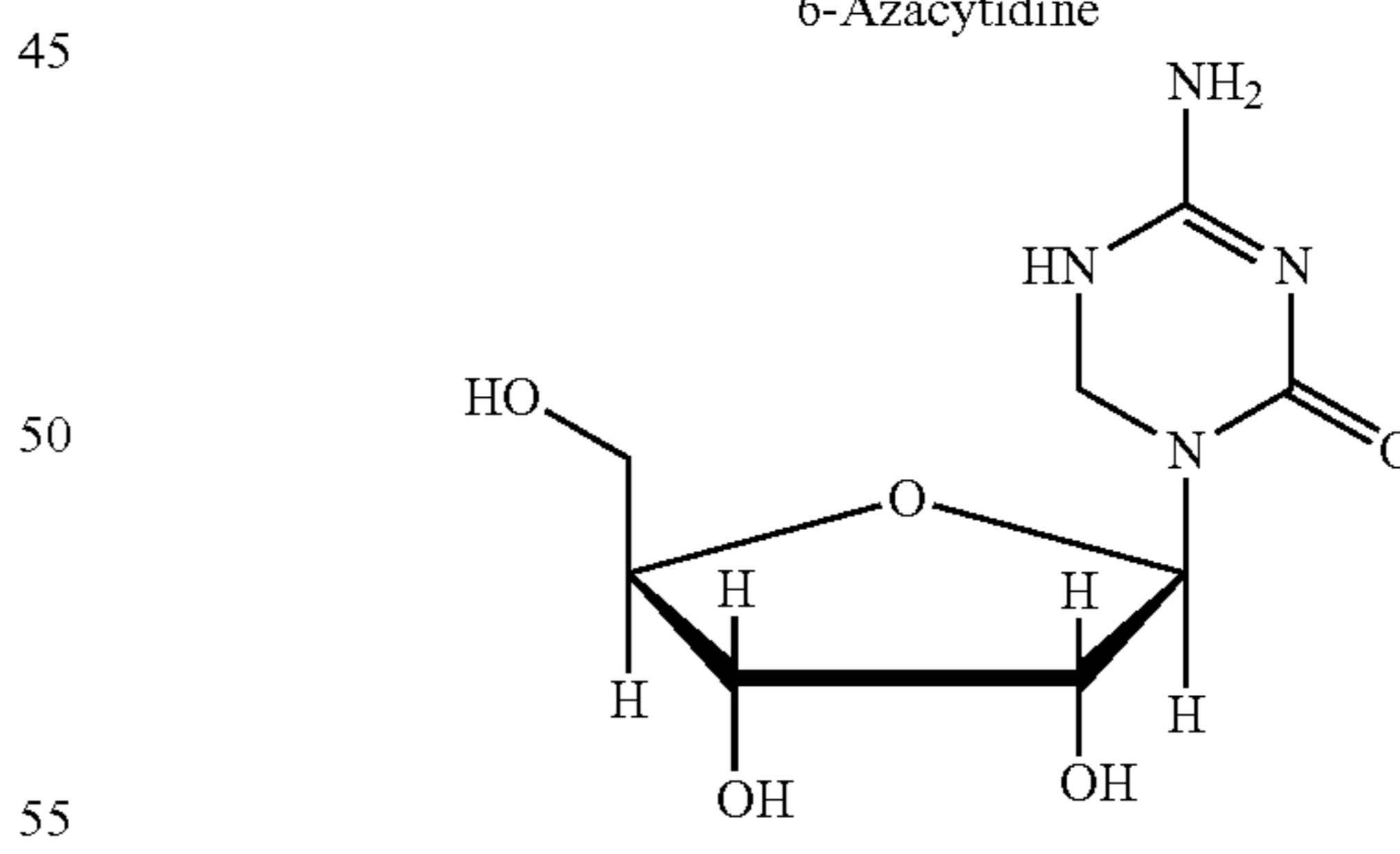
5-6-Dihydro-5-azacytidine
