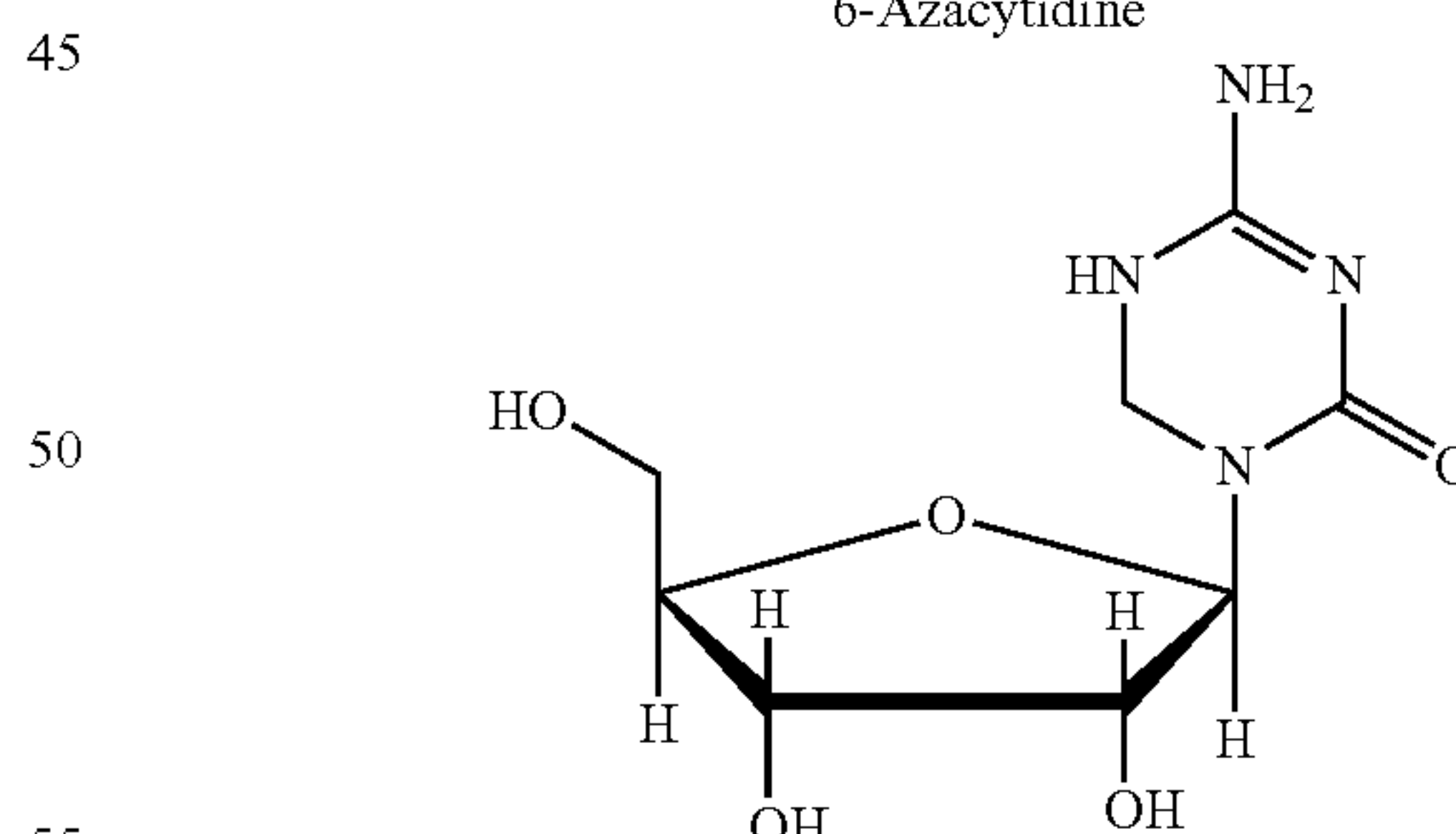
5-6-Dihydro-5-azacytidine
