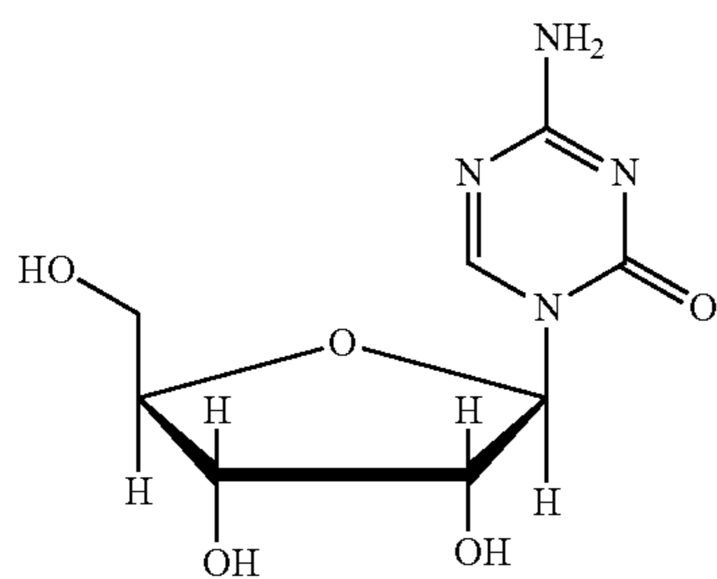
Azacitidine
