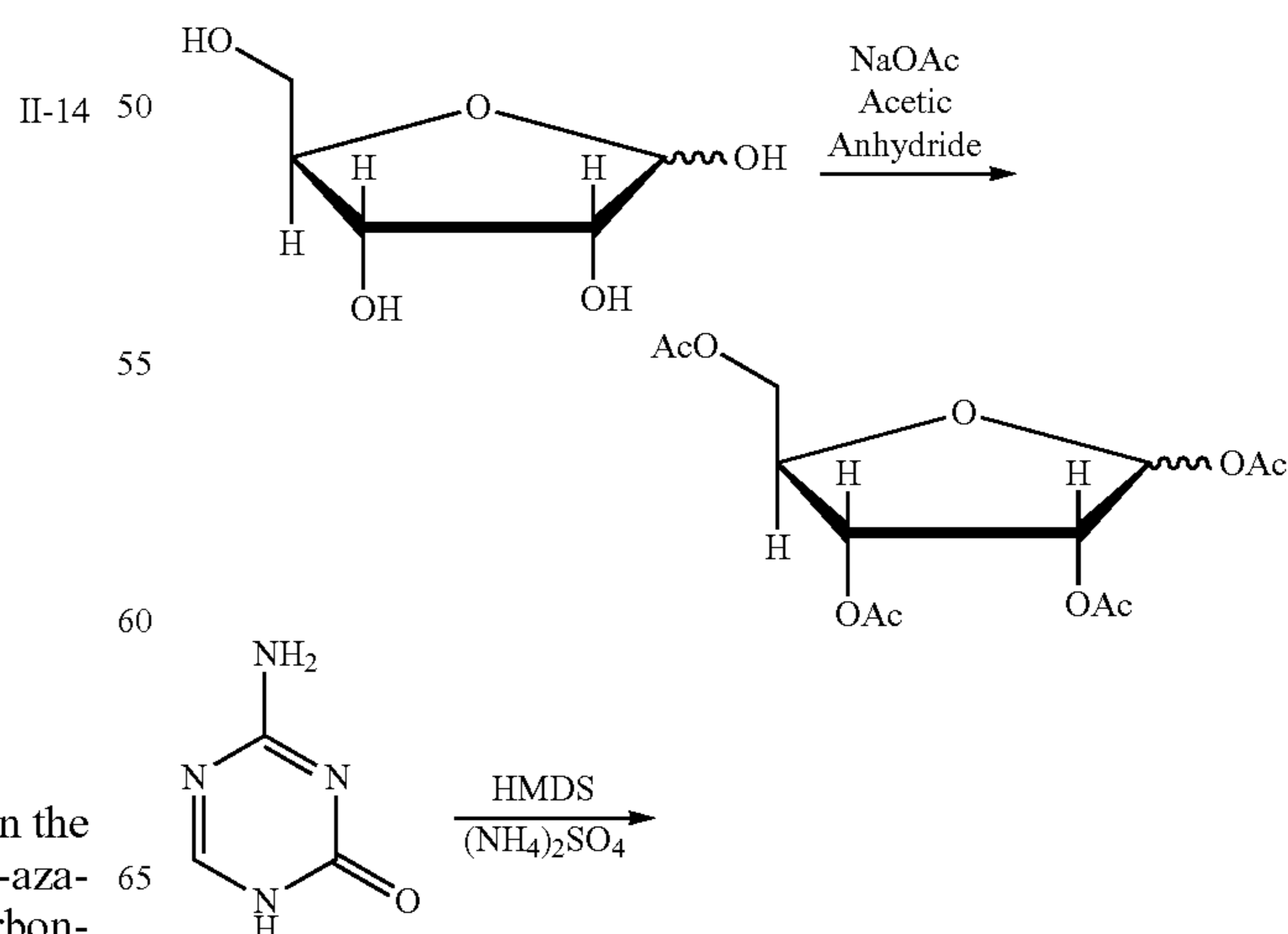
Scheme 1
