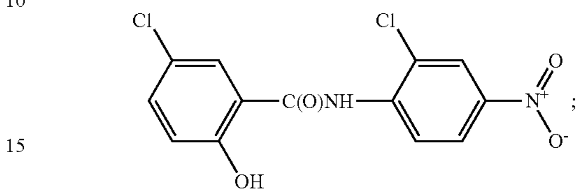
niclosamide
