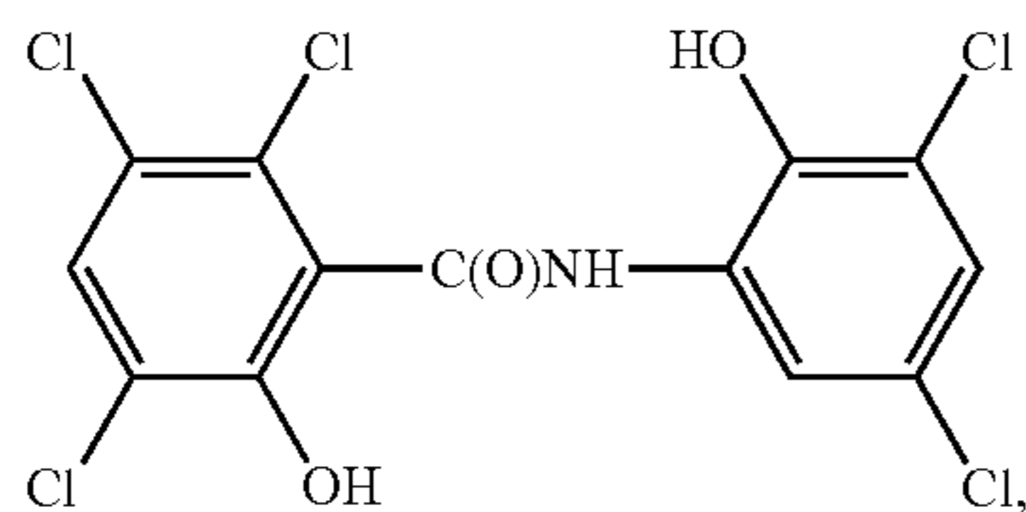
oxyclosanide
