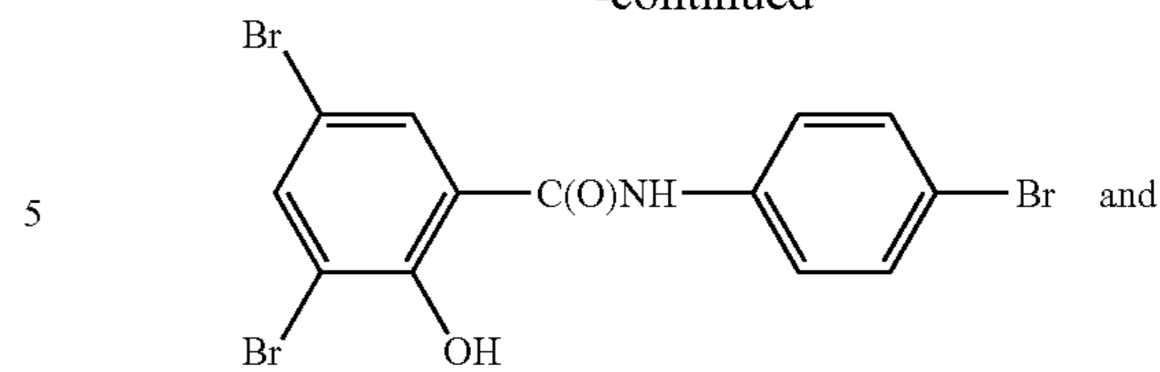
Tribromosalicylanilide
