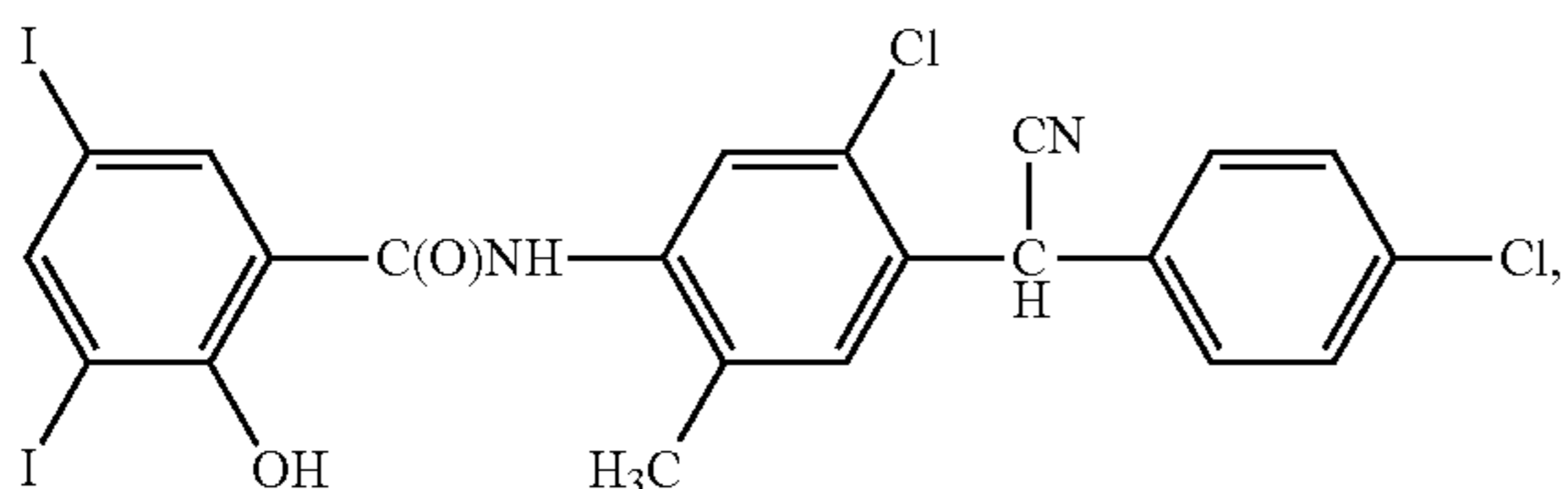
closantel
