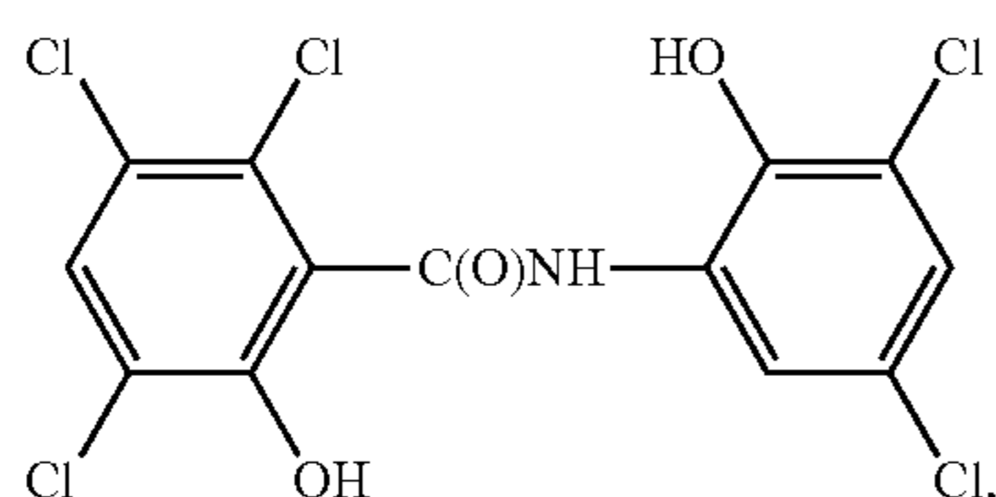
oxyclozanide
