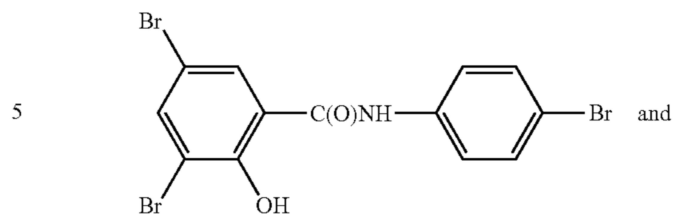
tribromosalalan
