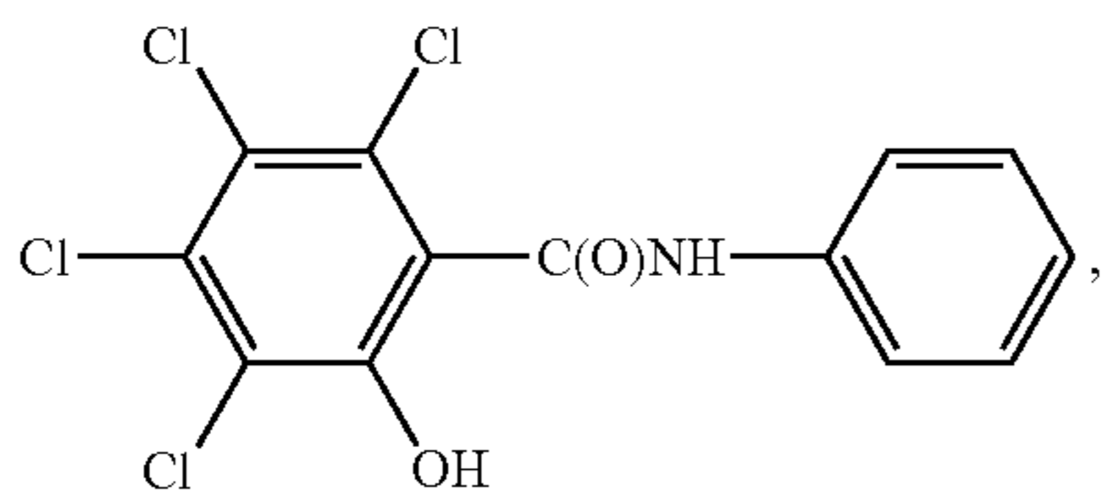
tetrachlorosalicylanilide
