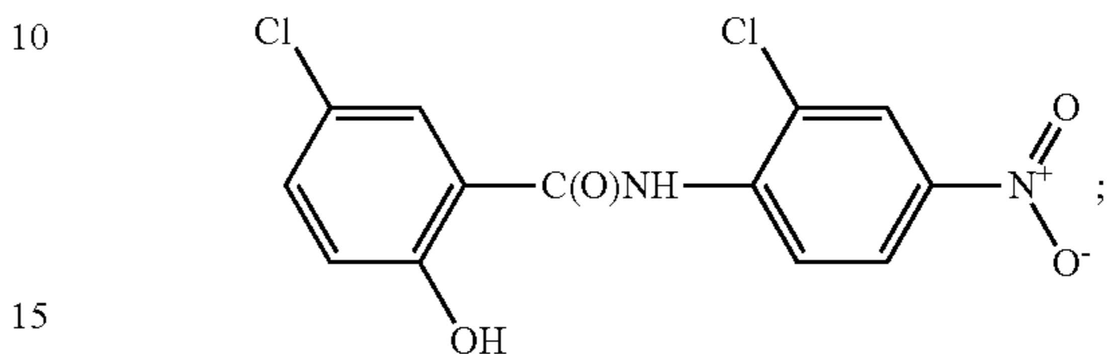
Niclosamine
