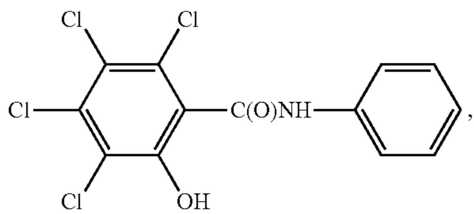
tetrachlorosalicylanilide
