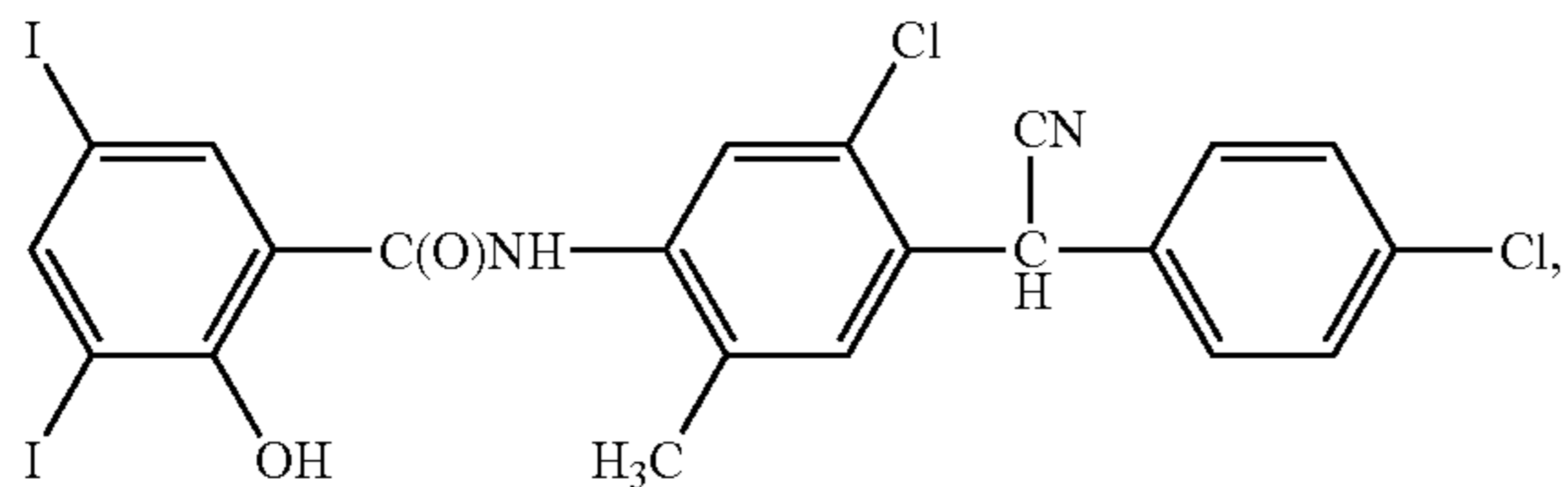
Closantel
