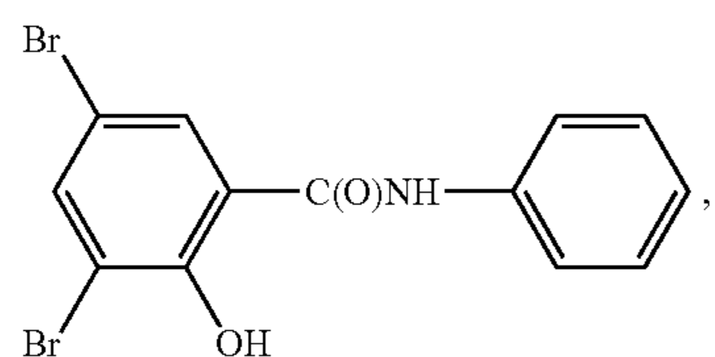
Dibromosalicylanilide
