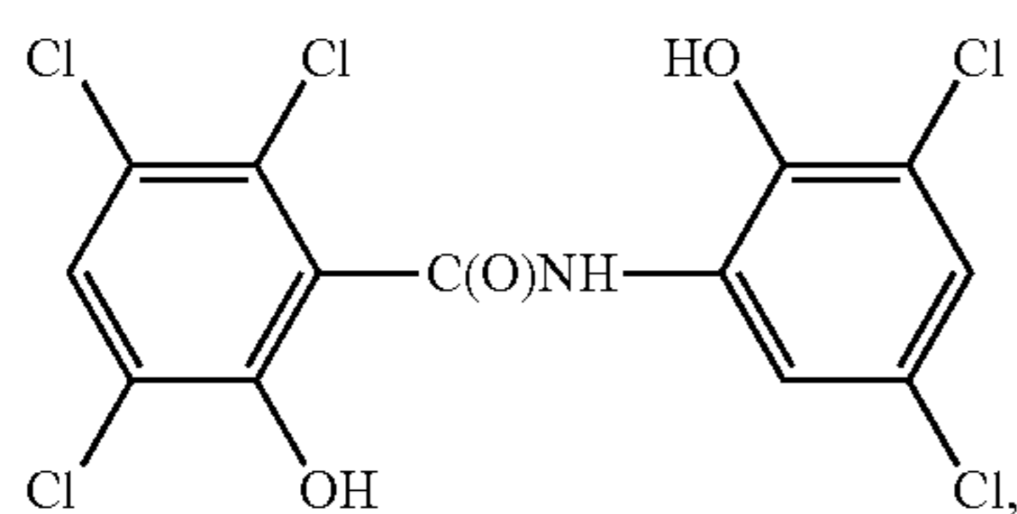
oxyclosanide
