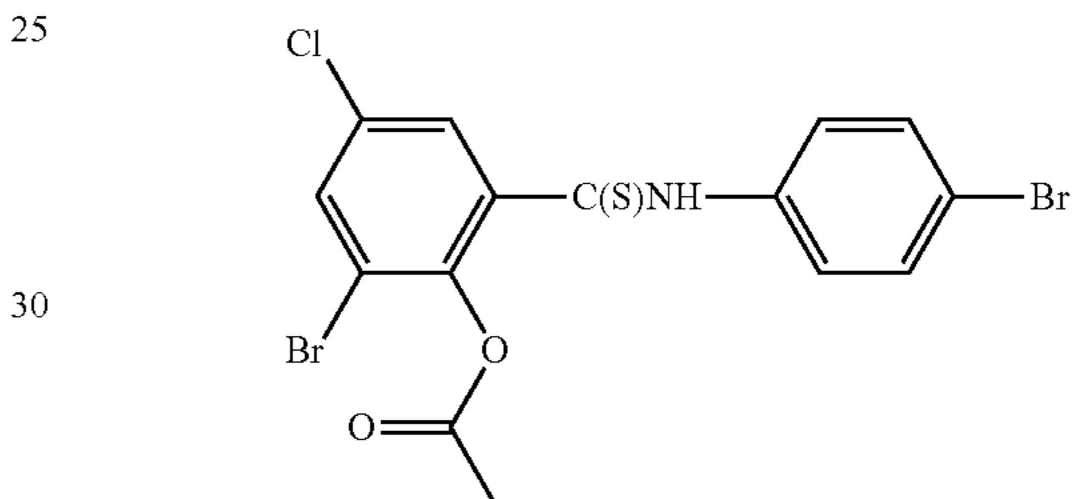
brotianide
