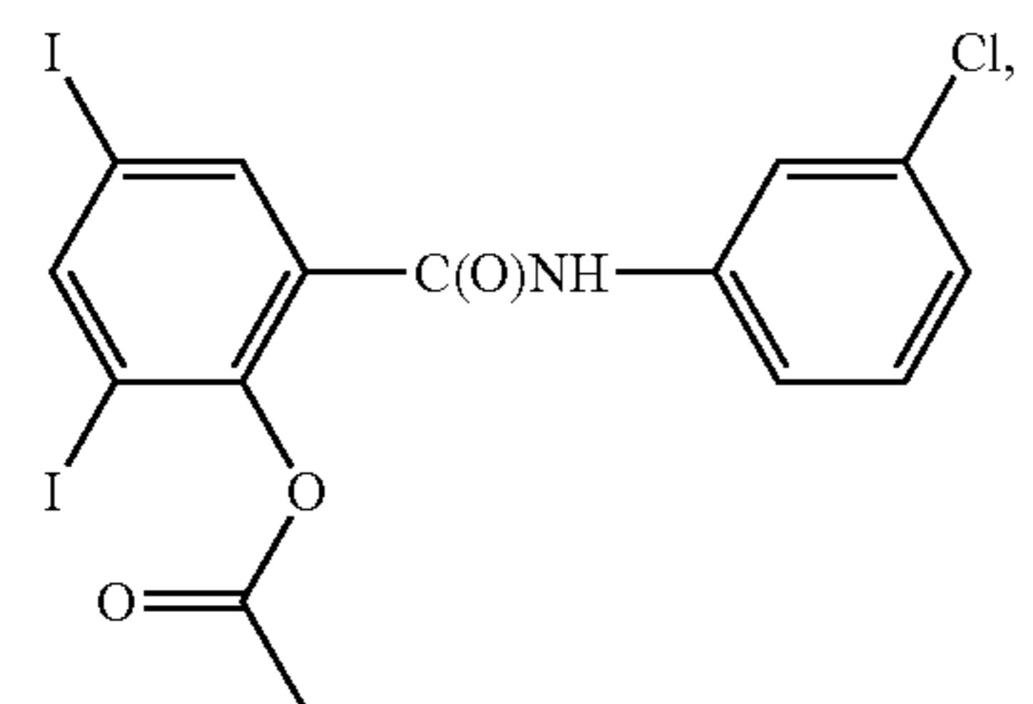
Clioquinone
