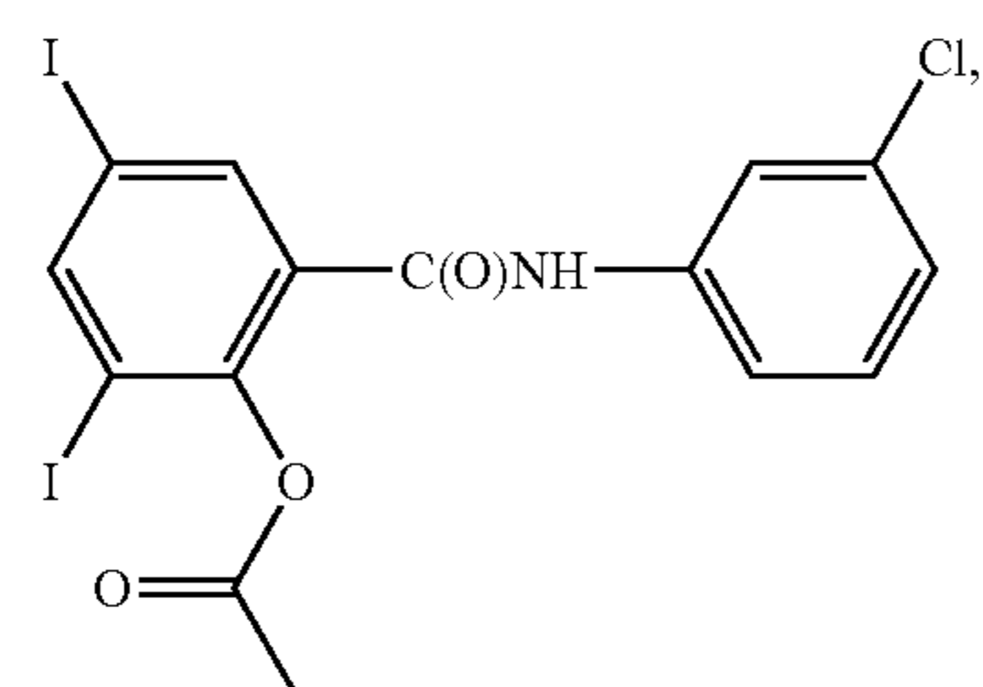
Clioquinone
