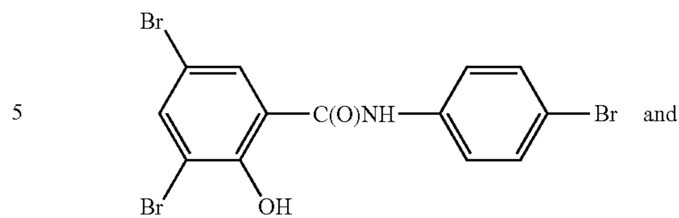
tribromosalalan
