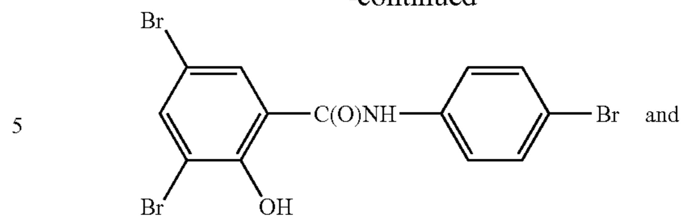
Tribromosalicylanilide
