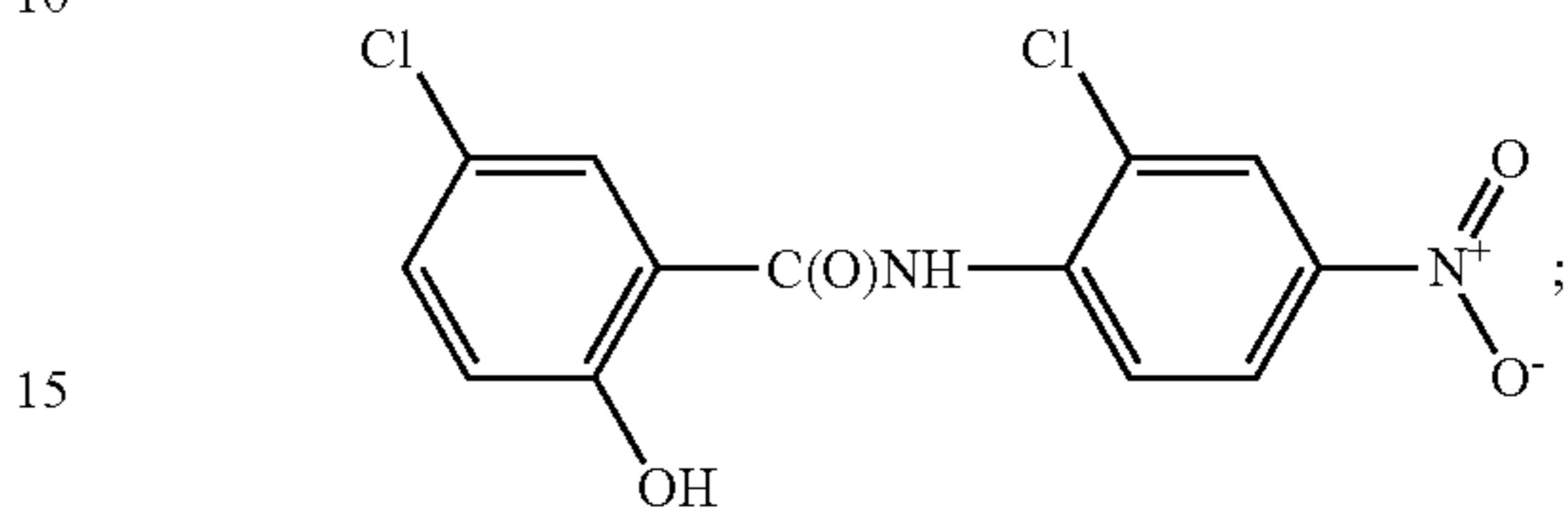
niclosamide
