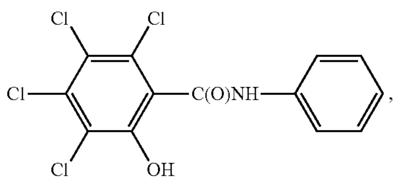
tetrachlorosalicylanilide
