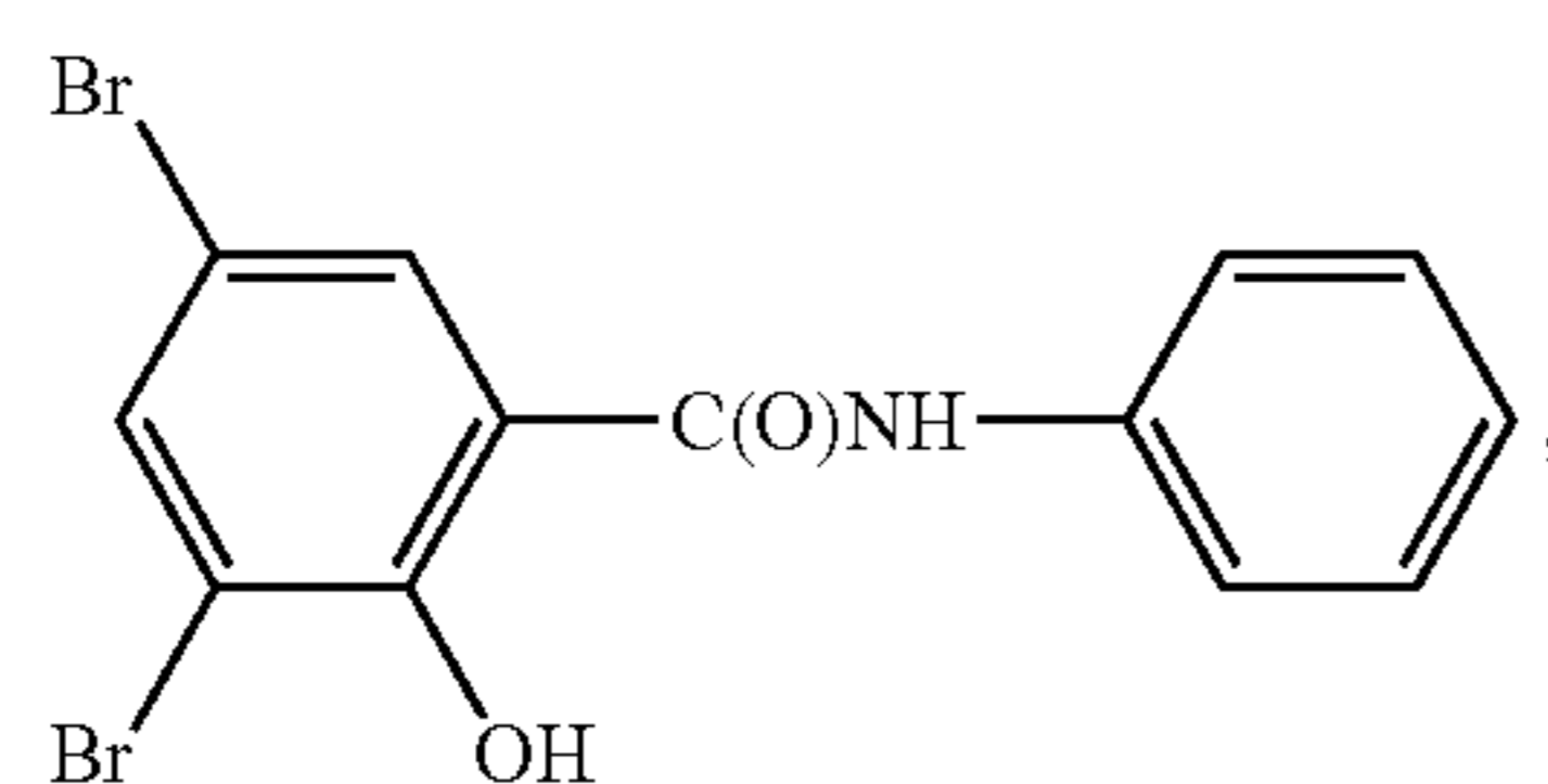
Dibromosalicylanilide
