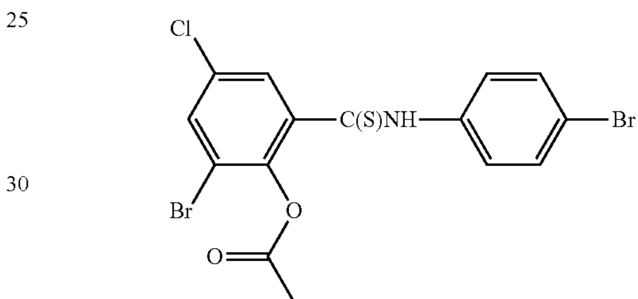
brotianide
