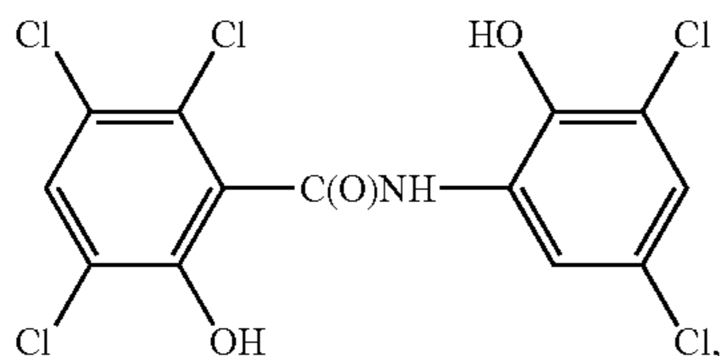
oxyclosanide
