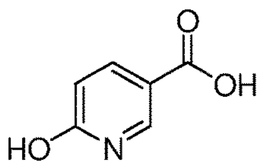
6-hydroxynicotinic acid
