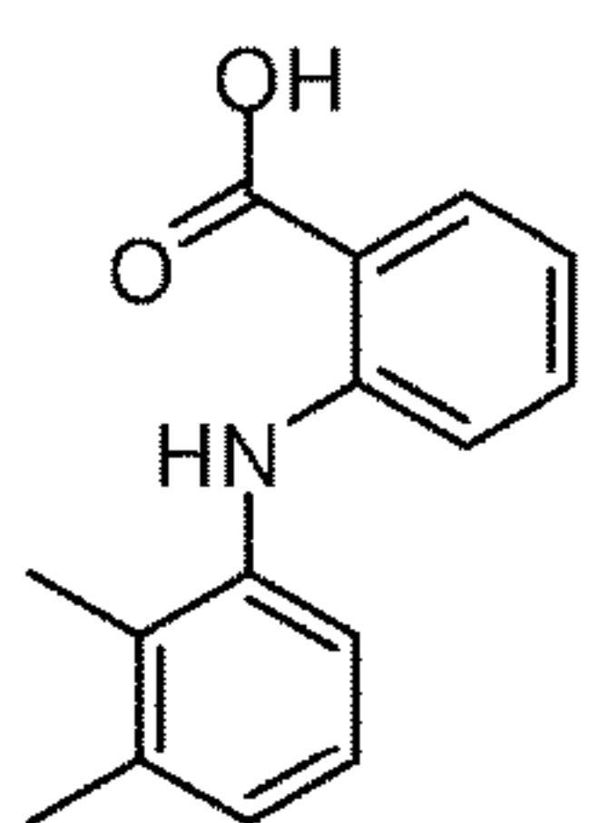
Mefenamic acid
