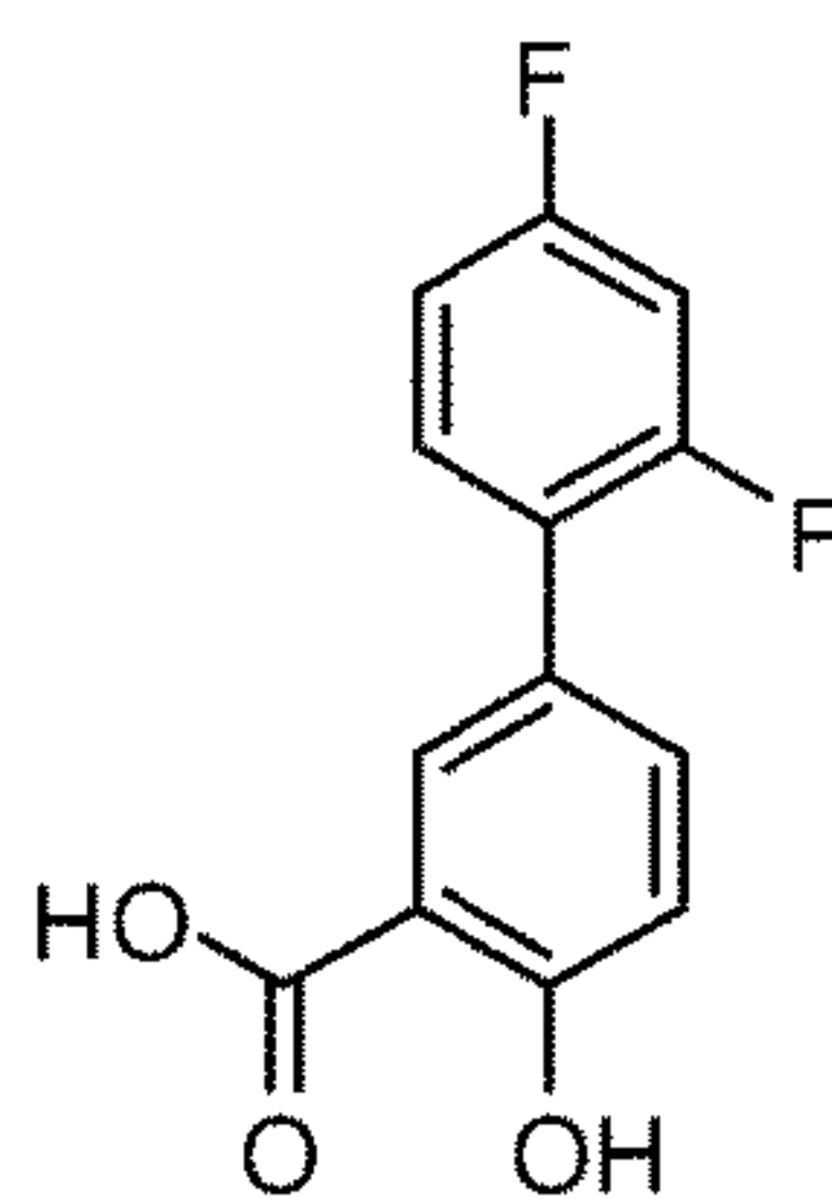
Diflusalal
