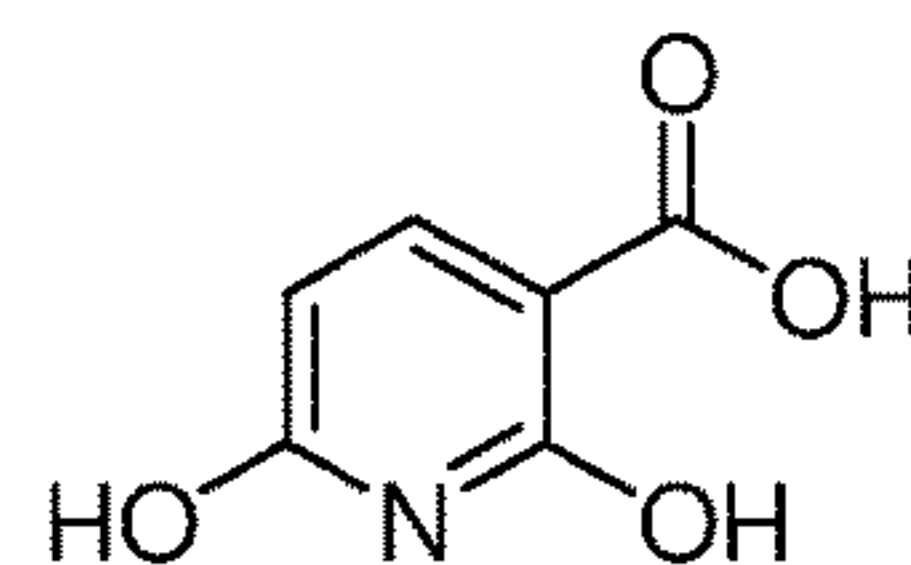
2,6-dihydroxynicotinic acid
