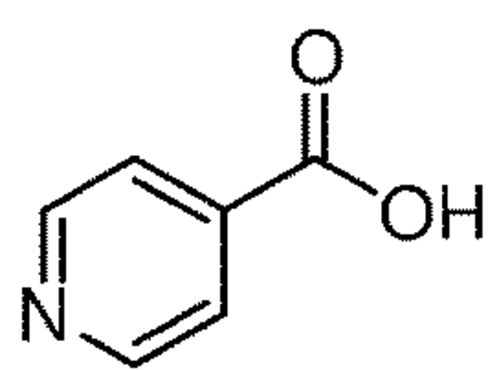
isonicotinic acid
