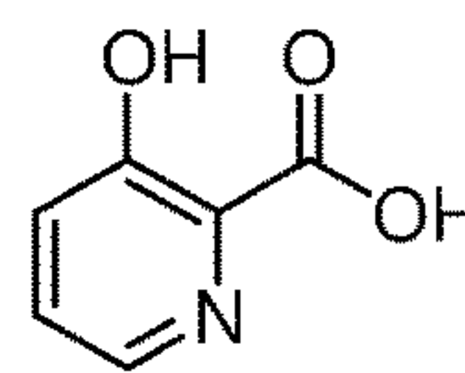
3-hydroxypicolinic acid
