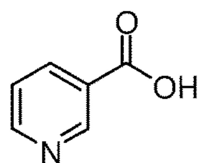
nicotinic acid
