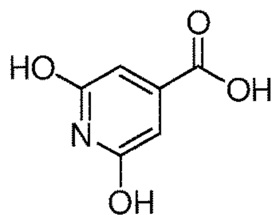
citrazinic acid
