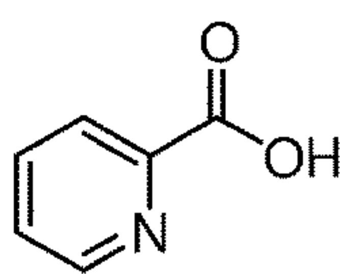
picolinic acid
