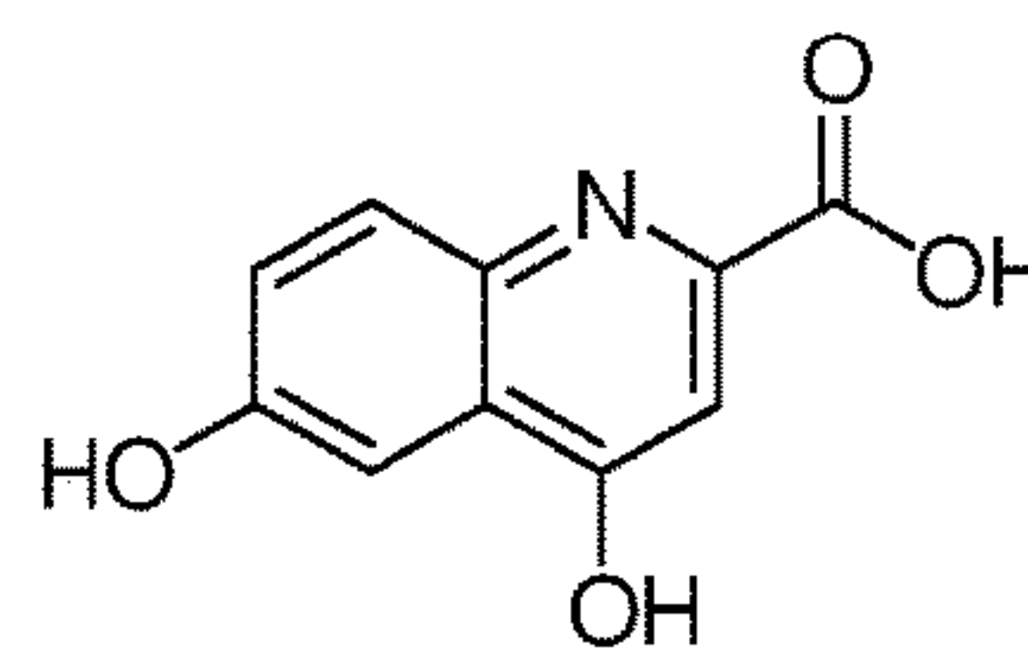
6-hydroxykynurenic acid
