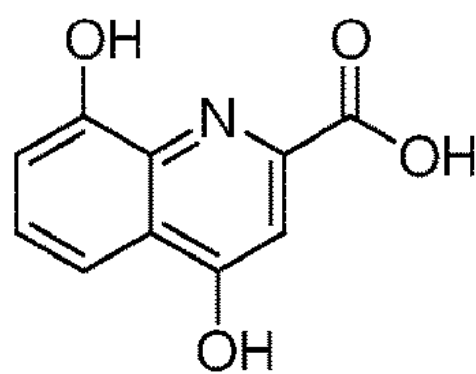
xanthurenic acid
