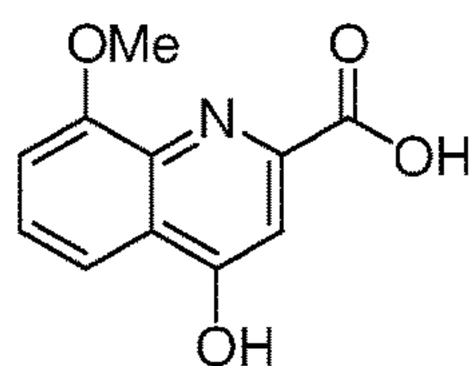
8-methoxykynurenic acid
