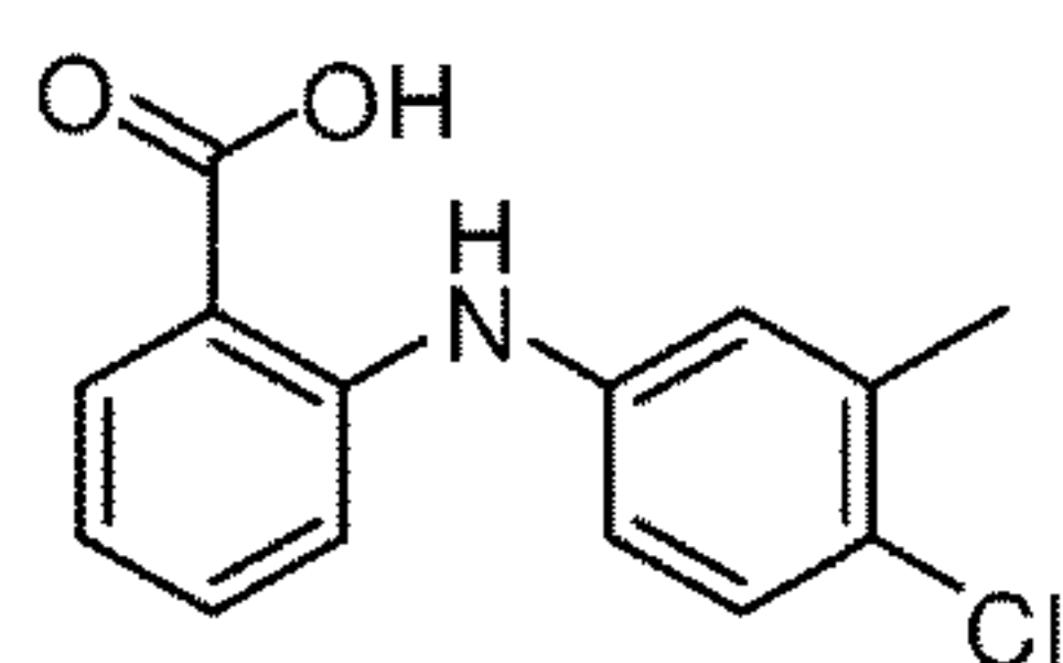
Tolfenamic acid
