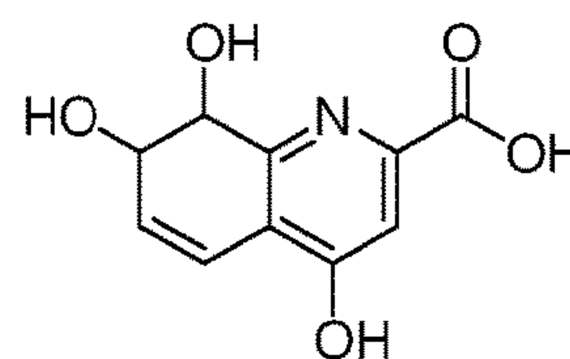
7,8-dihydro-7,8-dihydroxykynurenic acid
