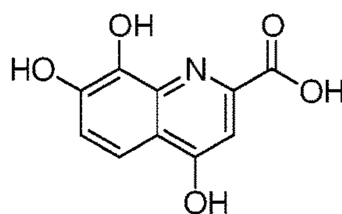
7,8-dihydroxykynurenic acid
