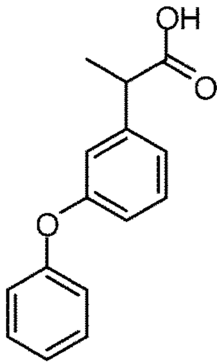
Fenoprofen
