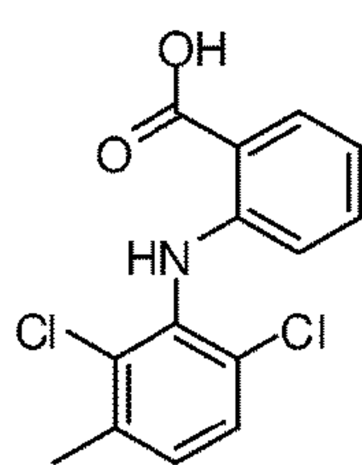
Meclofenamic acid
