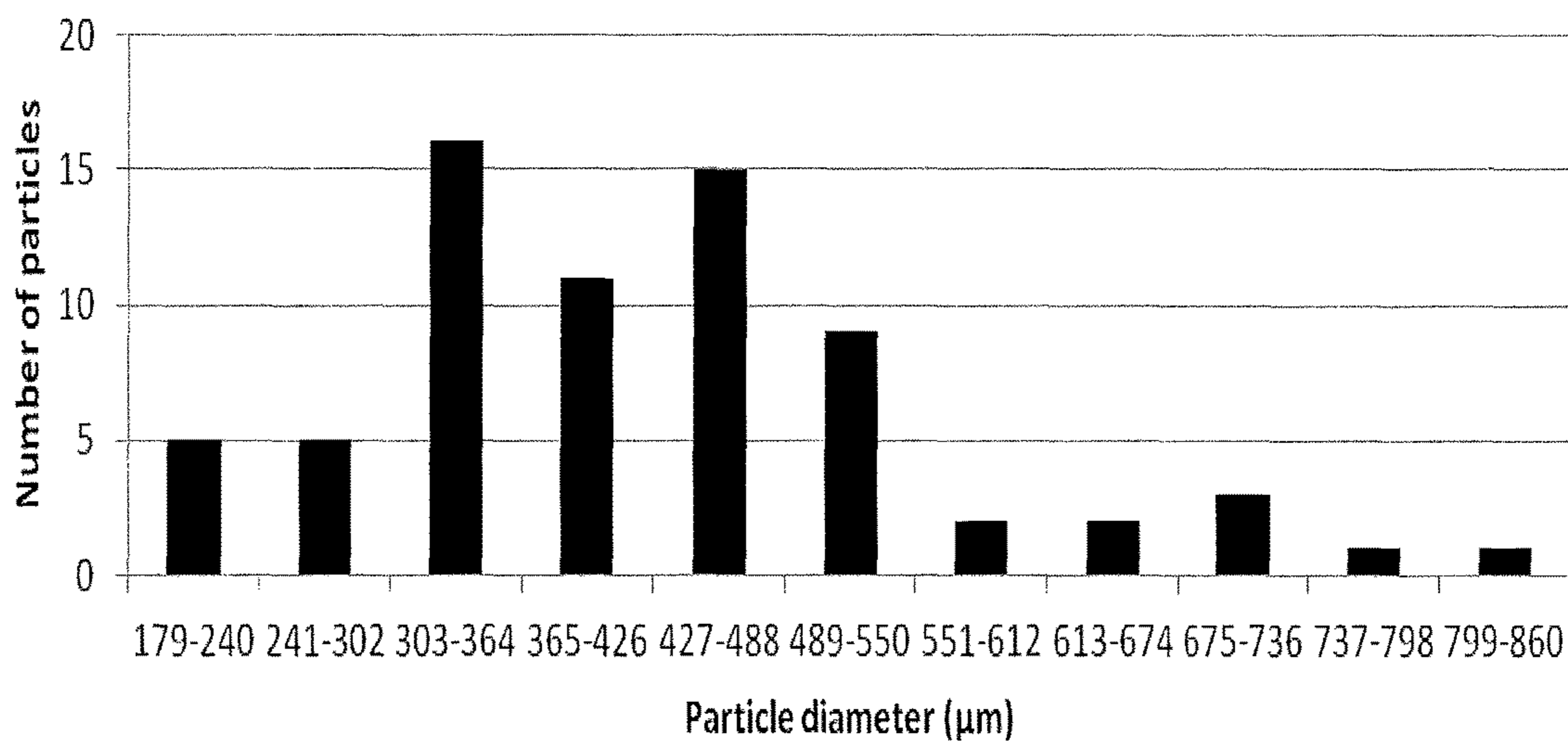
Figure 7. Particle Distribution for Formulation 4 Extended Release Formulation
