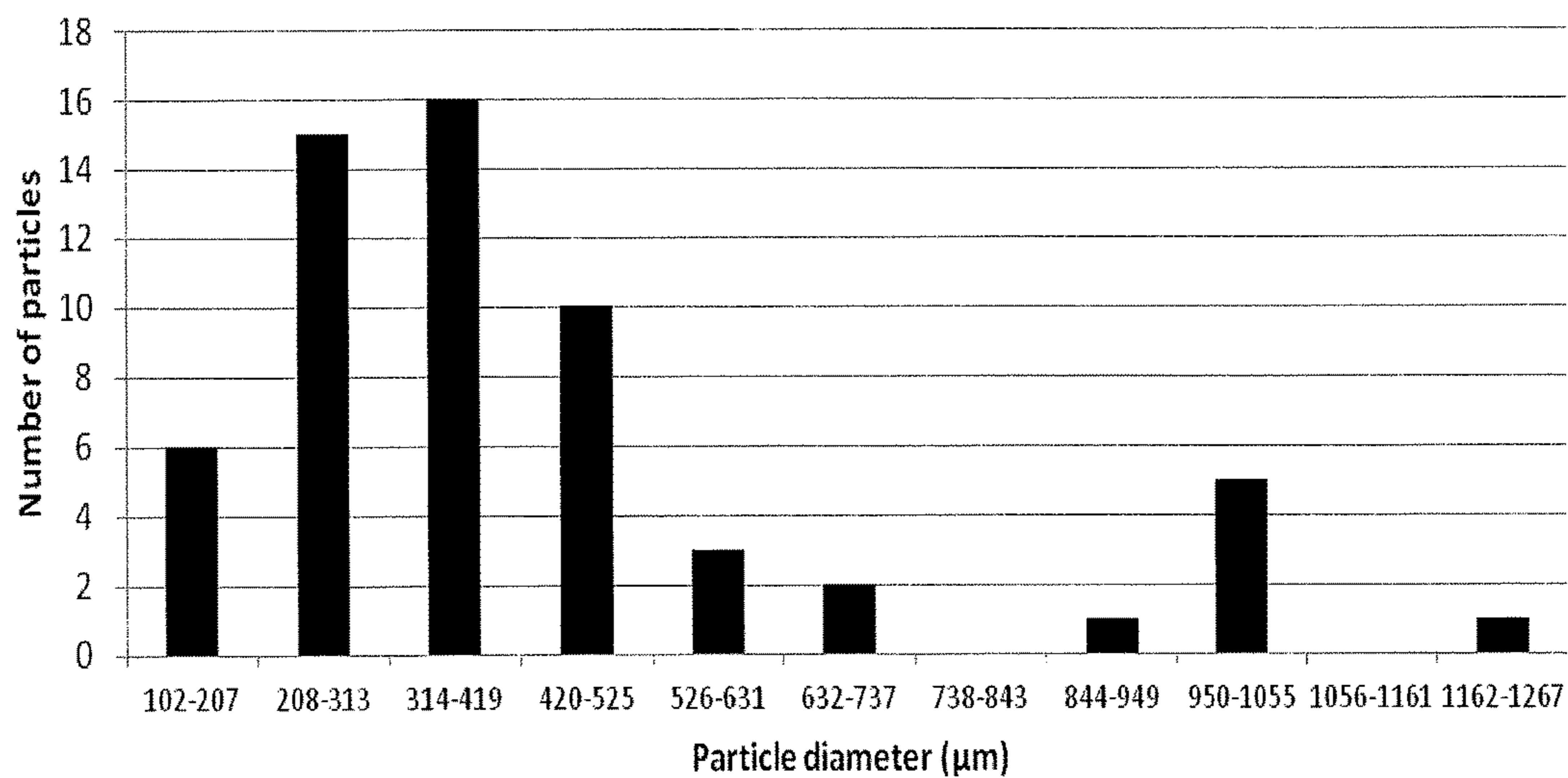
Figure 6. Particle Distribution for Formulation 2 Extended Release Formulation
