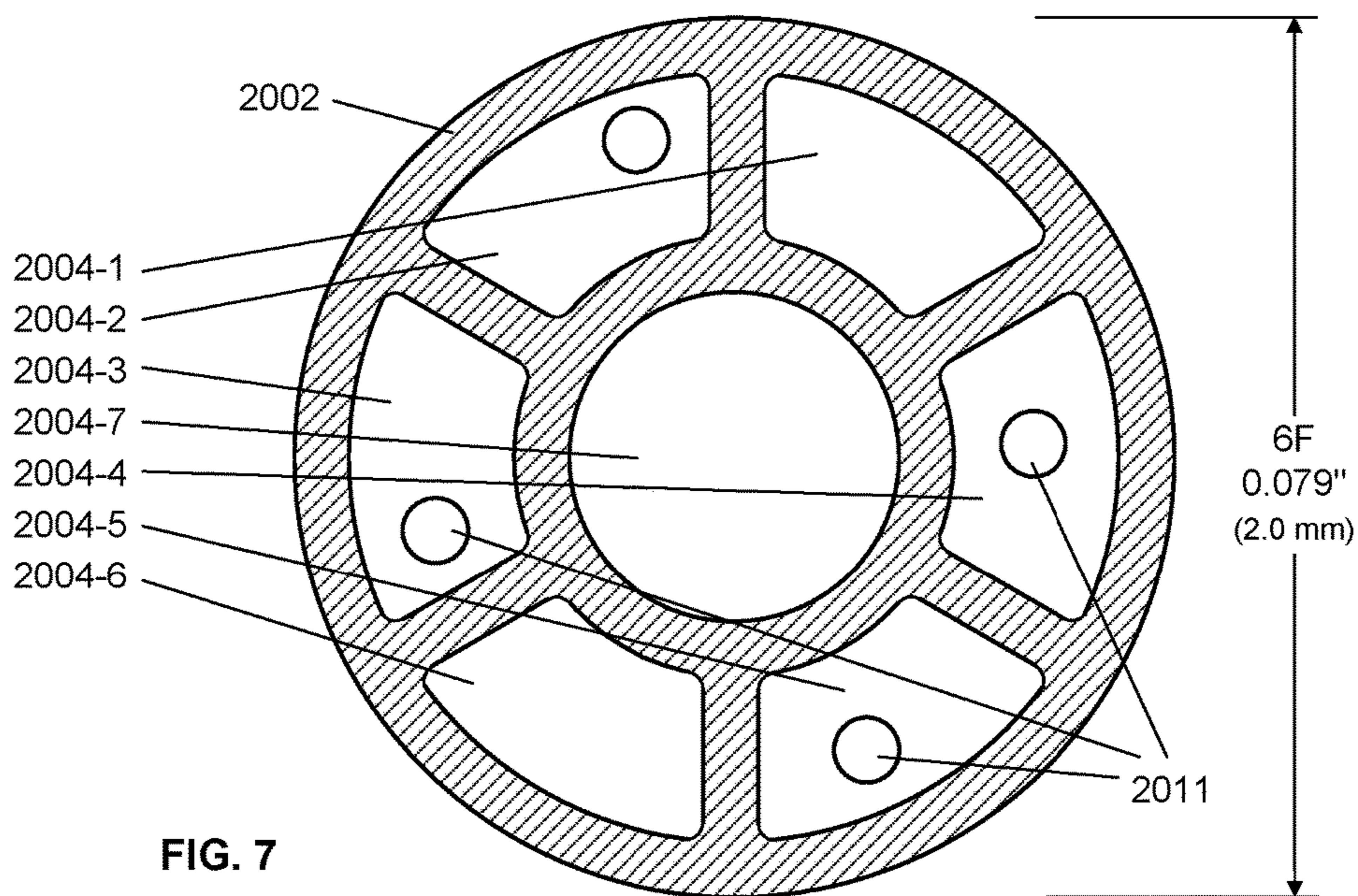
A-A CUT-THROUGH VIEW OF FIGS. 5, 6 AND 9
