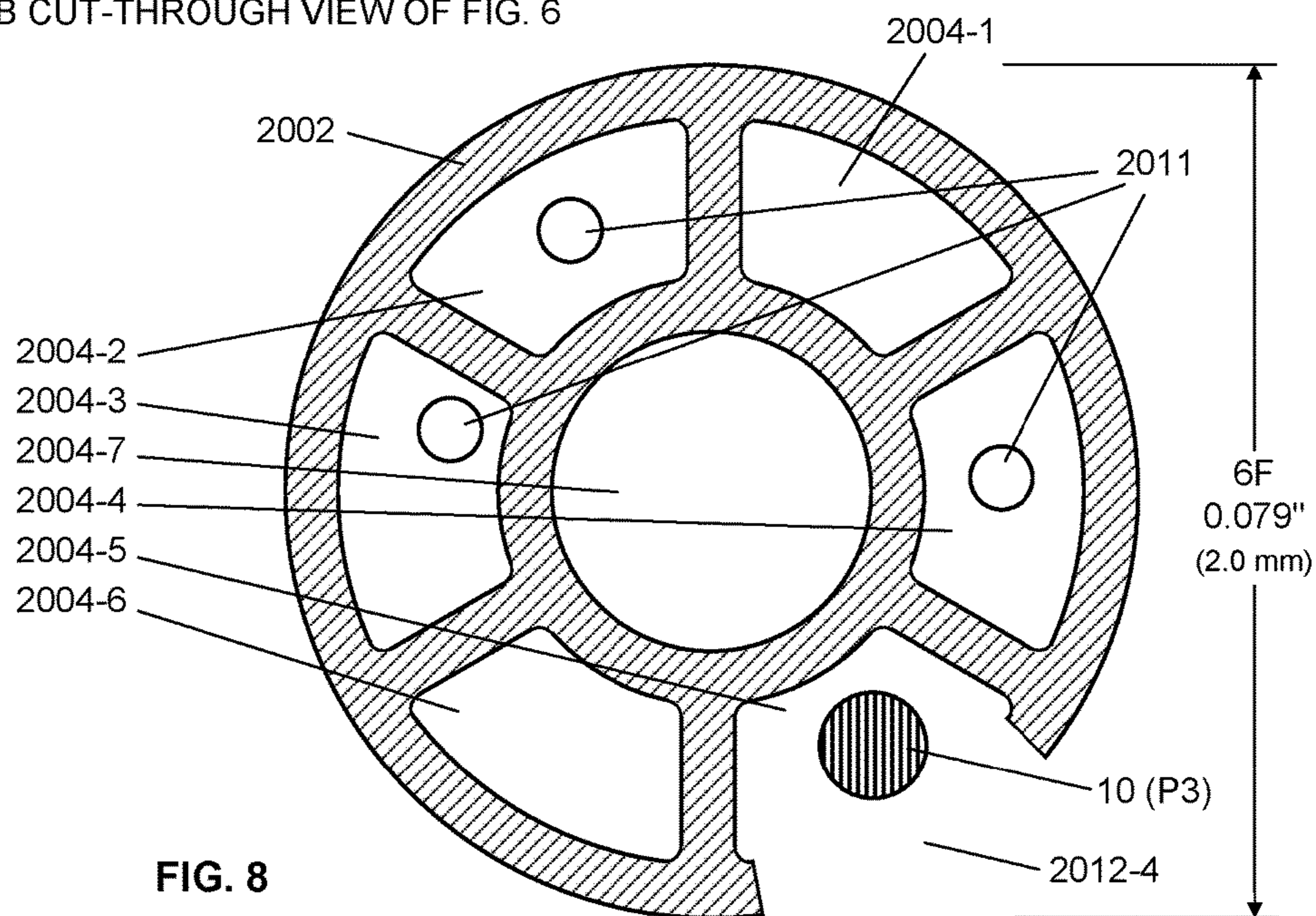
B-B CUT-THROUGH VIEW OF FIG. 6
