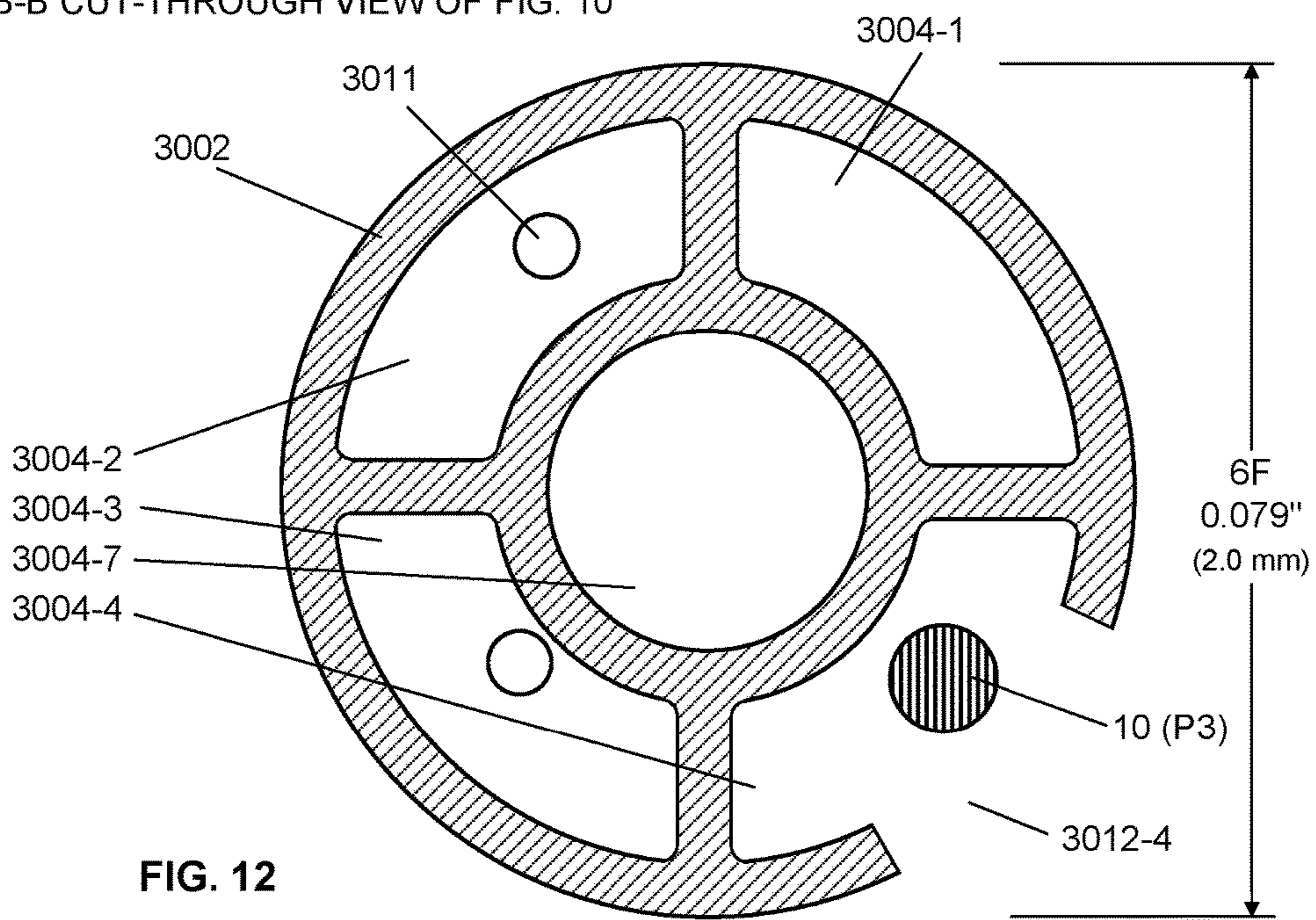
B-B CUT-THROUGH VIEW OF FIG. 10
