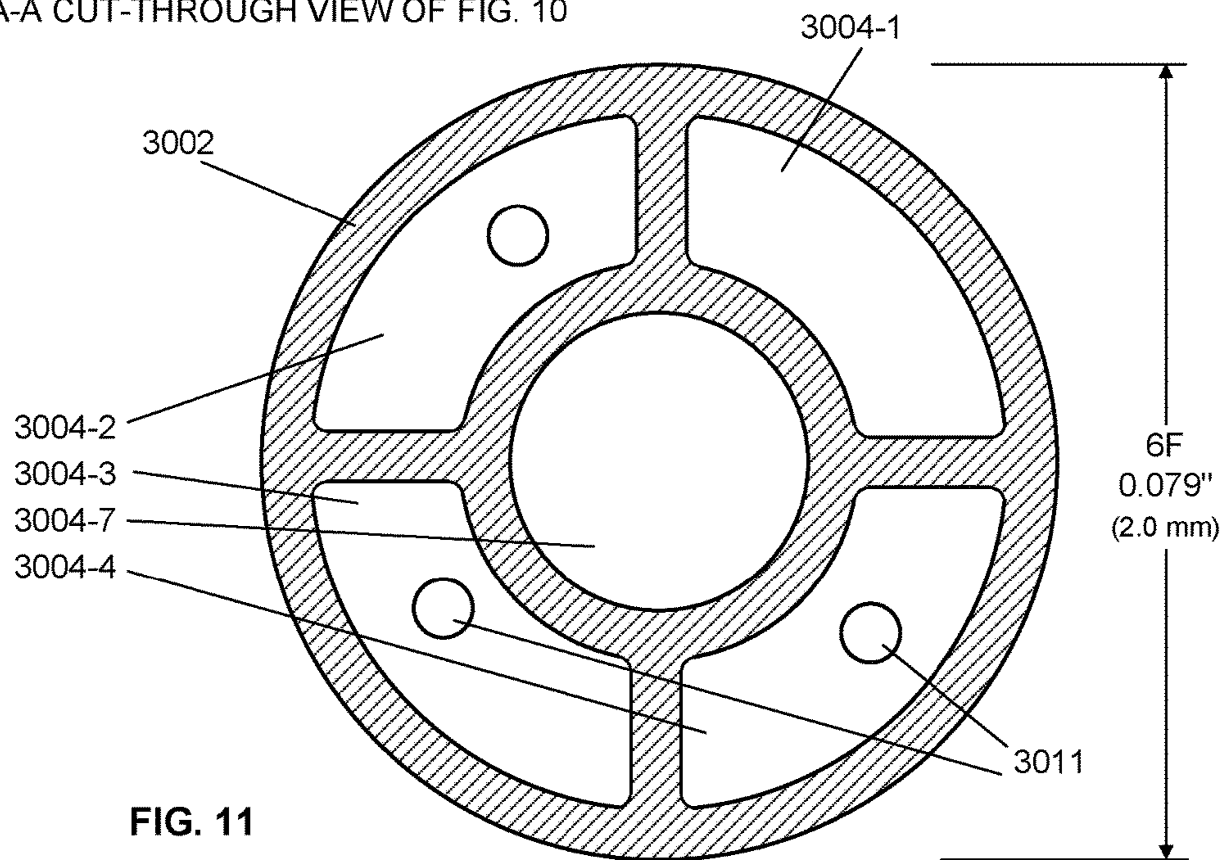
A-A CUT-THROUGH VIEW OF FIG. 10
