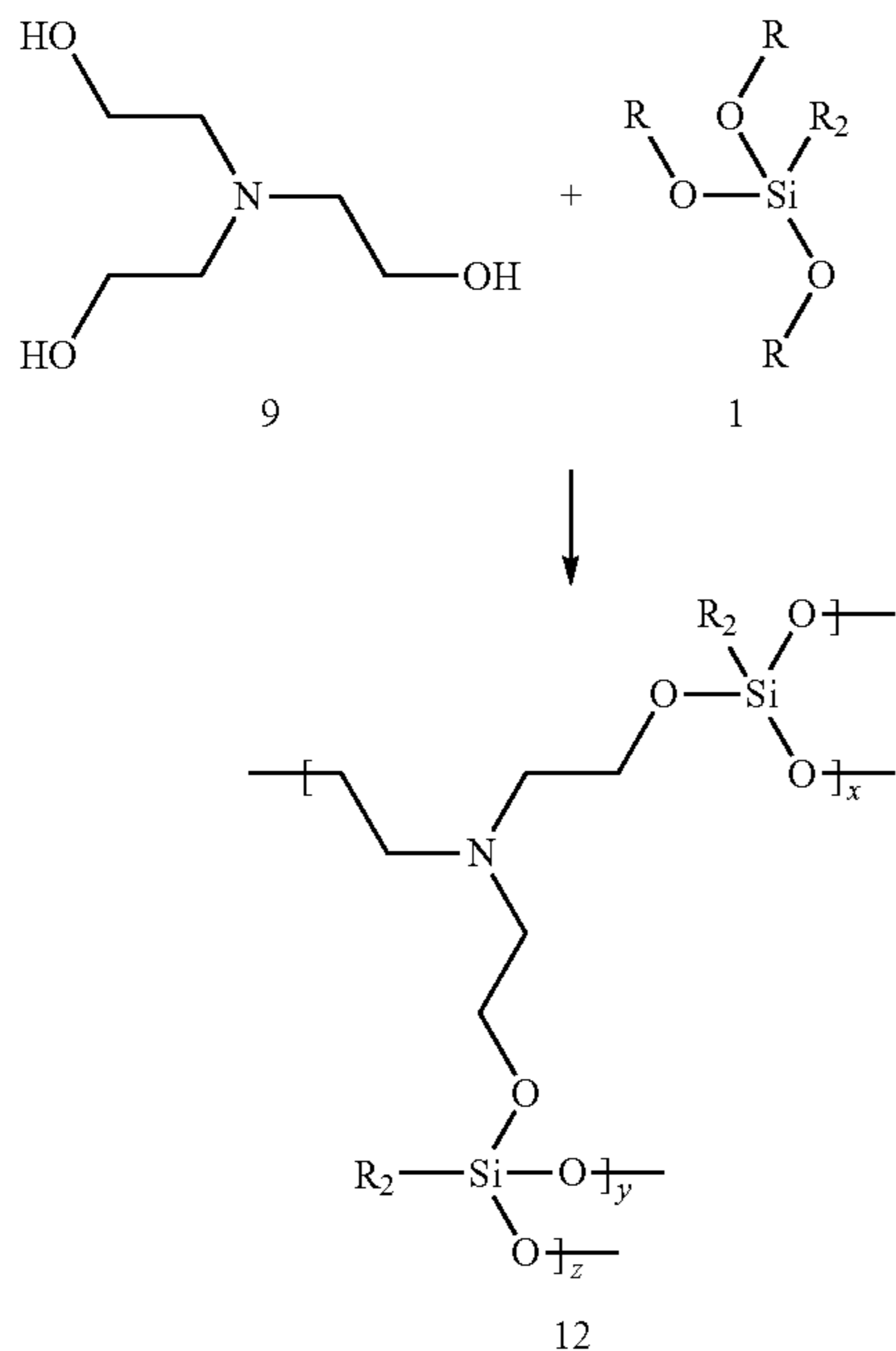
REACTION SCHEME 4
