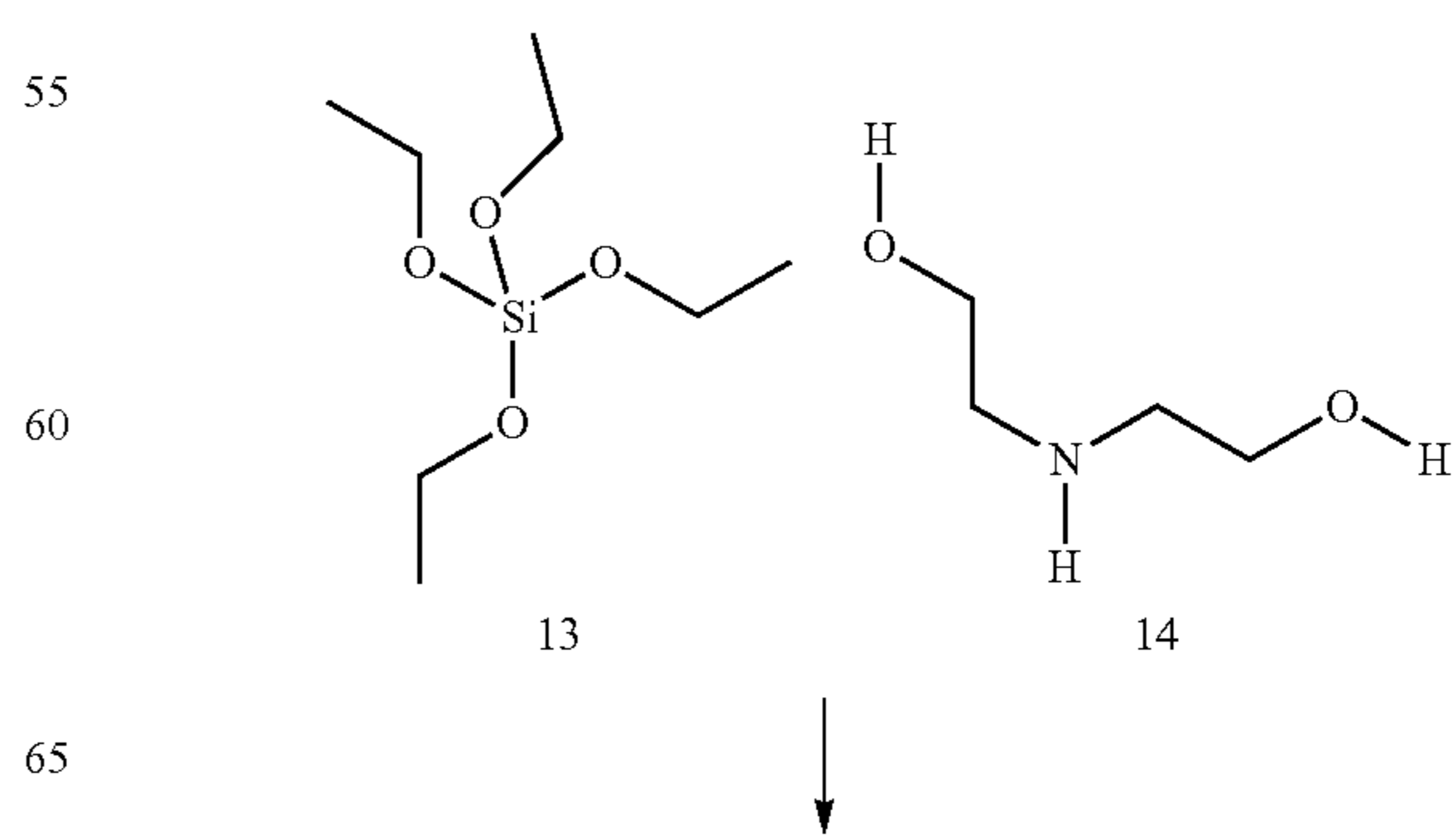
REACTION SCHEME 6
