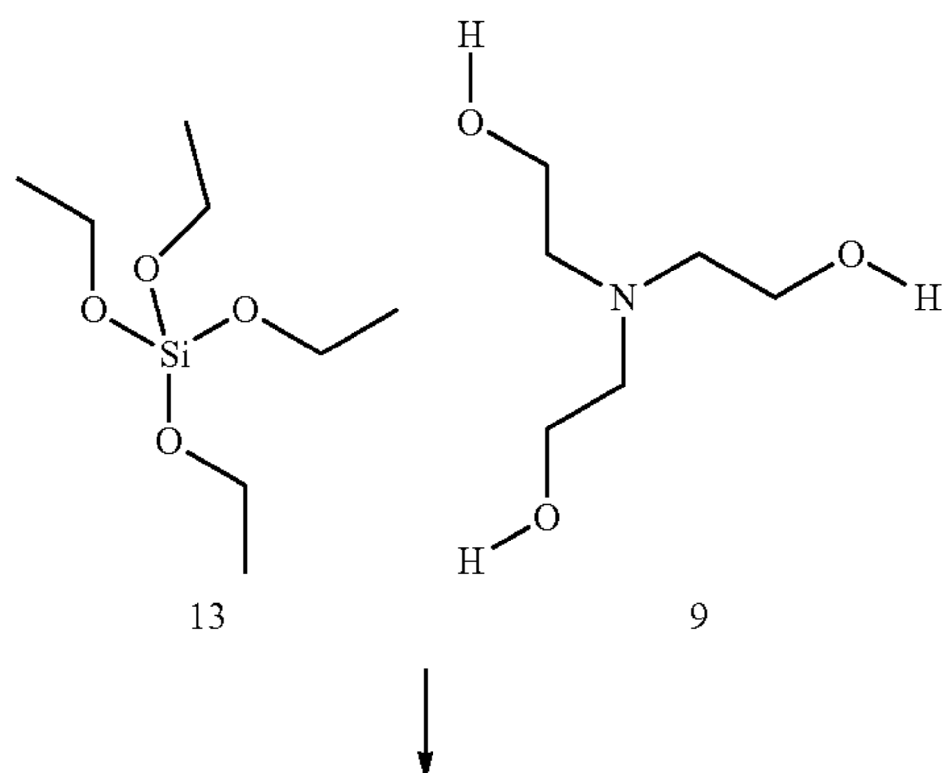
REACTION SCHEME 5
