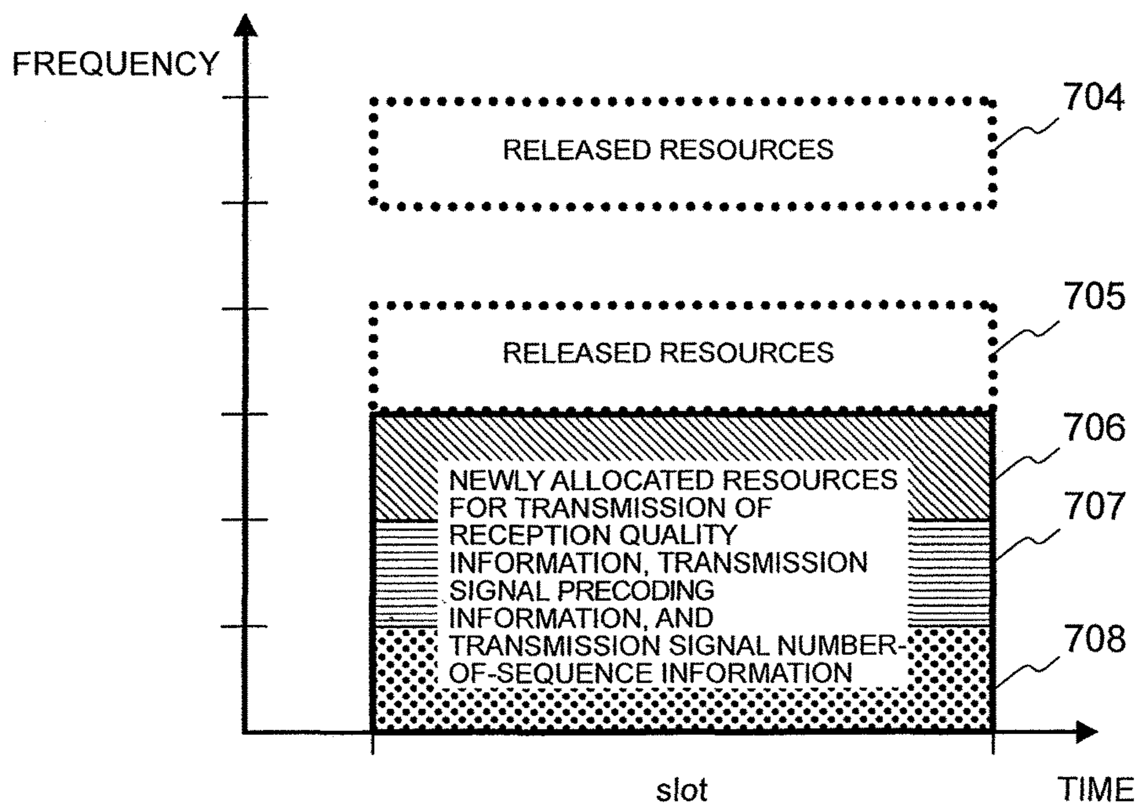
BAND CONTINUOUS ON THE FREQUENCY AXIS IS NEWLY RESERVED AND ALLOCATED TO THE MOBILE STATION APPARATUS TO RESPOND TO SC-FDMA
