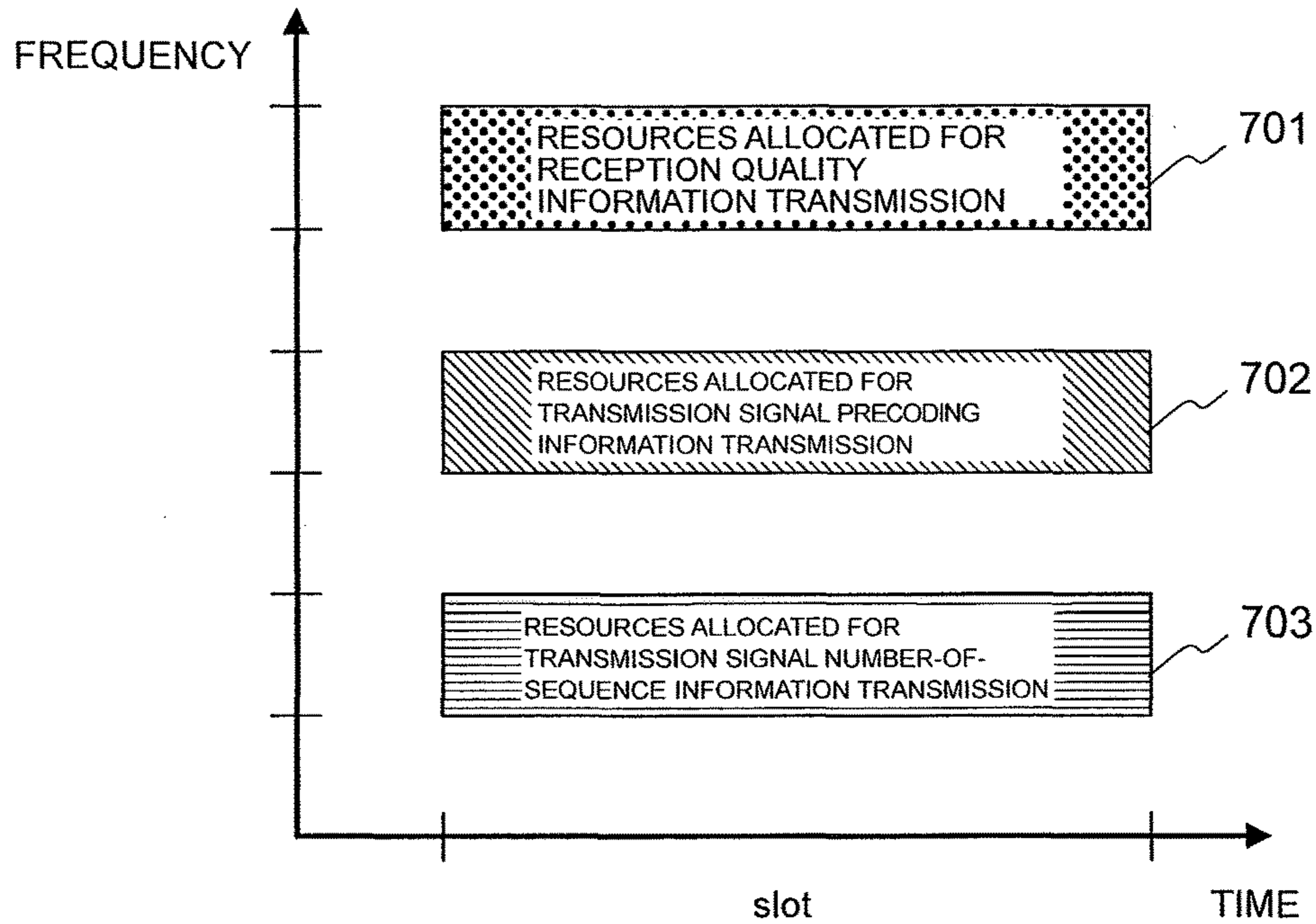
CASE WHERE A PLURALITY OF KINDS OF FEEDBACK INFORMATION IS ASSIGNED TO RESOURCES THAT ARE NOT CONTINUOUS IN THE SAME SLOT
