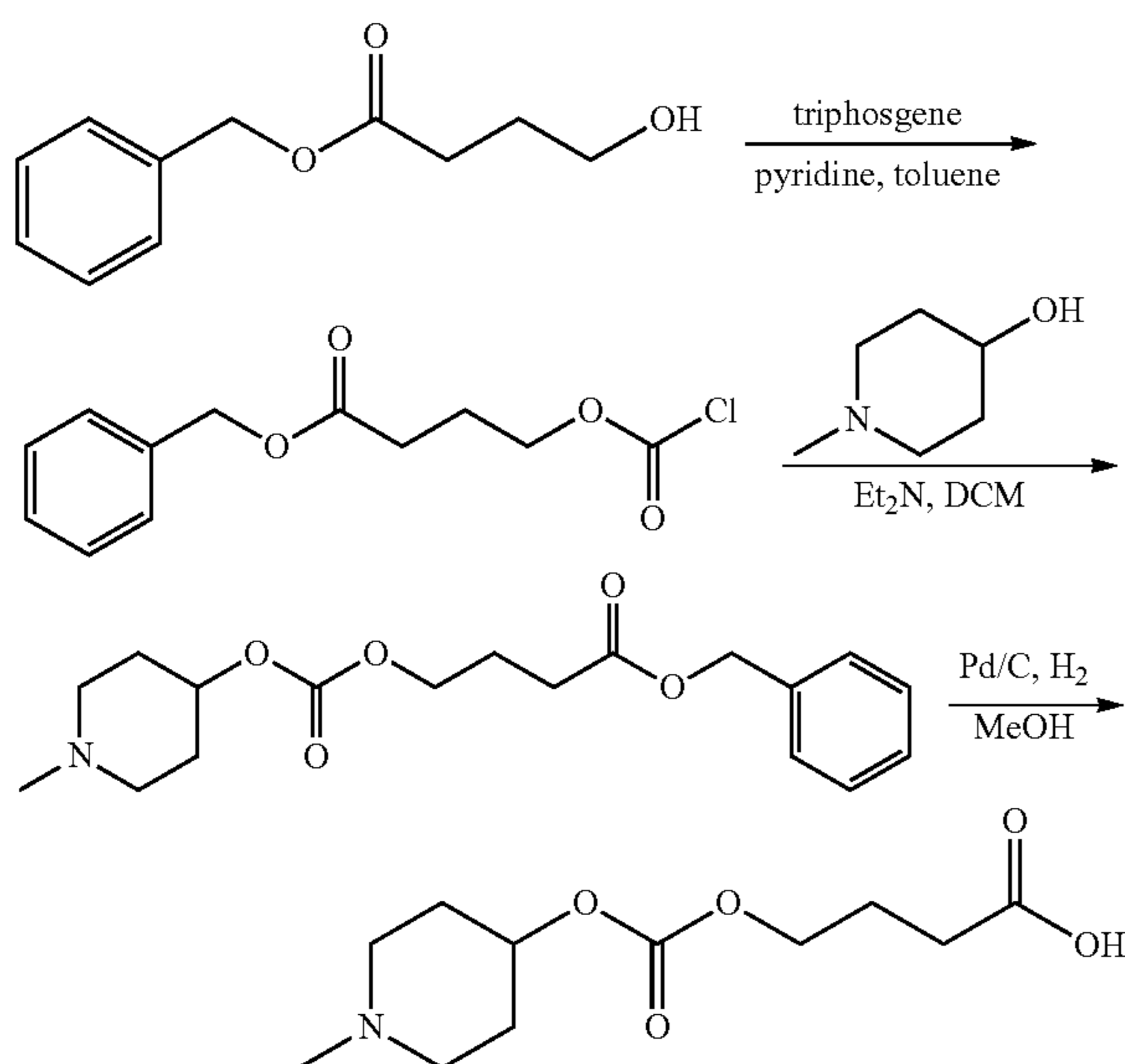
Scheme 12:
