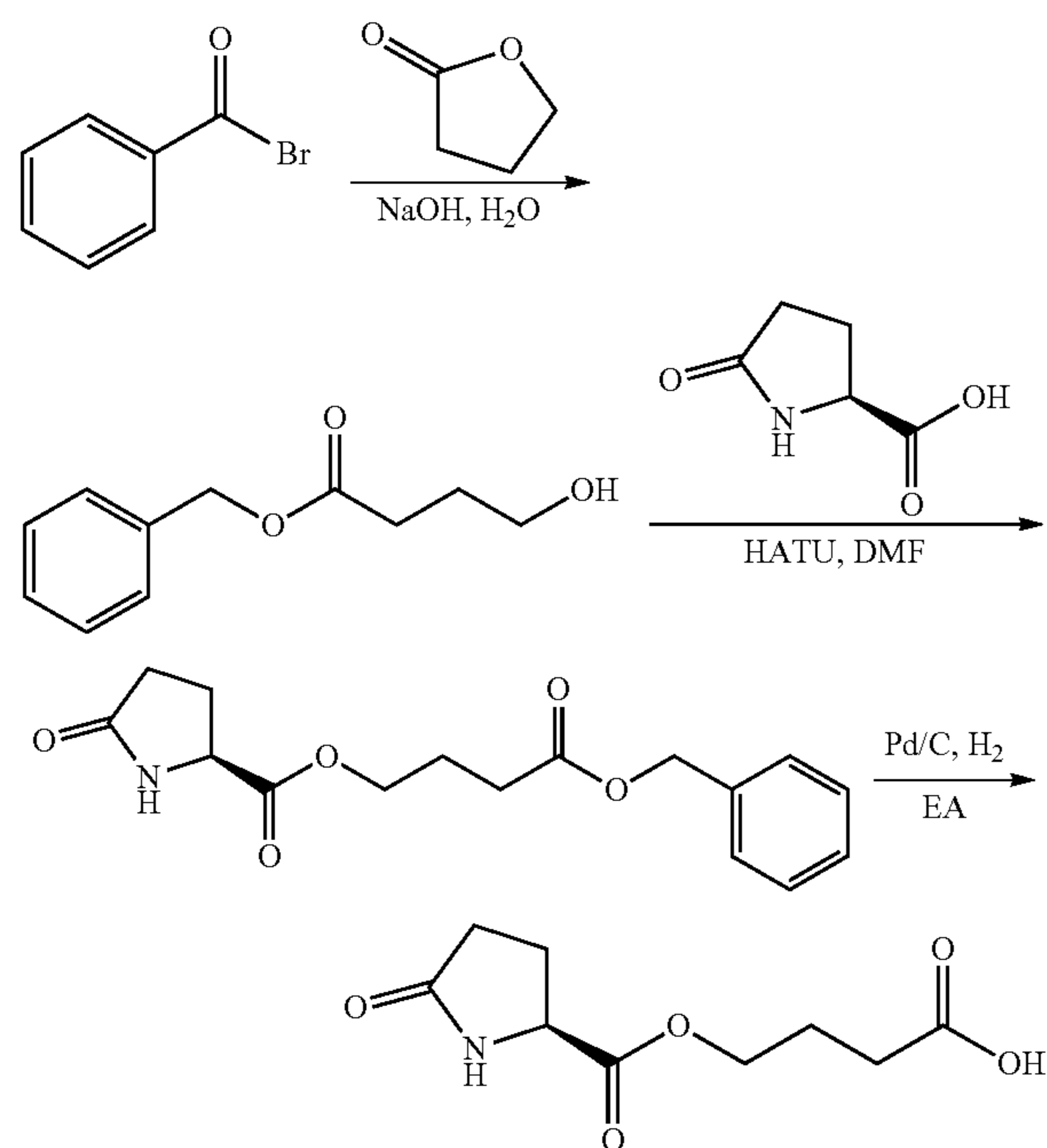
Scheme 9:
