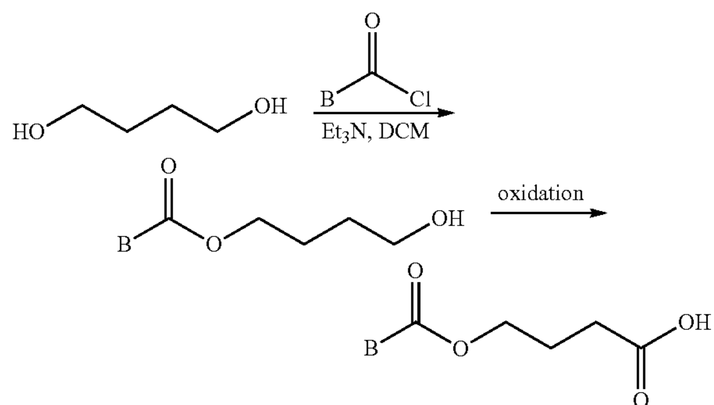
Scheme 1
