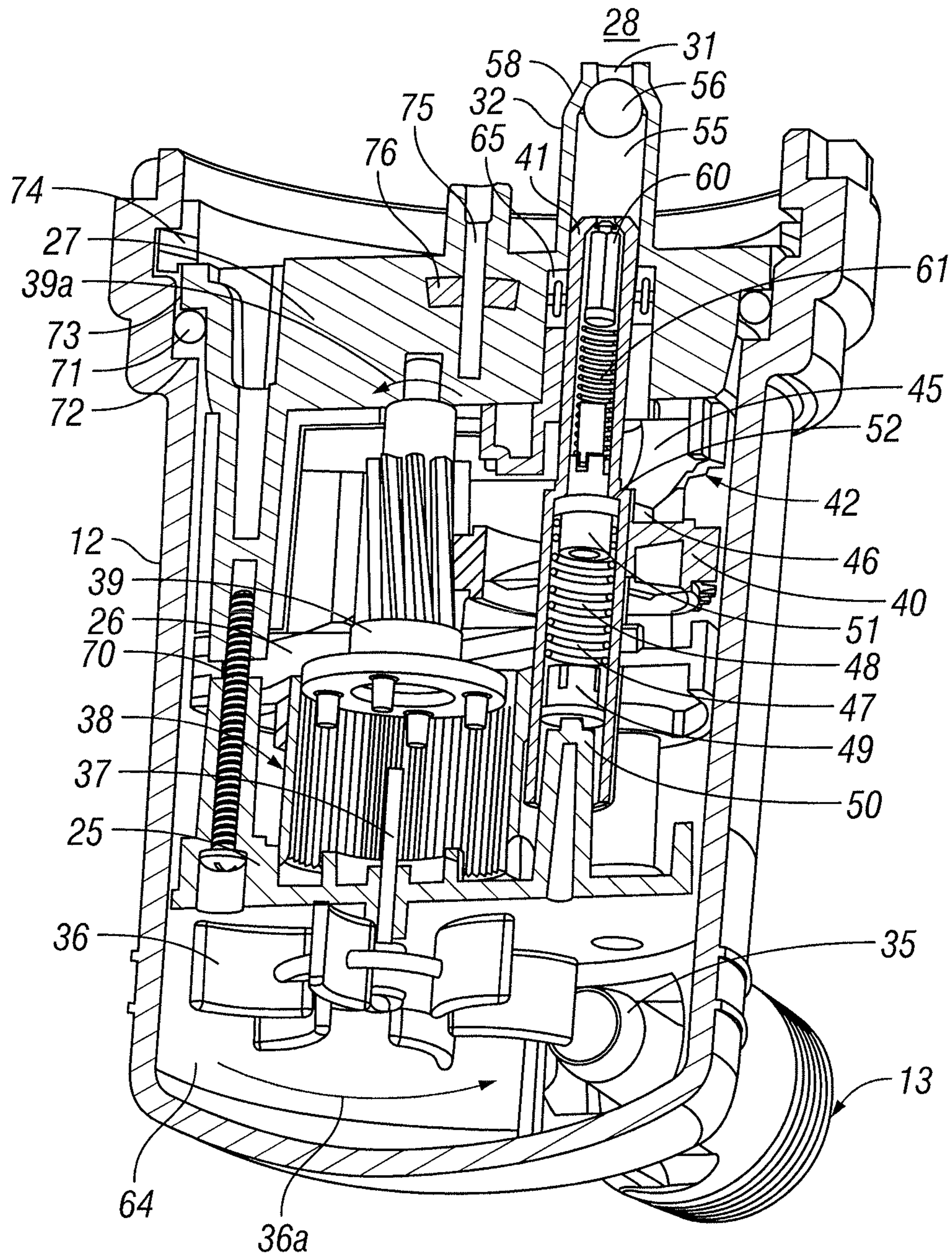
FIG. 2 (Prior Art)
