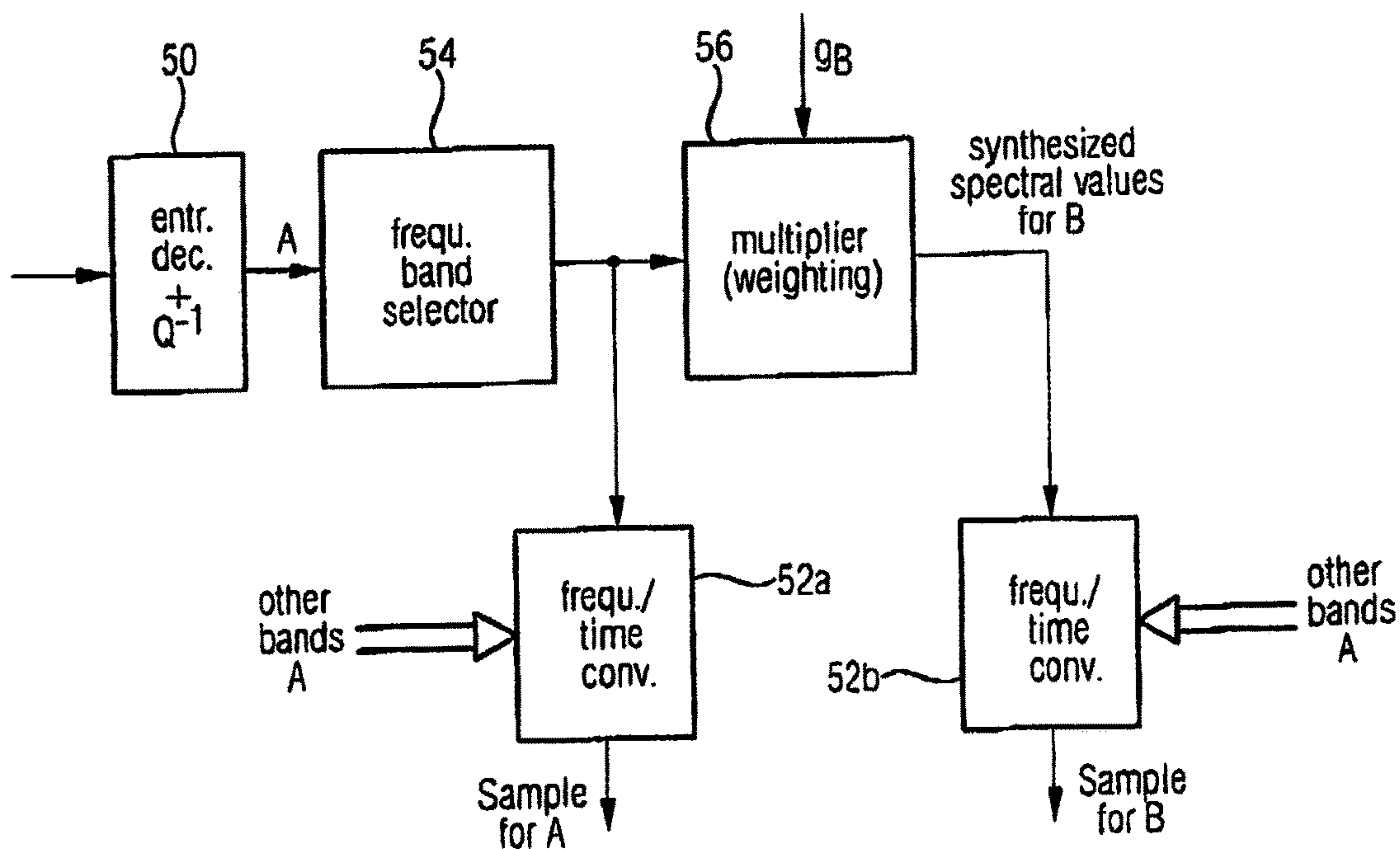
FIG 5 (decoder side)
