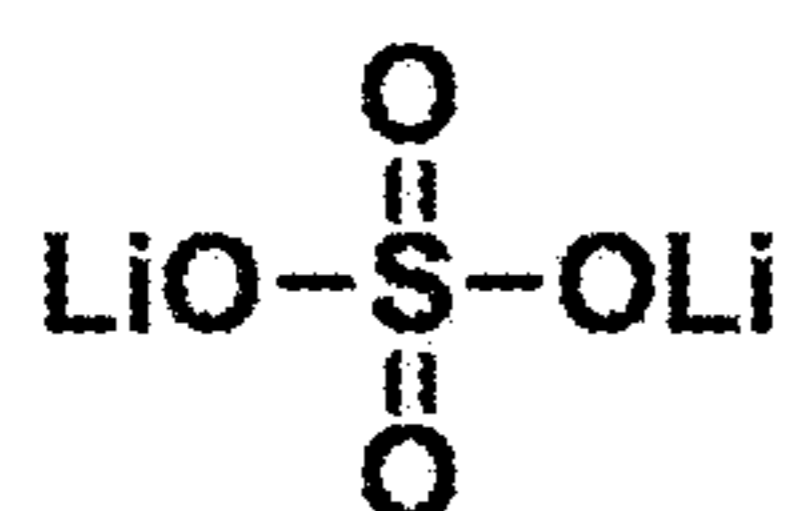
lithium sulfate
