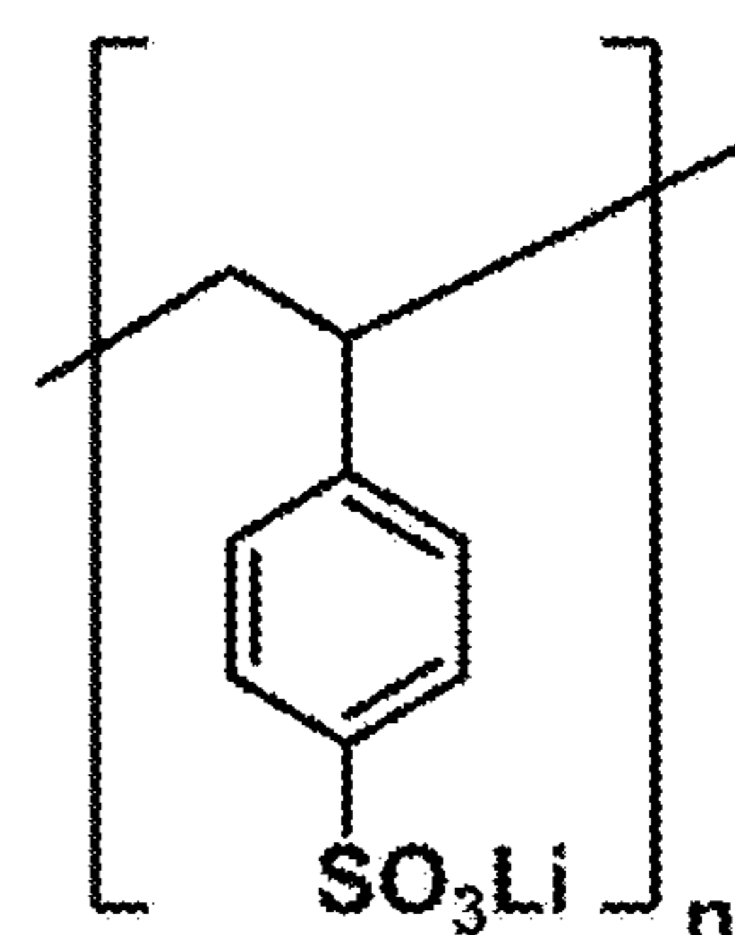
Poly(lithium-4-styrenesulfonate)
