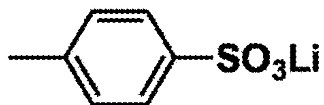
lithium 4-methylbenzenesulfonate
