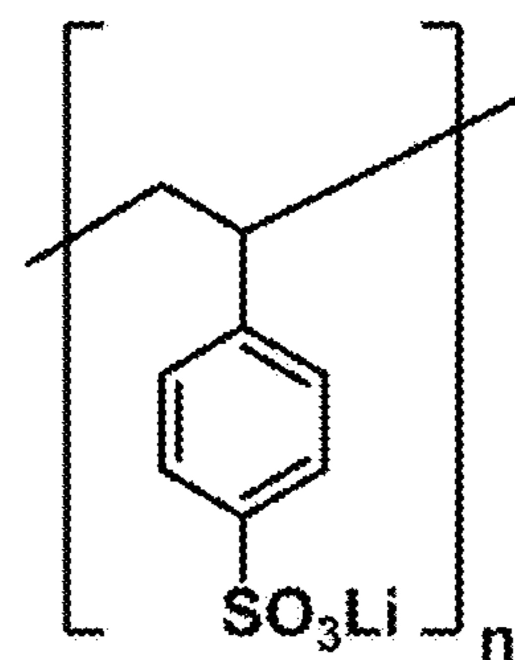
Poly(lithium-4-styrenesulfonate)
