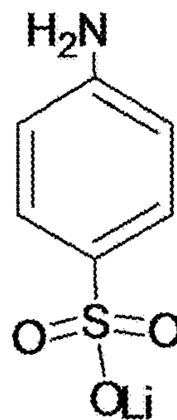
Poly(lithium-4-styrenesulfonate)
