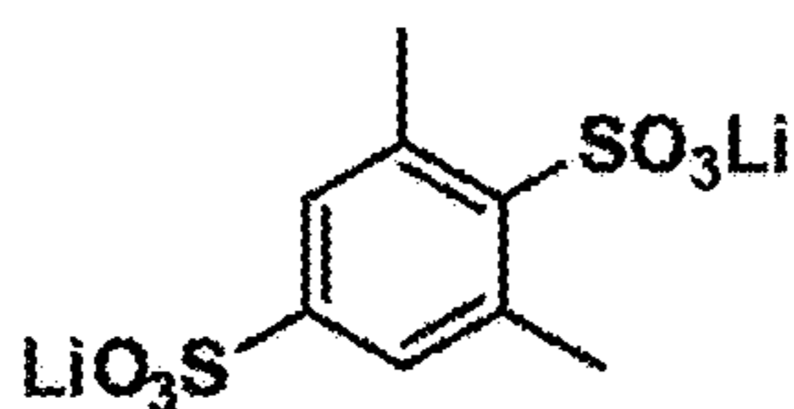
lithium 2,6-dimethylbenzene-1,4-disulfonate
