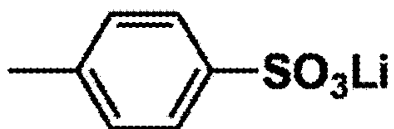
lithium 4-methylbenzenesulfonate
