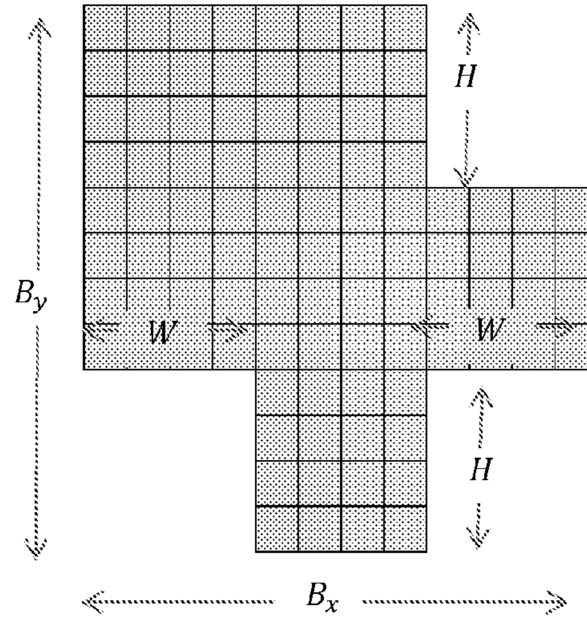
Figure A4a. "K" Shape Footprint
