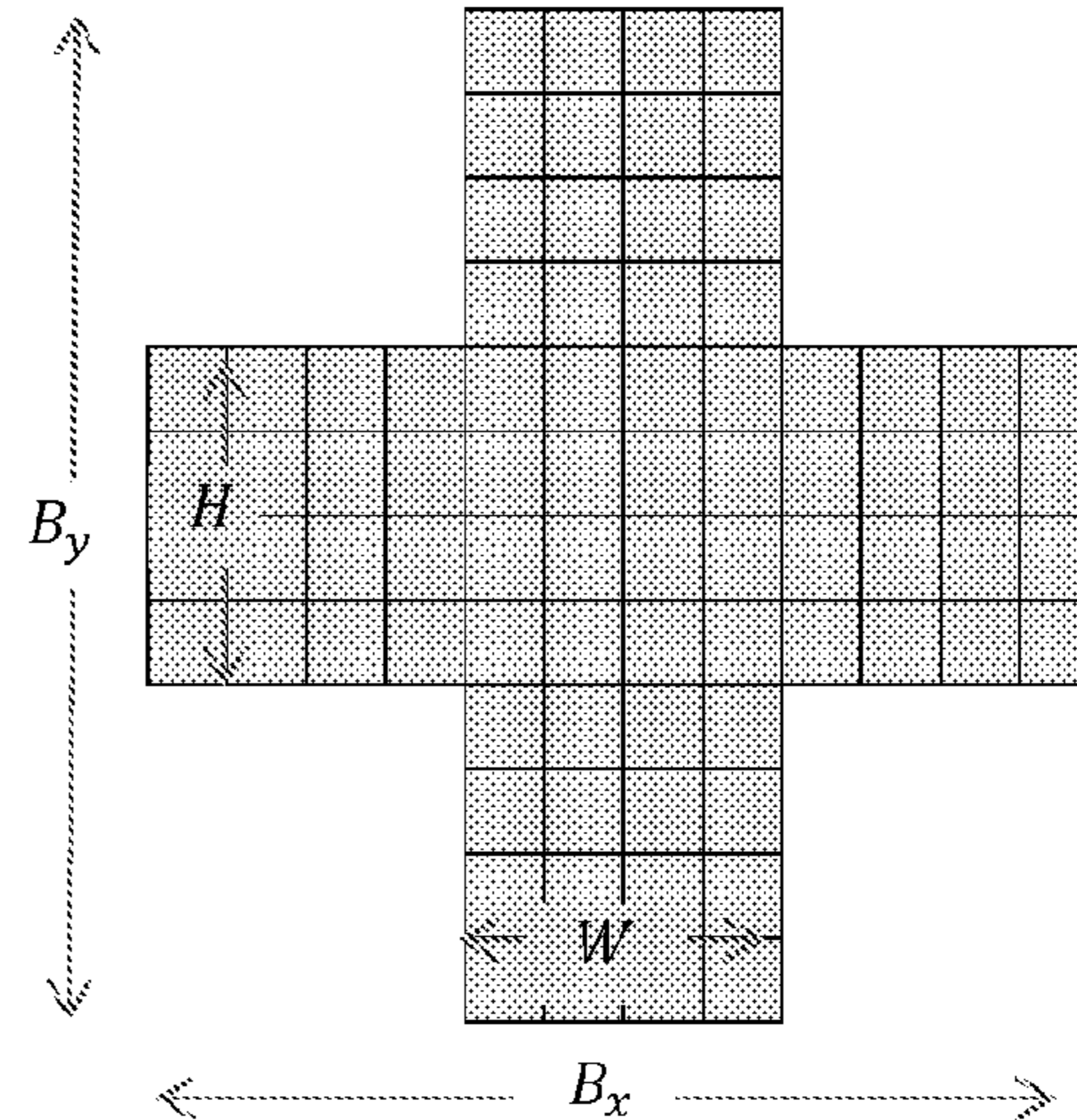
Figure A5a. "X" Shape Footprint
