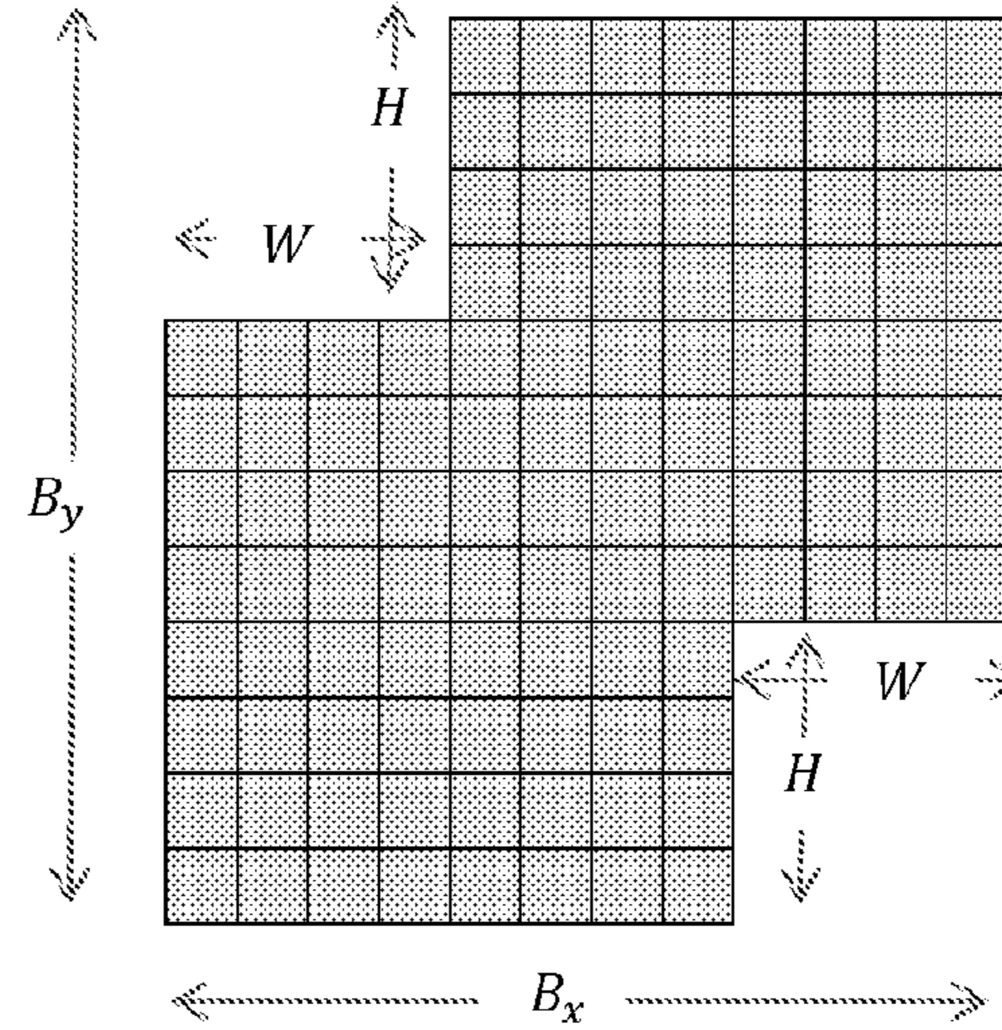
Figure A3a. "Z" Shape Footprint
