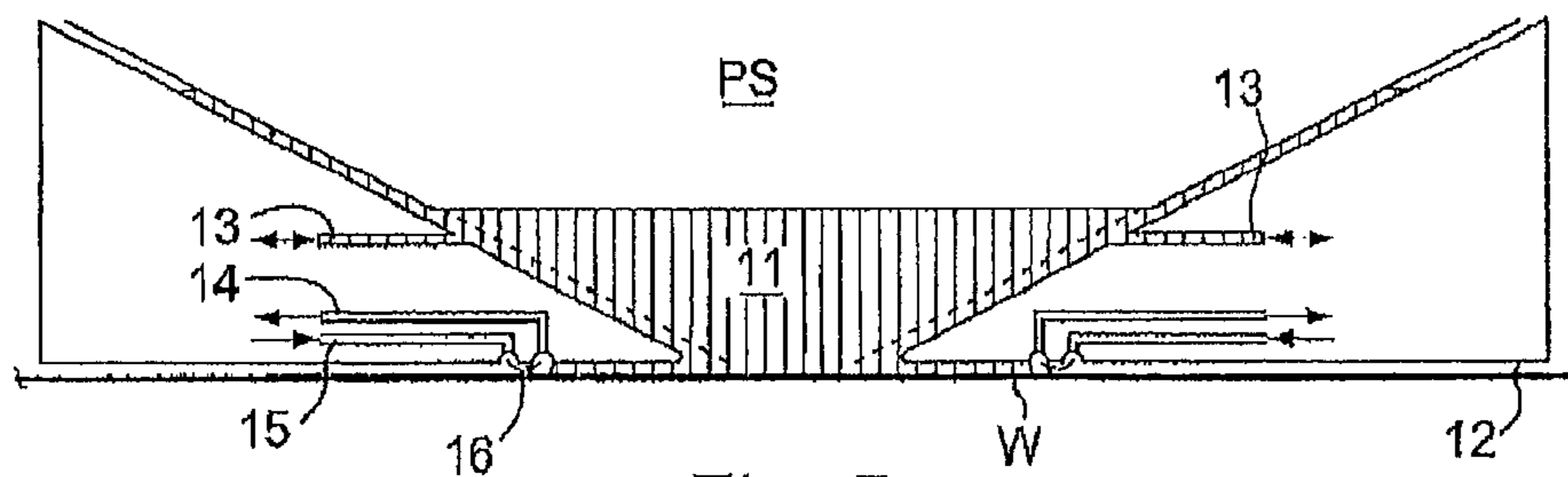
Fig. 5 (Prior Art)
