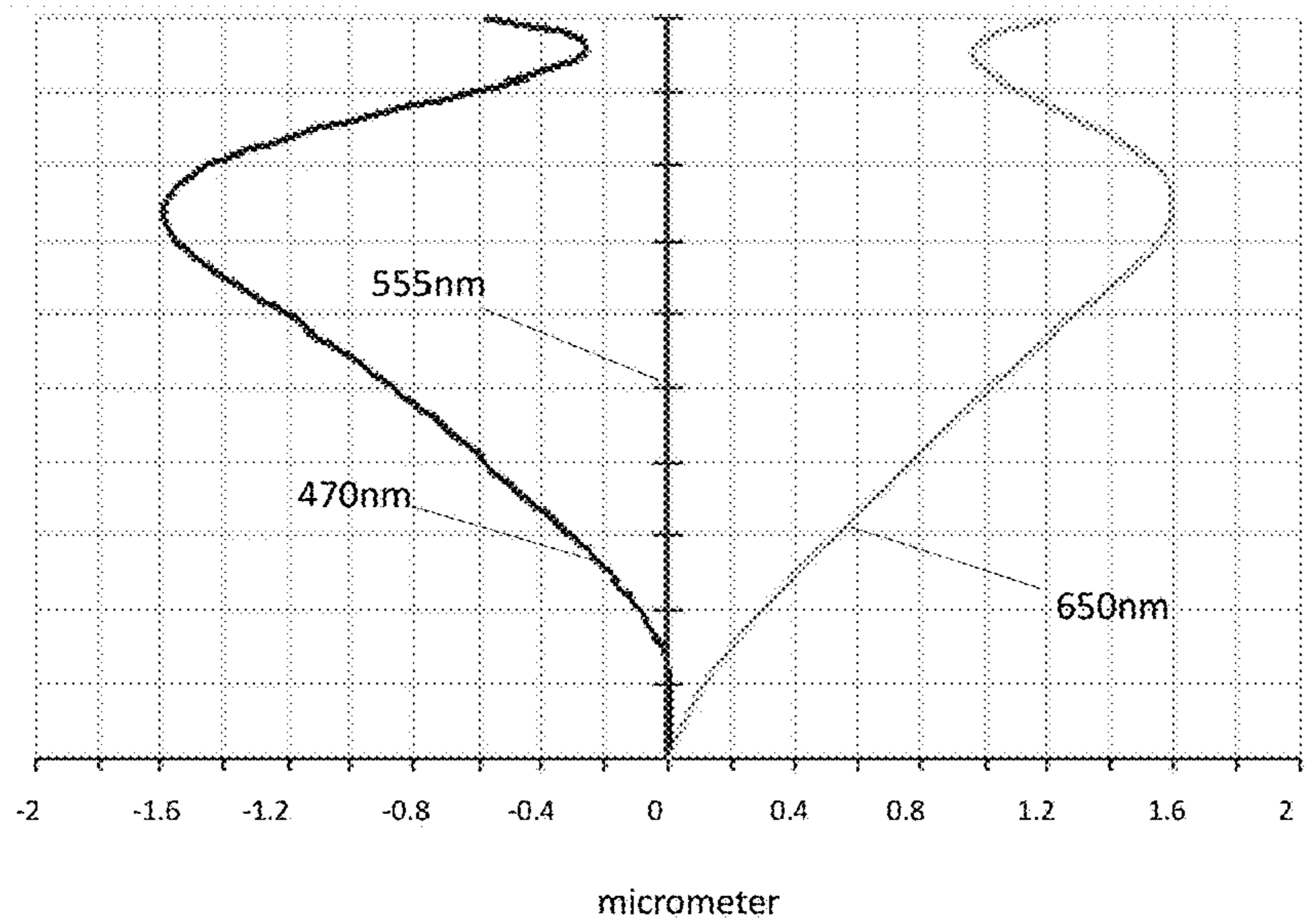
Lateral color
