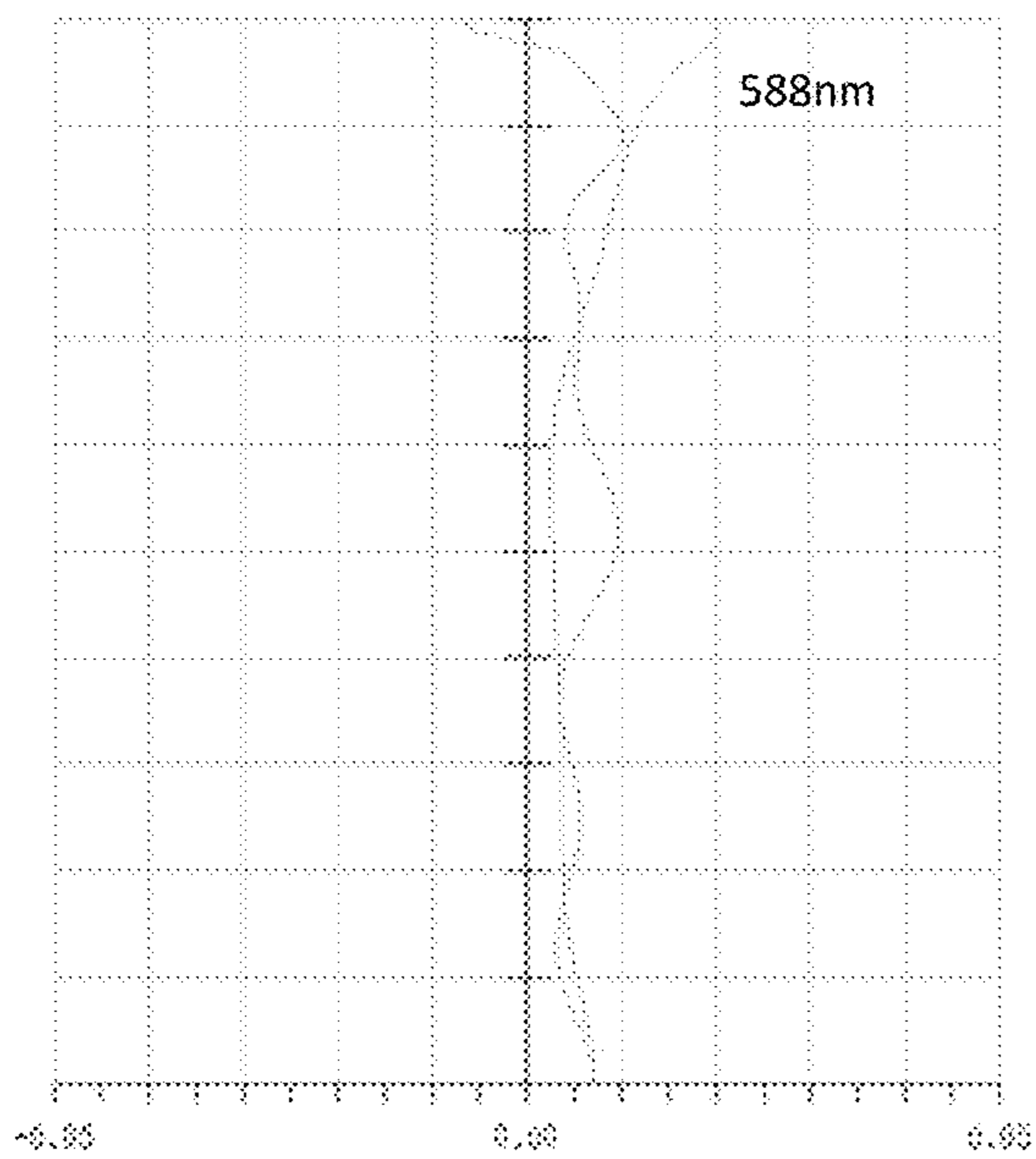
Field curvature
