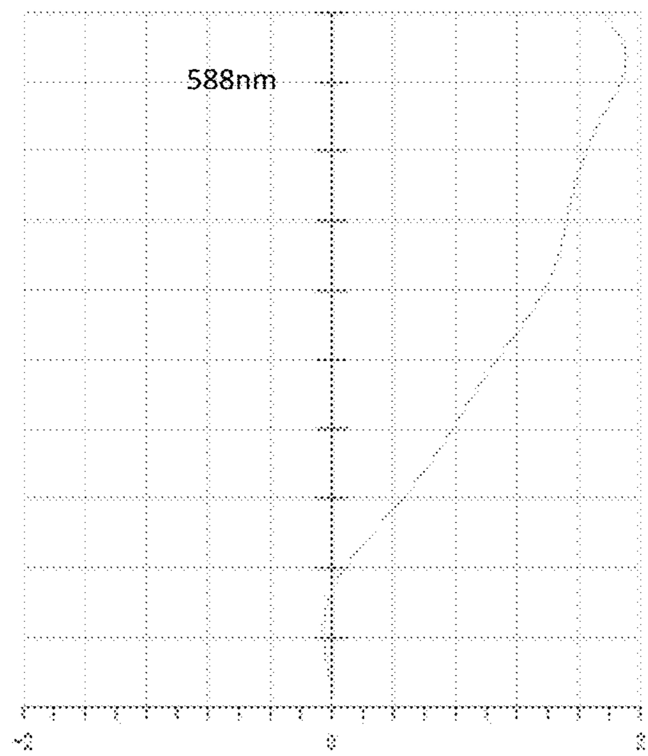
Distortion
