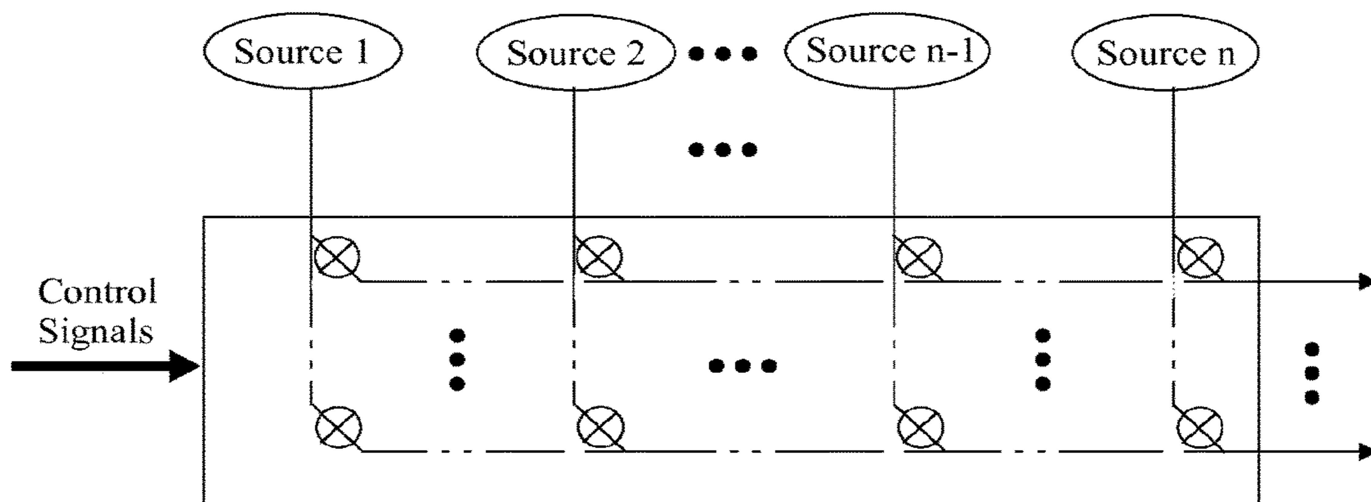
A Lattice/Matrix Valve Complex of Simple On/Off Valves
