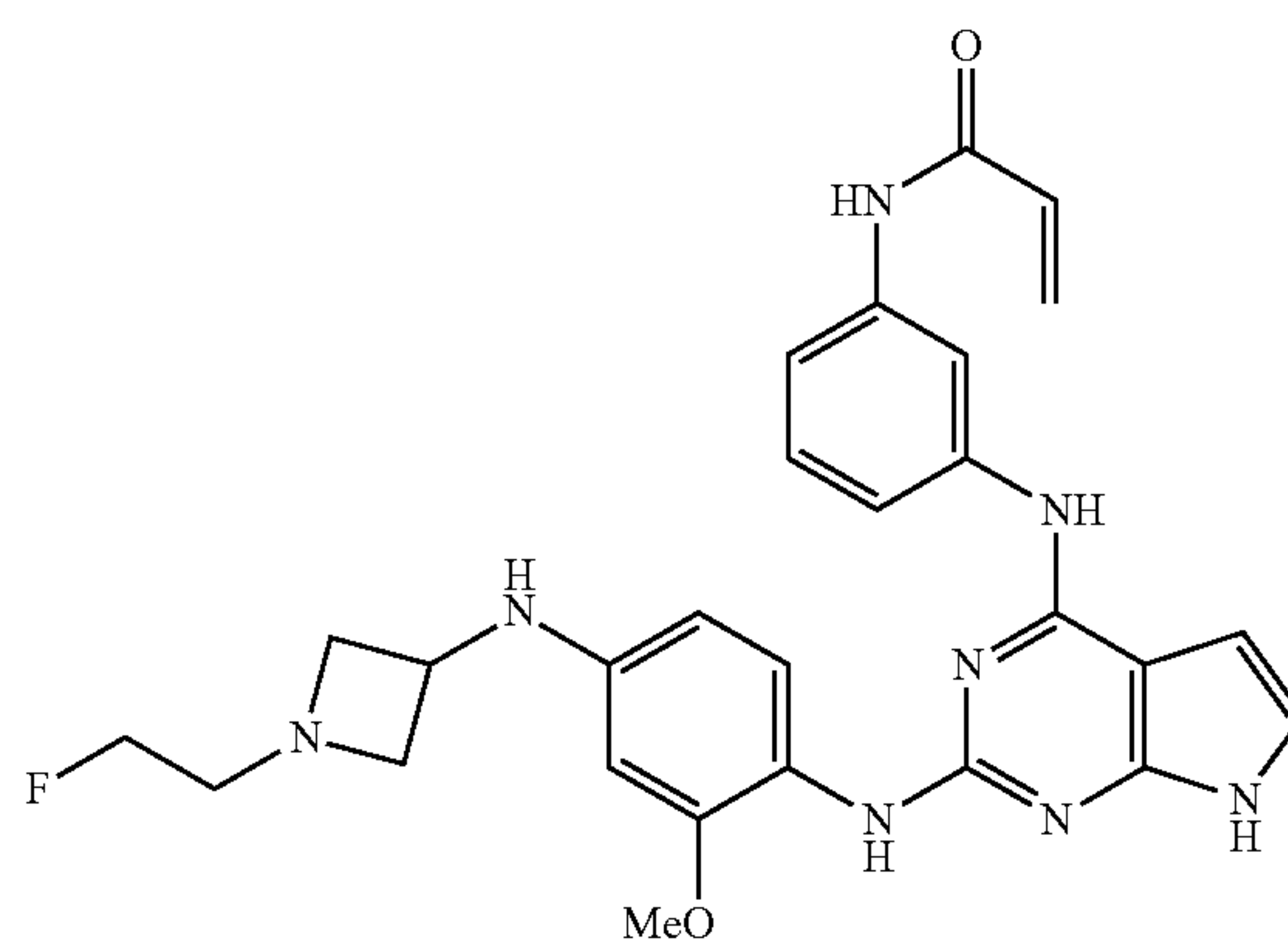
Compound 35
