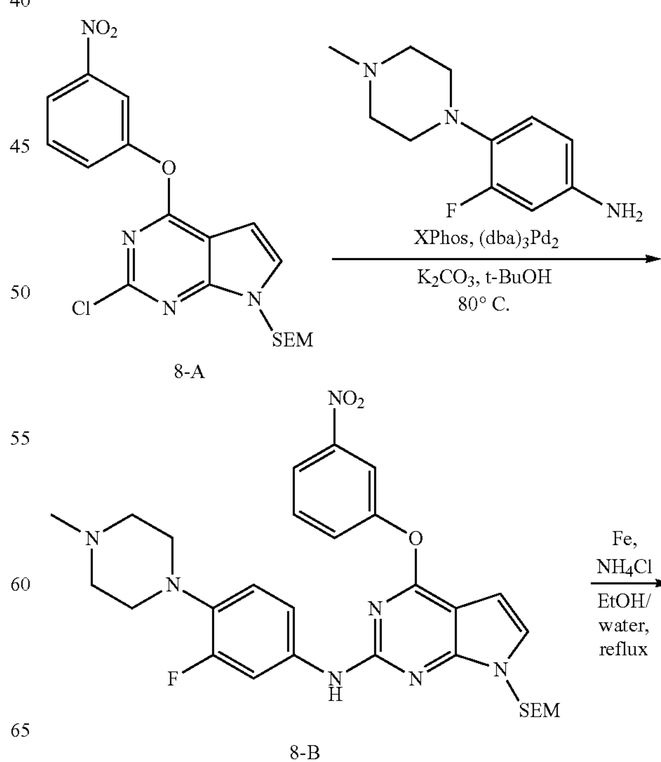
Scheme 8
