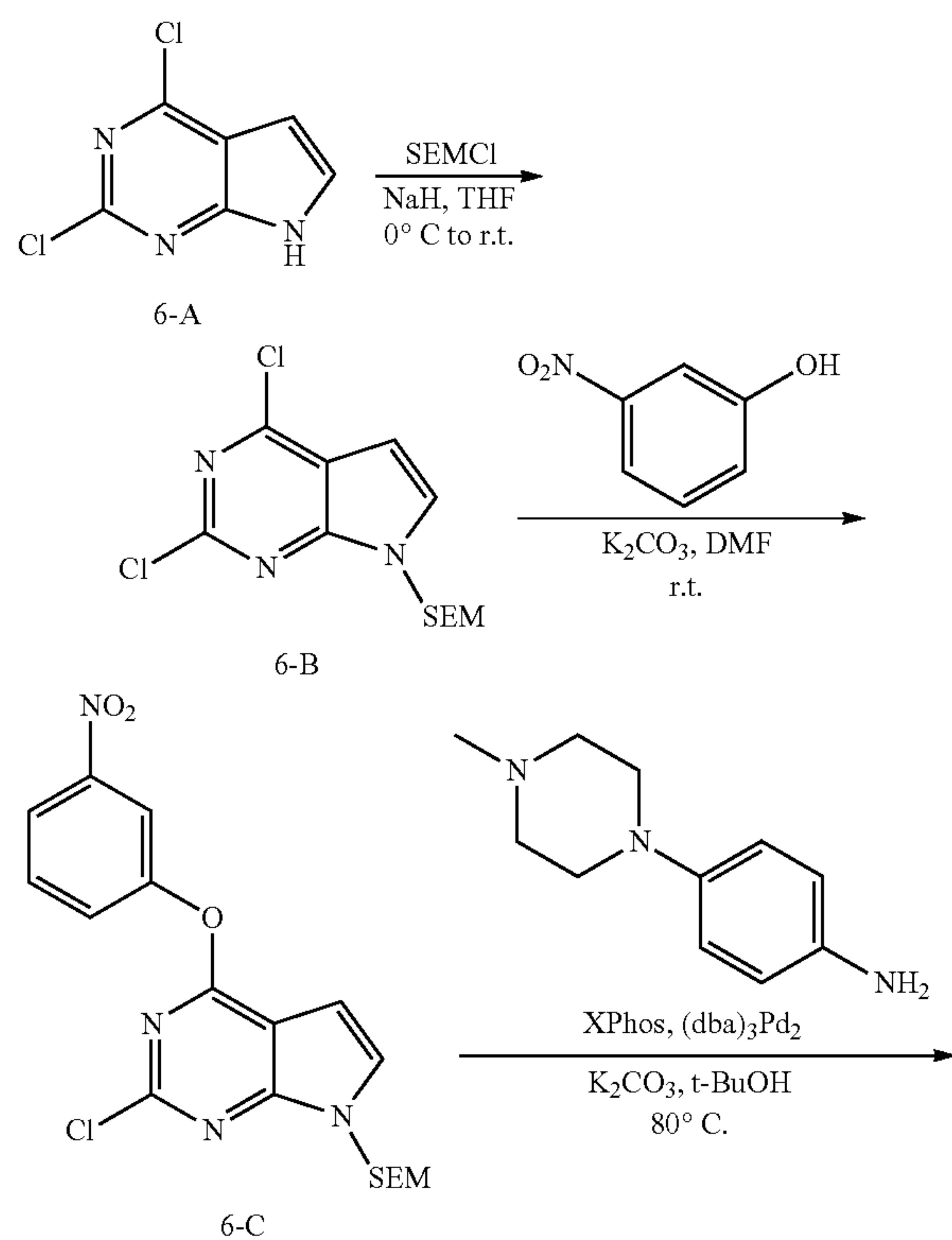
Scheme 6
