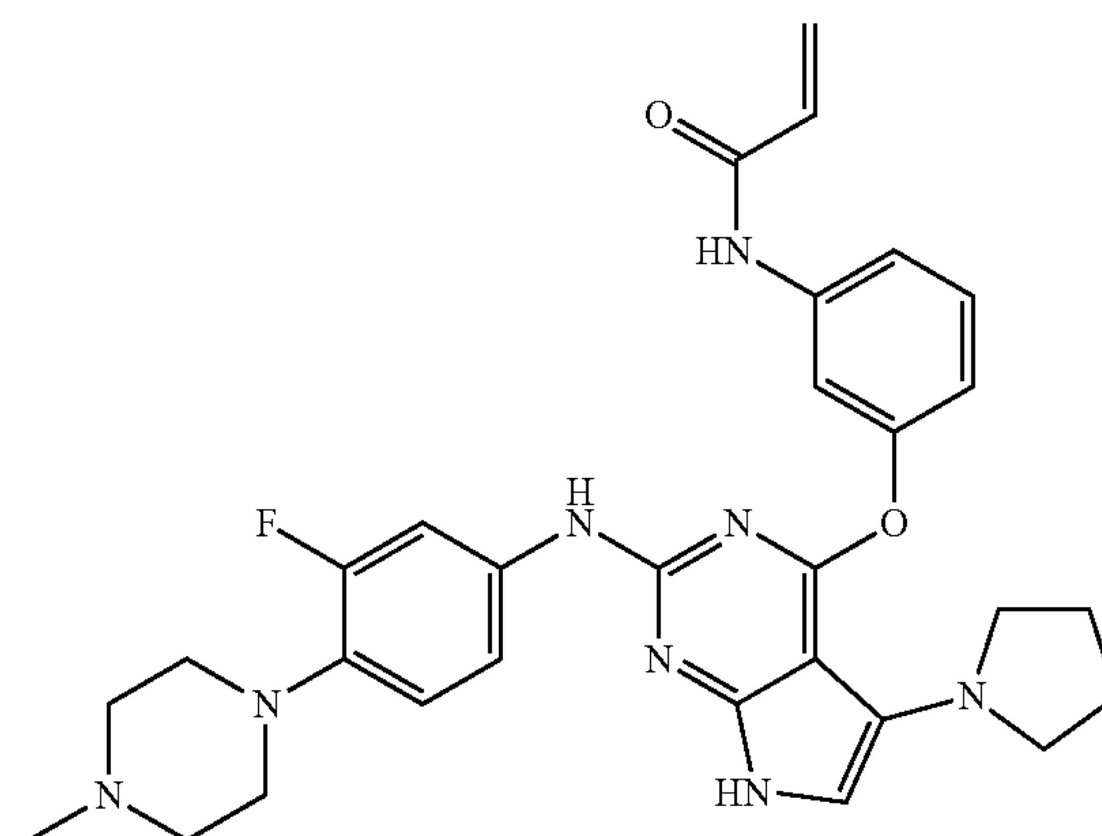
Compound 13
