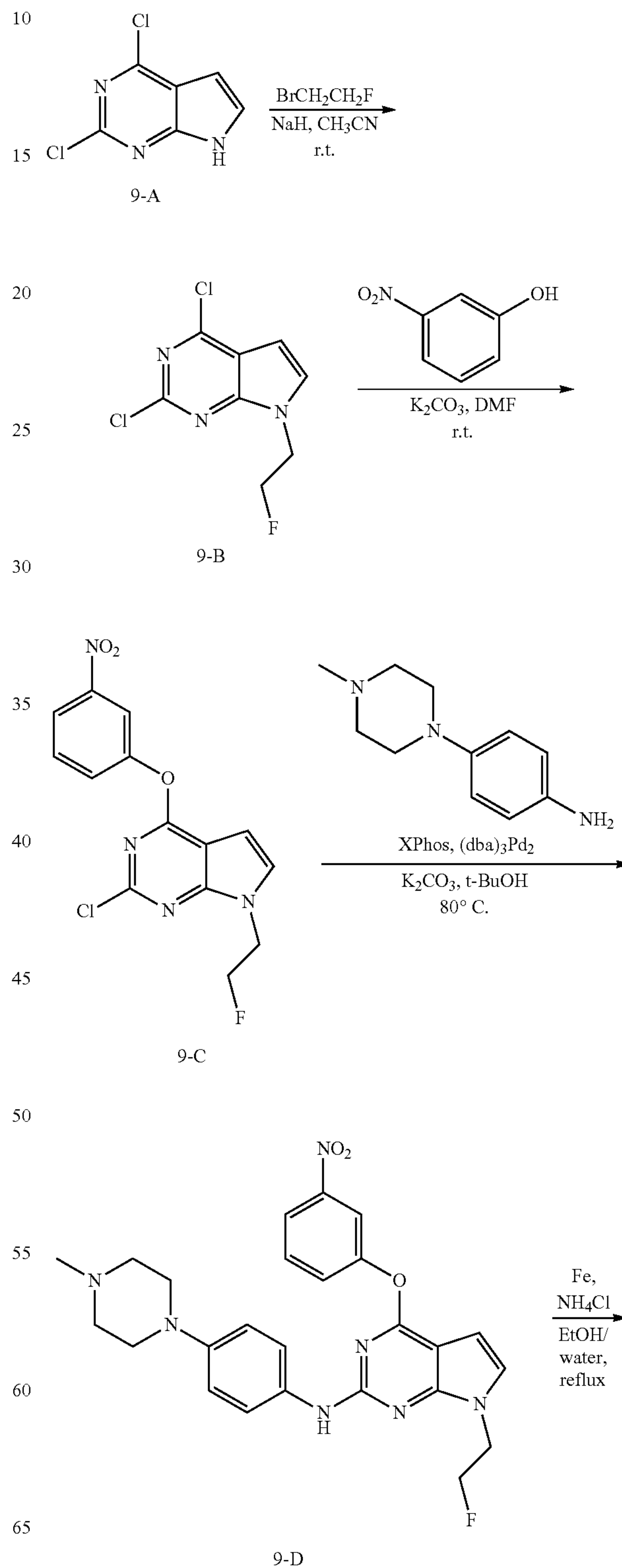
Scheme 9
