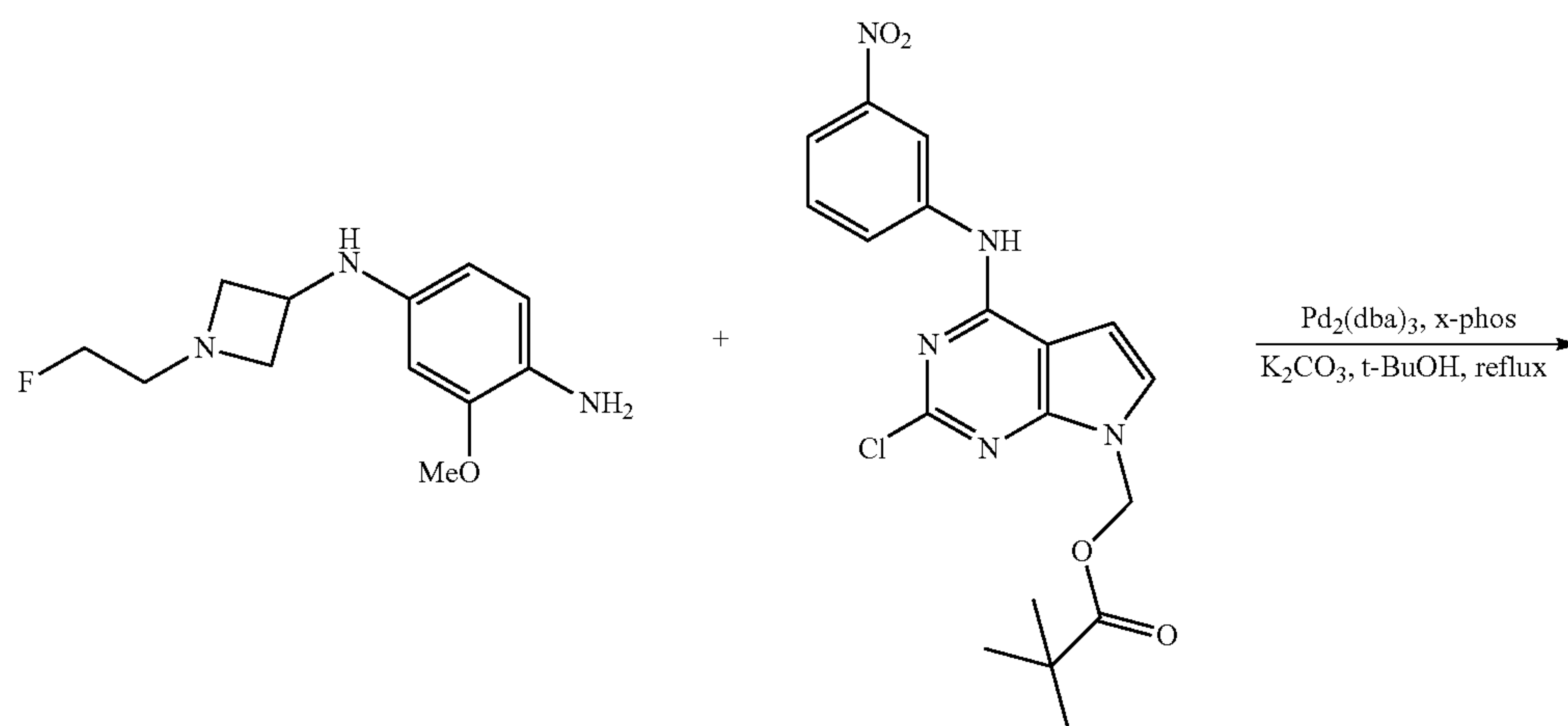
Scheme 5-1
