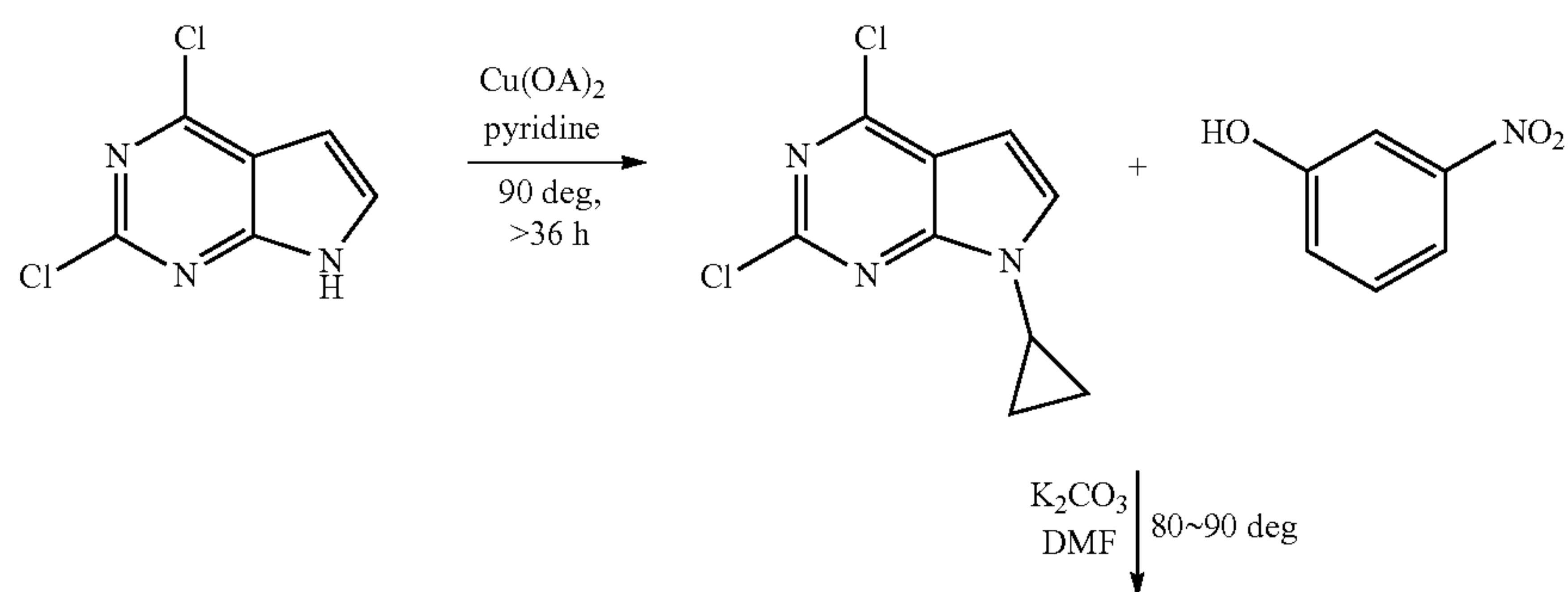
Scheme 5
