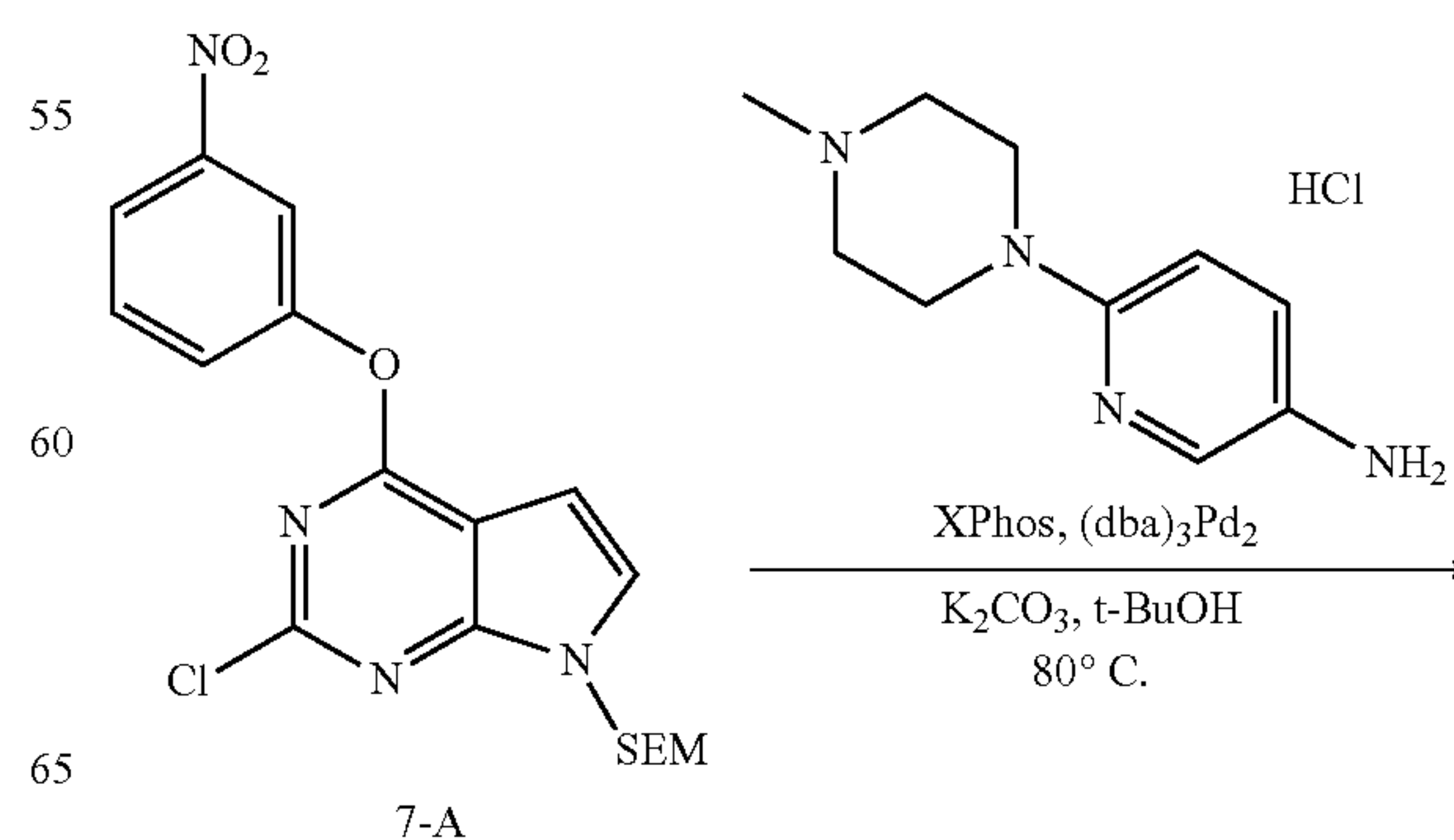
Scheme 7
