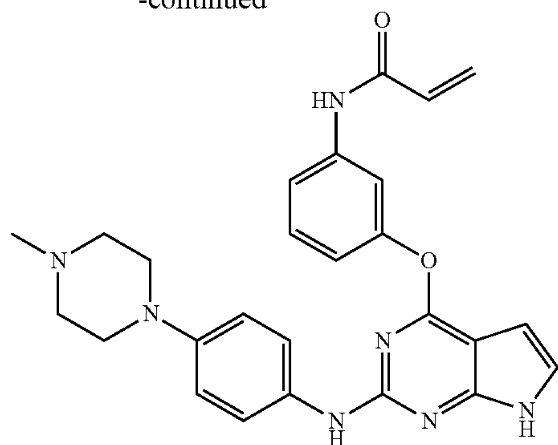
Compound 1
