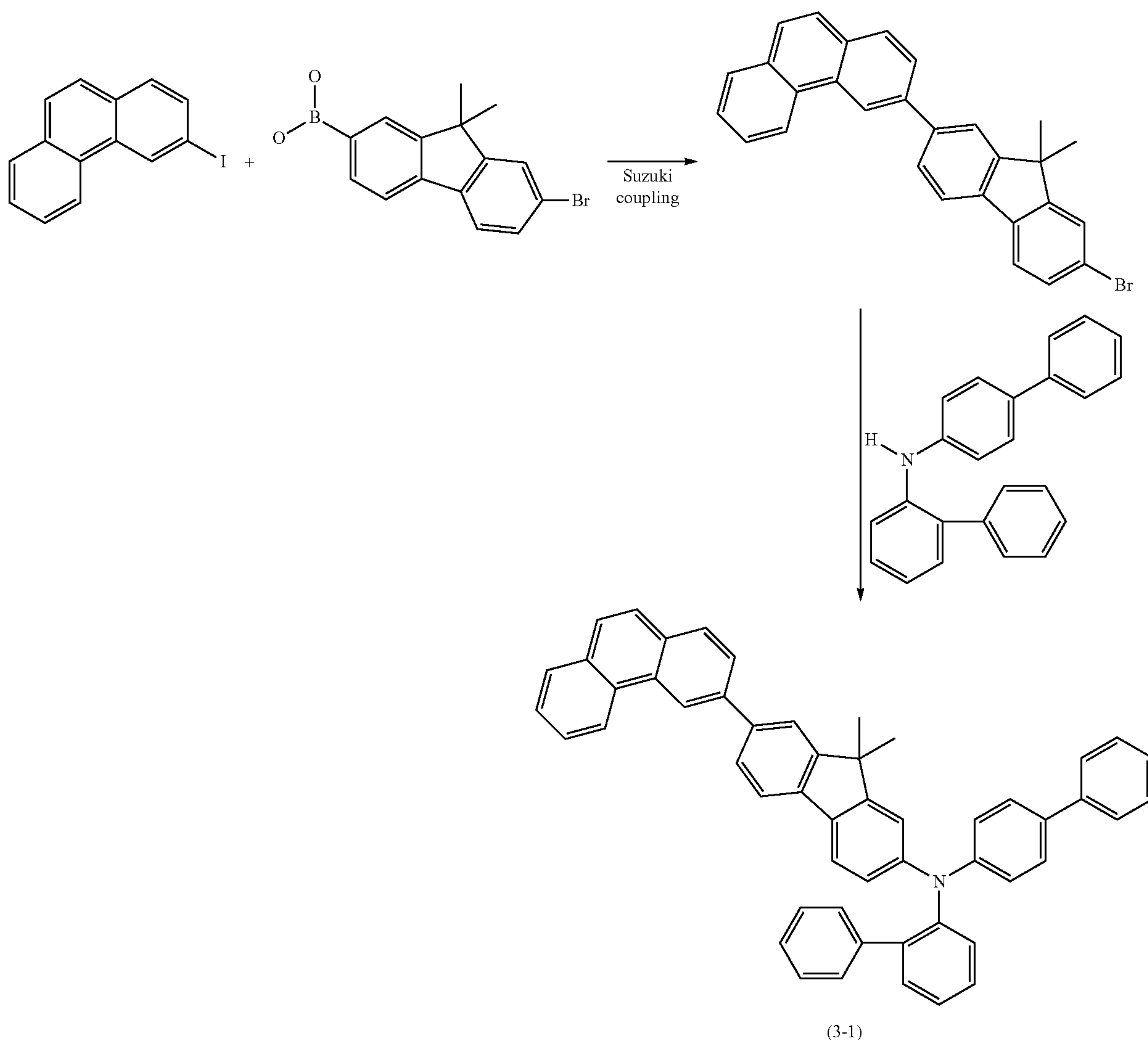
3-(7-Bromo-9,9-dimethyl-9H-fluoren-2-yl)phenanthrene
