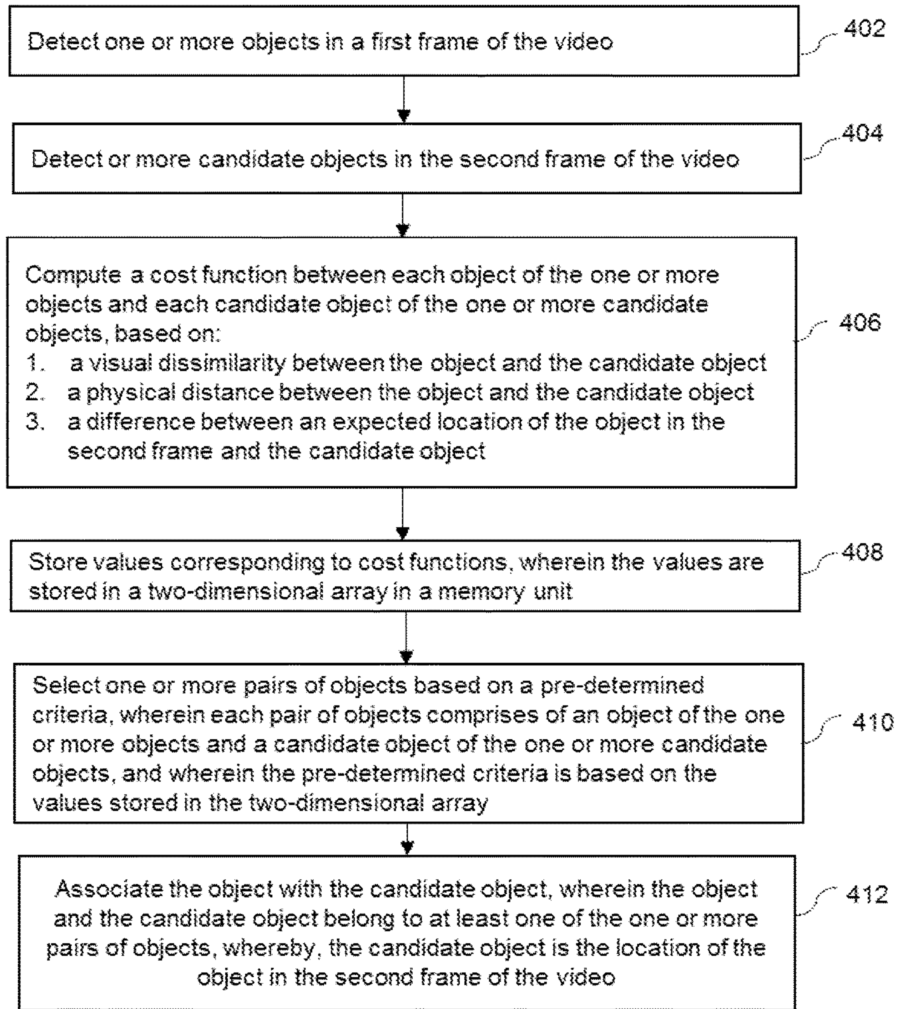
Method Flowchart – Object Detection and Tracking
