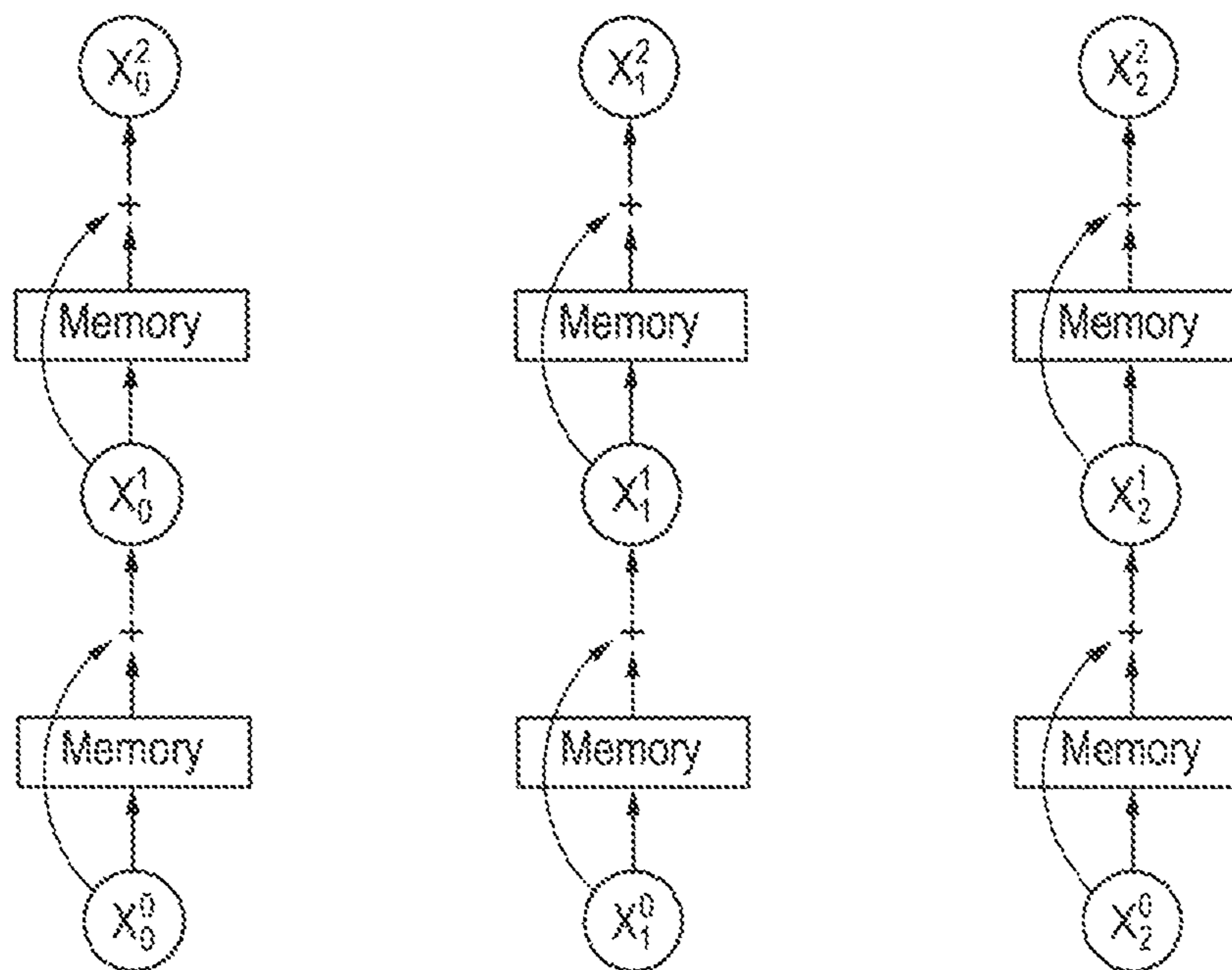
Neural Network
