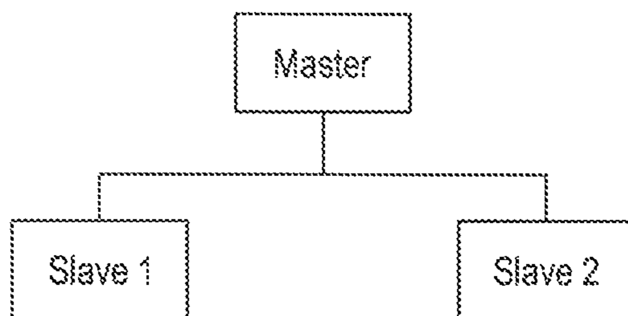
Hierarchical Systems
