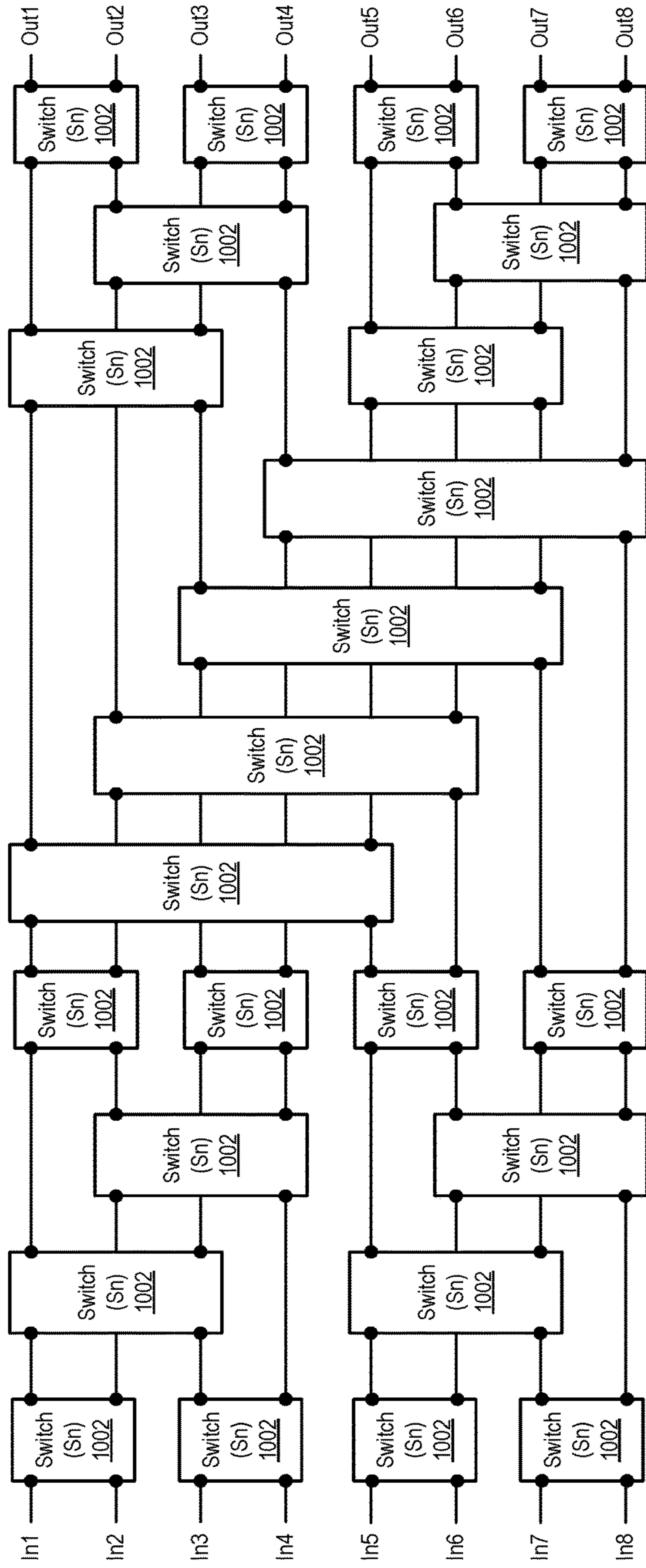
Bitonic Network - 1100
