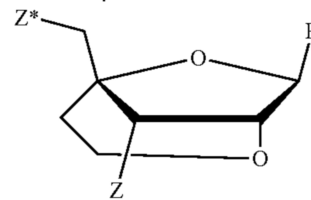
β-D-ENA
