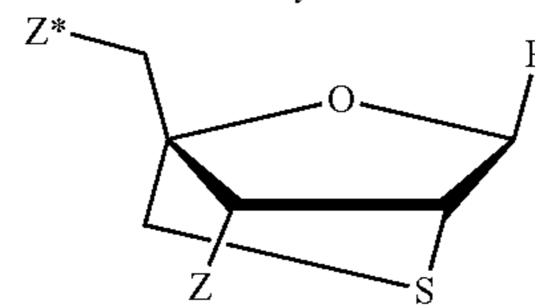
β-D-thio-LNA
