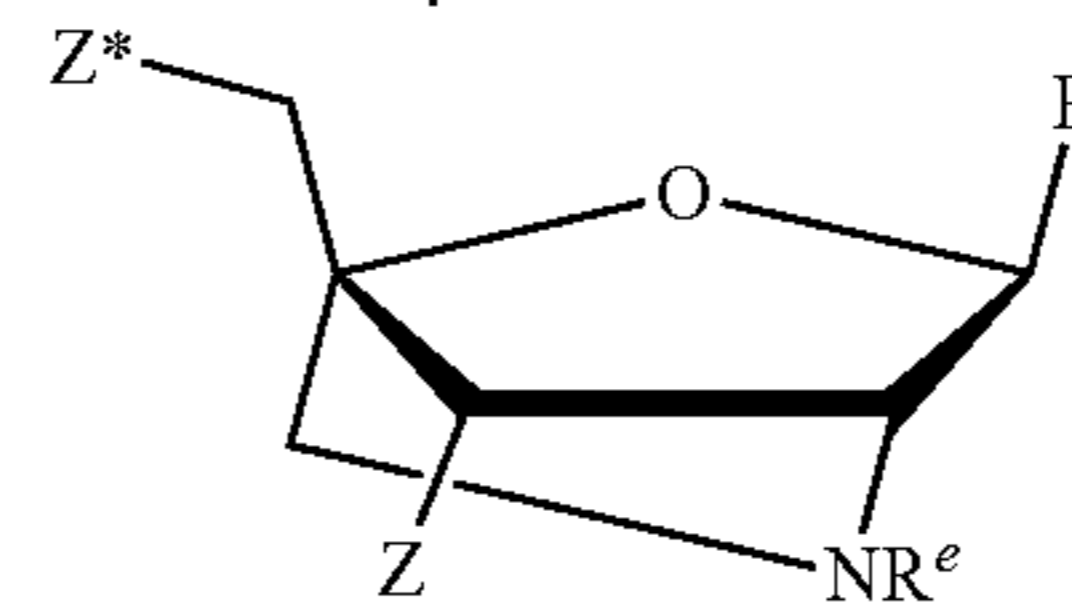
β-D-amino-LNA
