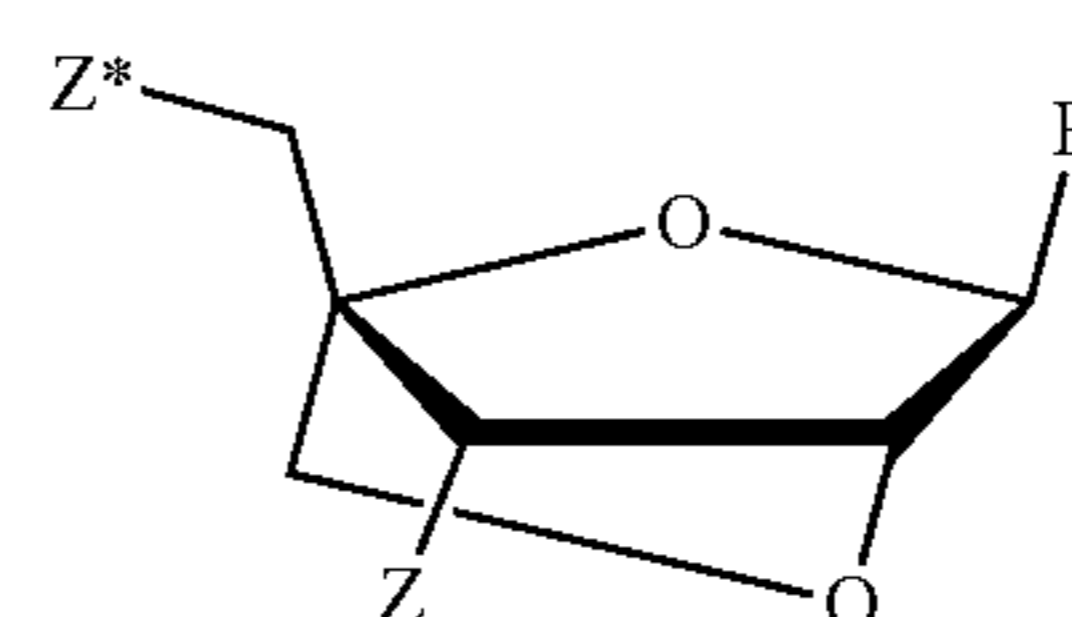
β-D-oxy-LNA
