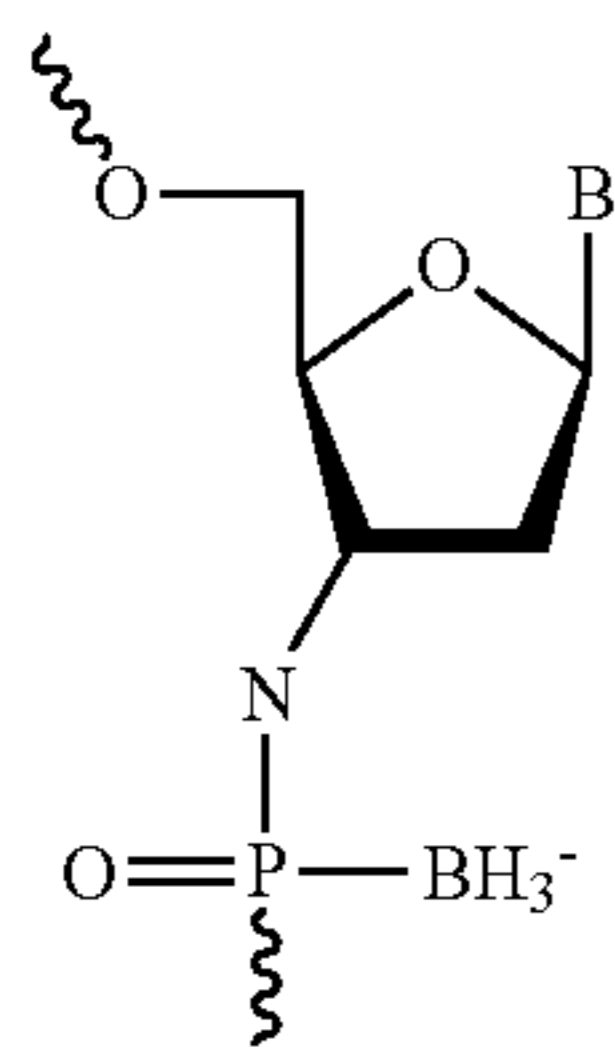
Boranophosphates
