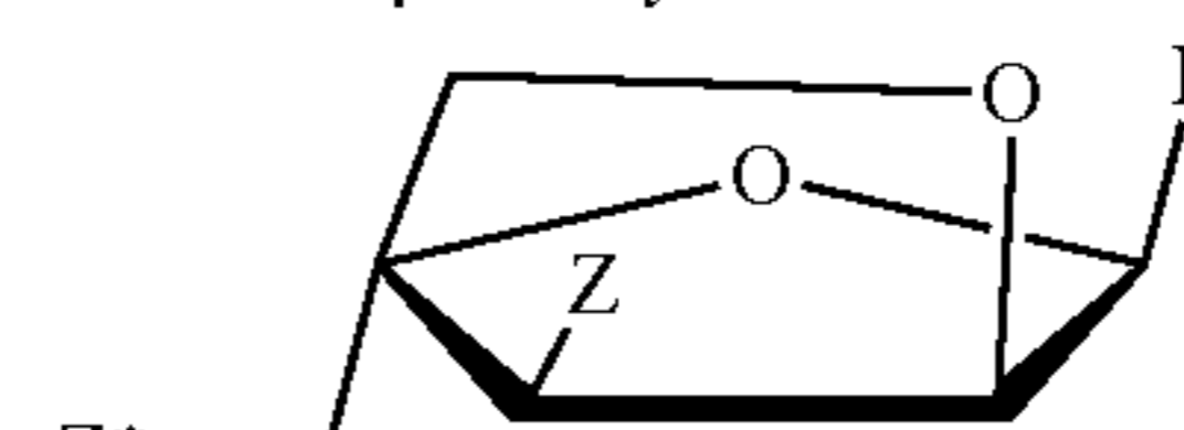
β-D-oxy-LNA
