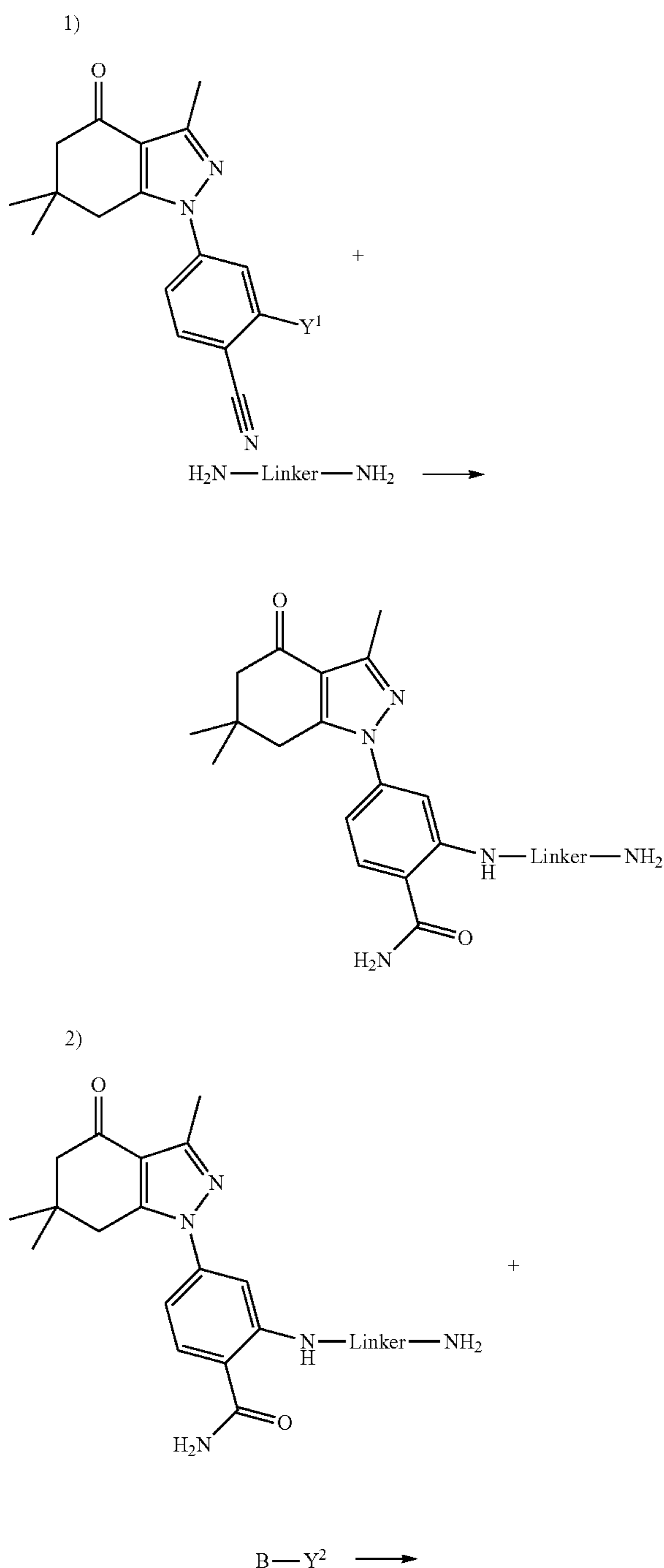
Scheme 1. Exemplary Synthesis
