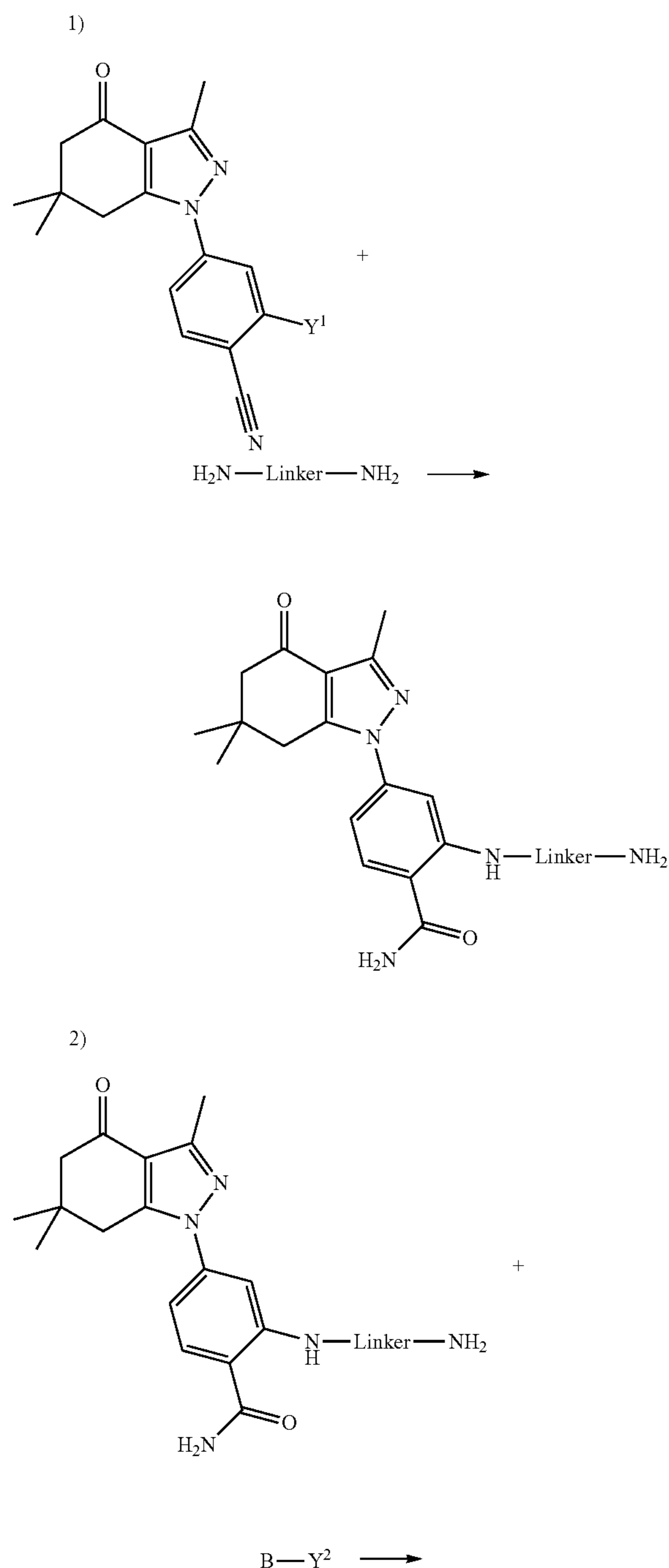
Scheme 1. Exemplary Synthesis
