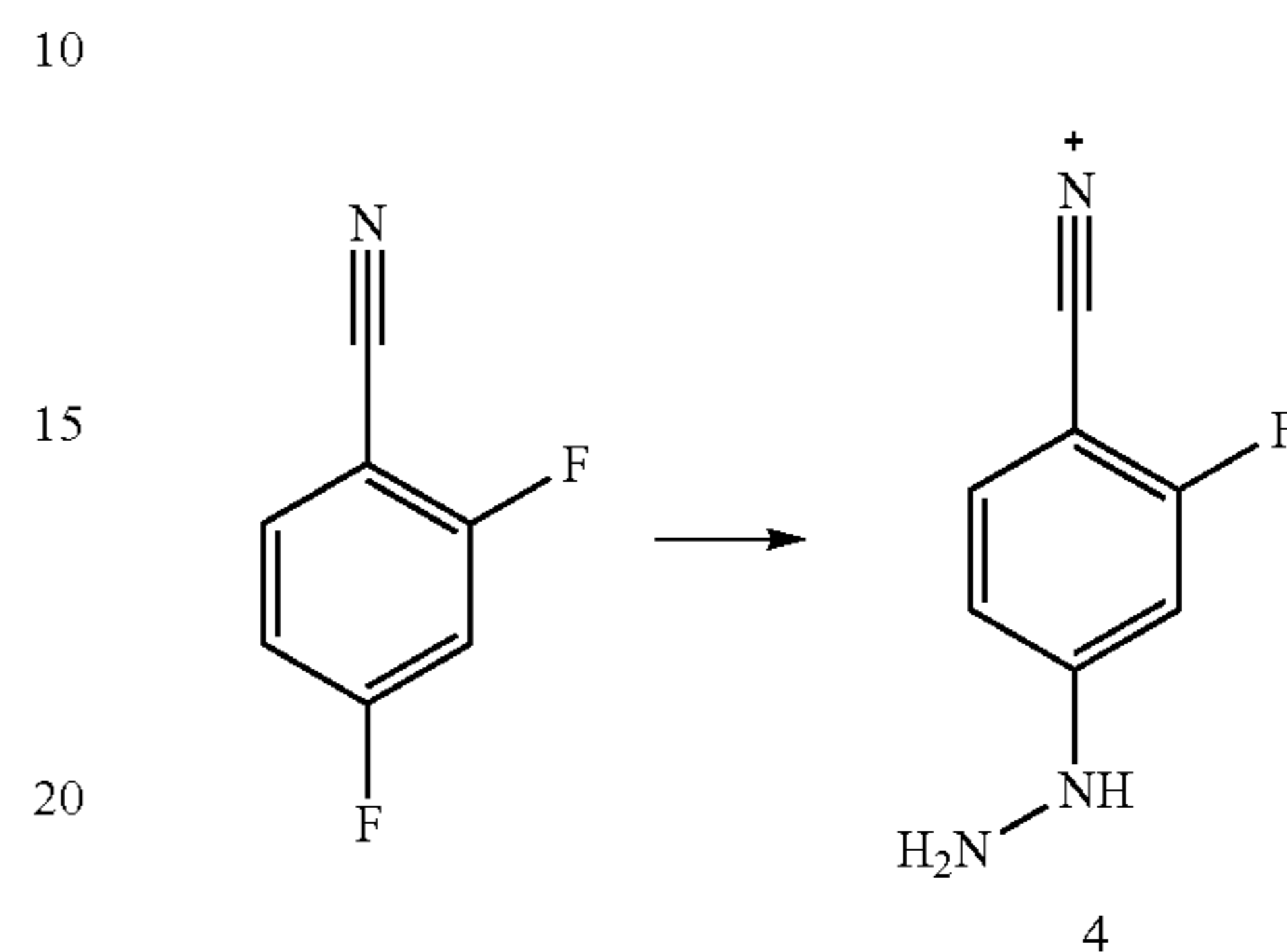
2-Fluoro-4-hydrazinylbenzonitrile (4)
