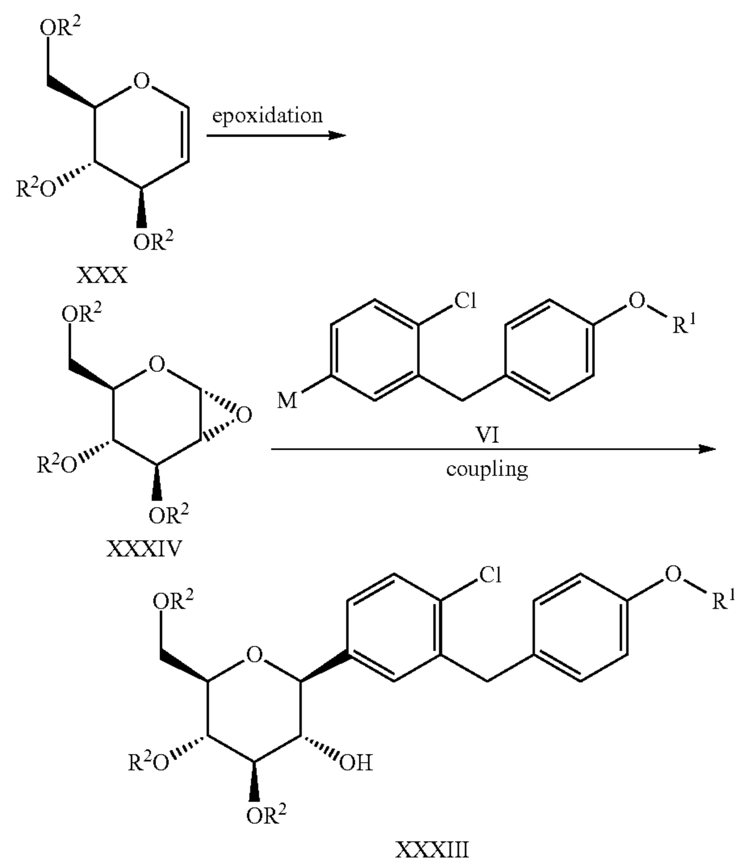
Scheme 2c: Synthesis of C-Glucosides-Approach 3
