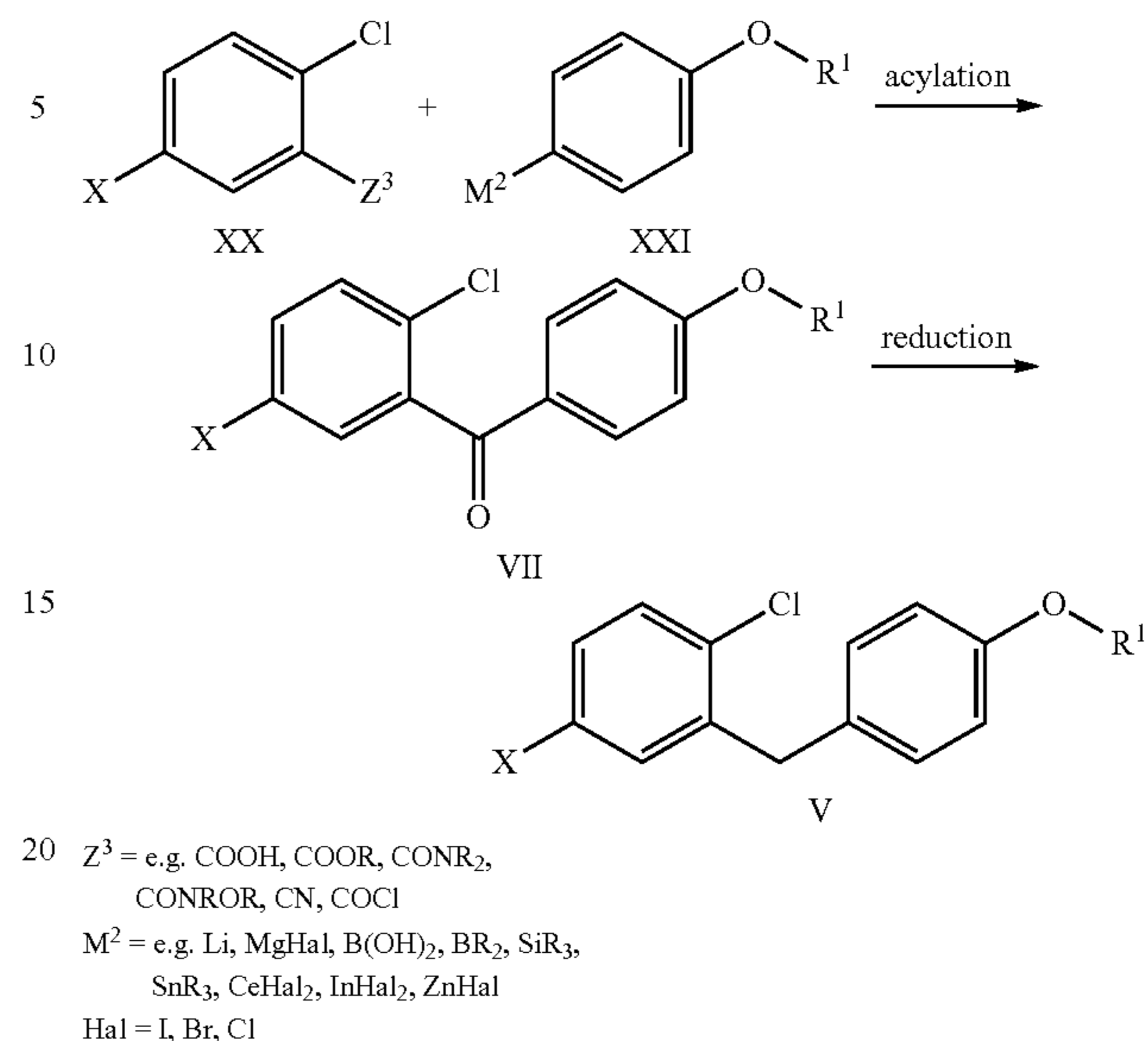
Scheme 8: Synthesis of Aglycon V-Approach 6
