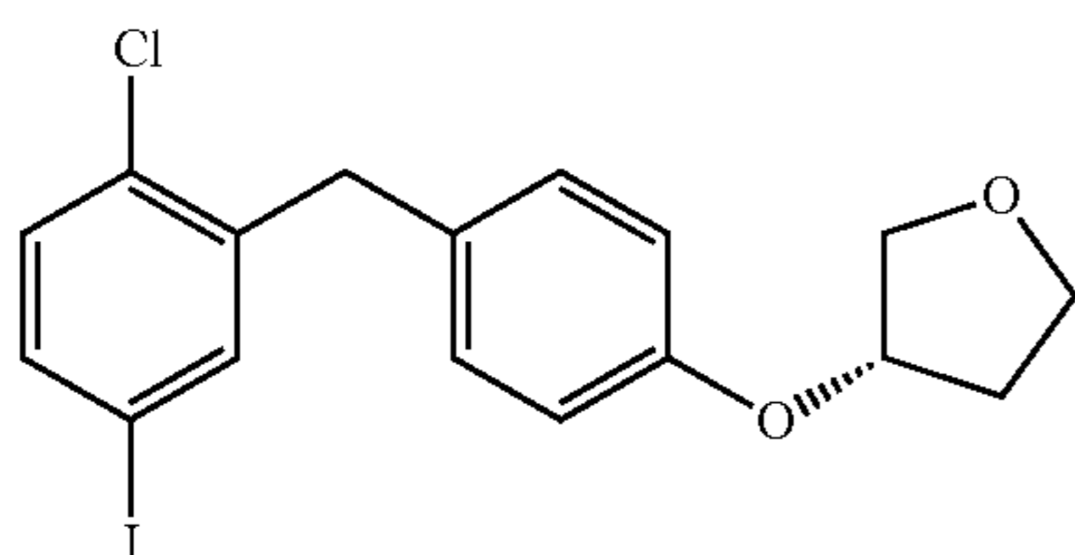
(S)-4-iodo-1-chloro-2-(4-(tetrahydrofuran-3-yloxy)-benzyl)-benzene
