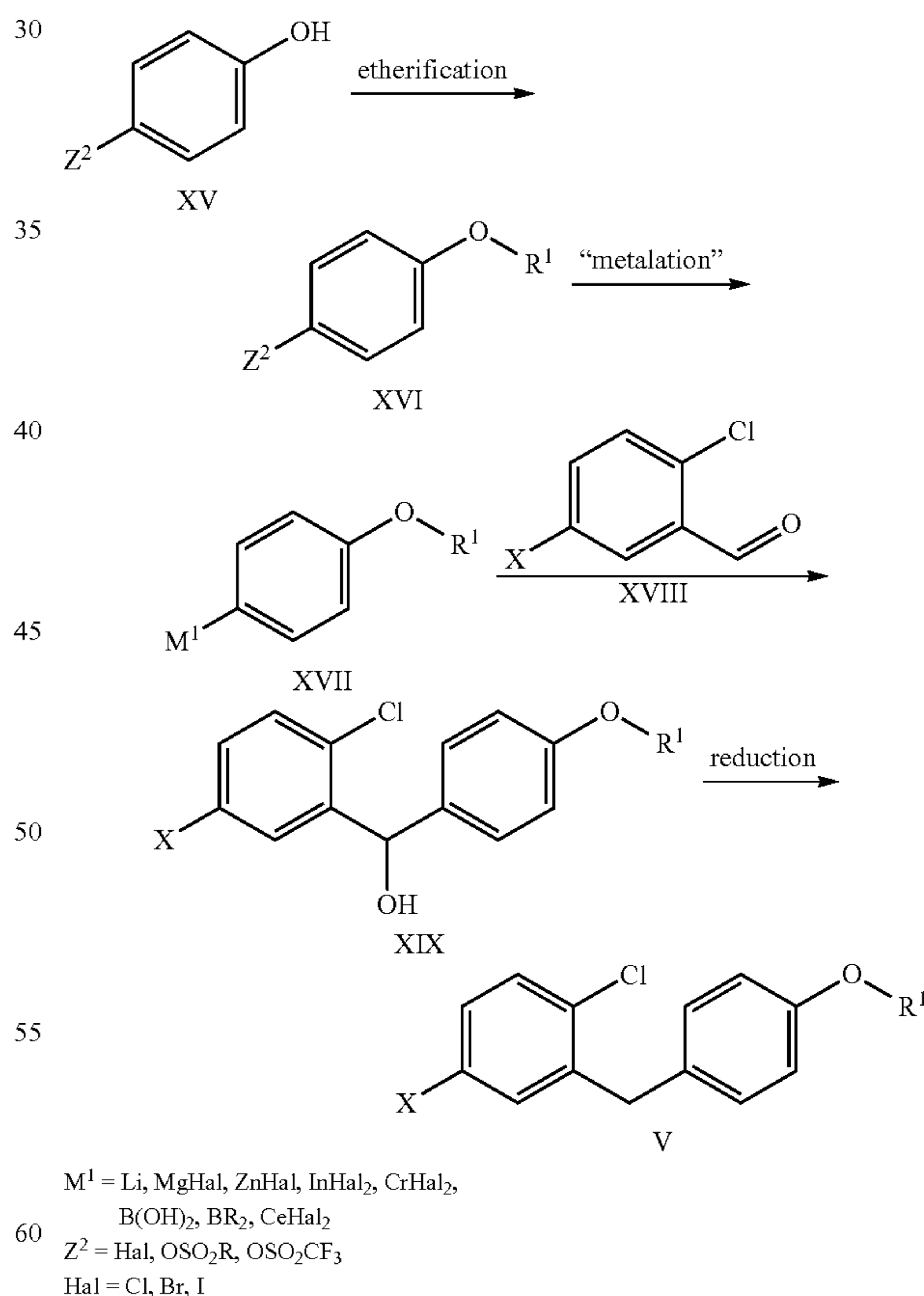
Scheme 7: Synthesis of Aglycon V-Approach 5
