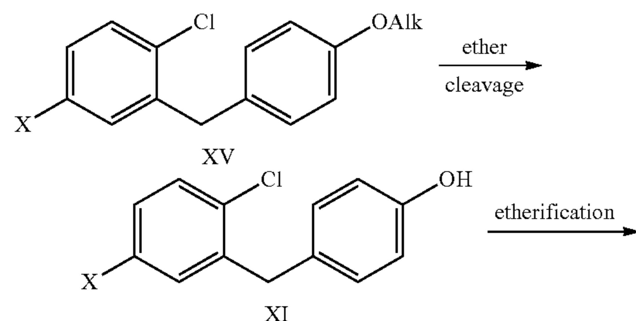
Scheme 4: Synthesis of Aglycon V-Approach 2
