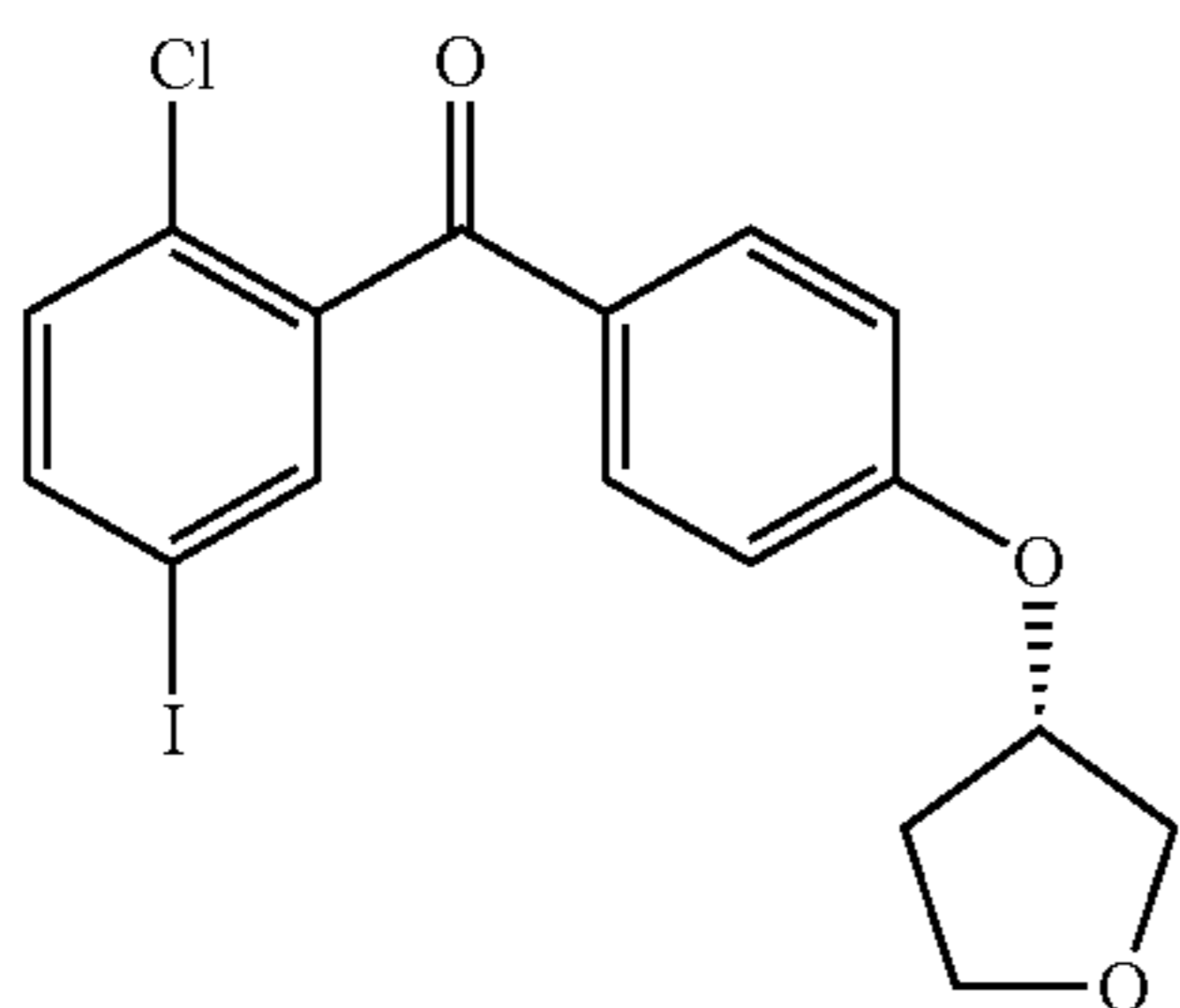
(2-Chloro-5-iodo-phenyl)-{4-[(S)-(tetrahydrofuran-3-yl)oxy]-phenyl}-methanone
