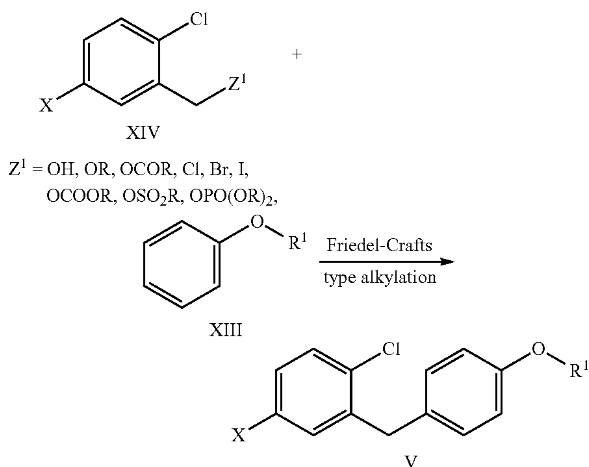
Scheme 6: Synthesis of Aglycon V-Approach 4
