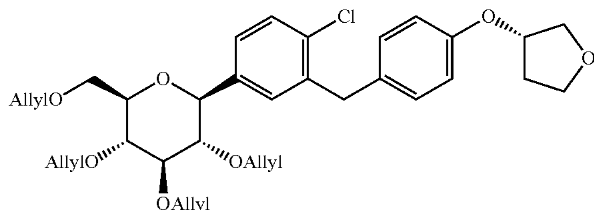
1-Chloro-4-(2,3,4,6-tetra-O-allyl-D-glucopyranos-1-yl)-2-(4-(S)-tetrahydrofuran-3-yloxy-benzyl)-benzene
