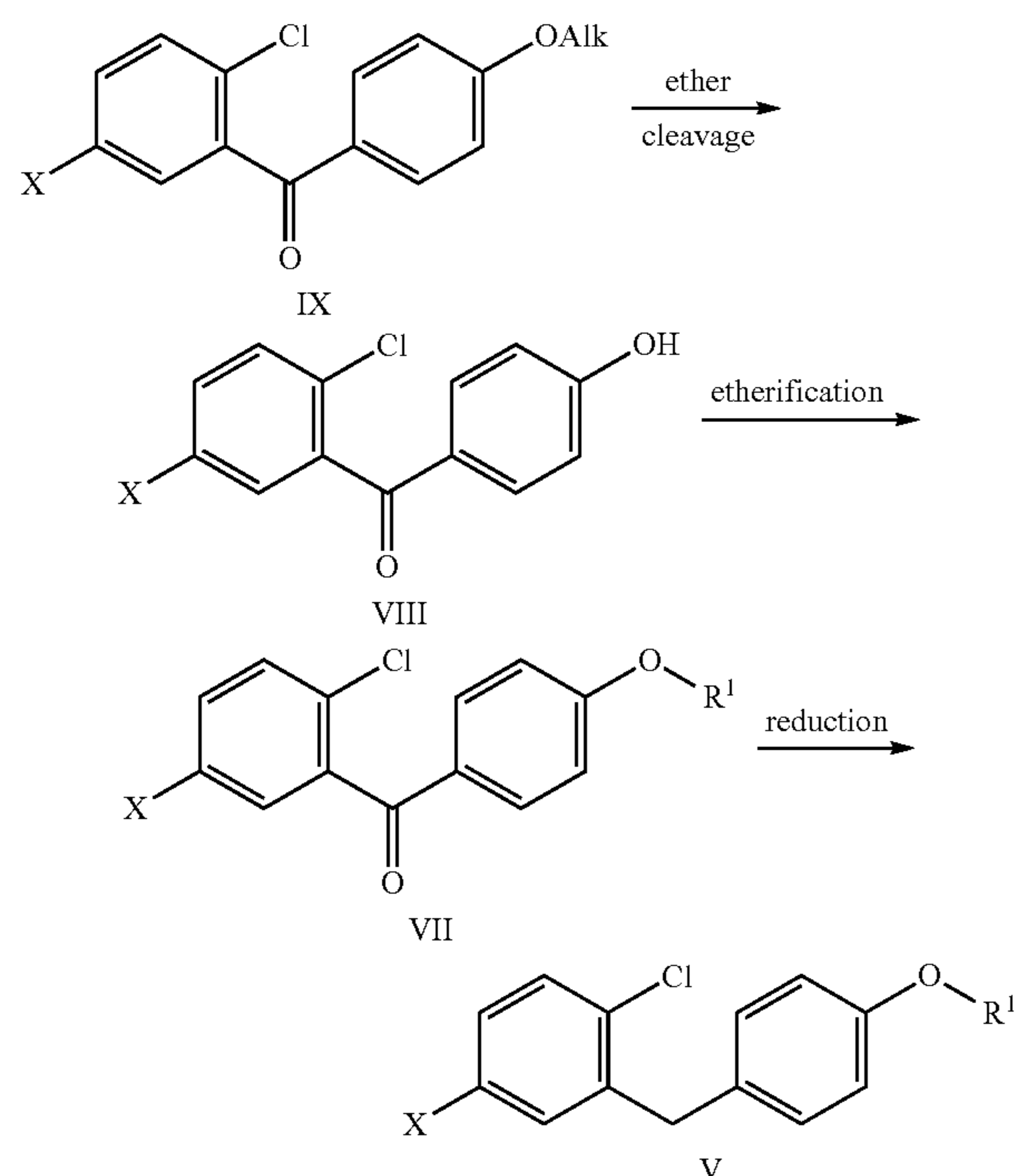
Scheme 3: Synthesis of Aglycon V-Approach 1
