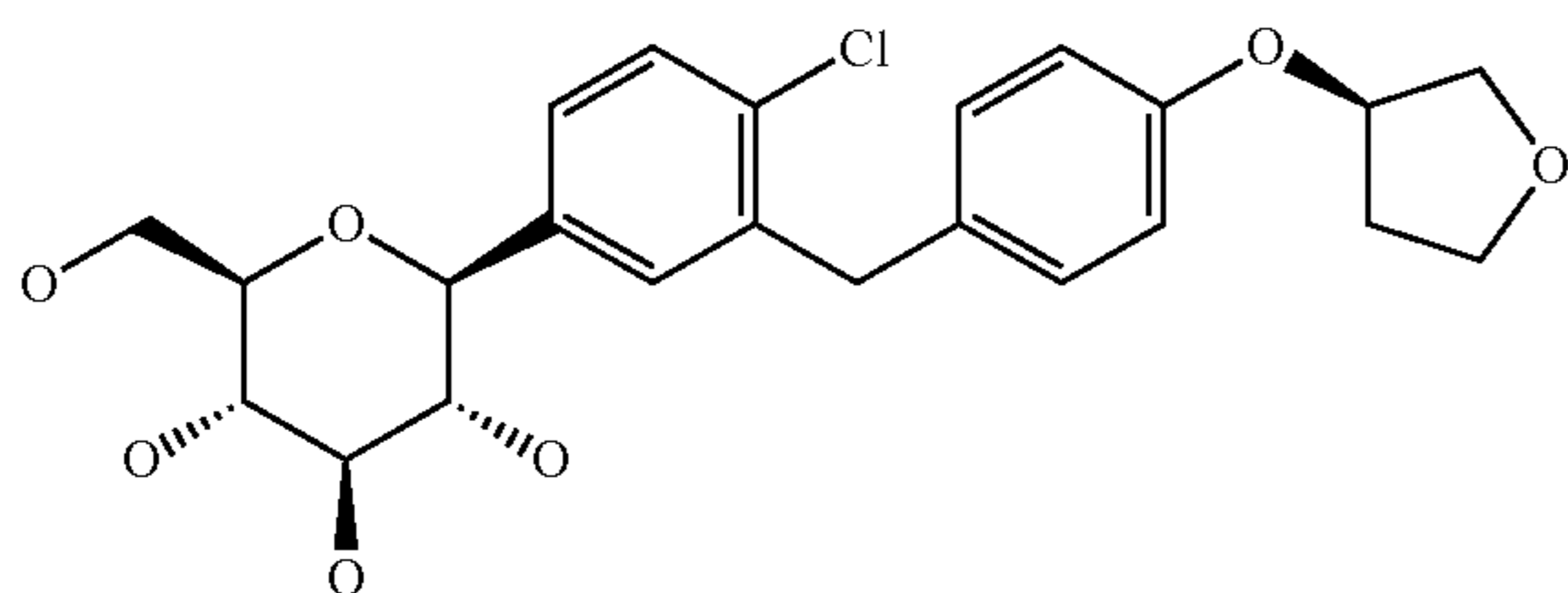
1-Chloro-4-(β-D-glucopyranos-1-yl)-2-(4-(R)-tetrahydrofuran-3-yloxy-benzyl)-benzene
