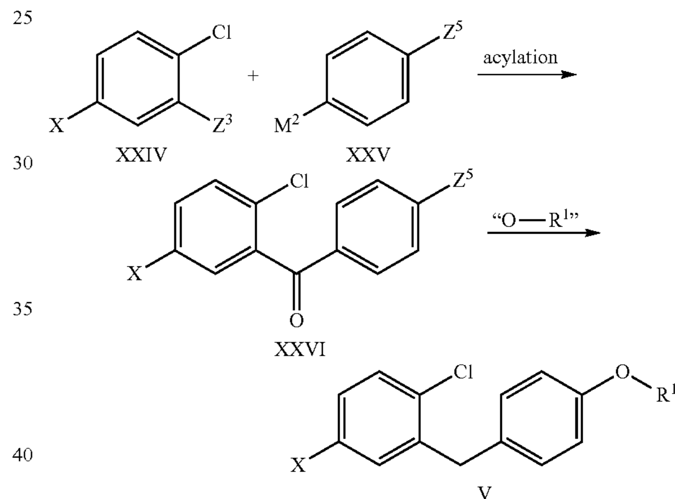
Scheme 10: Synthesis of Aglycon V-Approach 8
