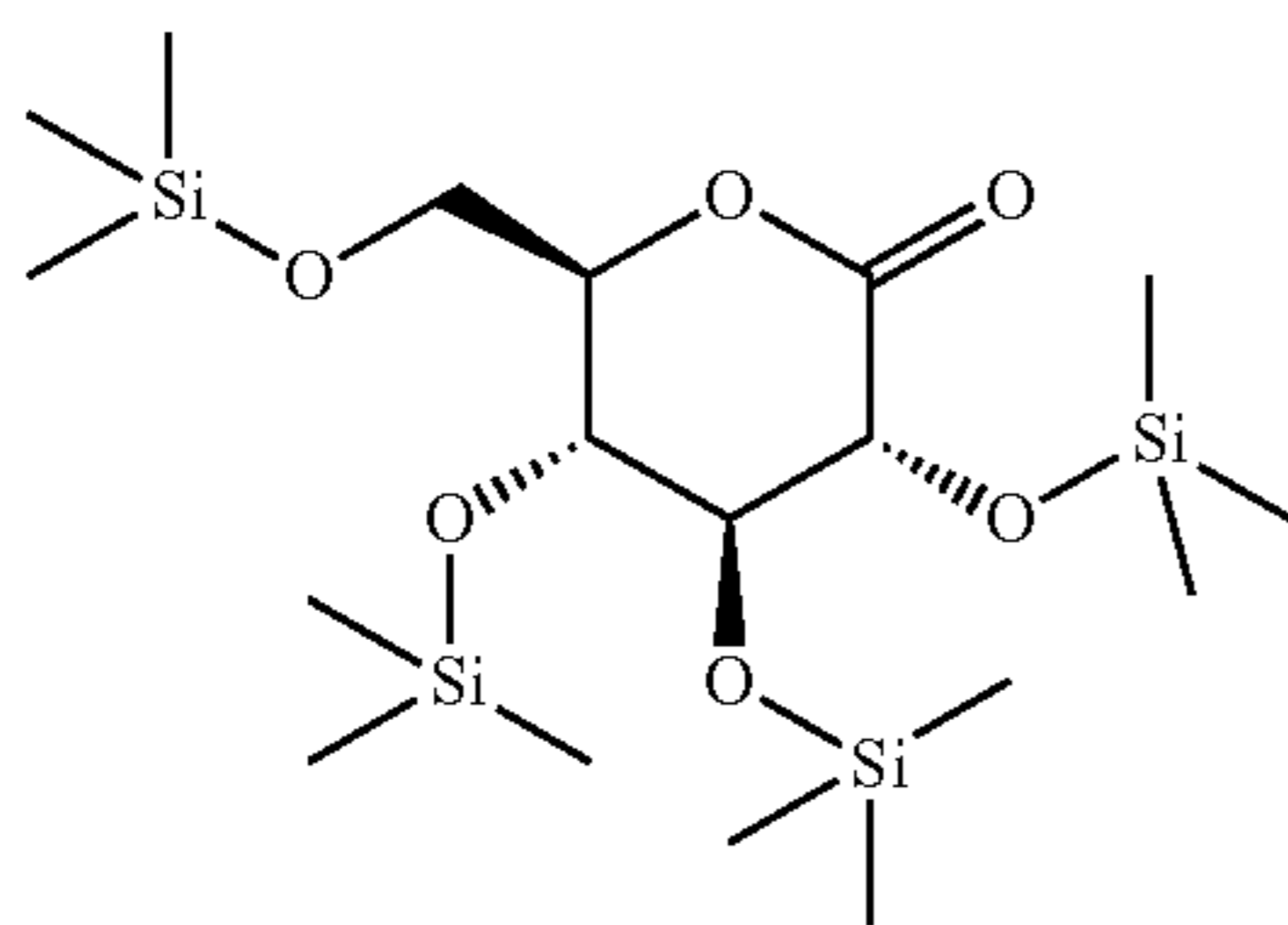
2,3,4,6-tetrakis-O-(trimethylsilyl)-D-glucopyranone
