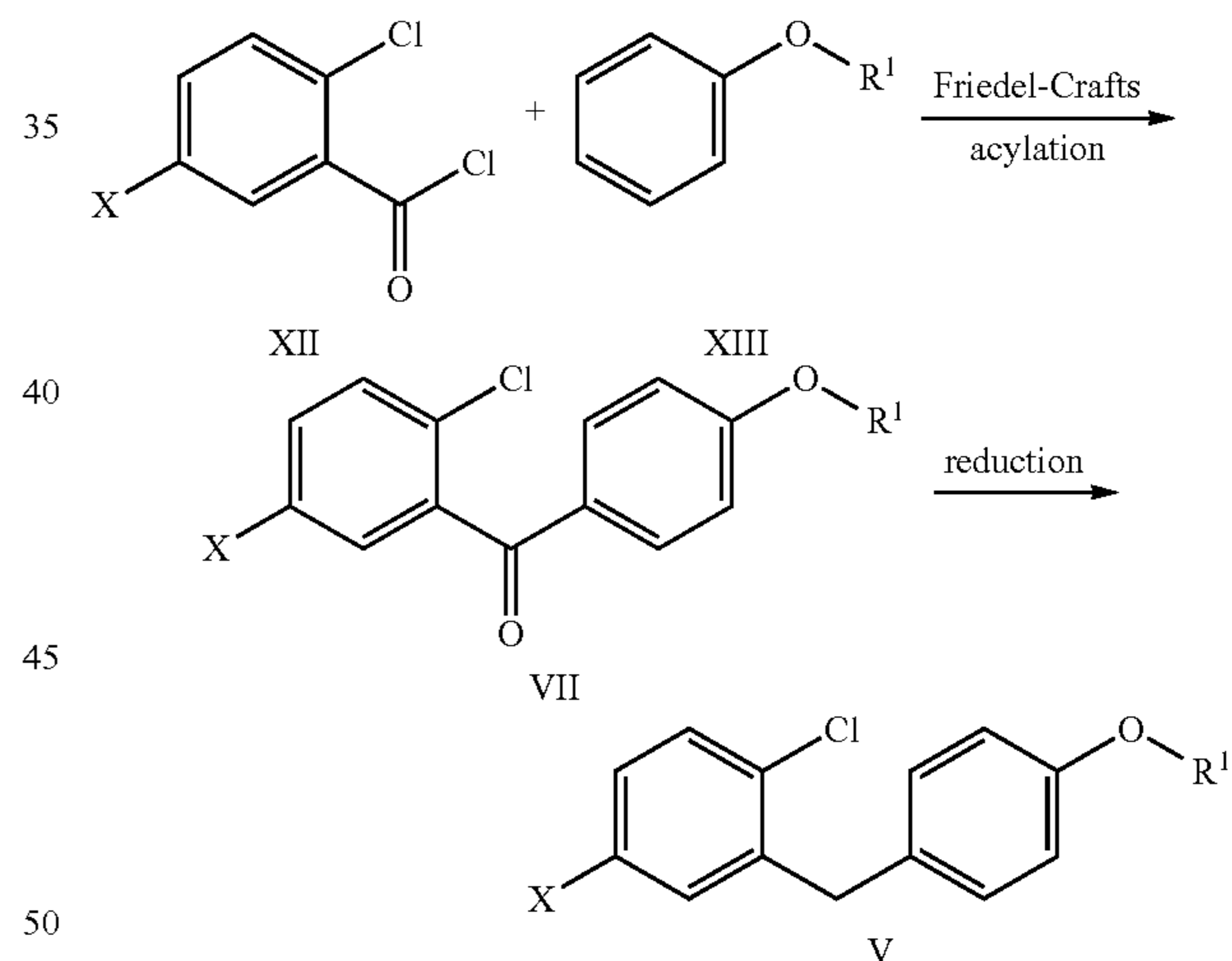
Scheme 5: Synthesis of Aglycon V-Approach 3
