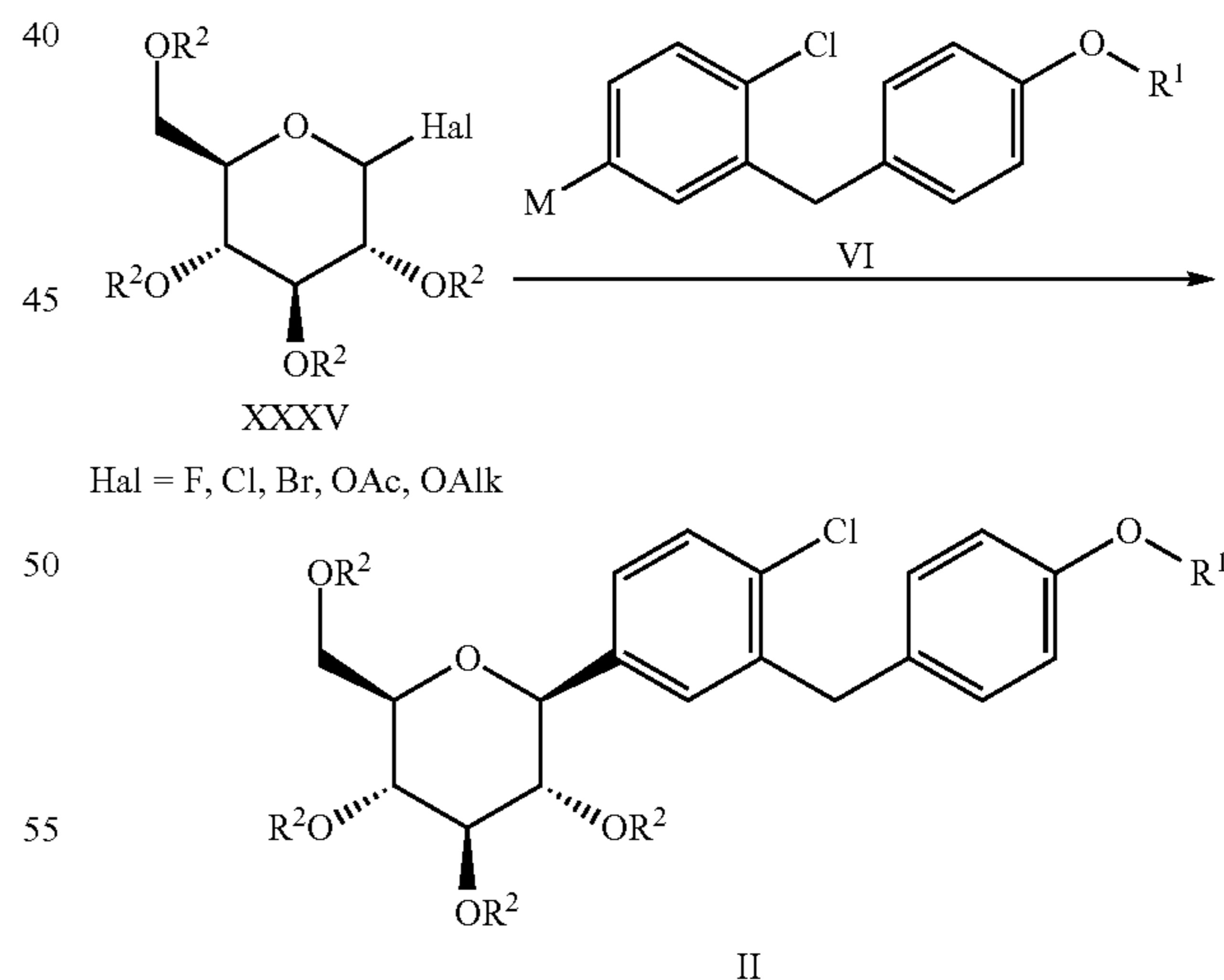
Scheme 2d: Synthesis of C-Glucoside-Approach 4
