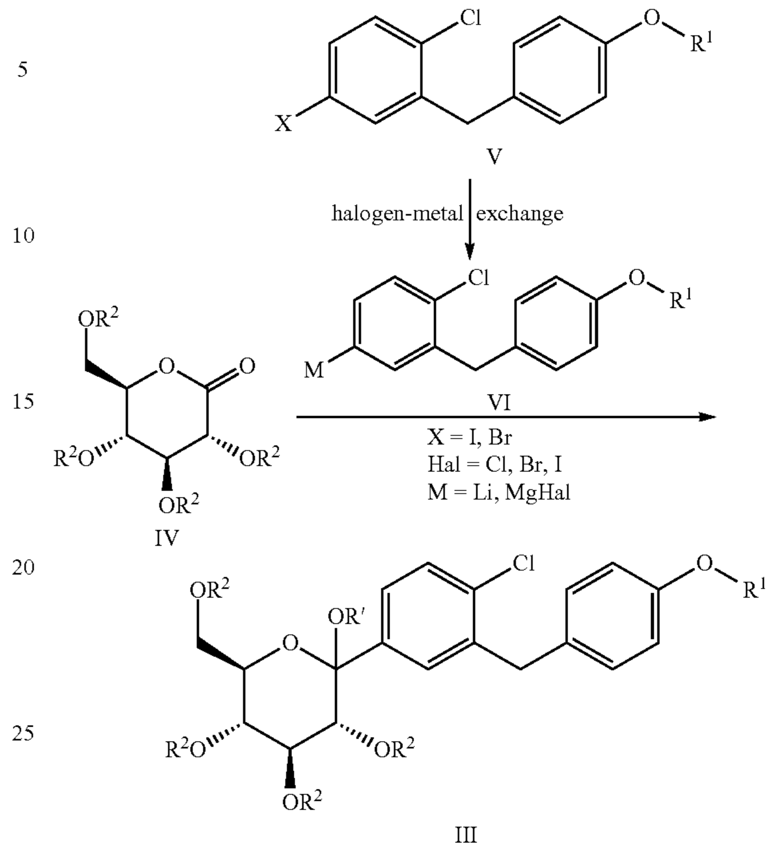
Scheme 2a: Addition of an Organometallic Compound to Gluconolactone
