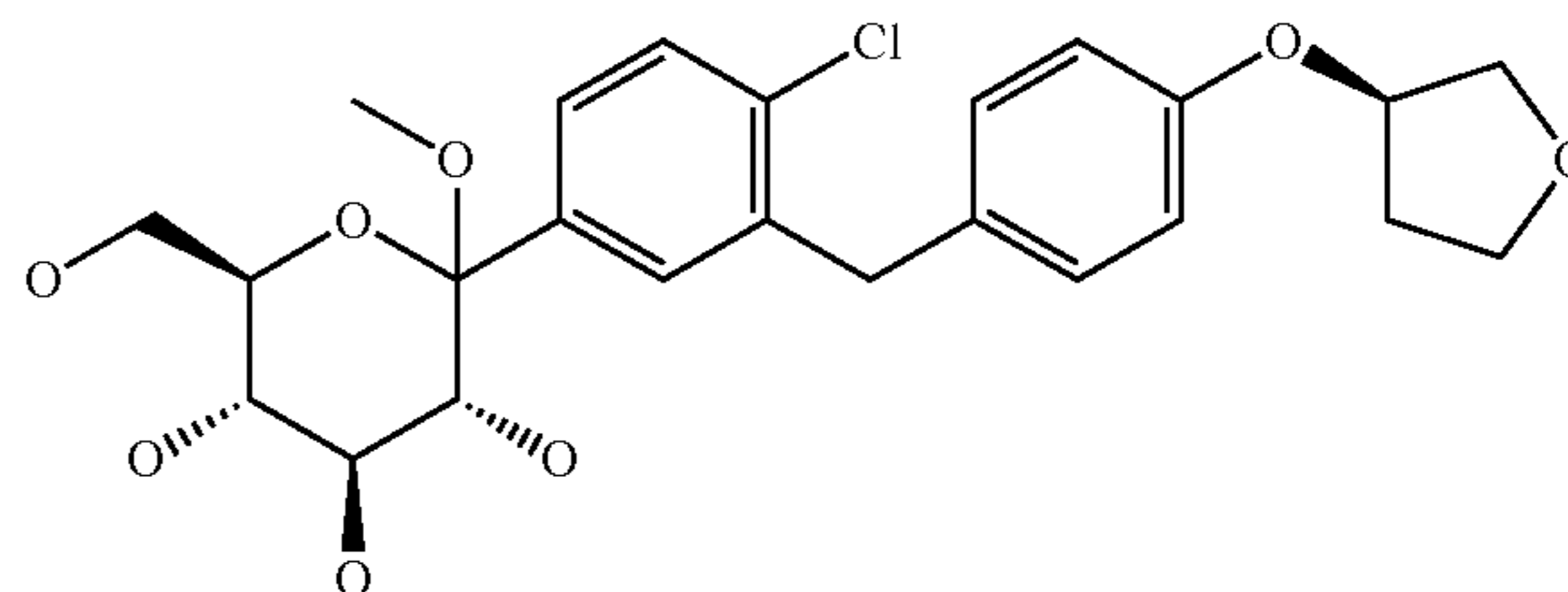
1-Chloro-4-(1-methoxy-D-glucopyranos-1-yl)-2-(4-(R)-tetrahydrofuran-3-yloxy-benzyl)-benzene
