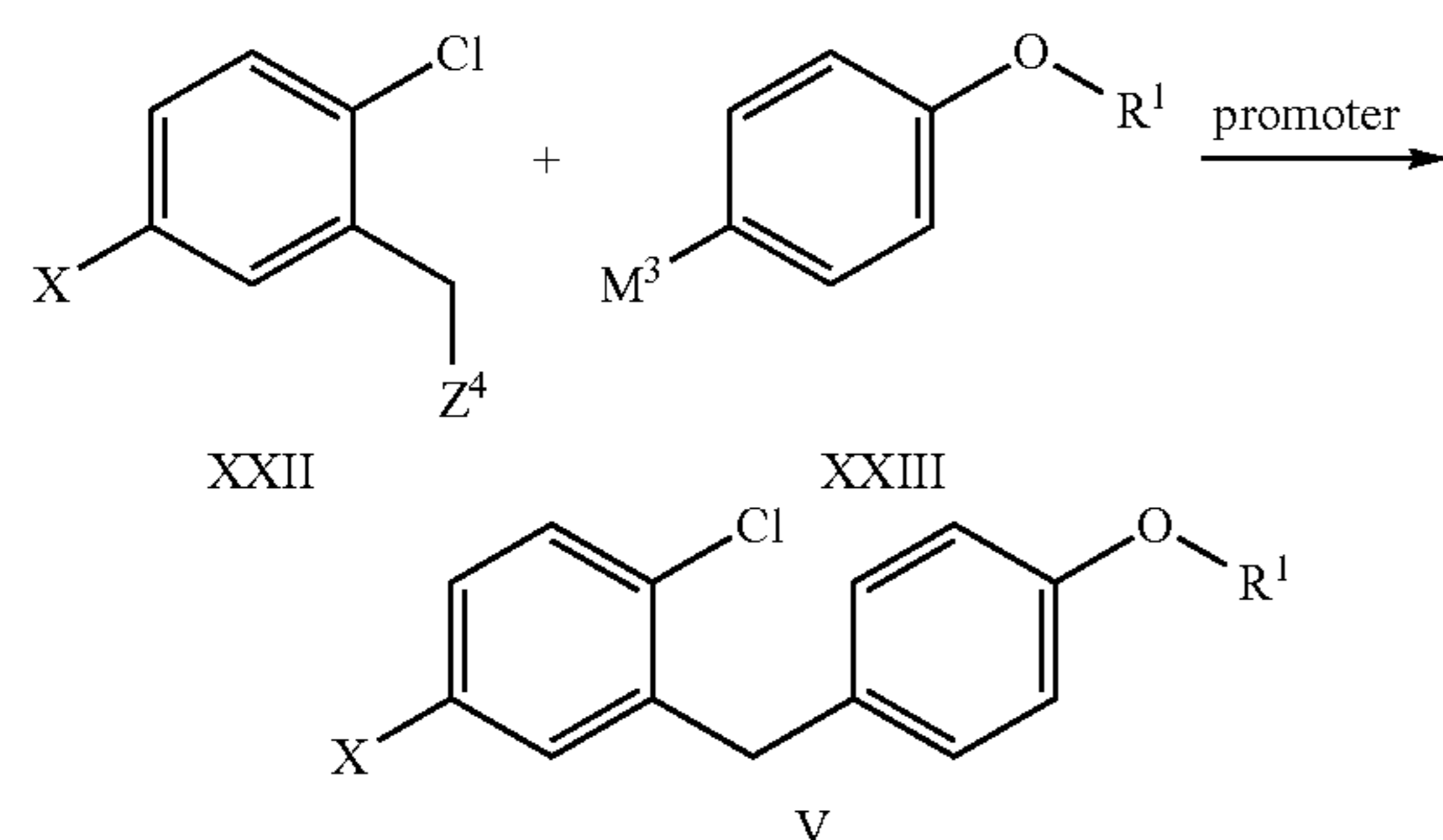
Scheme 9: Synthesis of Aglycon V-Approach 7
