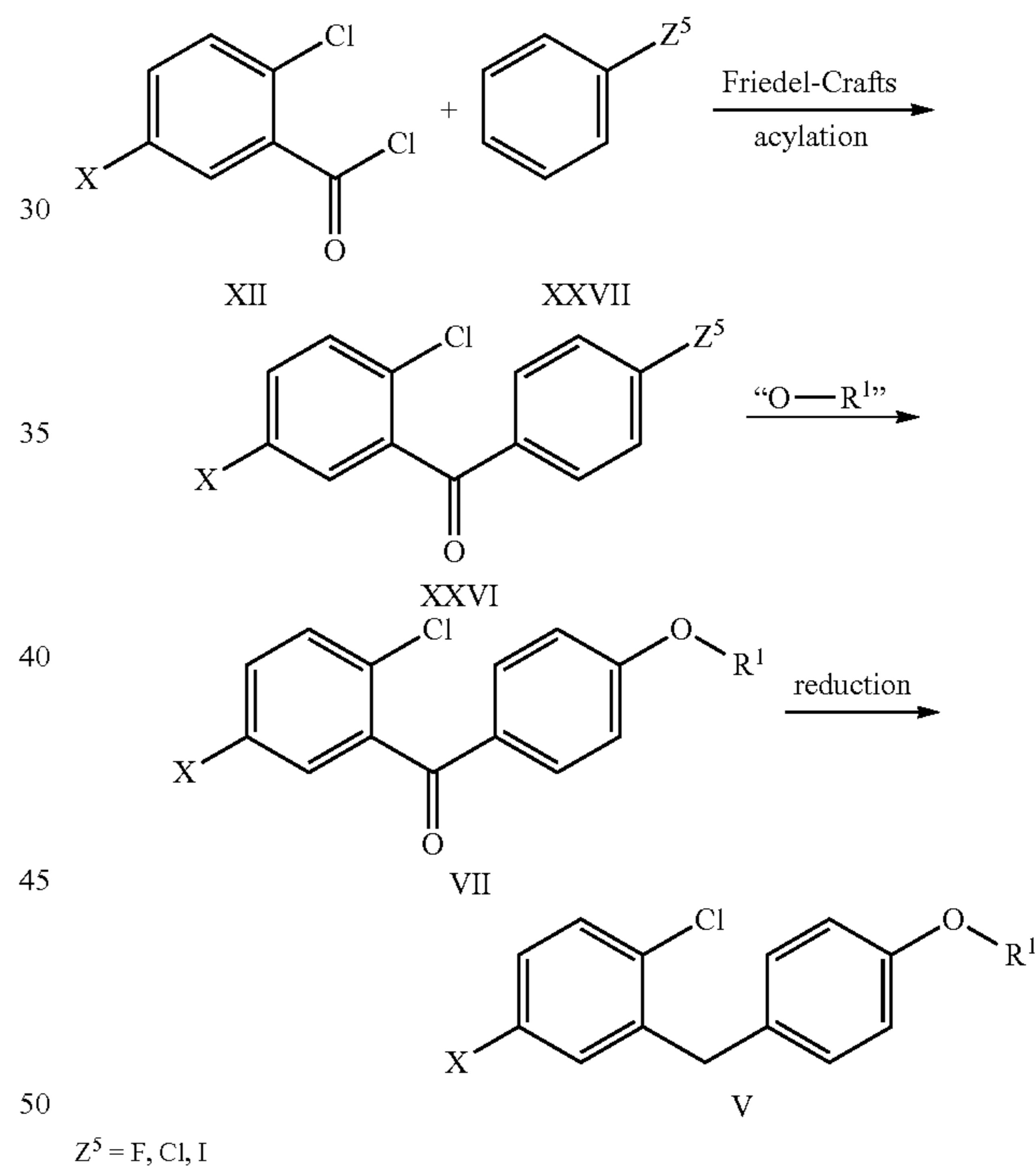
Scheme 11: Synthesis of Aglycon V-Preferred embodiment
