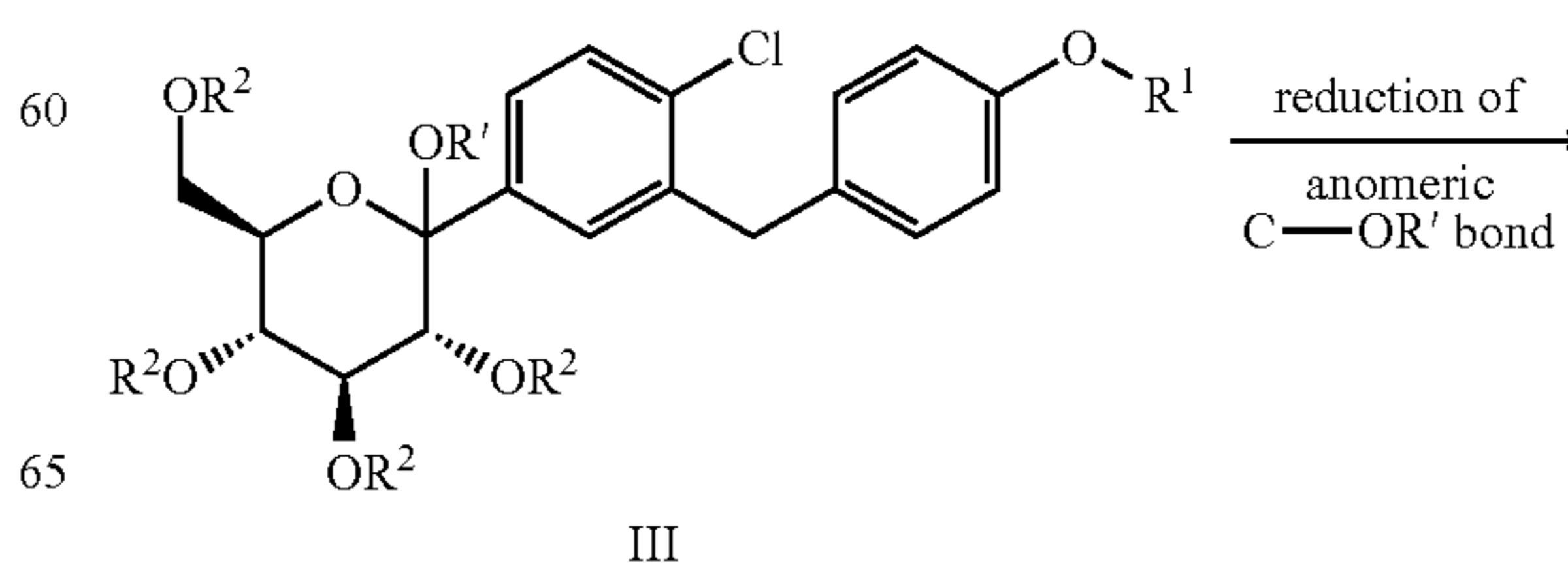
Scheme 1: Reduction of the compound III
