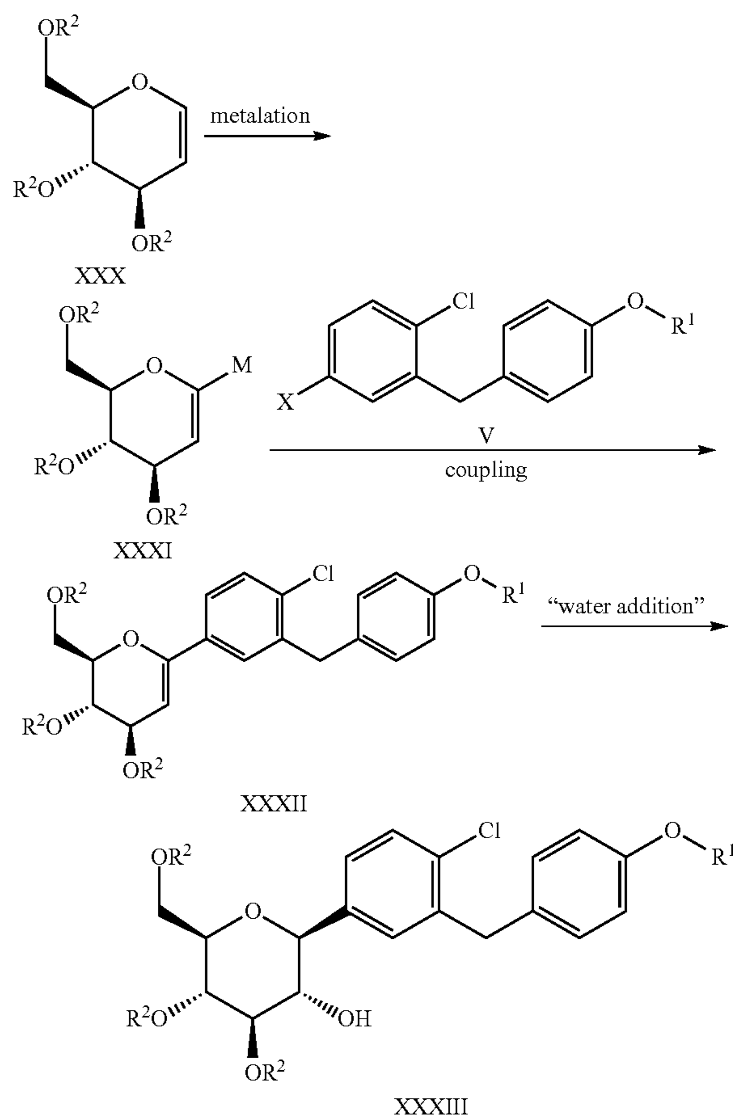
Scheme 2b: Synthesis of C-Glucosides-Approach 2
