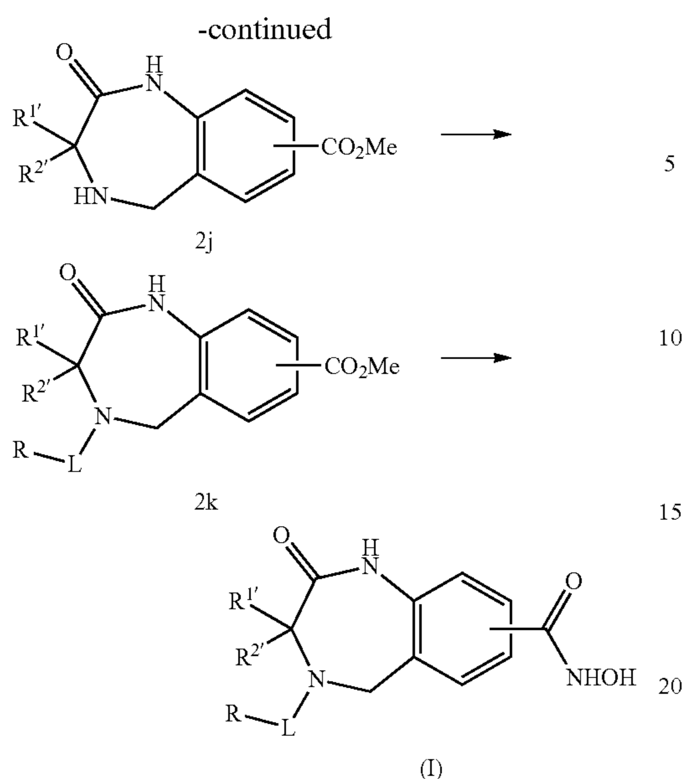
Scheme 3. General synthesis of sulfonamides described in the disclosure.
