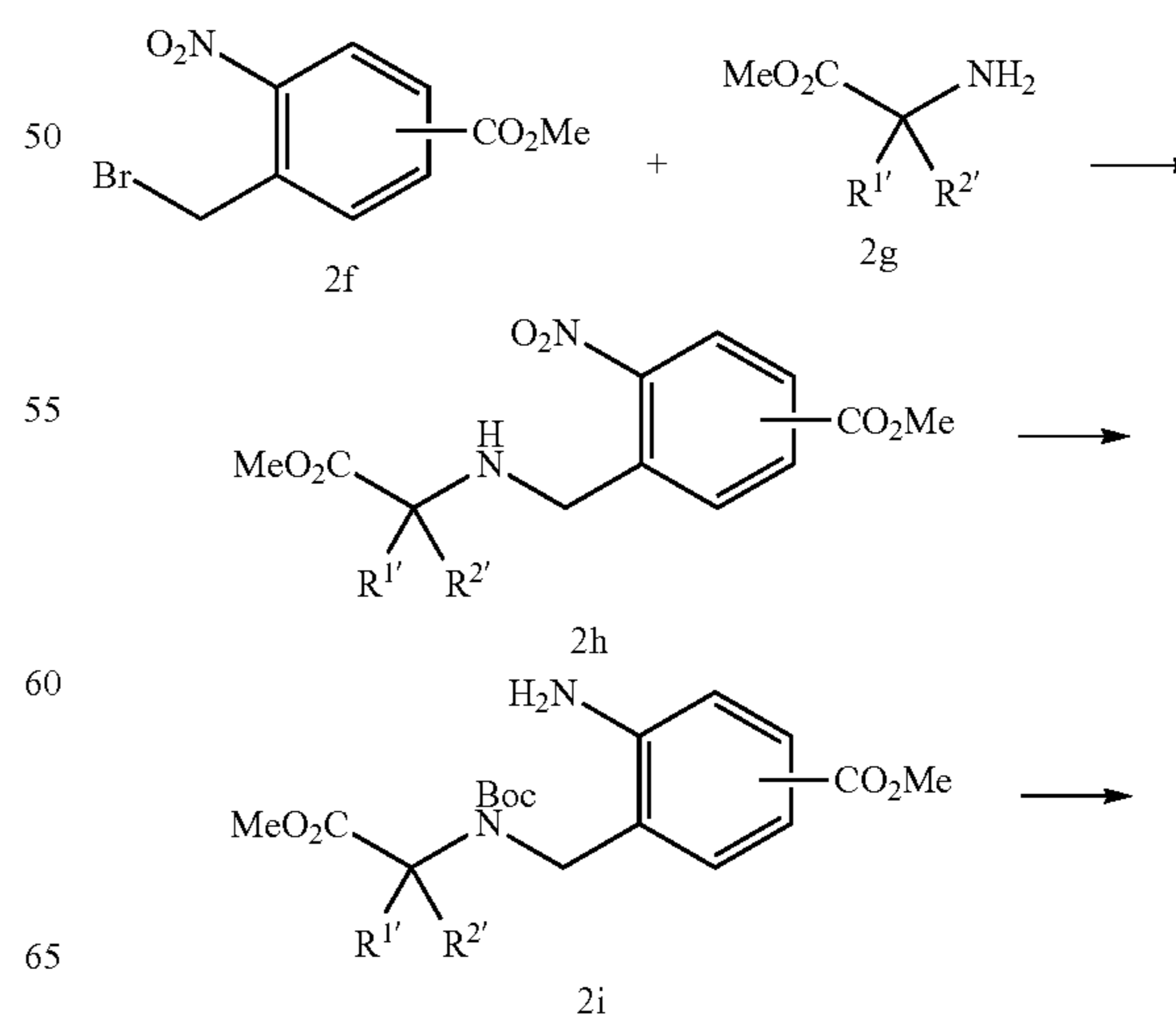
Scheme 2. General synthesis of amides described in the disclosure.
