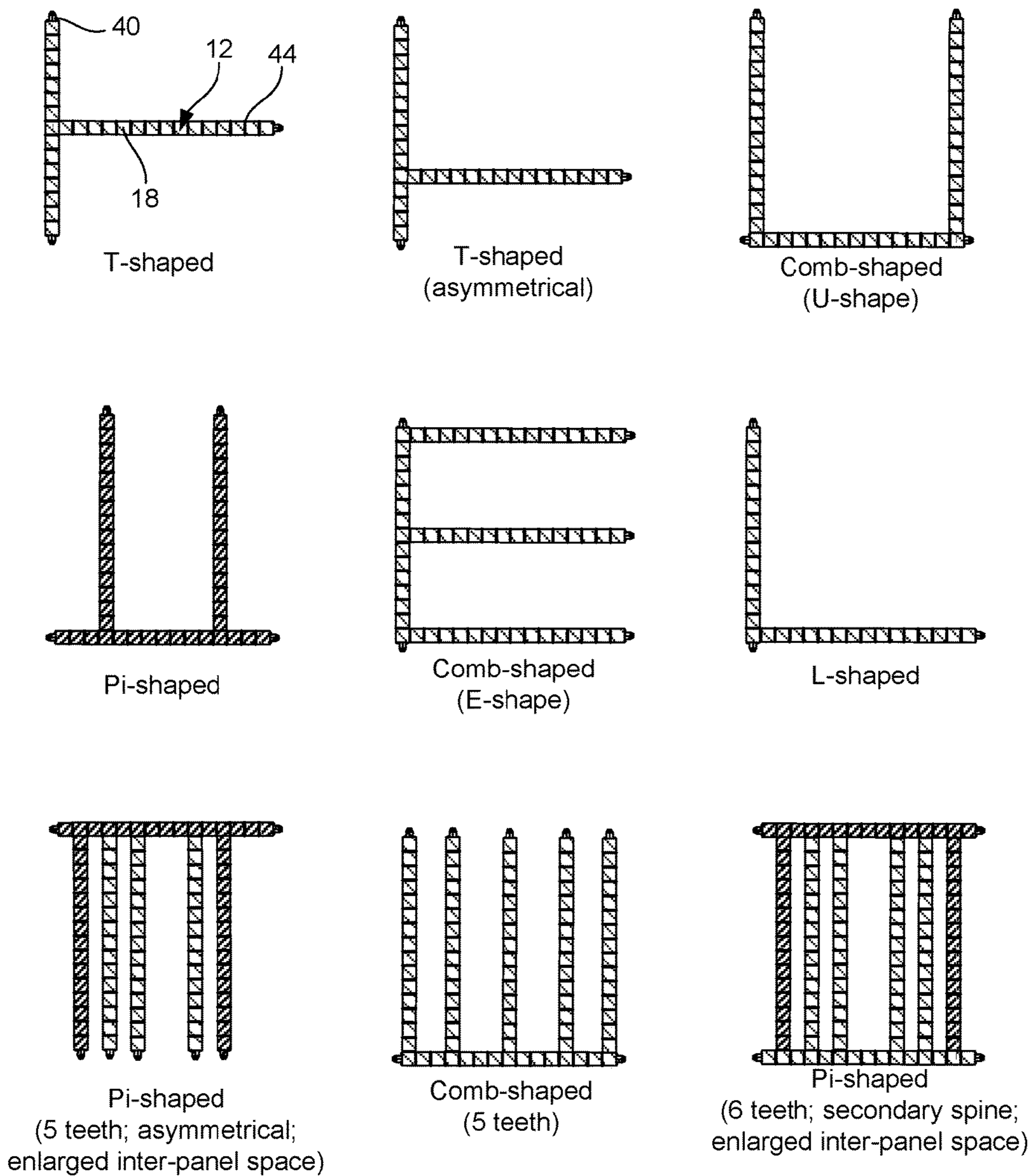
Example Sub-assemblies
