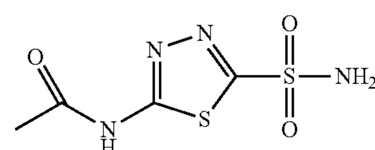
methazolamide
