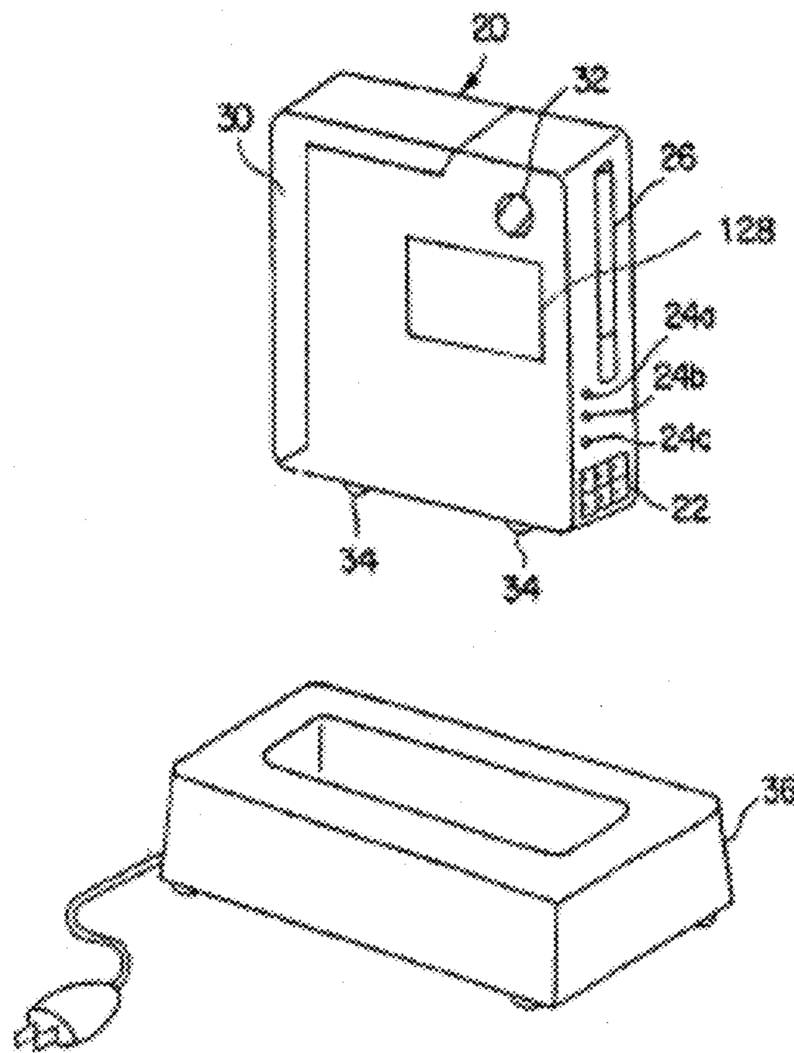
FIG. 2 (PRIOR ART)
