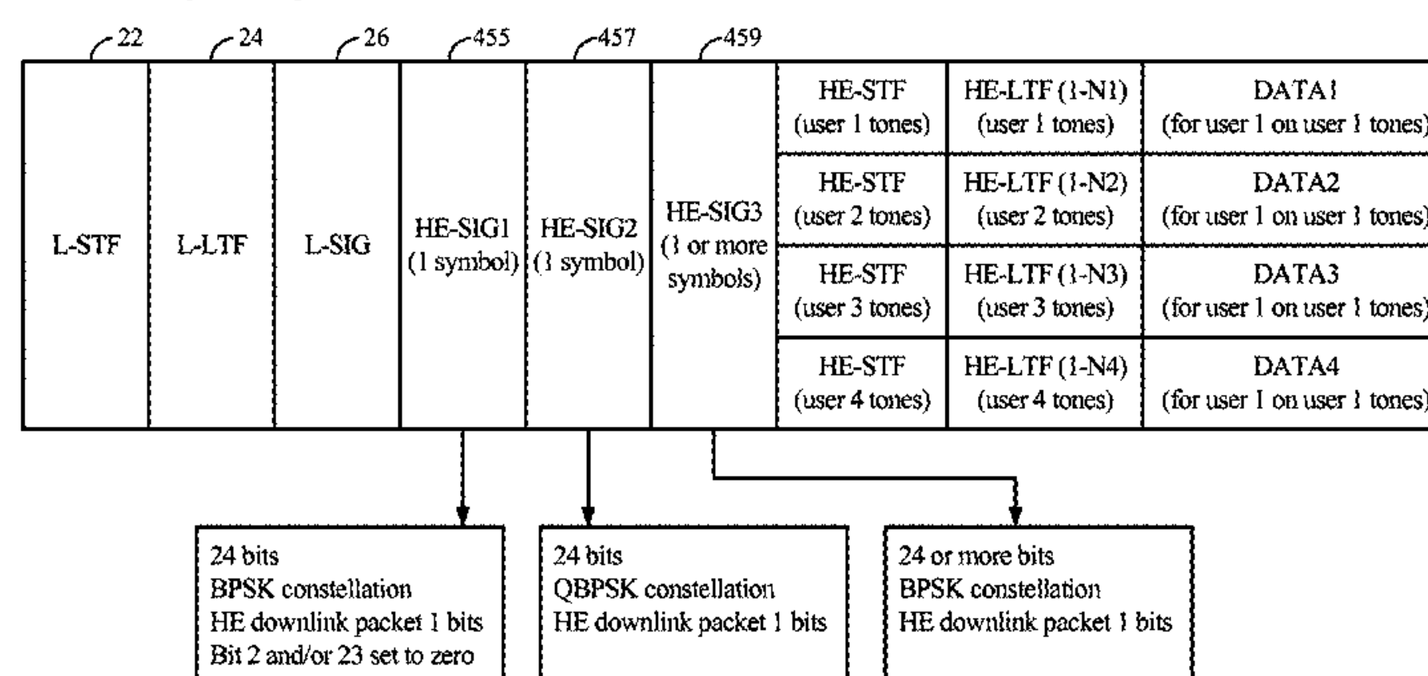
HE downlink packet implementation 3:
