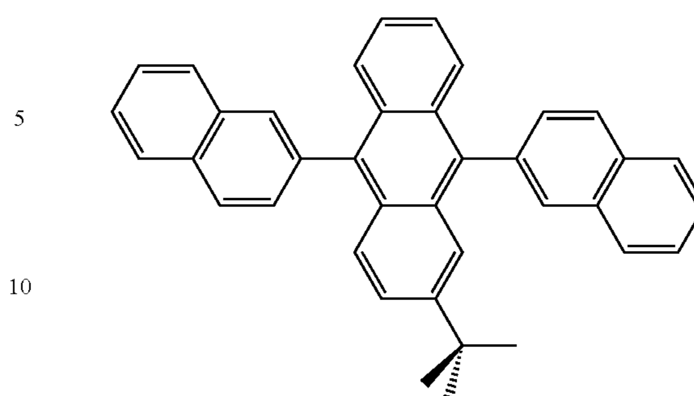
TBADN
