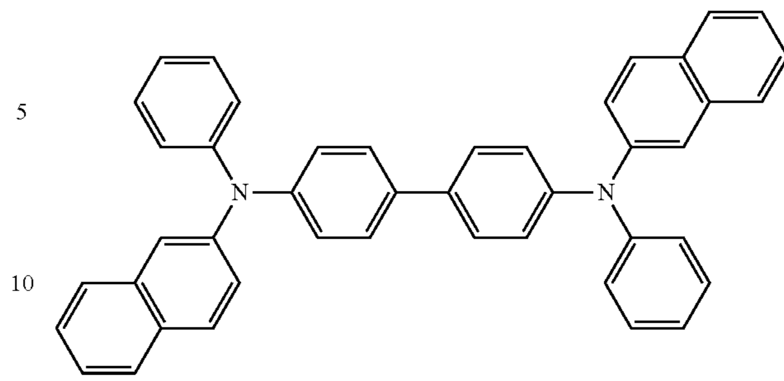
\beta -NPB
