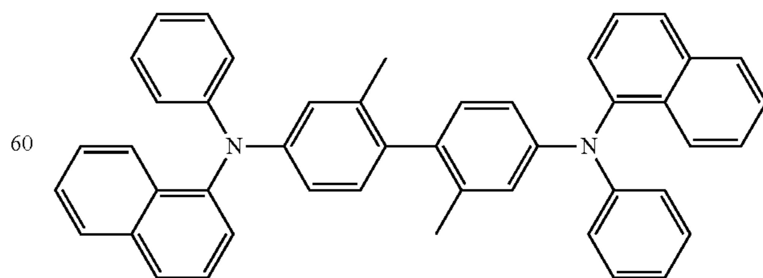
\alpha -NPB
