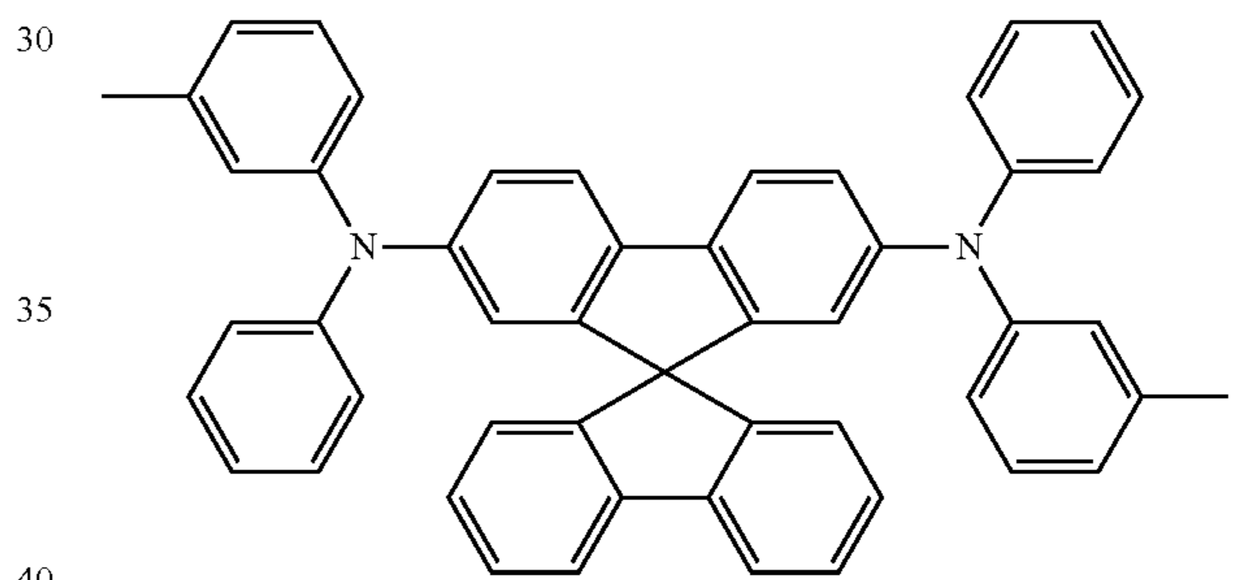
Spiro-TPD
