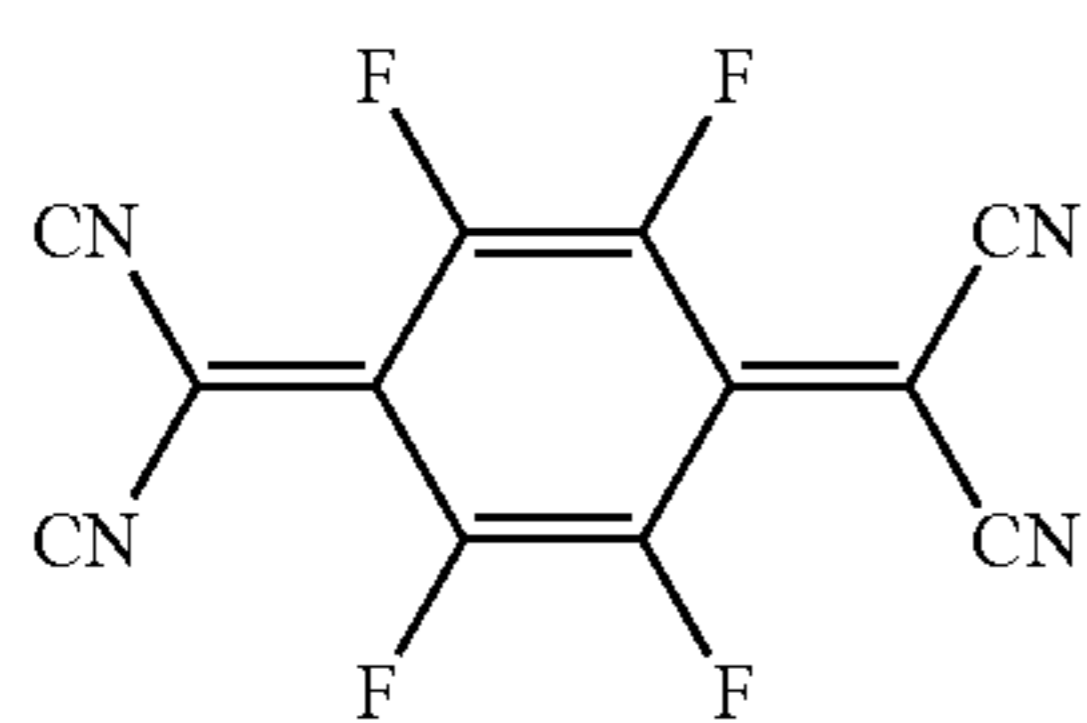
&lt;F4-TCNQ&gt;
