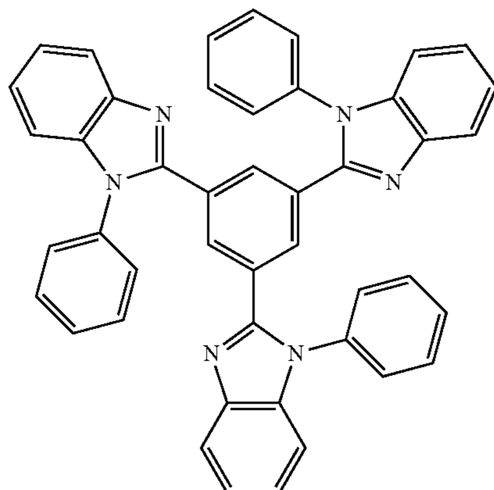
TPBi
