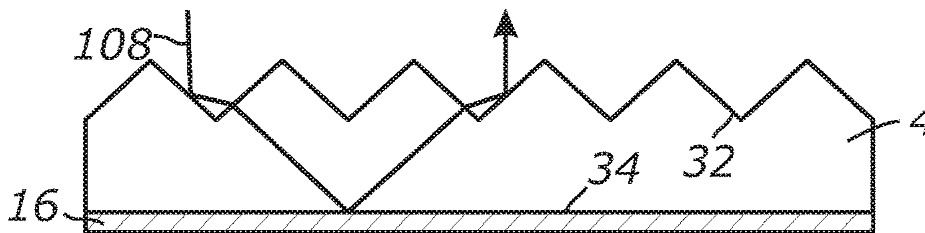
FIG. 2 (PRIOR ART)
