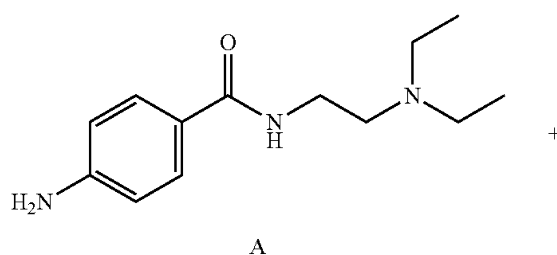
Scheme II
