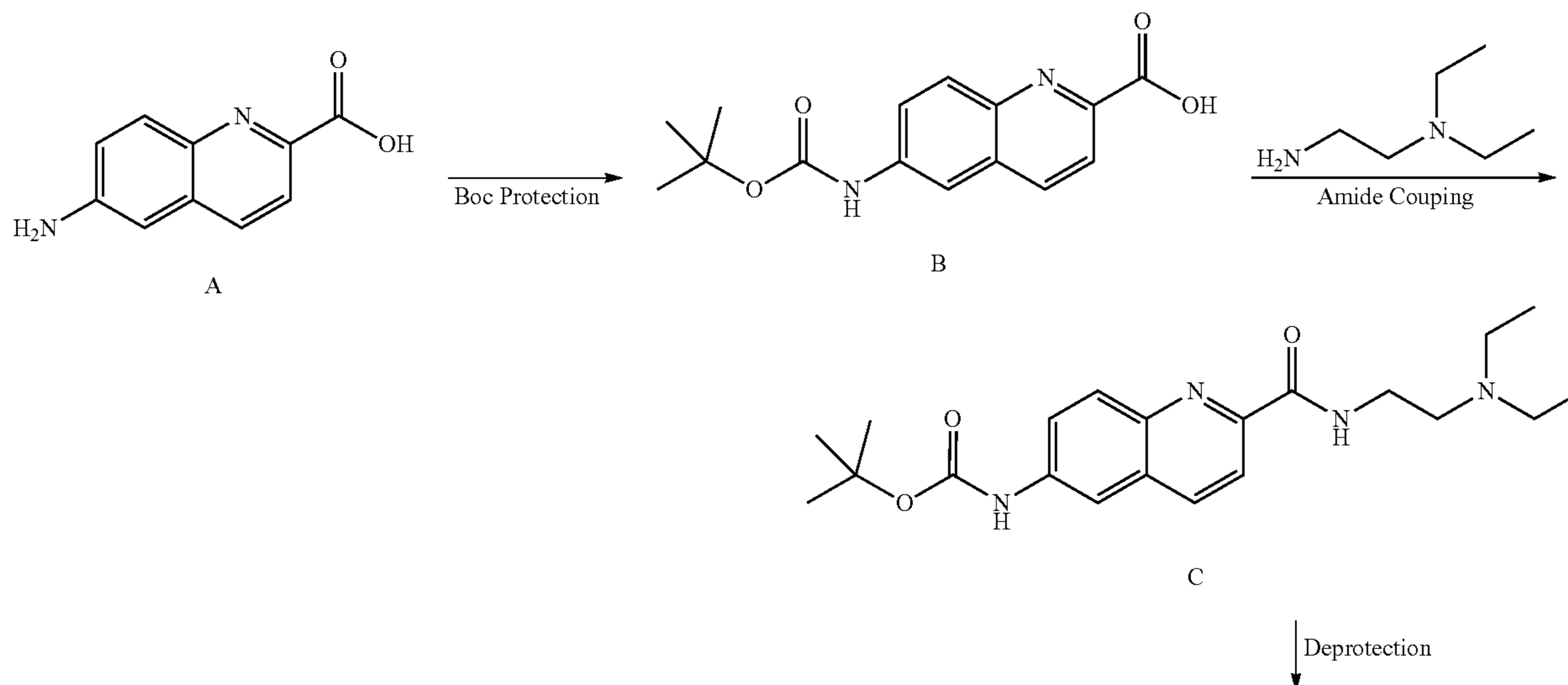
Scheme I
