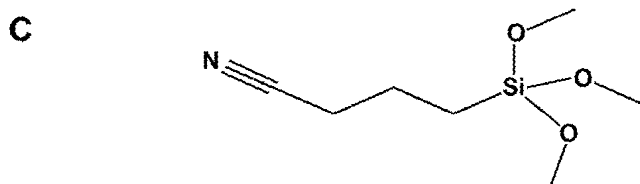
3-Cyanopropyltrimethoxysilane
