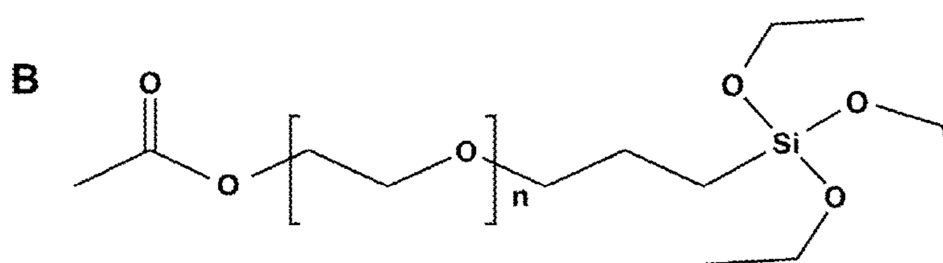
2-[(Acetoxy(polyethyleneoxy)propyl)]triethoxysilane
