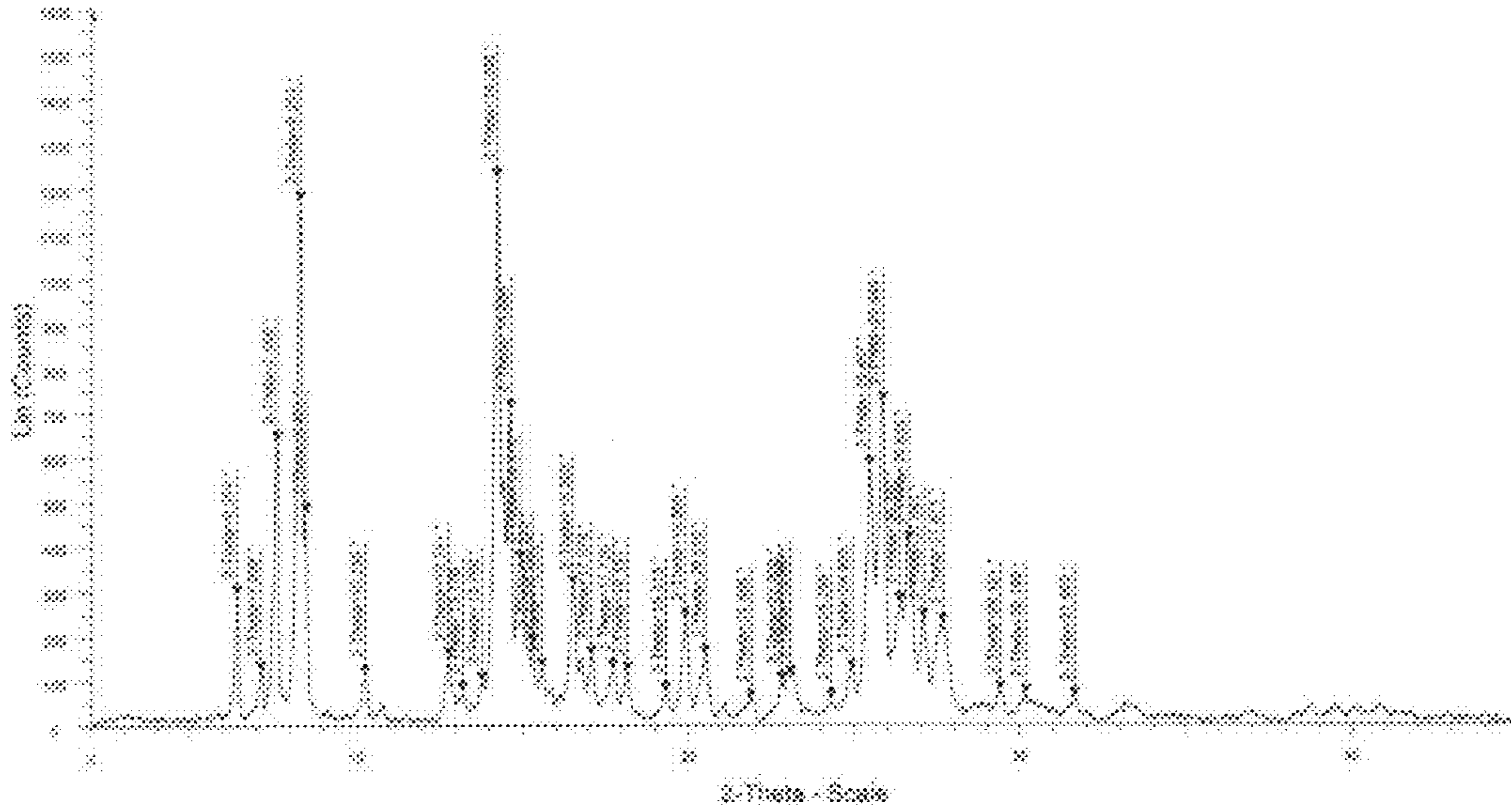
Figure-5: X-Ray powder diffraction pattern of Tavaborole Form IV
