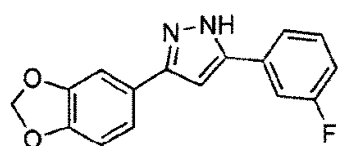
anle186b C_{16}H_{11}FN_2O_2 Mol. Wt.: 282,27
