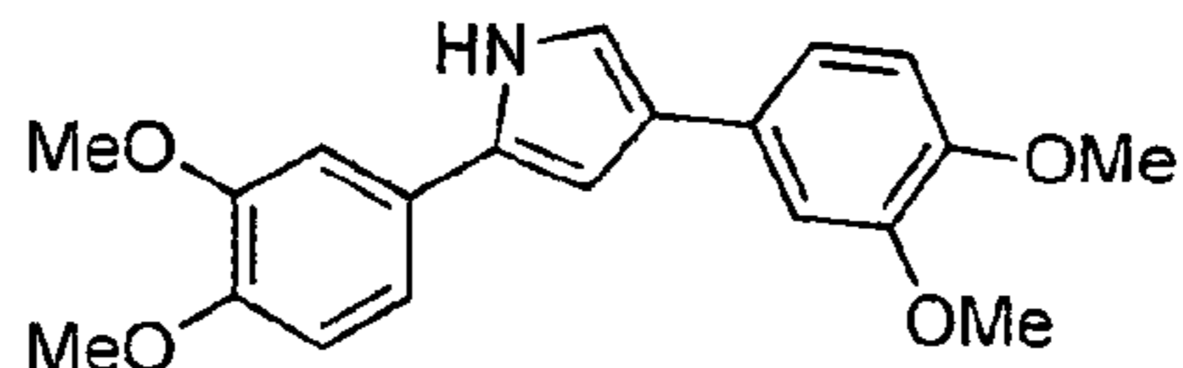
sery167 C_{20}H_{21}NO_4 Mol. Wt.: 339,39
