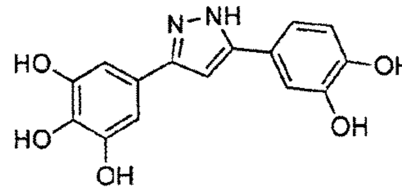
anle143c C_{15}H_{12}N_2O_5 Mol. Wt.: 300,27
