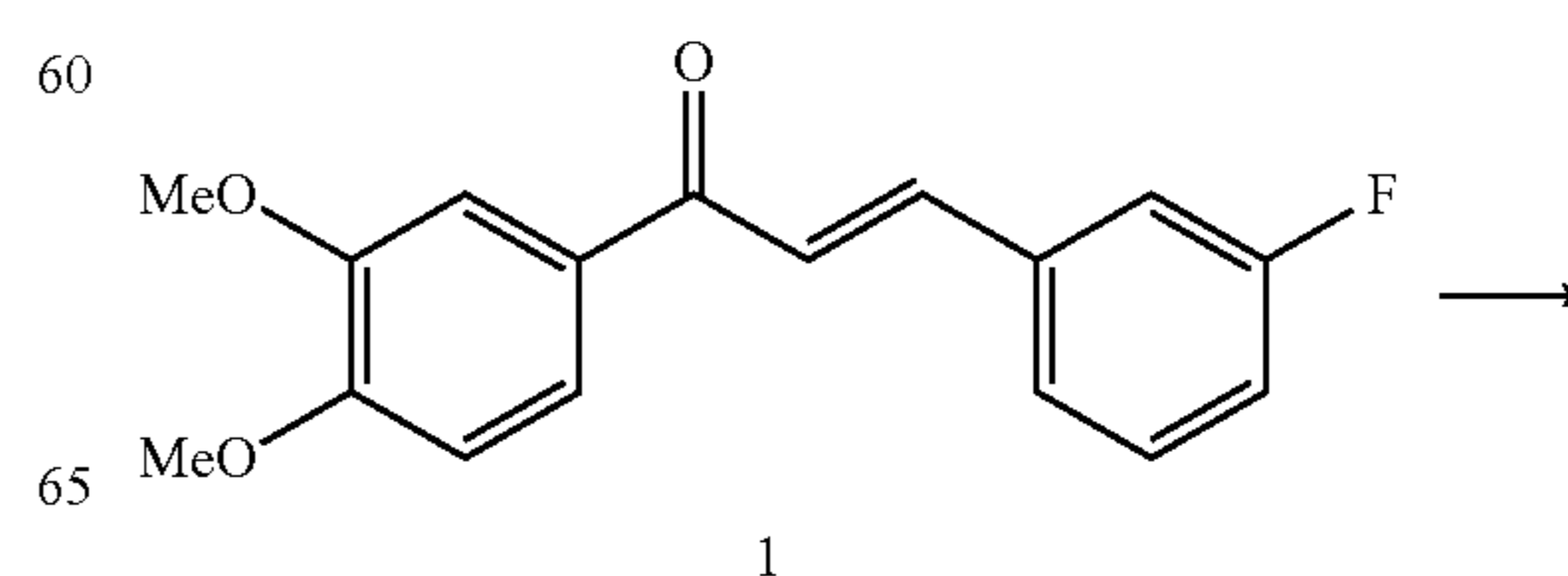
Scheme 5: Synthesis of pyrazolines
