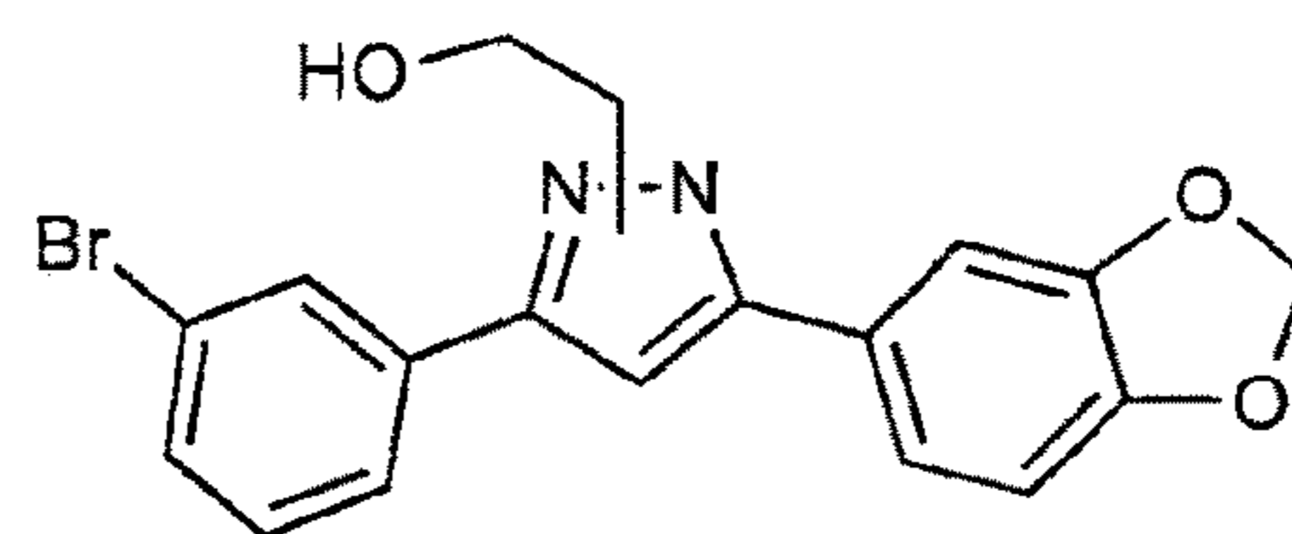
sery329 C_{18}H_{15}BrN_2O_3 Mol. Wt.: 387,23
