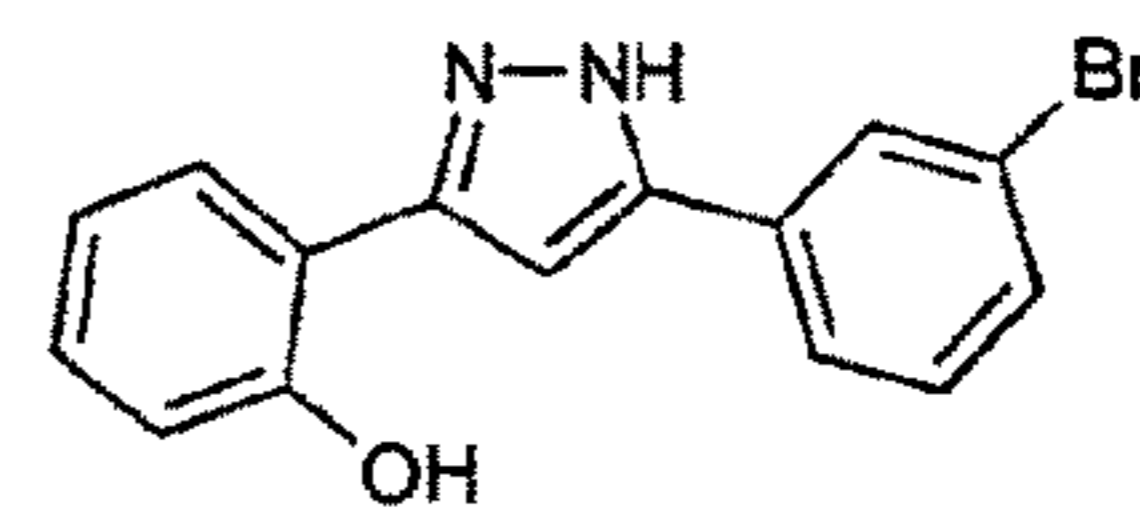
sery260a C_{15}H_{11}BrN_2O Mol. Wt.: 315,16
