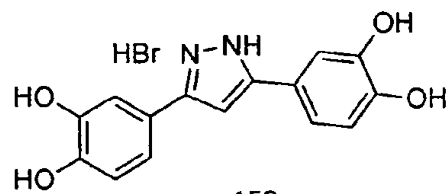
sery159a C_{15}H_{13}BrN_2O_4 Mol. Wt.: 365,18
