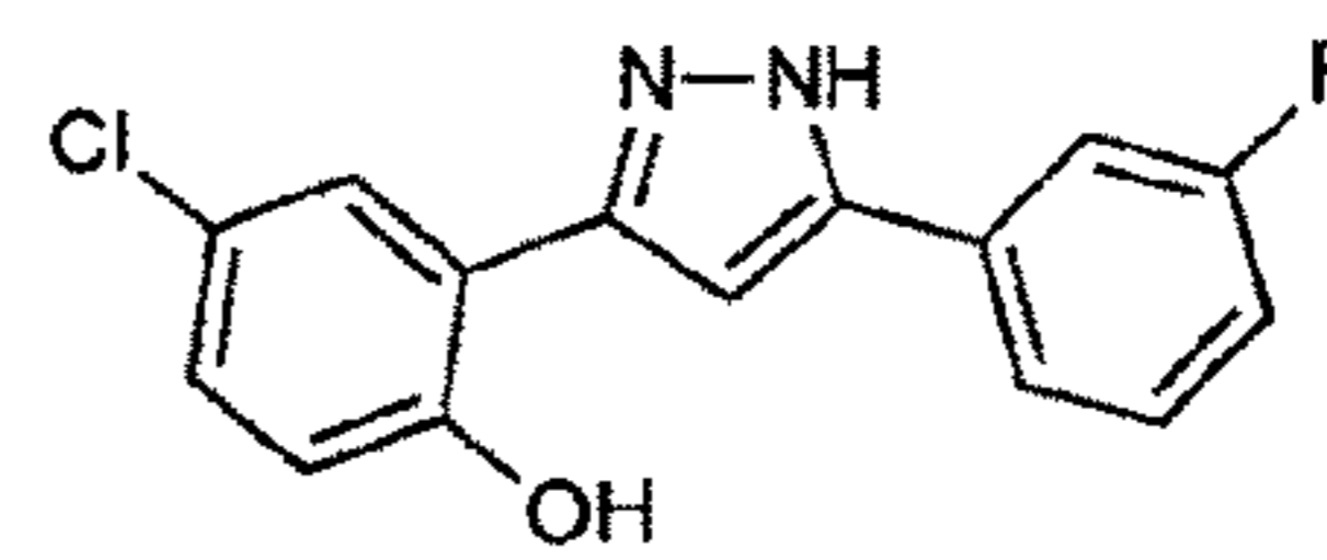
sery263b C_{15}H_{10}ClFN_2O Mol. Wt.: 288,7
