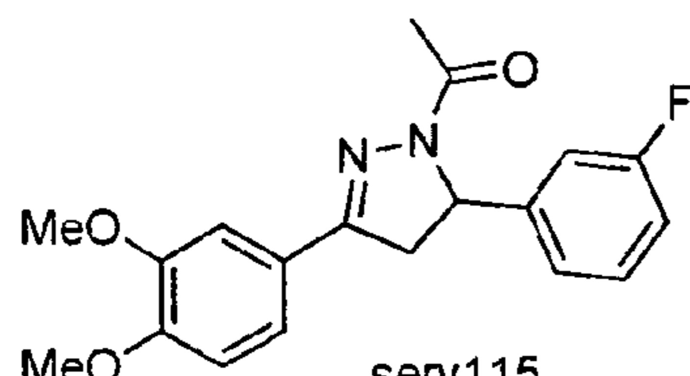
sery115 C_{19}H_{19}FN_2O_3 Mol. Wt.: 342,36
