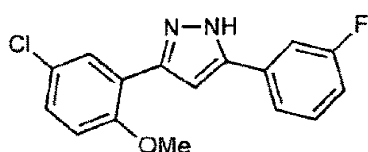
sery261b C_{16}H_{12}ClFN_2O Mol. Wt.: 302,73
