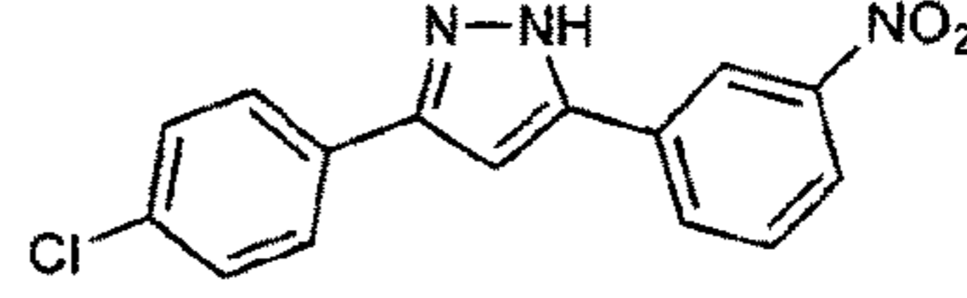
sery278a C_{15}H_{10}ClN_3O_2 Mol. Wt.: 299,71
