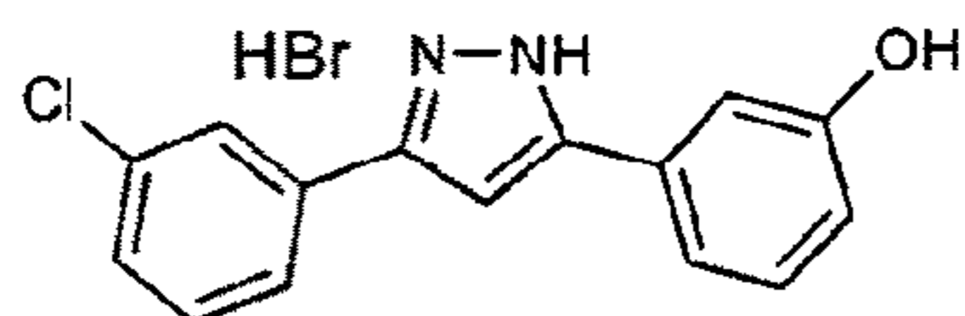
sery320c C_{15}H_{12}BrClN_2O Mol. Wt.: 351,63
