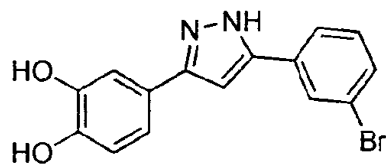
anle136b C_{18}H_{17}FN_2O_3 Mol. Wt.: 328,34
