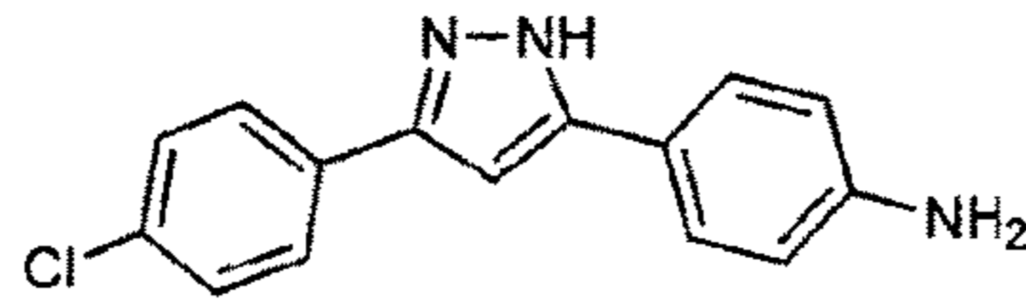
sery280b C_{15}H_{12}ClN_3 Mol. Wt.: 269,73
