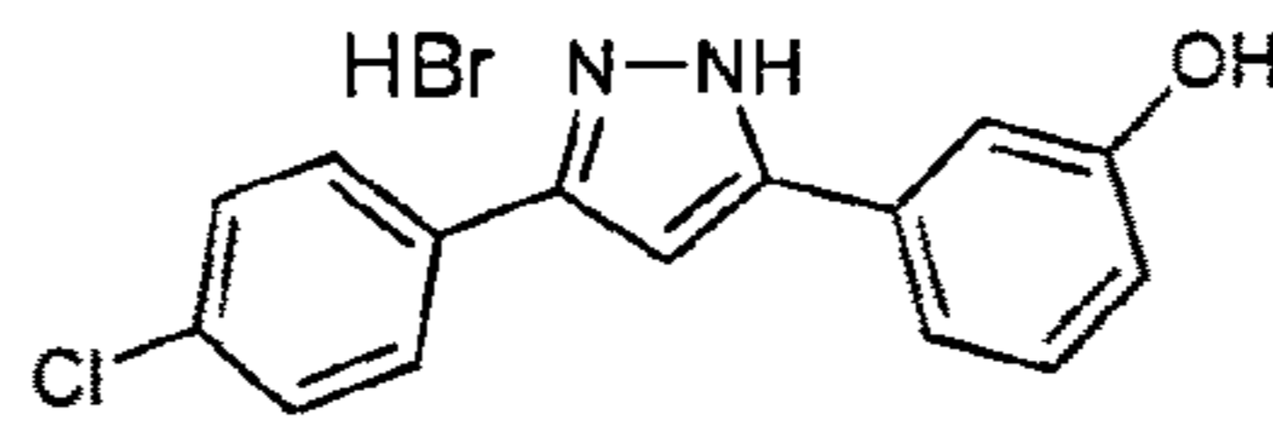
sery320b C_{15}H_{12}BrClN_2O Mol. Wt.: 351,63
