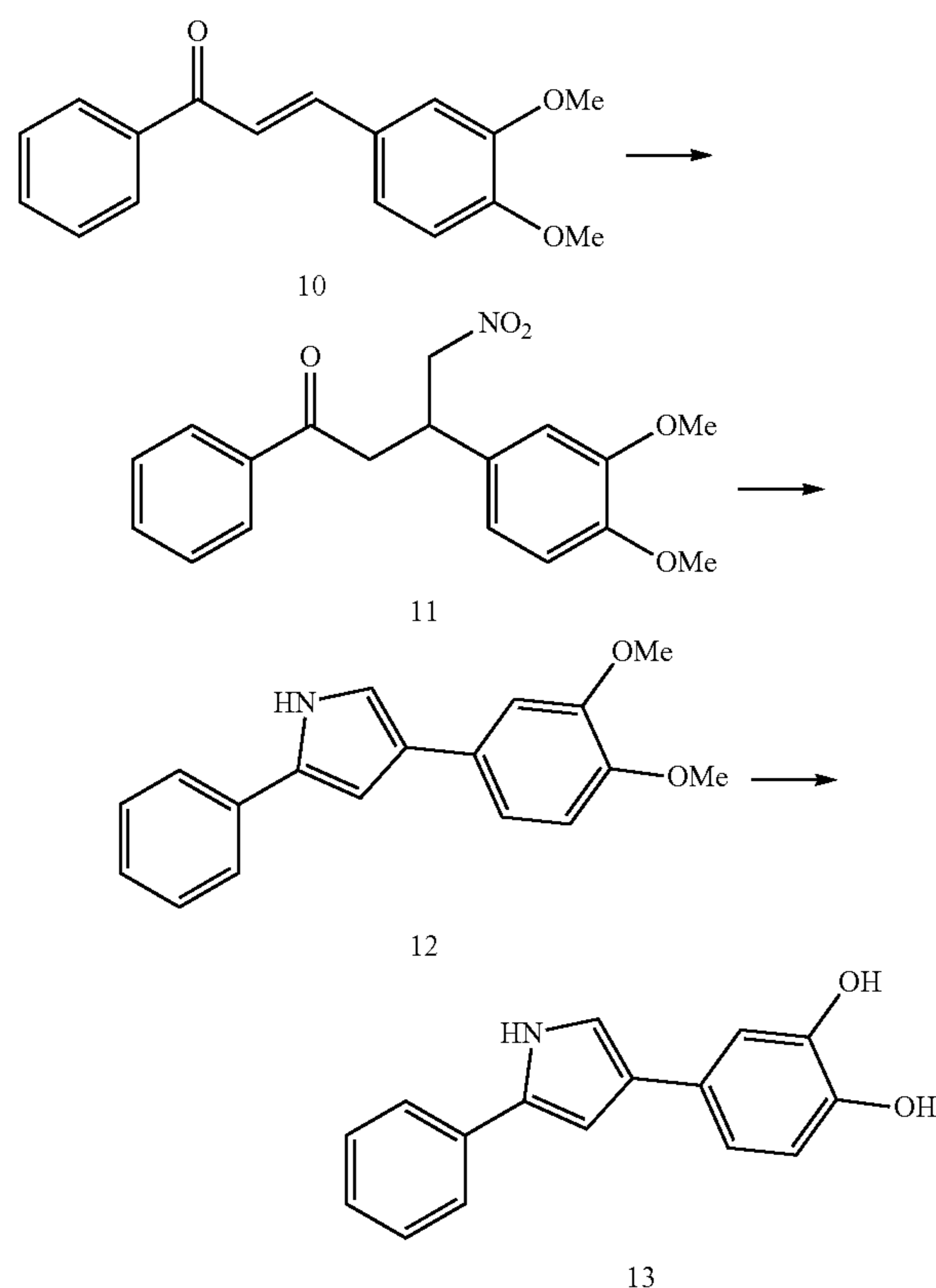
Scheme 4: Synthesis of pyrroles
