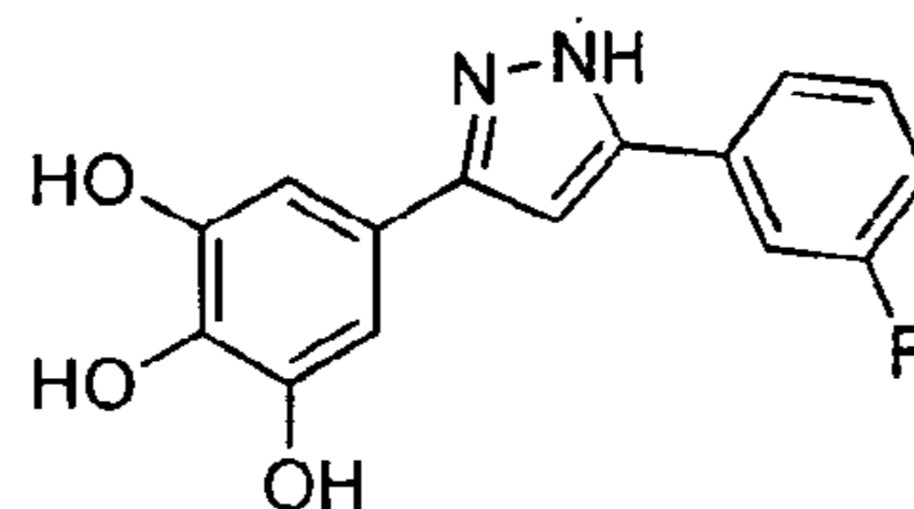
anle136c C_{15}H_{11}FN_2O_3 Mol. Wt.: 286,26
