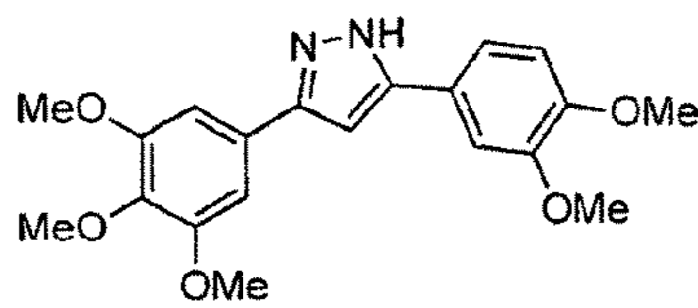
anle143b C_{19}H_{19}BrN_2O_4 Mol. Wt.: 419,27
