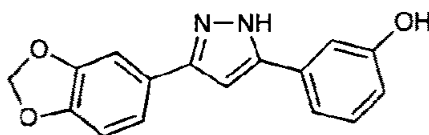
sery313b C_{16}H_{12}N_2O_3 Mol. Wt.: 280,28
