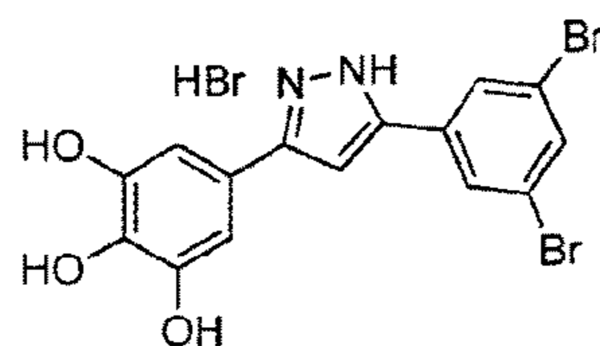
anle145c C_{15}H_{11}Br_3N_2O_3 Mol. Wt.: 506,97
