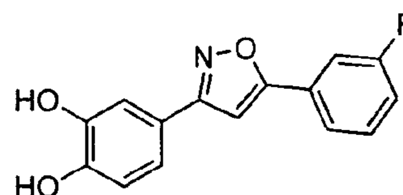
sery117 C_{15}H_{10}FNO_3 Mol. Wt.: 271,24
