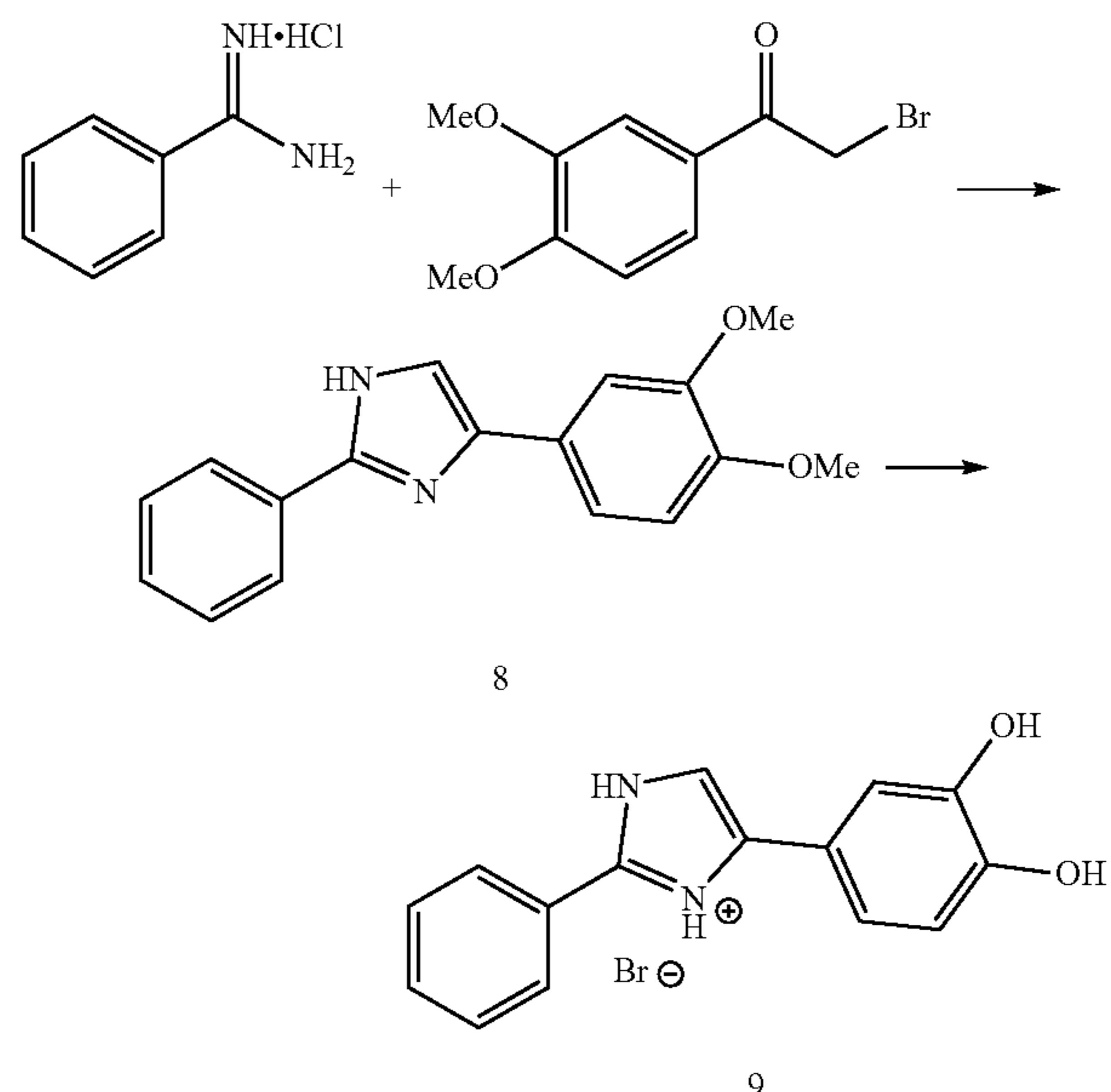
Scheme 3: Synthesis of imidazoles
