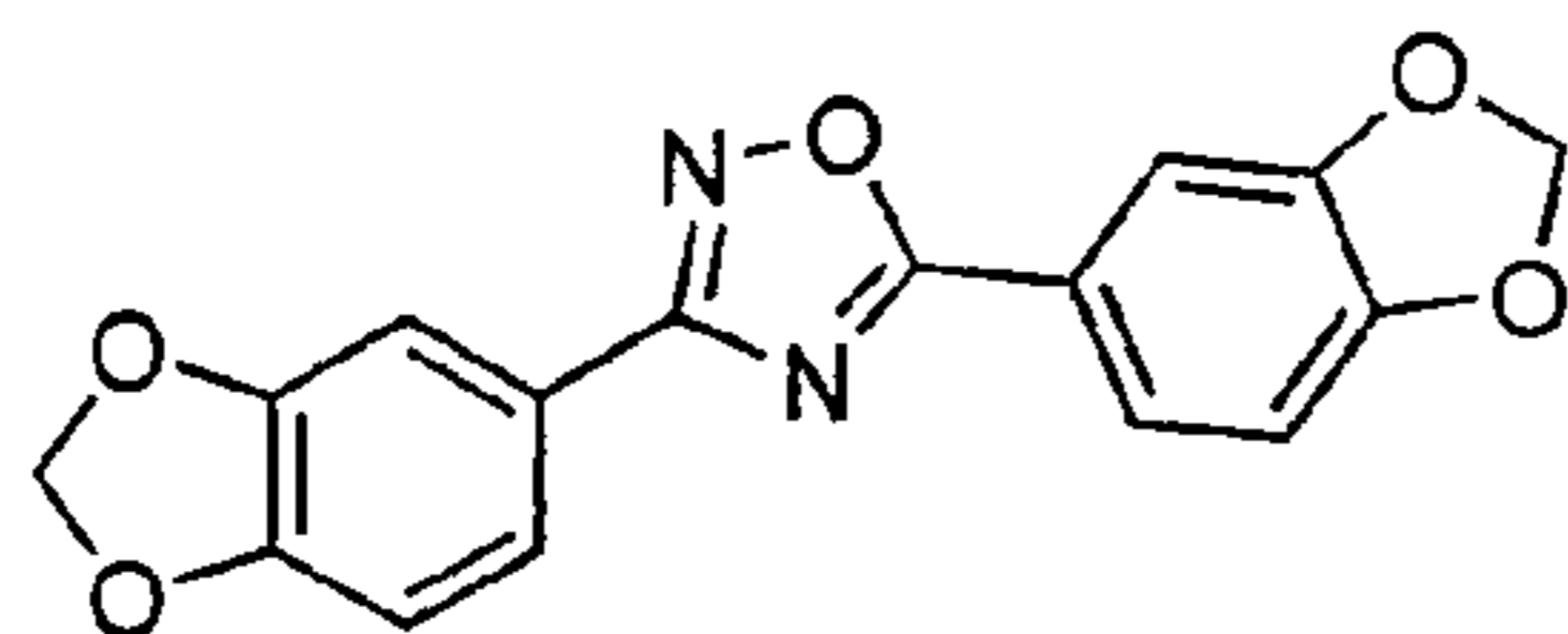
sery129 C_{16}H_{10}N_2O_5 Mol. Wt.: 310,26
