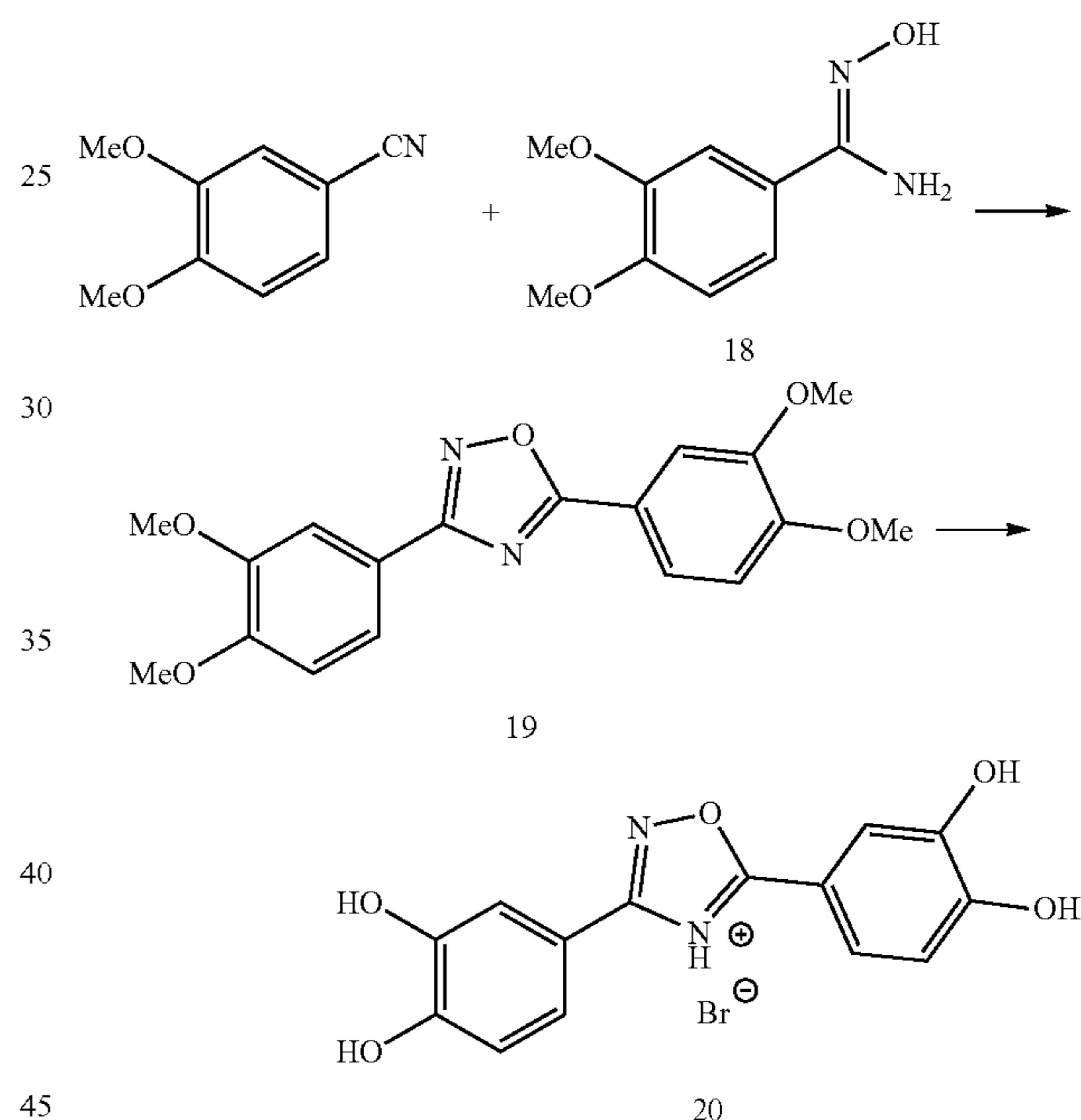
Scheme 7: Synthesis of 1,2,4-oxadiazoles
