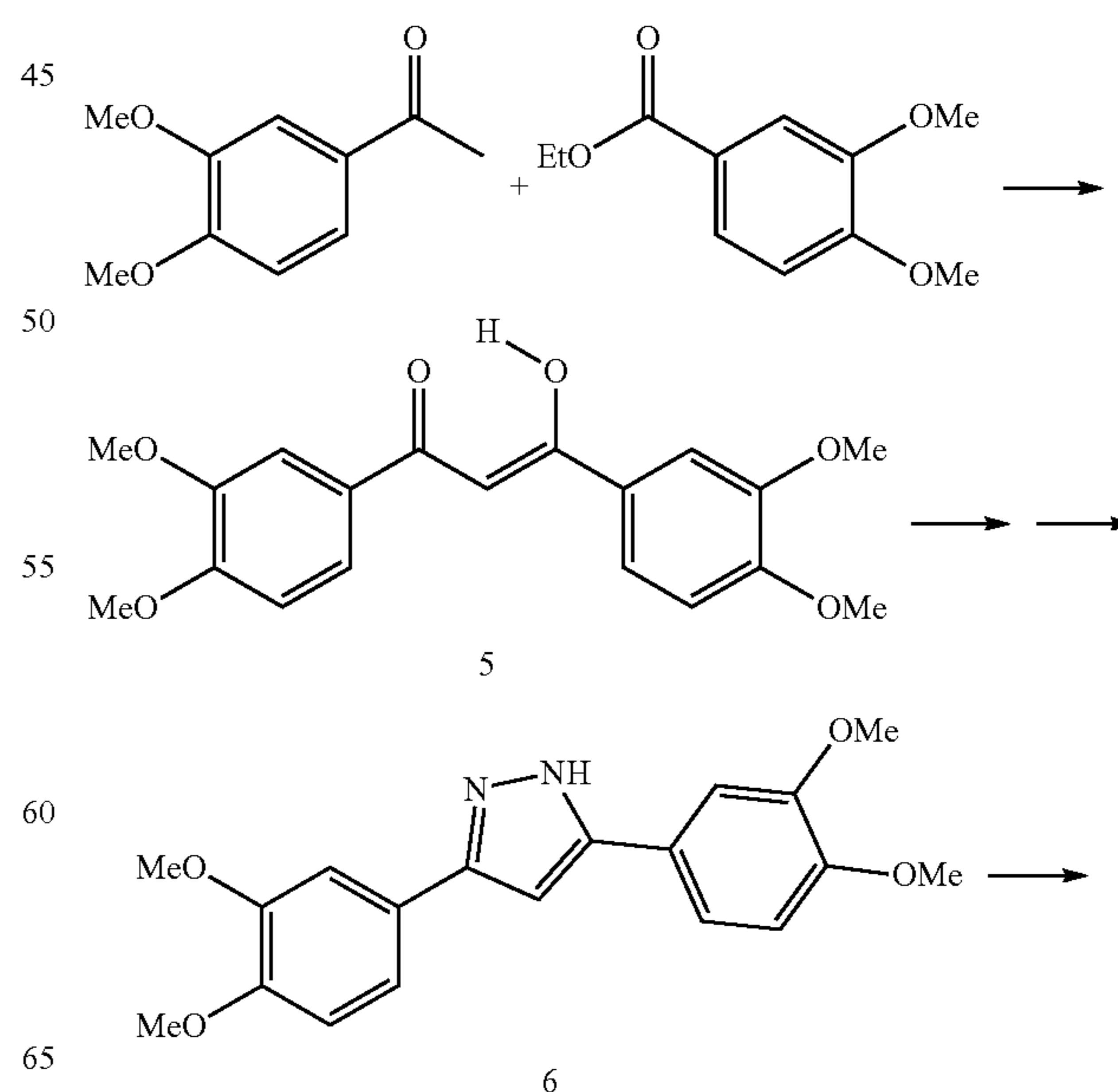
Scheme 2: Synthesis of pyrazoles
