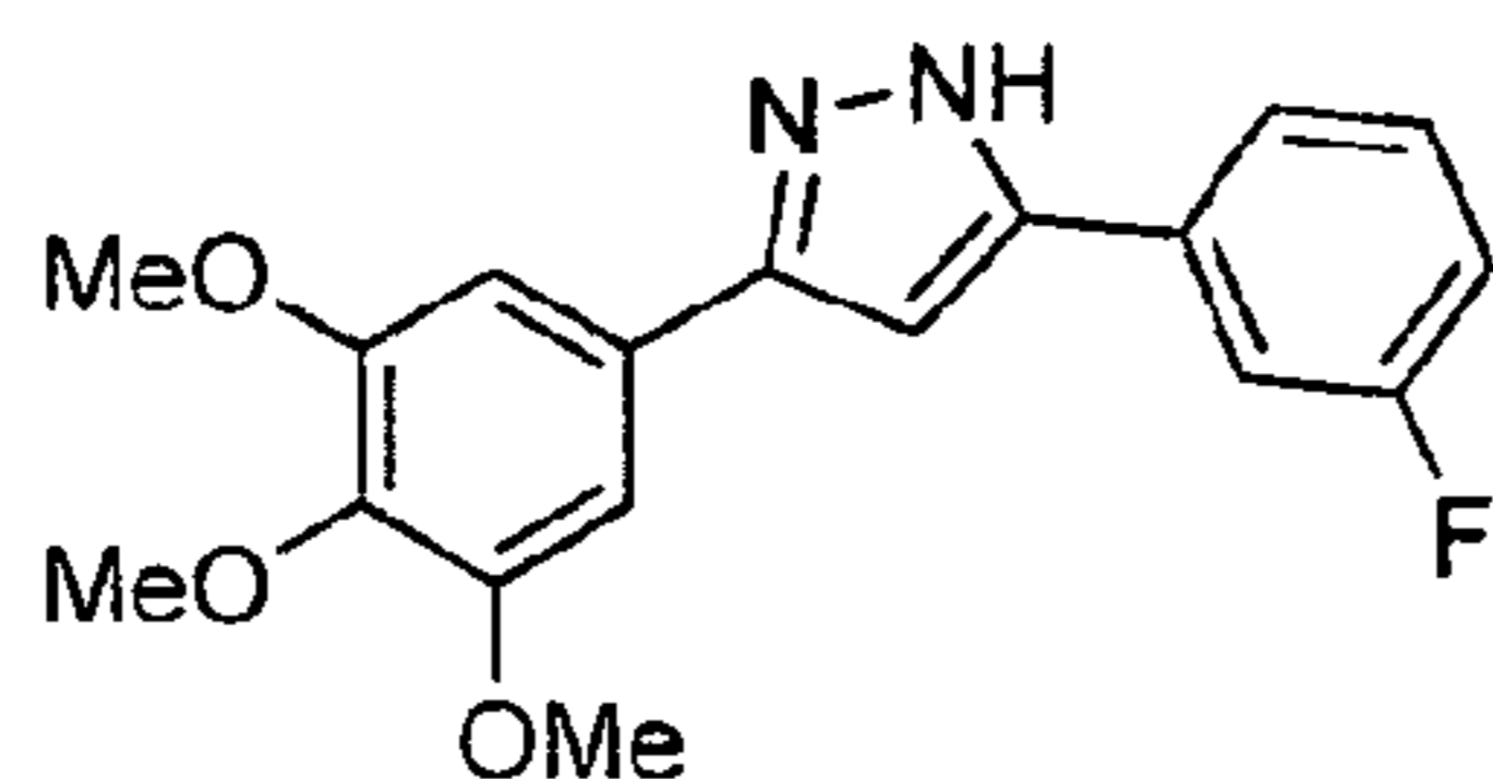
anle136b C_{18}H_{17}FN_2O_3 Mol. Wt.: 328,34
