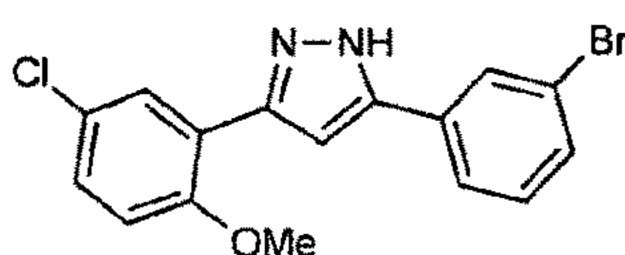
sery257b C_{16}H_{12}BrClN_2O Mol. Wt.: 363,64
