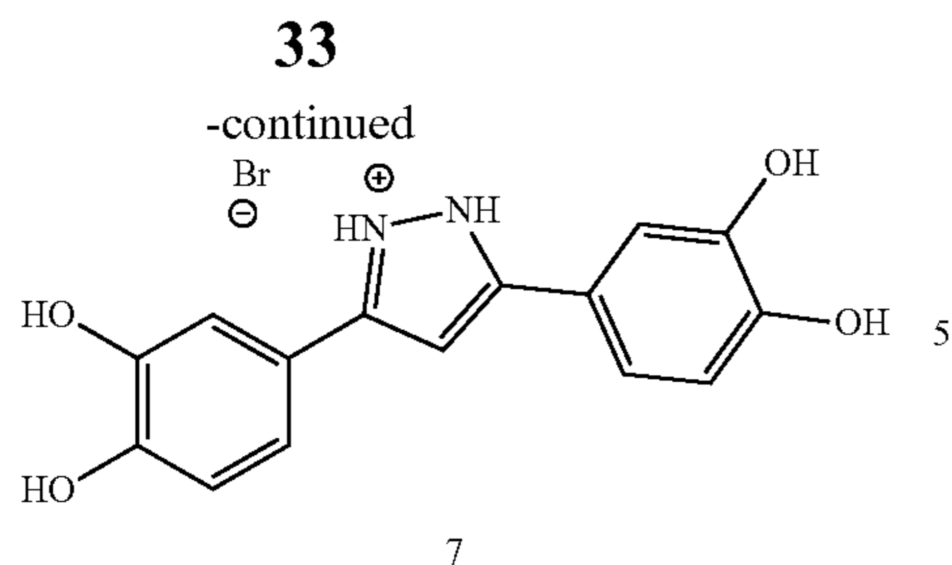
1,3-Bis(3,4-dimethoxyphenyl)-propan-1,3-dione (5) [Anselme, 1967]
