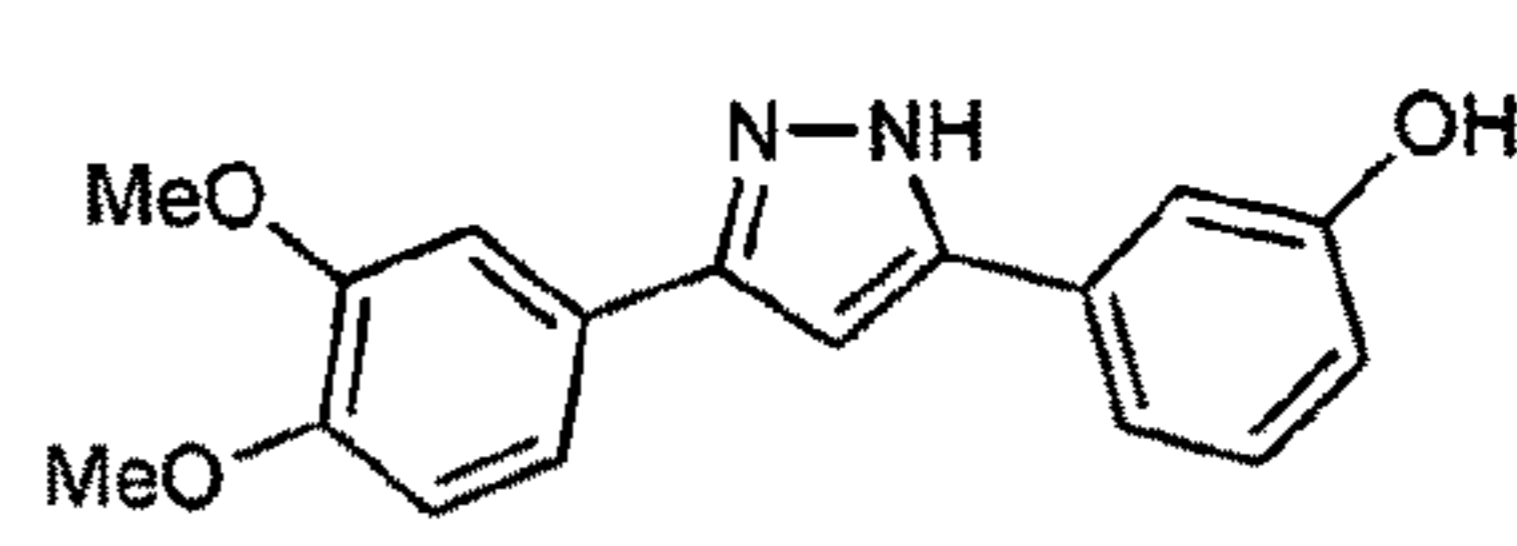
sery310b C_{17}H_{16}N_2O_3 Mol. Wt.: 296,32
