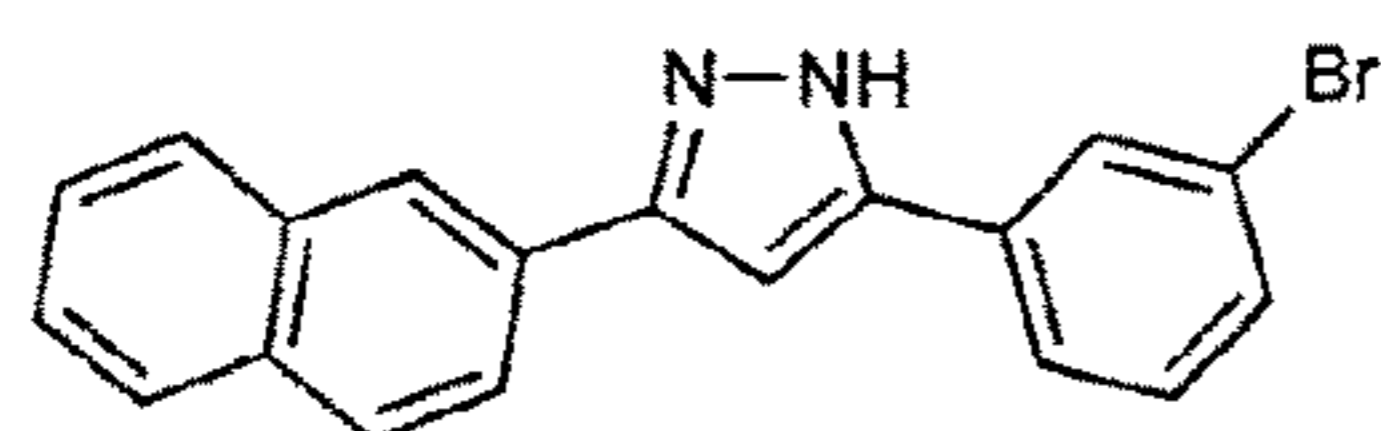
sery292b C_{19}H_{13}BrN_2 Mol. Wt.: 349,22
