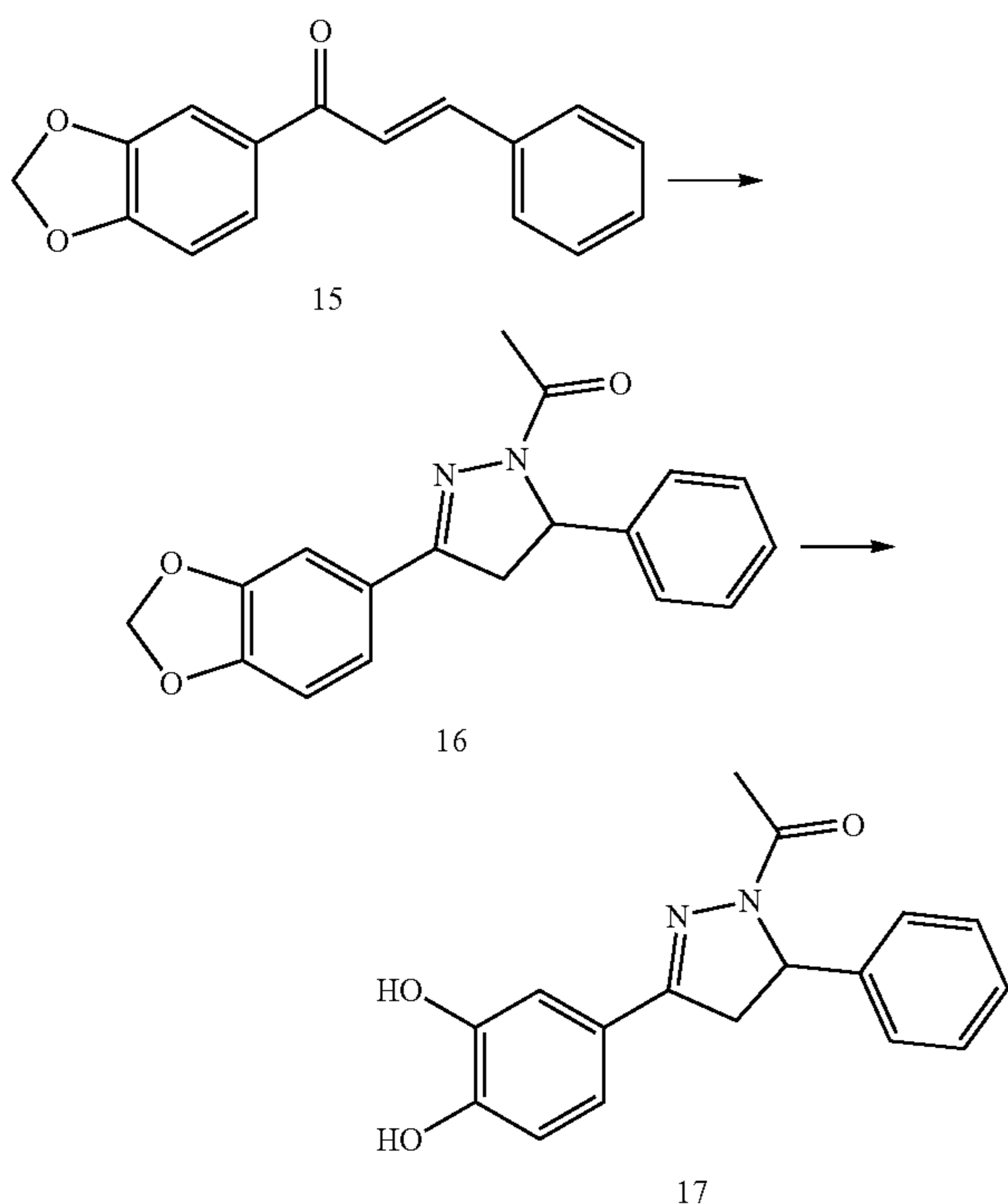
Scheme 6: Synthesis of N-Ac-pyrazolines
