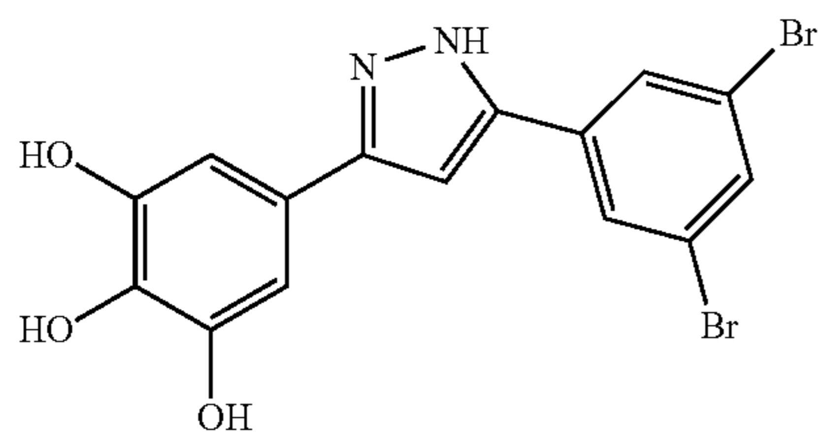
5-(3,5-Dibromophenyl)-3-(3,4,5-trihydroxyphenyl)pyrazole (anle145d)
