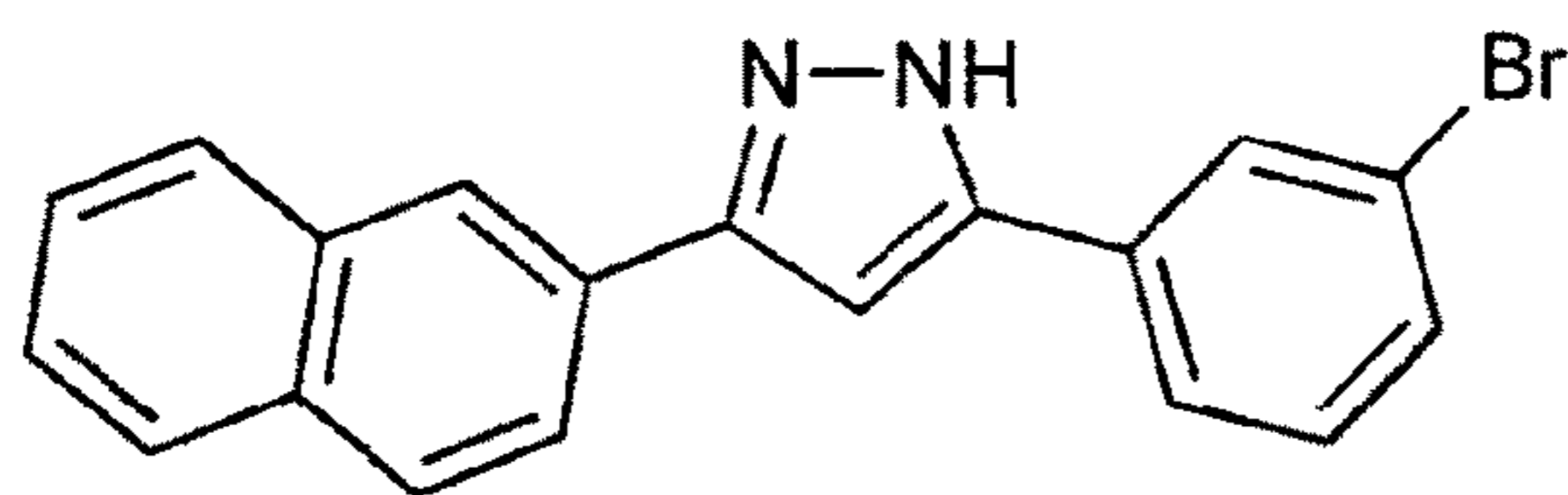
sery292b C_{19}H_{13}BrN_2 Mol. Wt.: 349,22
