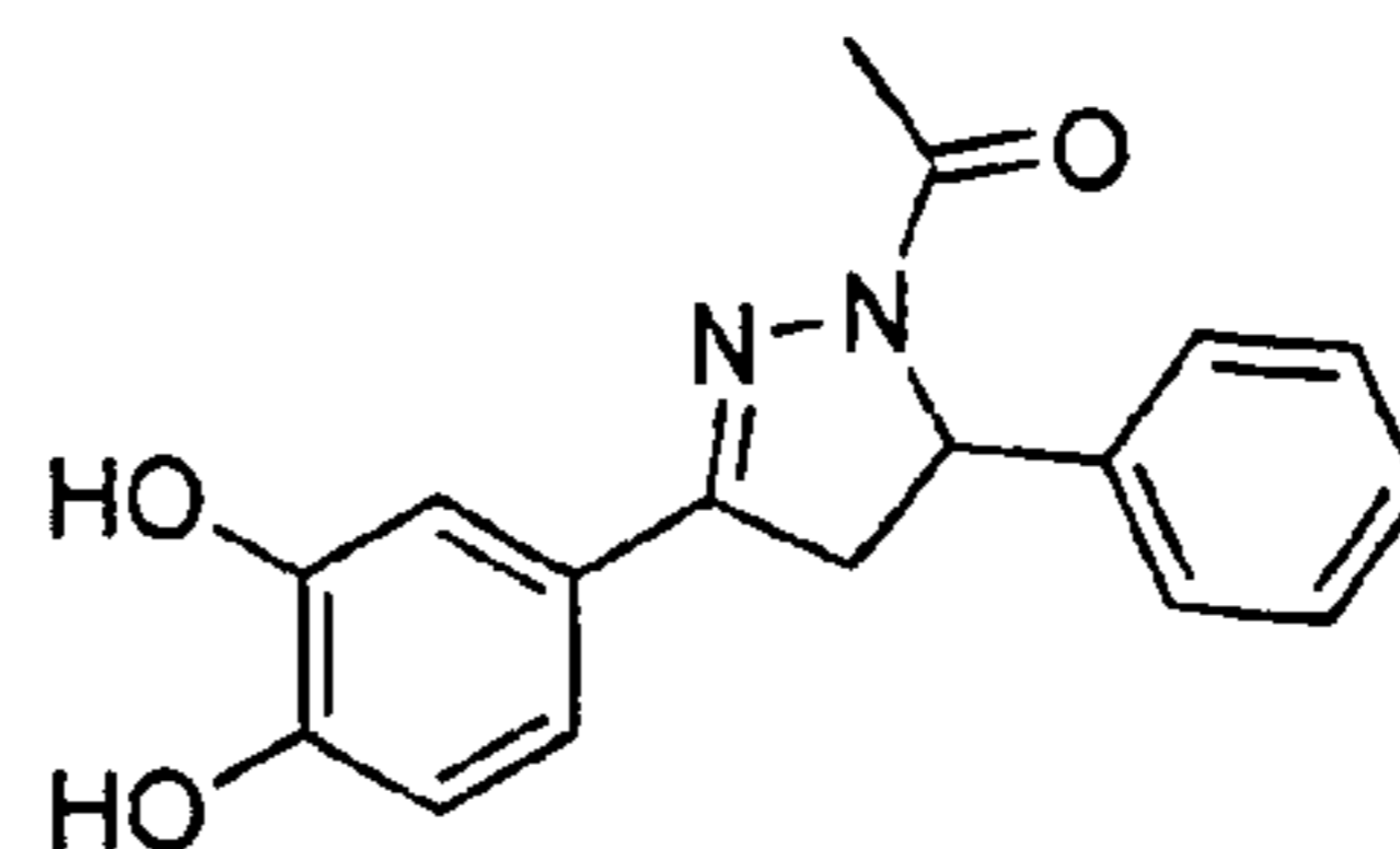
sery105 C_{17}H_{16}N_2O_3 Mol. Wt.: 296,32
