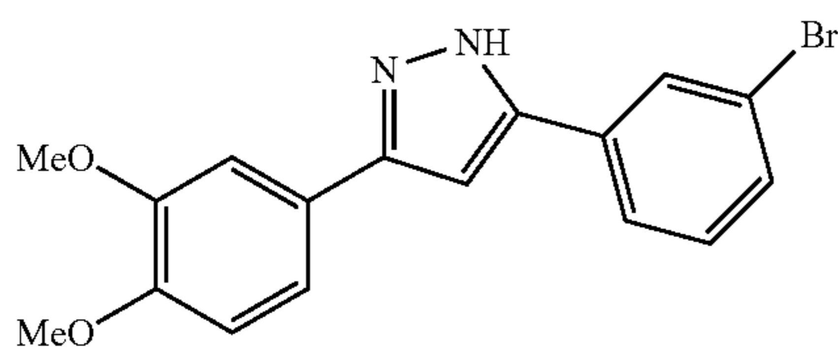
5-(3-Bromophenyl)-3-(3,4-dimethoxyphenyl)pyrazole (sery255b)
