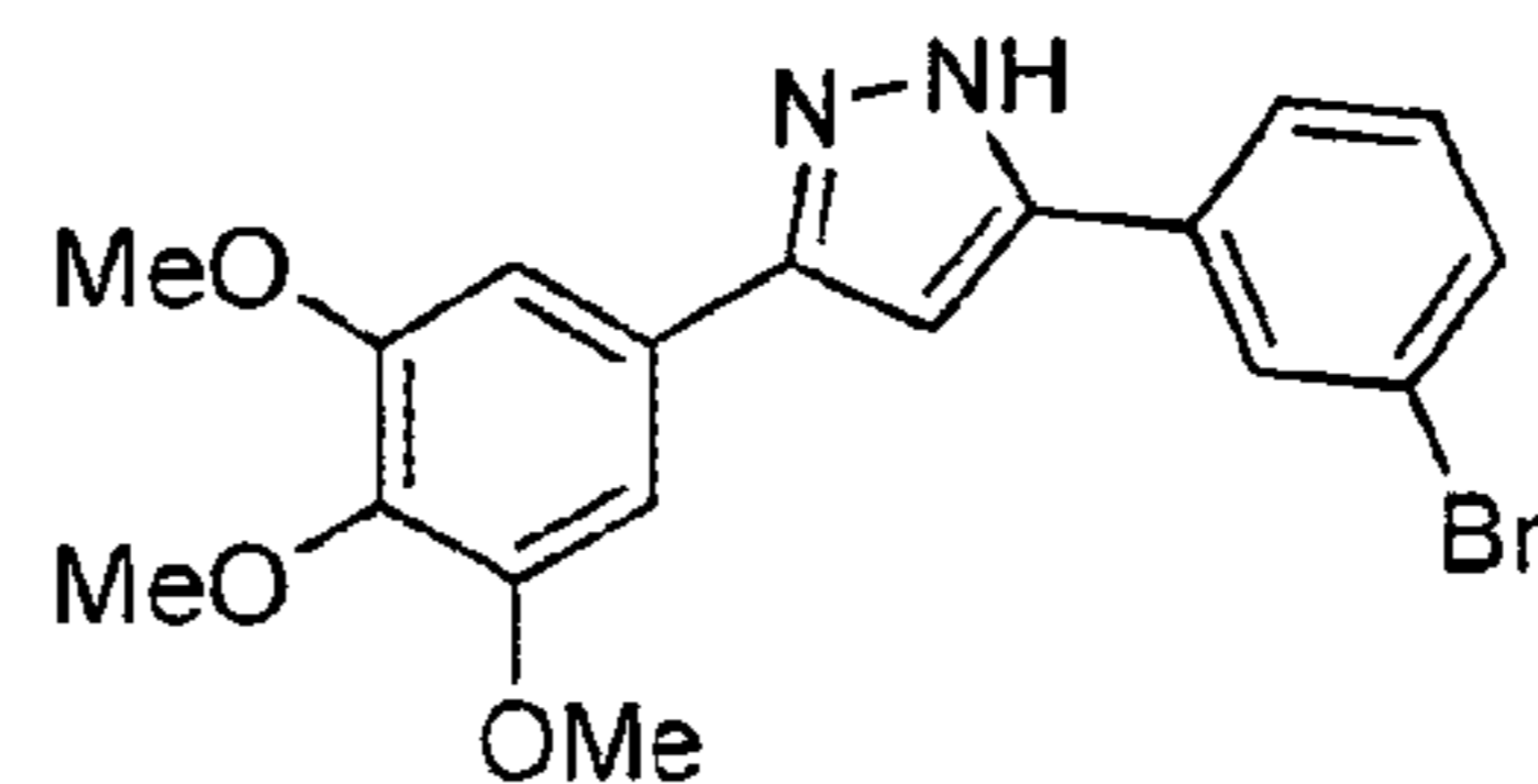
anle142b C_{18}H_{17}BrN_2O_3 Mol. Wt.: 389,24
