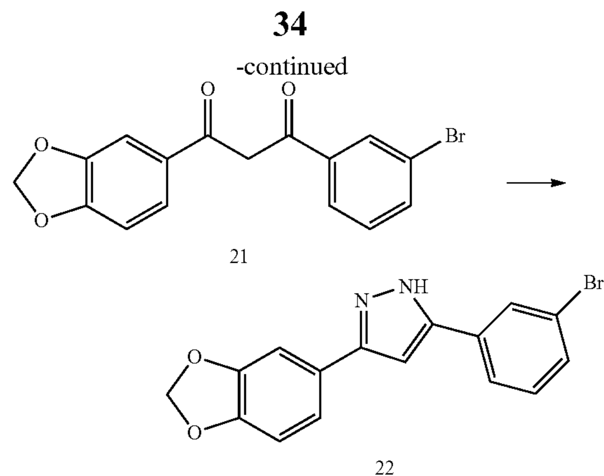
1-(1,3-Benzodioxol-5-yl)-3-(3-bromophenyl)-propan-1,3-dione (21) [Anselme, 1967]
