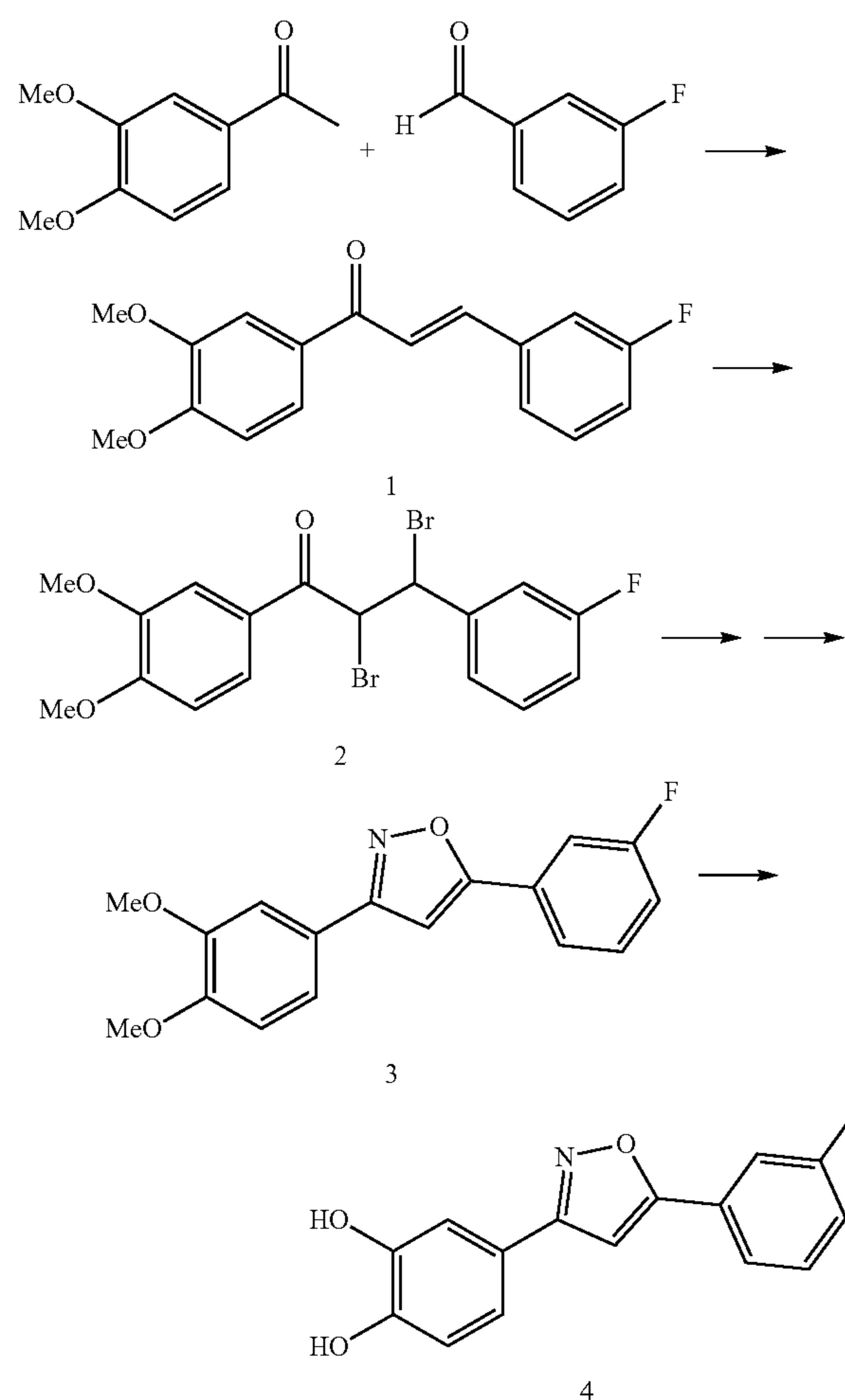
Scheme 1: Synthesis of isoxazoles
