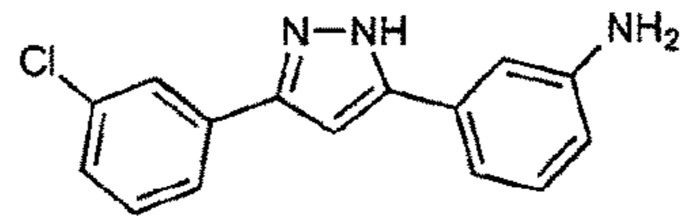
sery275b C_{15}H_{12}ClN_3 Mol. Wt.: 269,73
