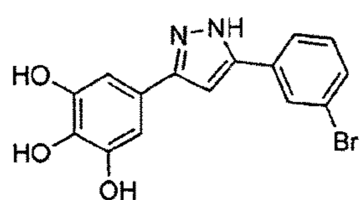
anle142c C_{15}H_{11}BrN_2O_3 Mol. Wt.: 347,16
