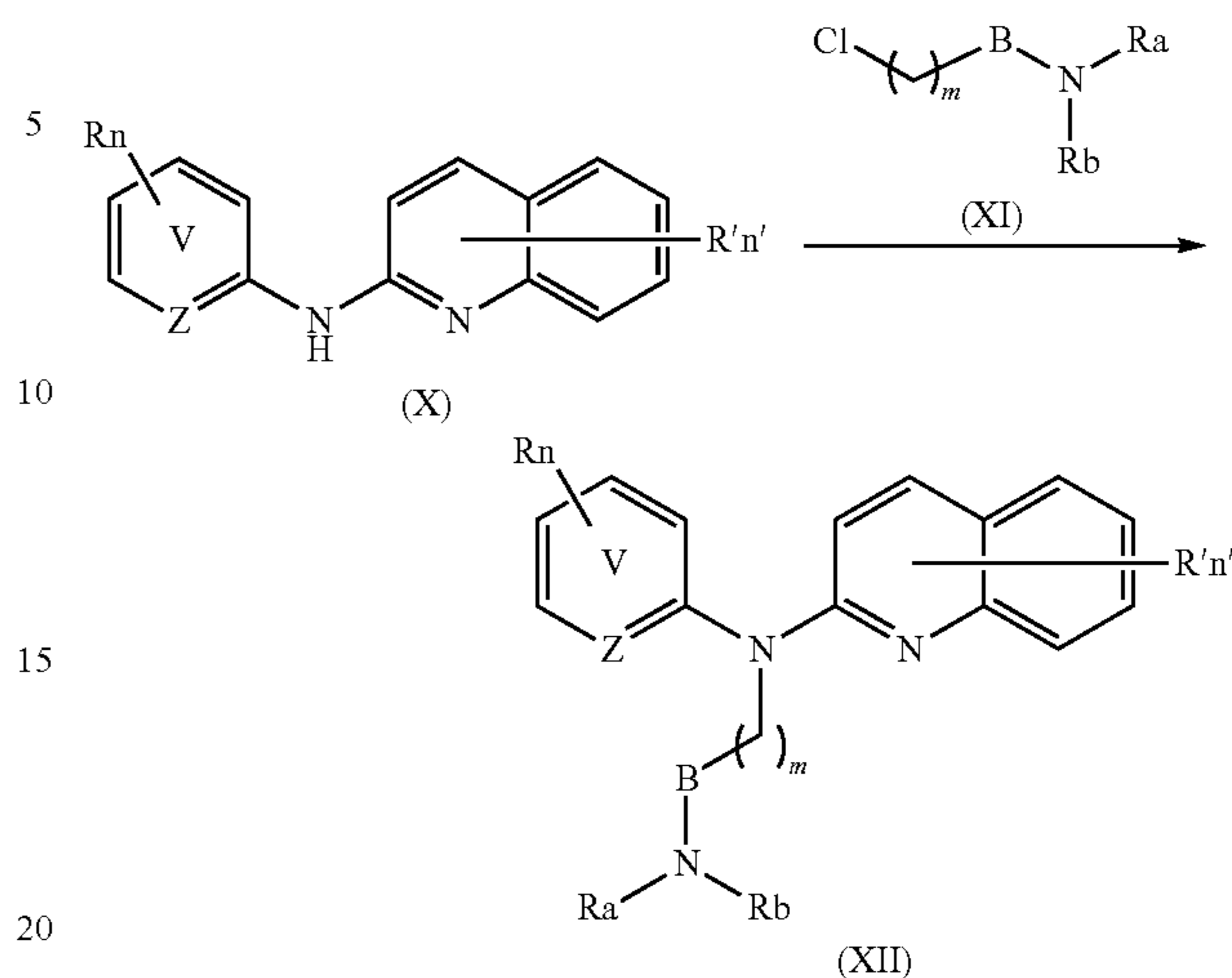
Scheme 3
