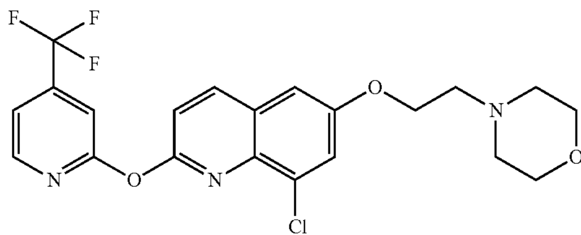
Formula (Ie)
