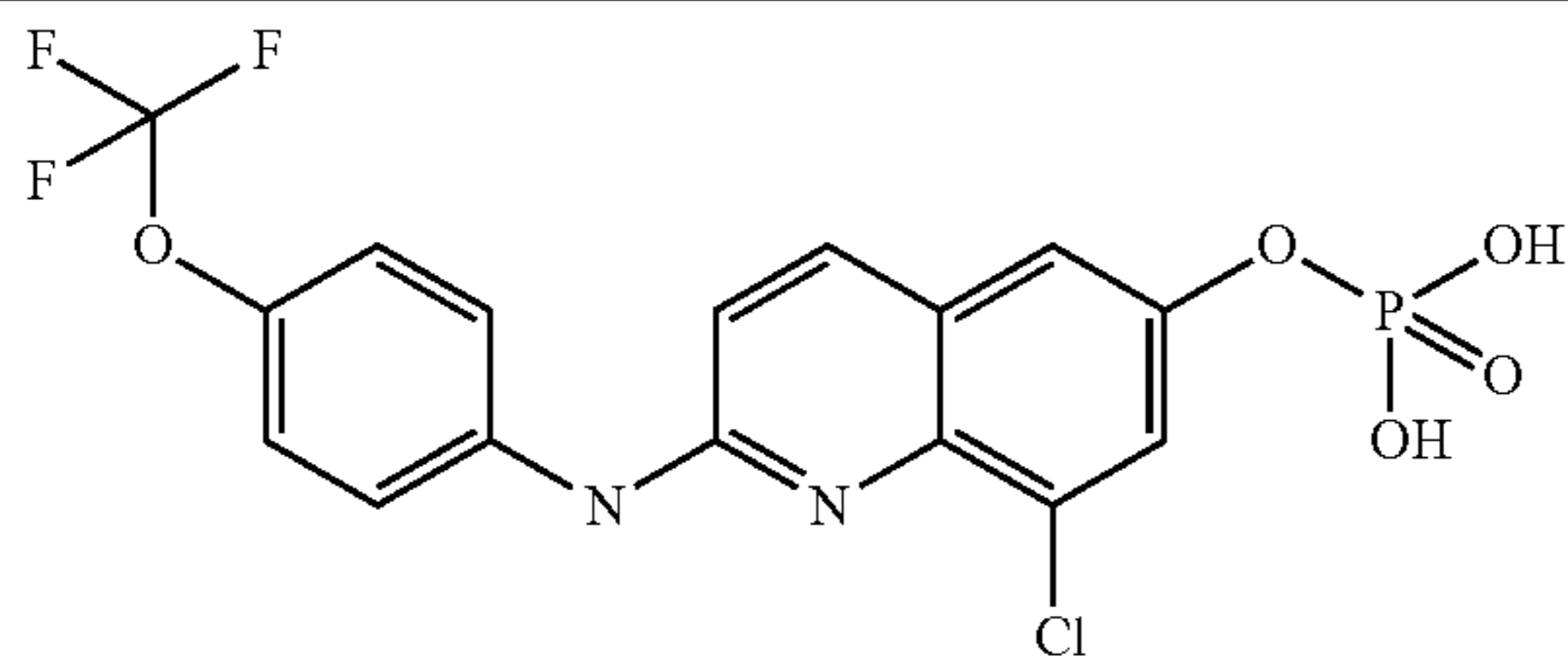
Formula (Ic)
