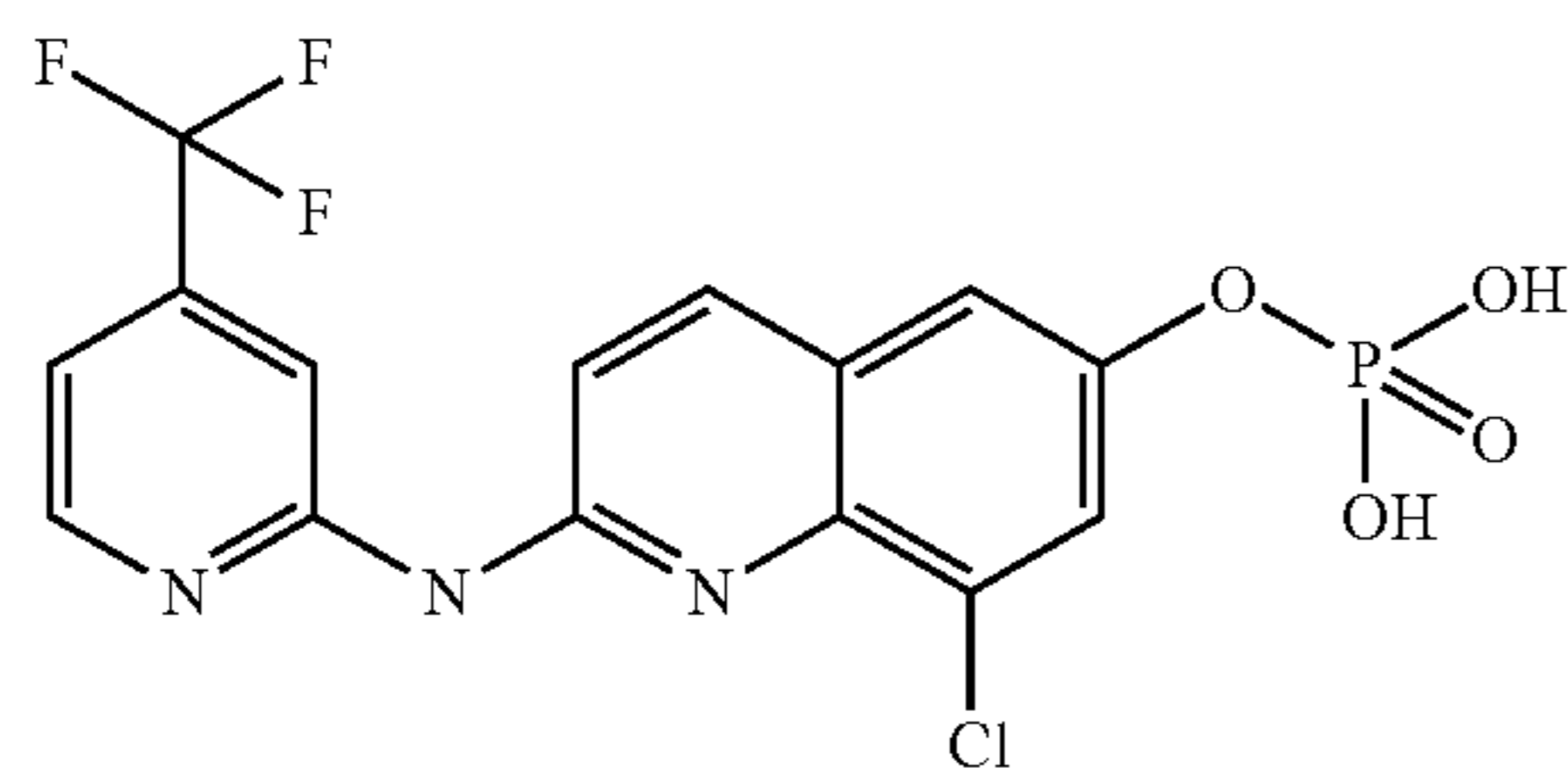
Formula (Ib)
