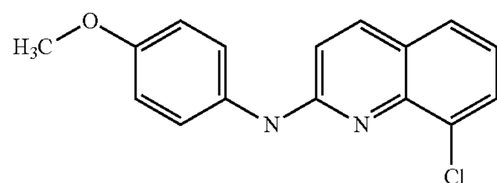
Formula (Ib)
