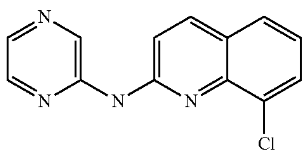
Formula (Id)
