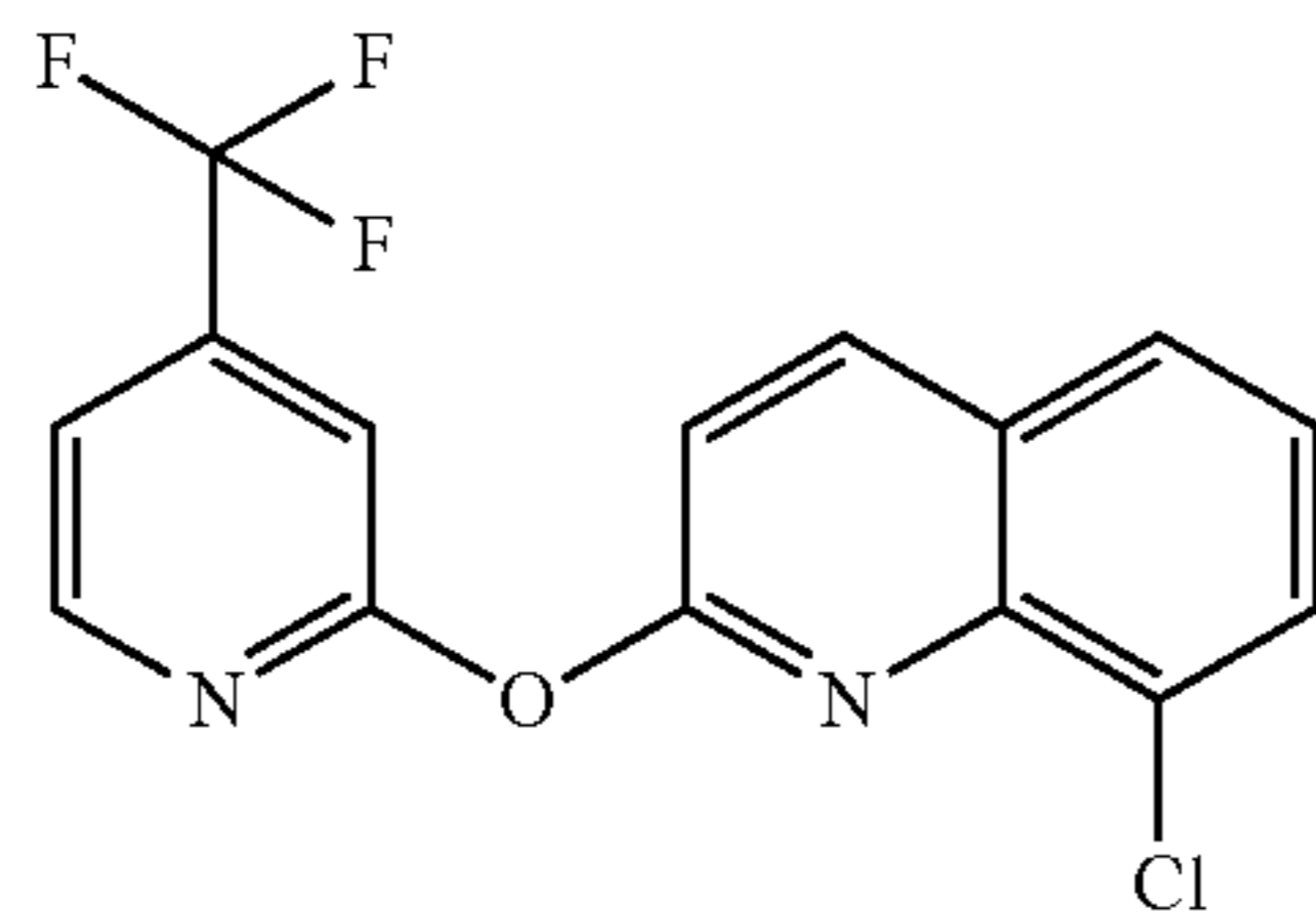
Formula (Id)
