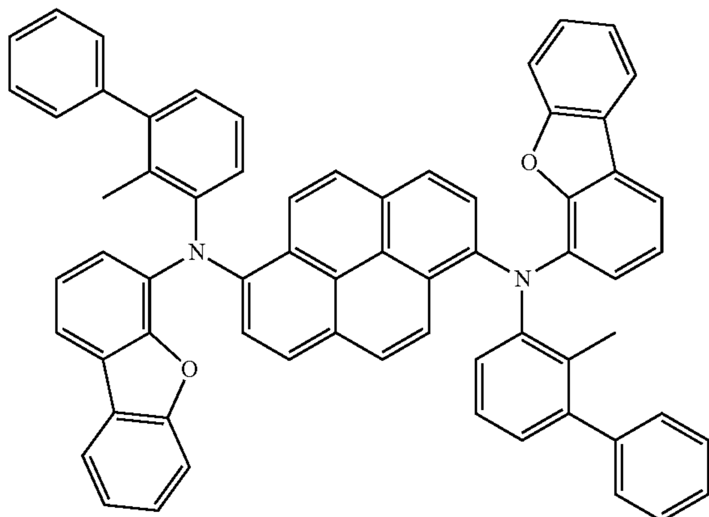
Comparative Compound 2
