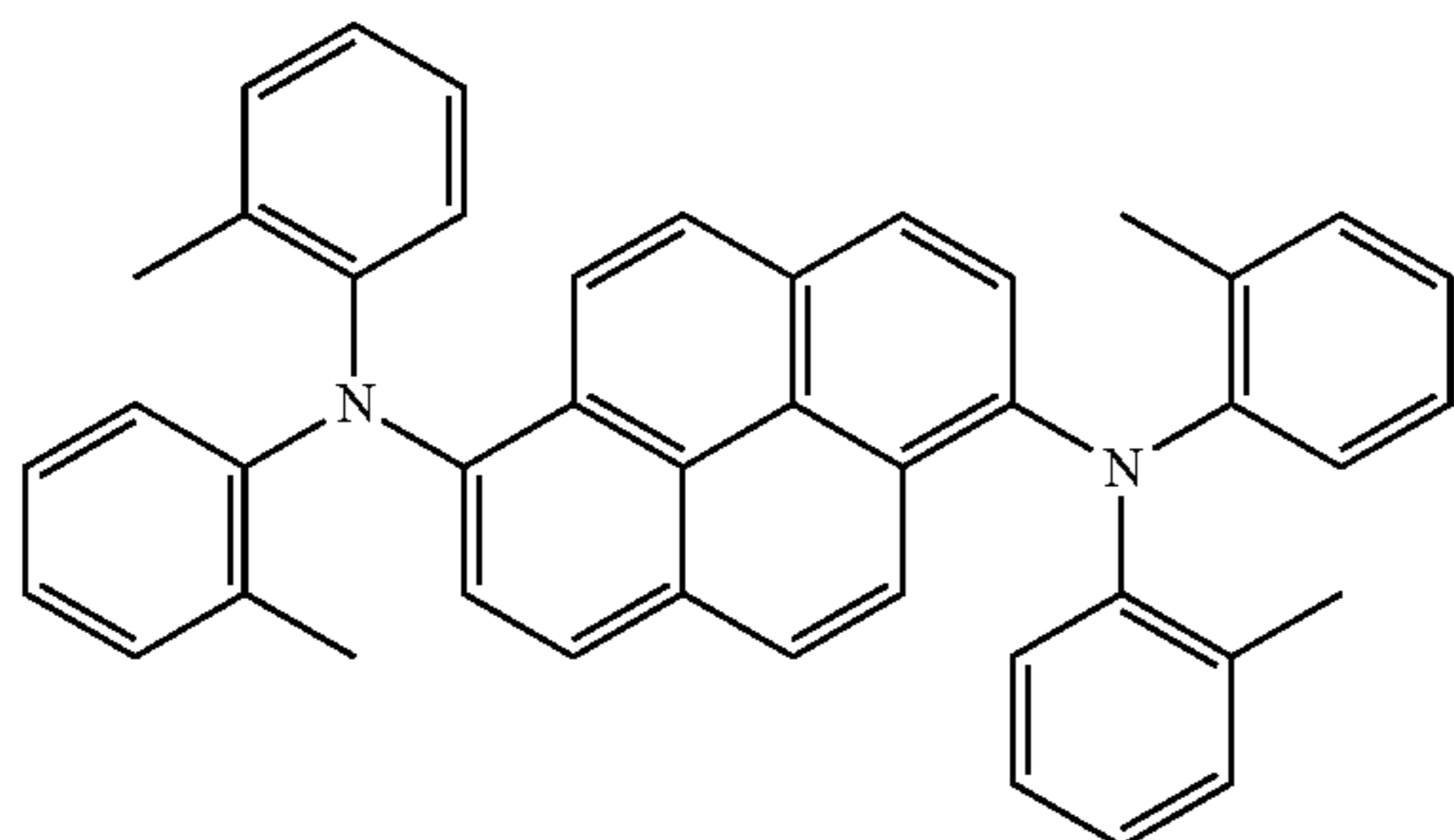
Comparative Compound 3
