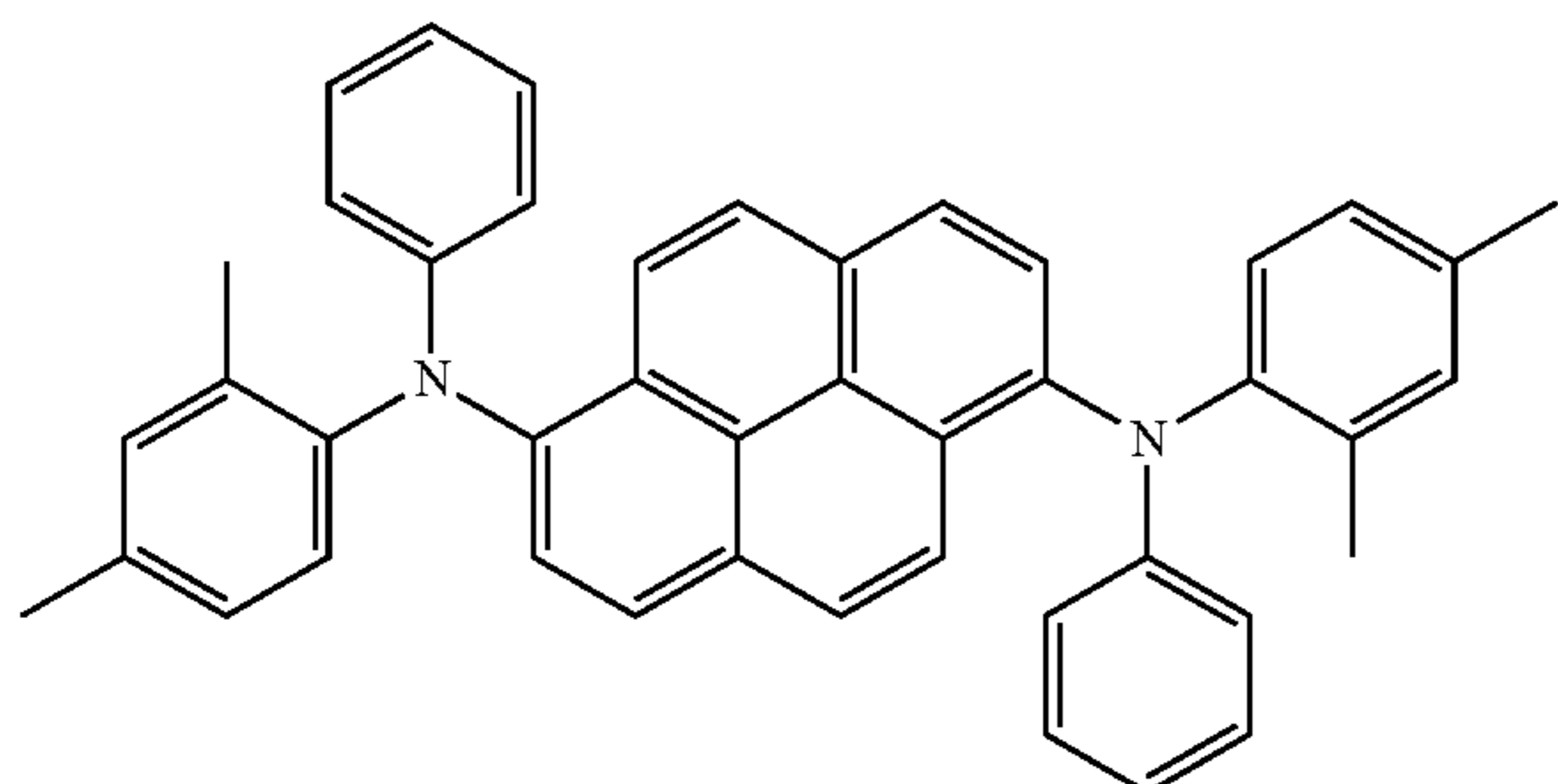
Comparative Compound 5
