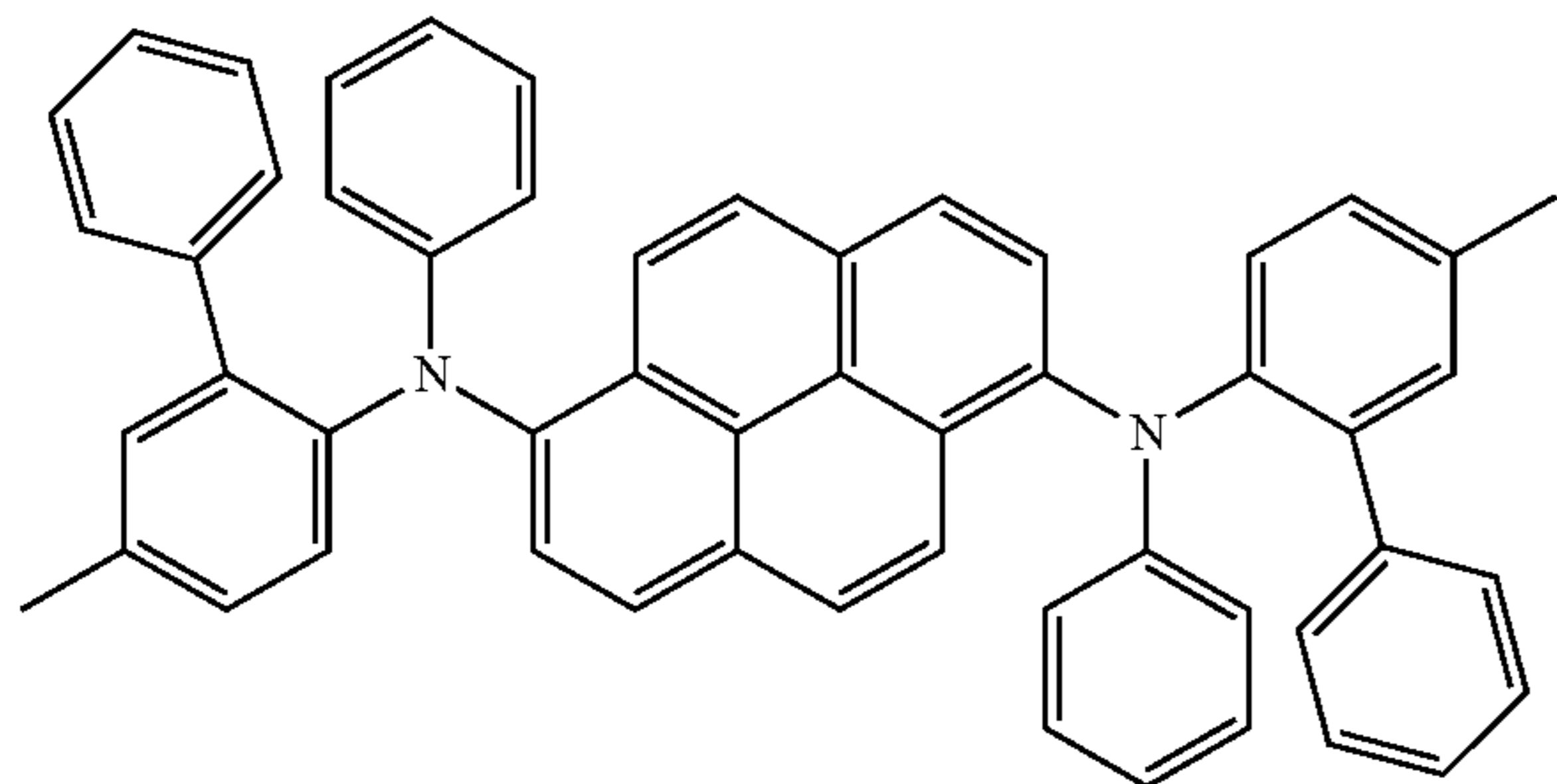
Comparative Compound 4
