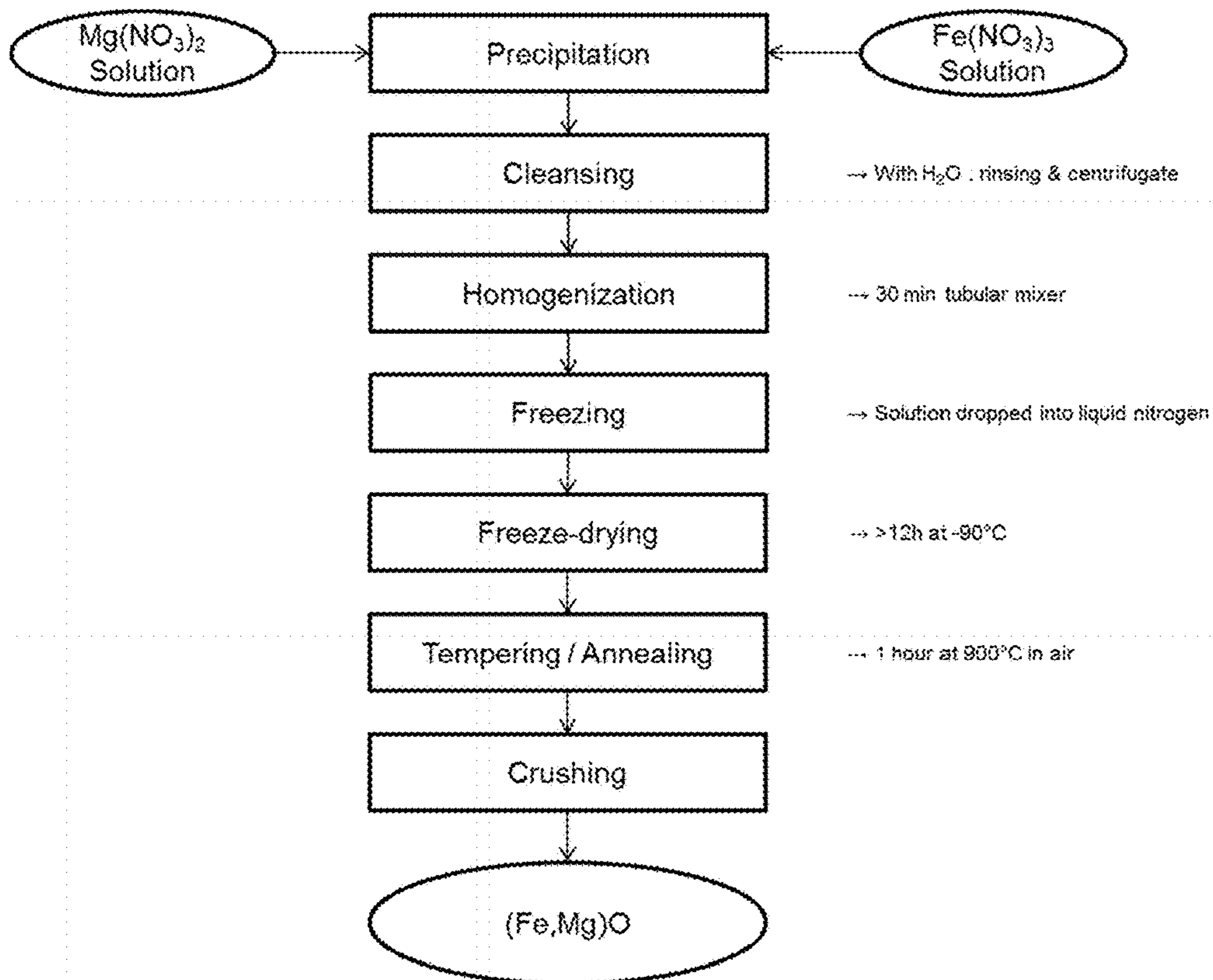
FIG. 1: preparation of oxides
