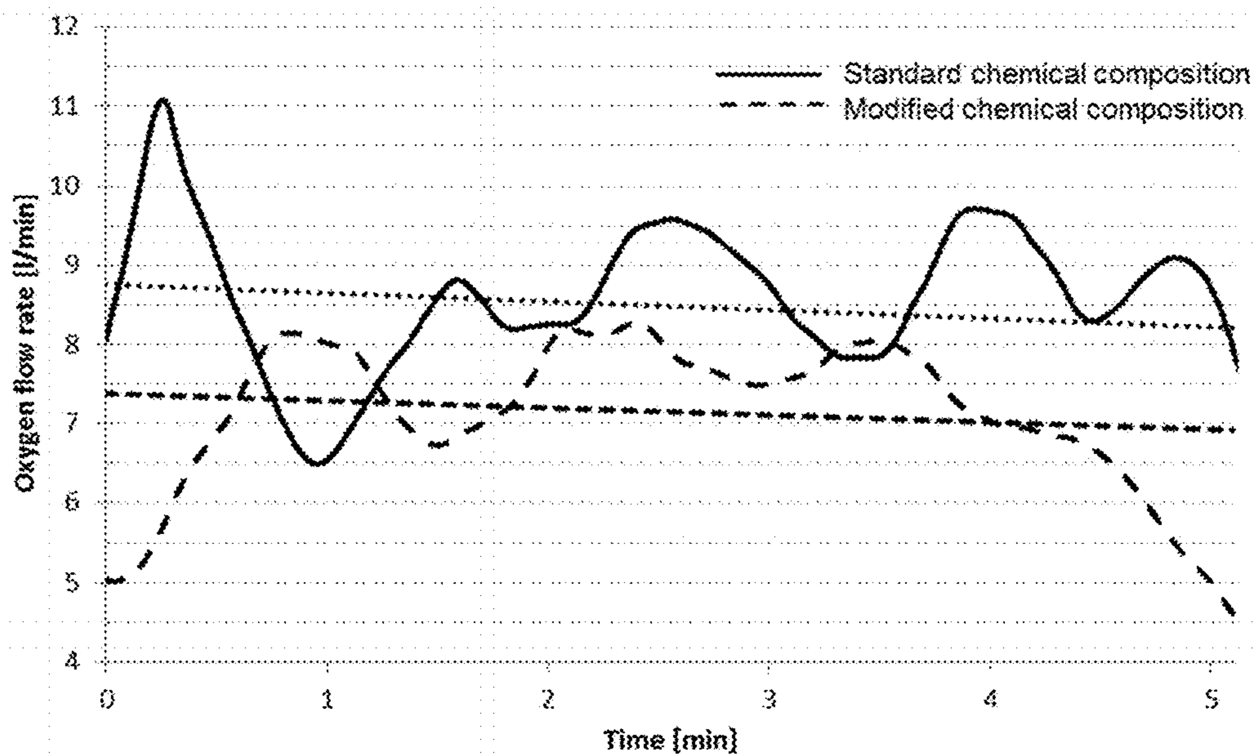
FIG. 2: Decomposition of sodium chlorate using thermally treated (Fe,Mg)O
