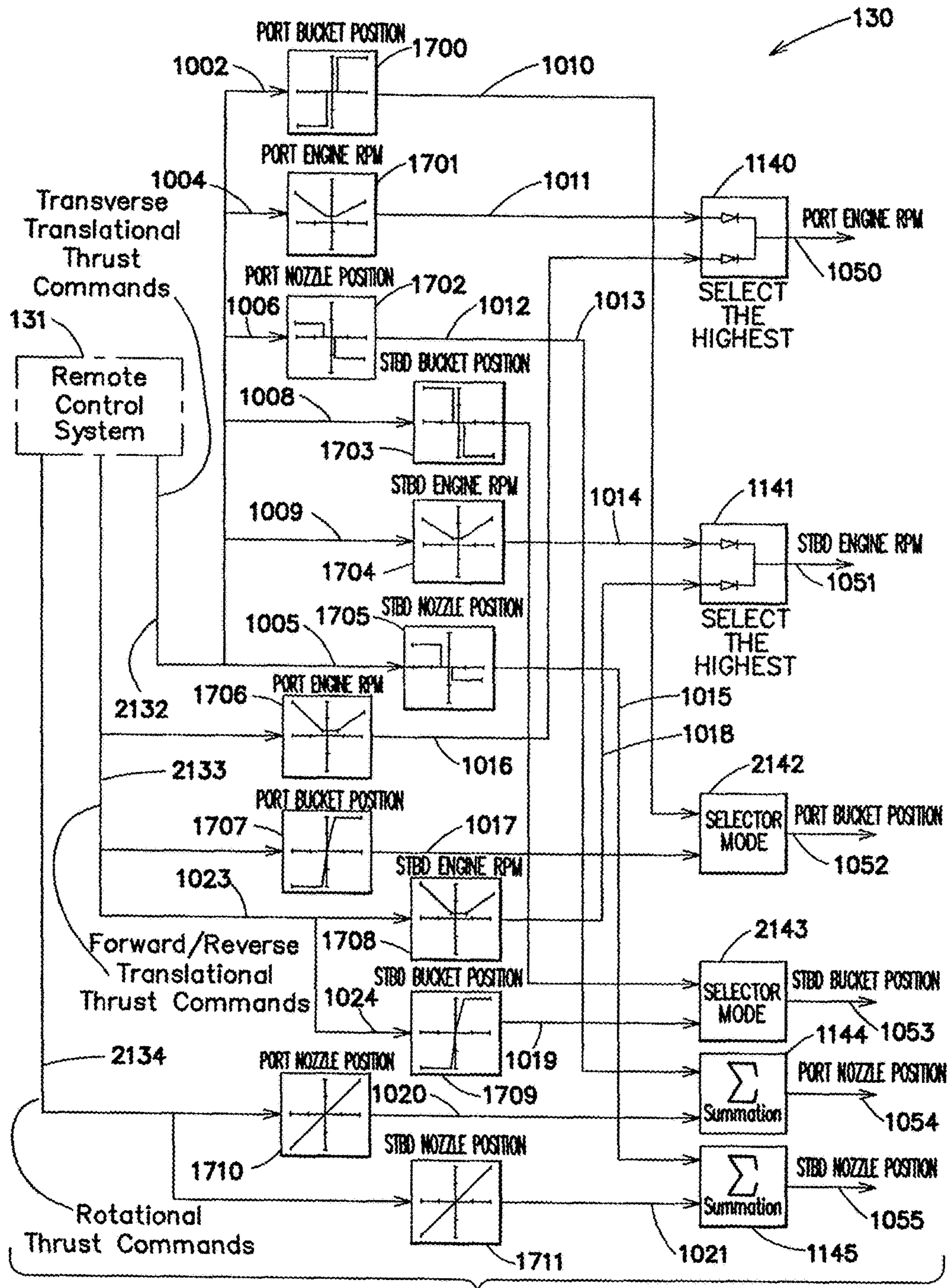
TWIN WATERJET SIGNAL DIAGRAM REMOTELY CONTROLLED
