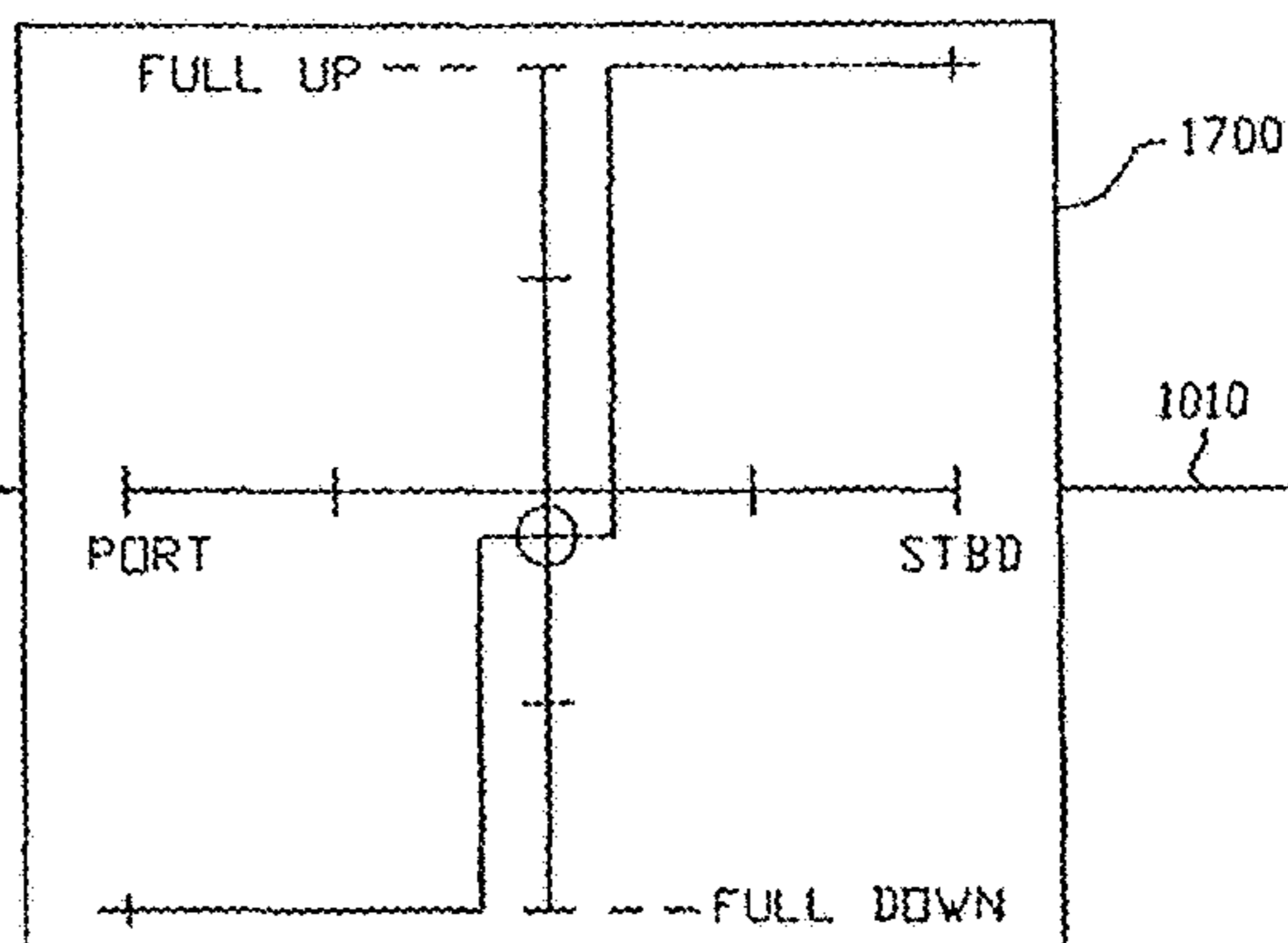
FIG. 14D PORT BUCKET POSITION
