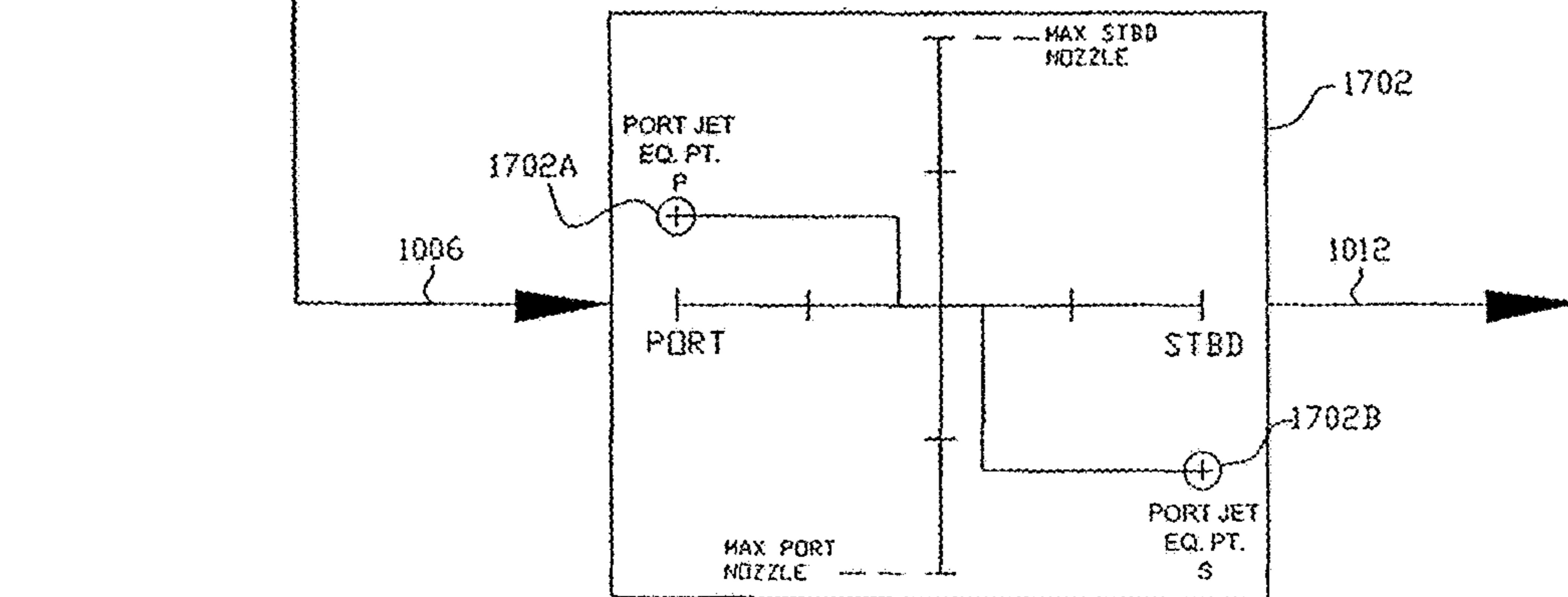
FIG. 14F PORT NOZZLE POSITION
