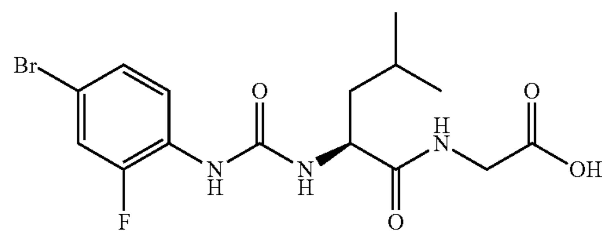
{{(2S)-2-{{(4-bromo-2-fluorophenyl)carbamoyl}amino}-4-methylpentanoyl]amino}acetic acid
