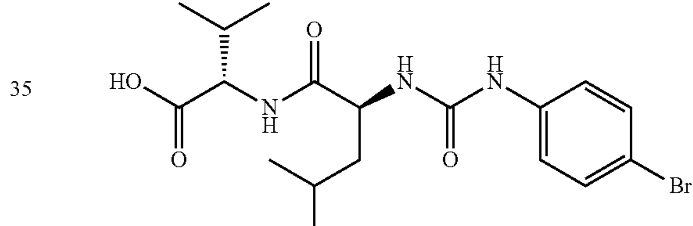
(2S)-2-[[2S)-2-[[4-bromophenyl]carbamoyl]amino]-4-methylpentanoyl]amino}-3-methylbutanoic acid
