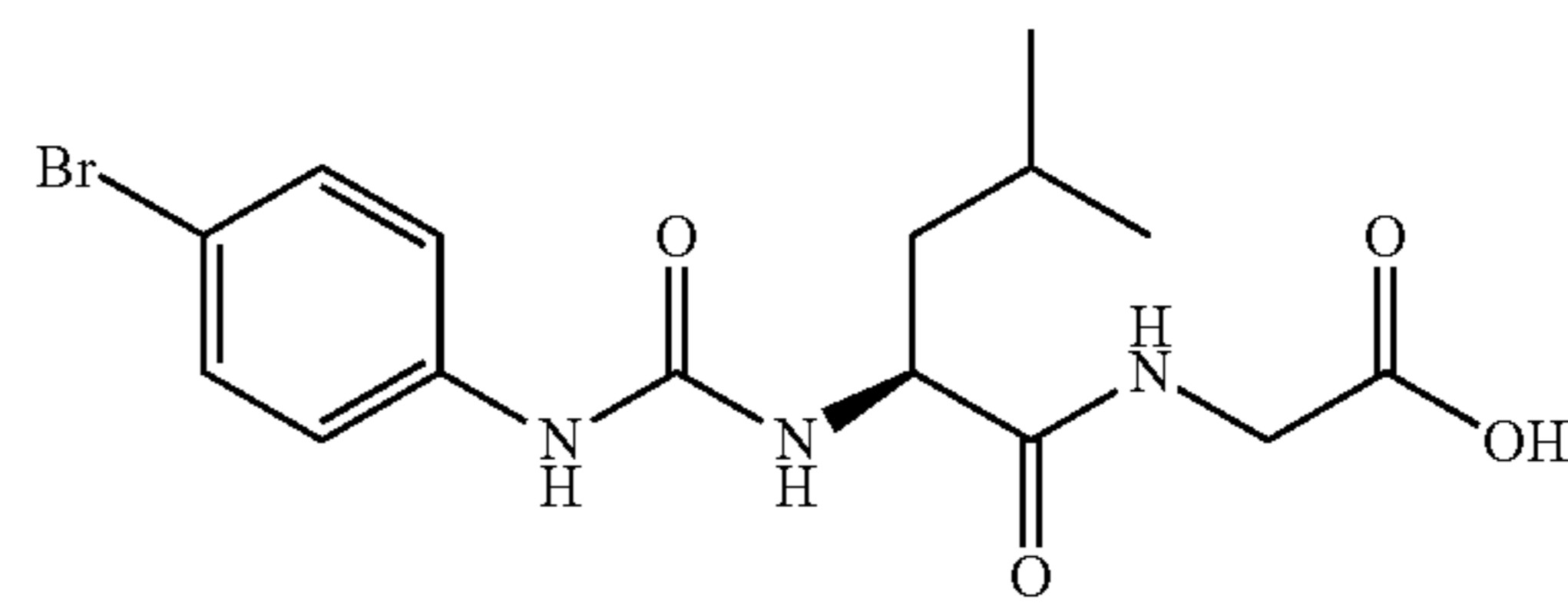
{{(2S)-2-{{(4-bromophenyl)carbamoyl}amino}-4-methylpentanoyl]amino}acetic acid
