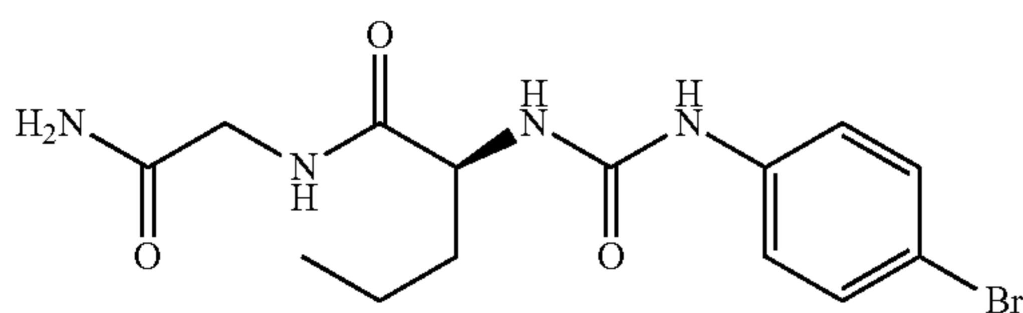
(2S)-N-(2-amino-2-oxoethyl)-2-[[4-bromophenyl]carbamoyl]amino pentanamide
