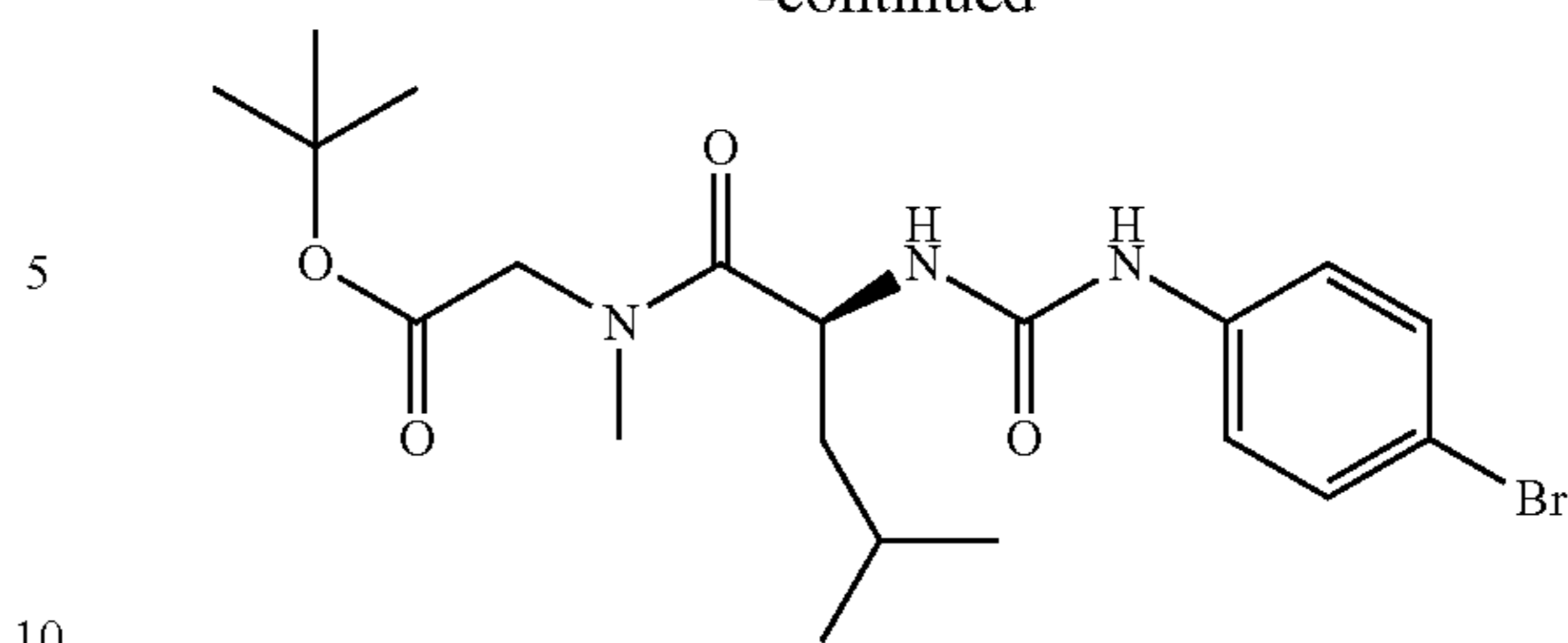
tert-butyl{[(2S)-2-({[4-bromophenyl]carbamoyl}amino)-4-methylpentanoyl](methyl)amino}acetate
