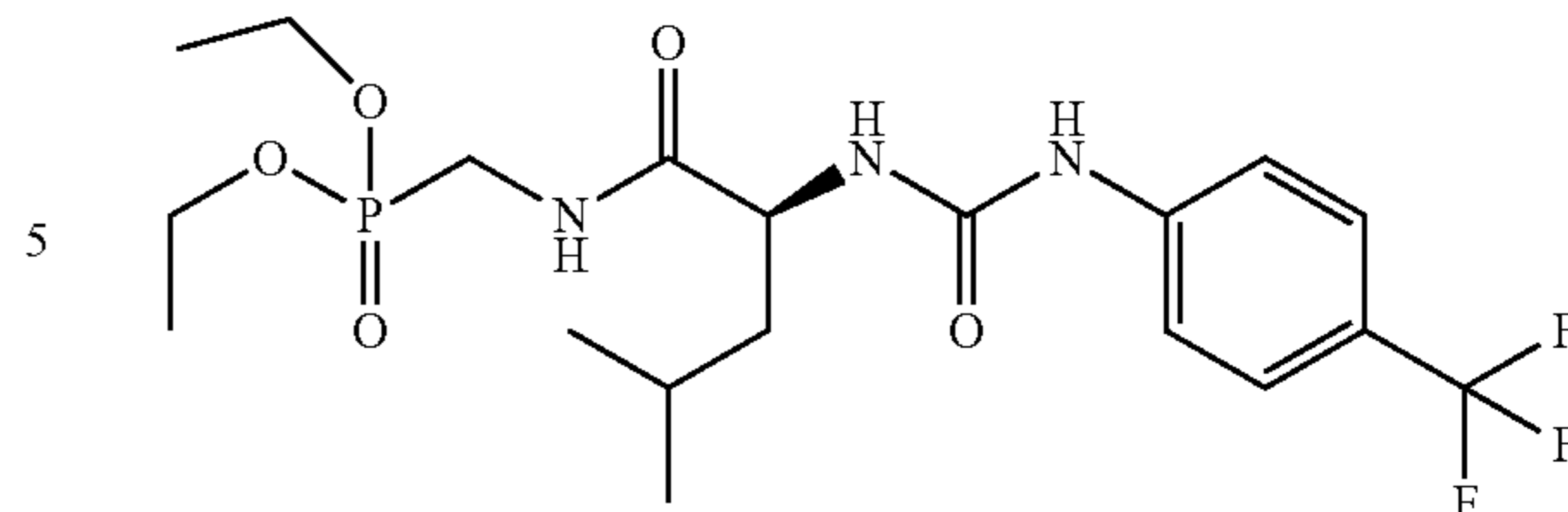
diethyl{{(2S)-4-methyl-2-{{(4-(trifluoromethyl)phenyl}carbamoyl}amino)pentanoyl]amino)methyl}phosphonate
