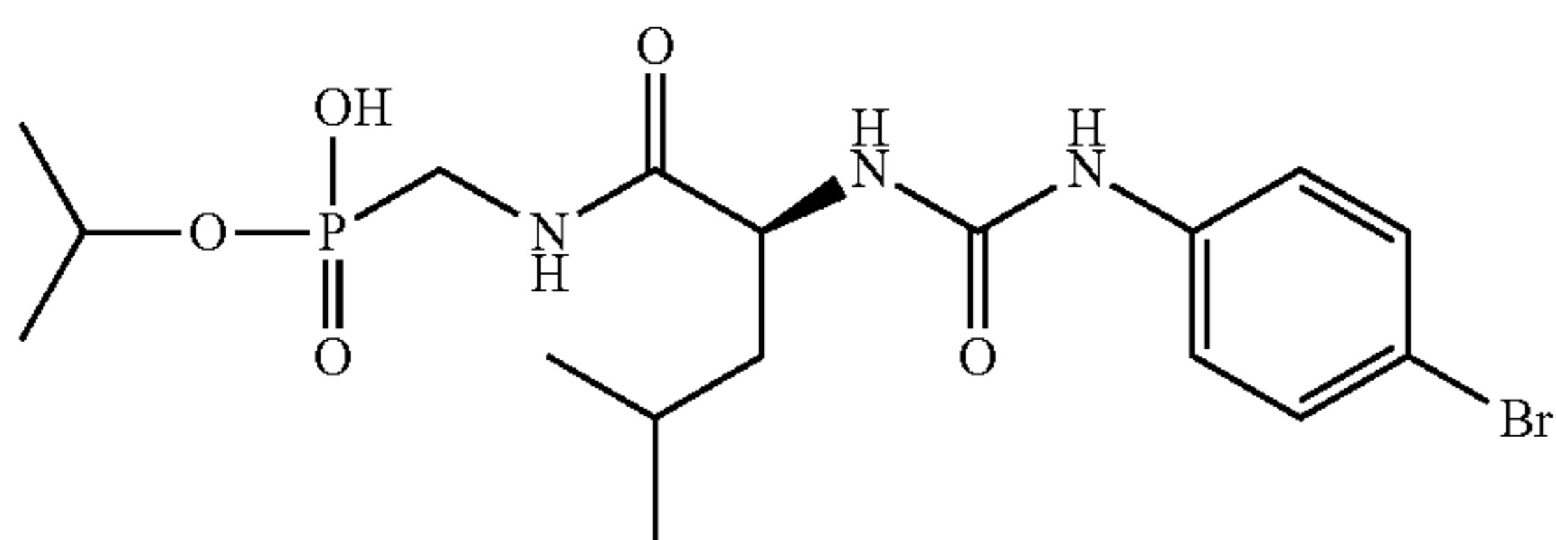
propan-2-yl hydrogen{{(2-{{(4-bromophenyl)carbamoyl}amino}pentanoyl]amino)methyl}phosphonate
