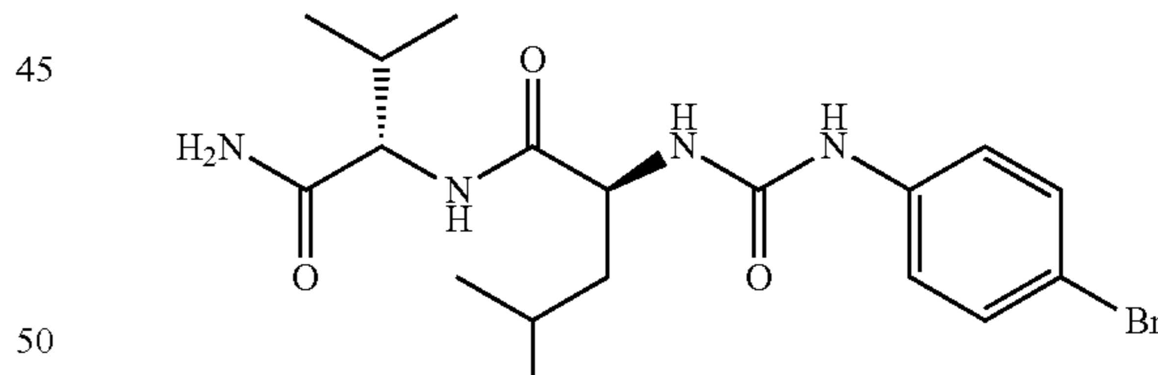
(2S)-N-[(2S)-1-amino-3-methyl-1-oxobutan-2-yl]-2-[[4-bromophenyl]carbamoyl]amino-4-methylpentanamide
