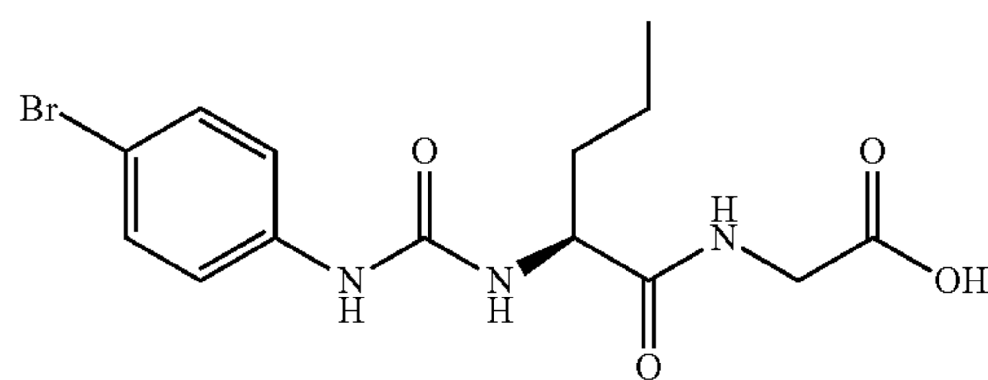
{[(2S)-2-{{(4-bromophenyl)carbamoyl}amino}pentanoyl]amino}acetic acid
