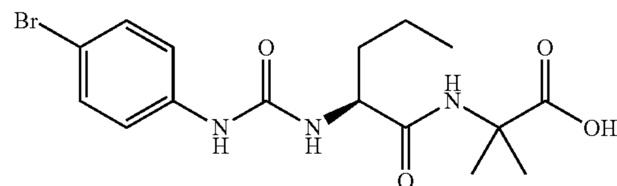
2-{{(2S)-2-{{(4-bromophenyl)carbamoyl}amino}-4-methylpentanoyl]amino}-2-methylpropanoic acid
