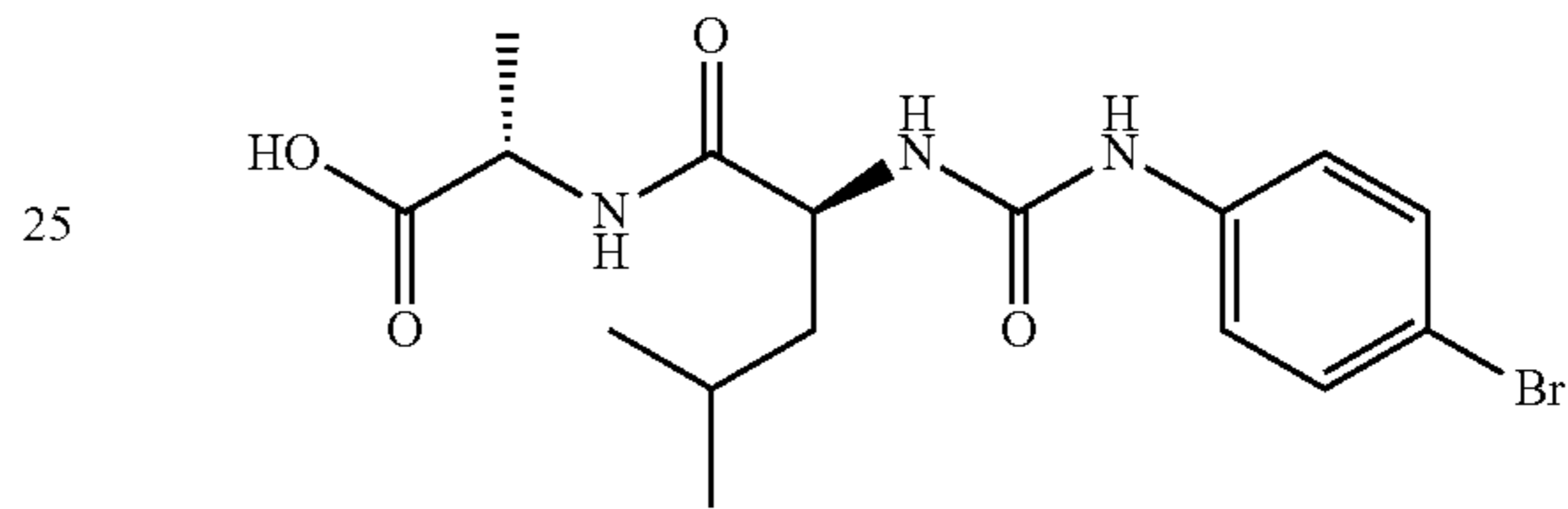
(2S)-2-[[2S)-2-[[4-bromophenyl]carbamoyl]amino]-4-methylpentanoyl]amino}propanoic acid
