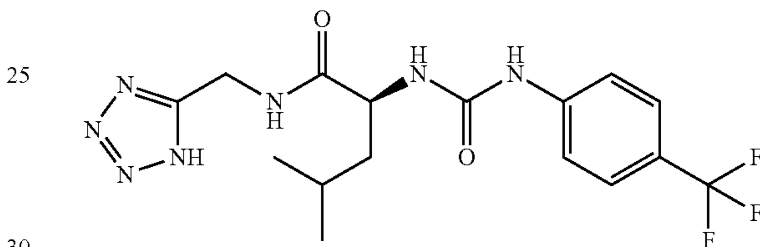
(2S)-4-methyl-N-(1H-tetrazol-5-ylmethyl)-2-((4-(trifluoromethyl)phenyl)carbamoyl)amino)pentanamide
