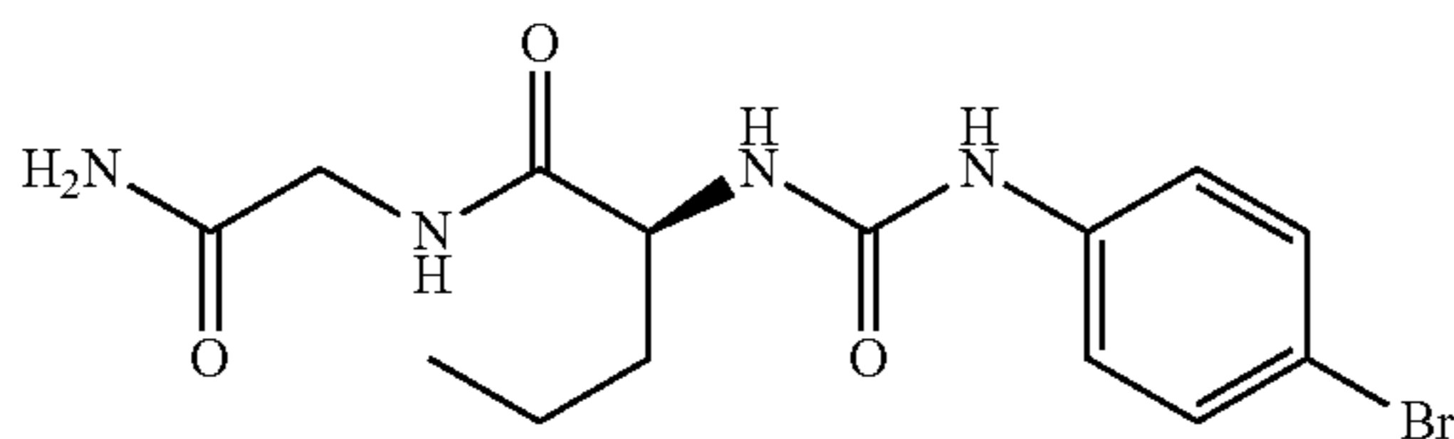
(2S)-N-(2-amino-2-oxoethyl)-2-[[4-bromophenyl]carbamoyl]amino pentanamide
