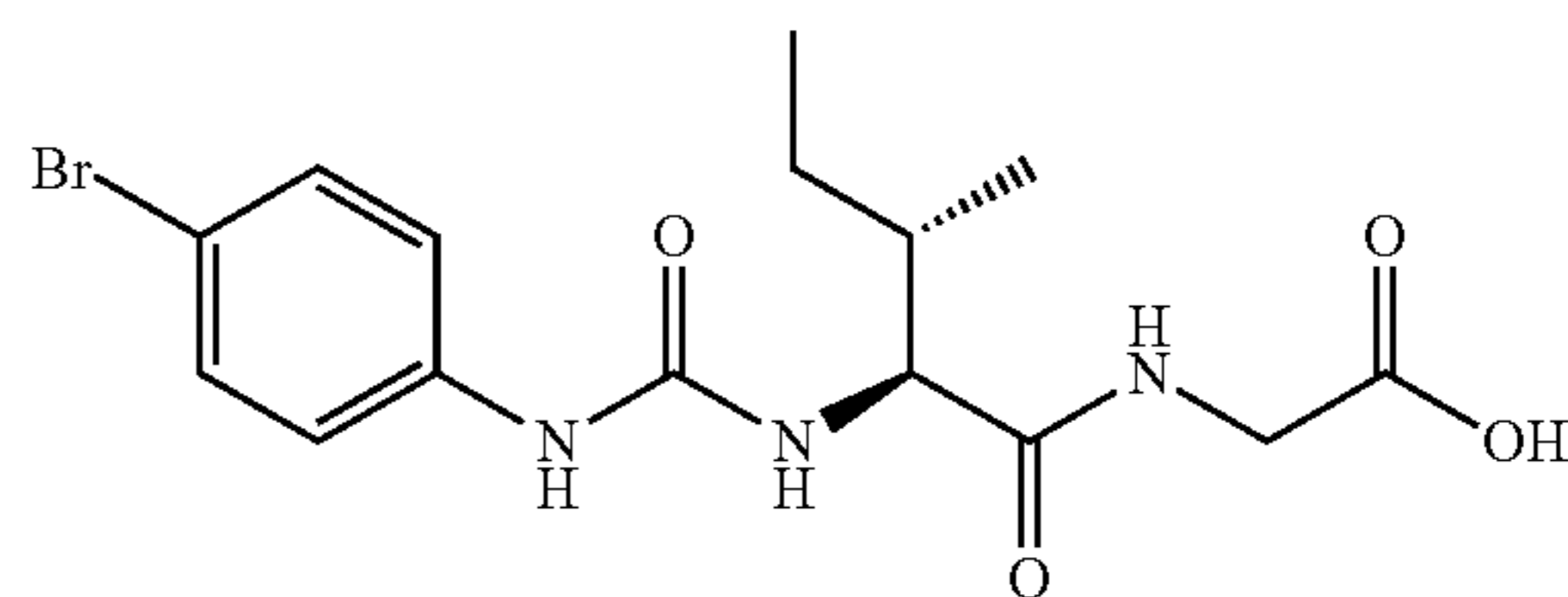
{{(2S,3S)-2-{{(4-bromophenyl)carbamoyl}amino}-3-methylpentanoyl]amino}acetic acid
