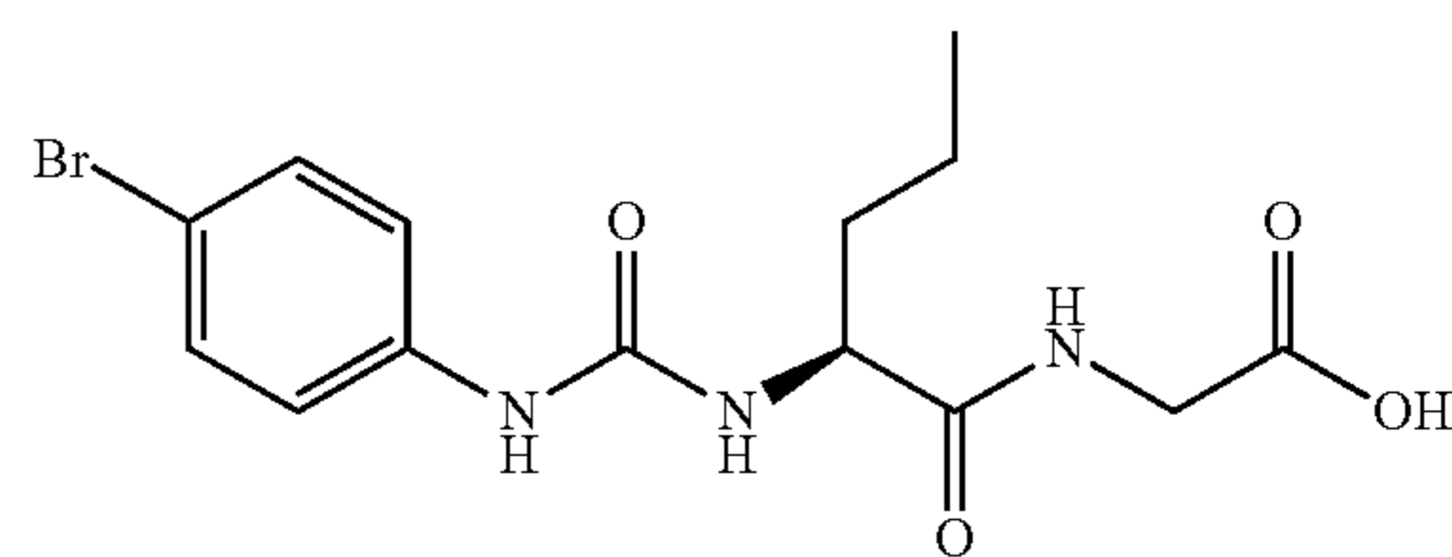
{[(2S)-2-{{(4-bromophenyl)carbamoyl}amino}pentanoyl]amino}acetic acid
