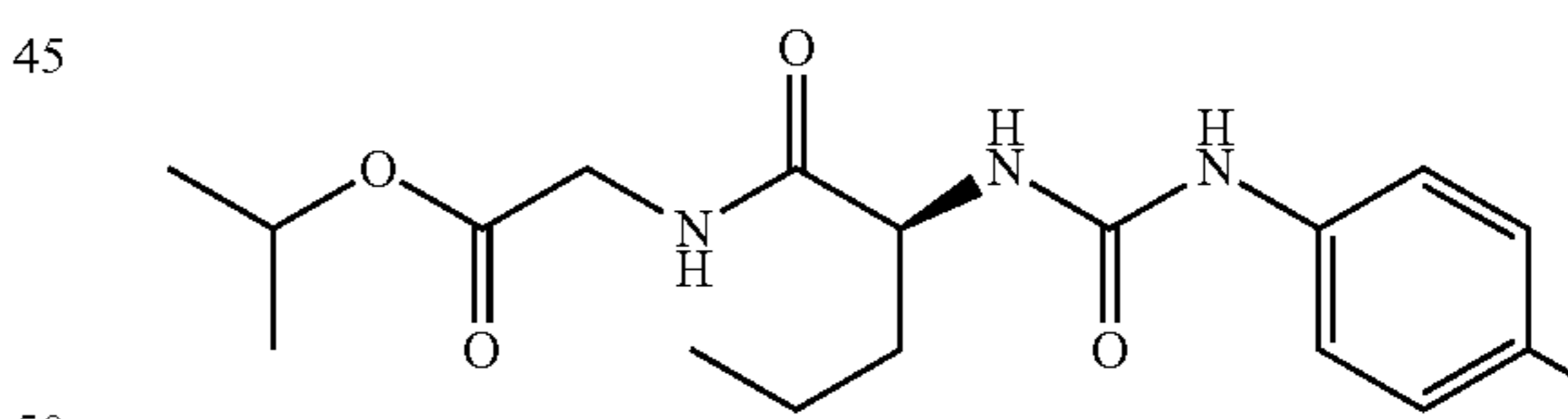
propan-2-yl{{(2S)-2-{{(4-bromophenyl)carbamoyl}amino}pentanoyl amino}acetate
