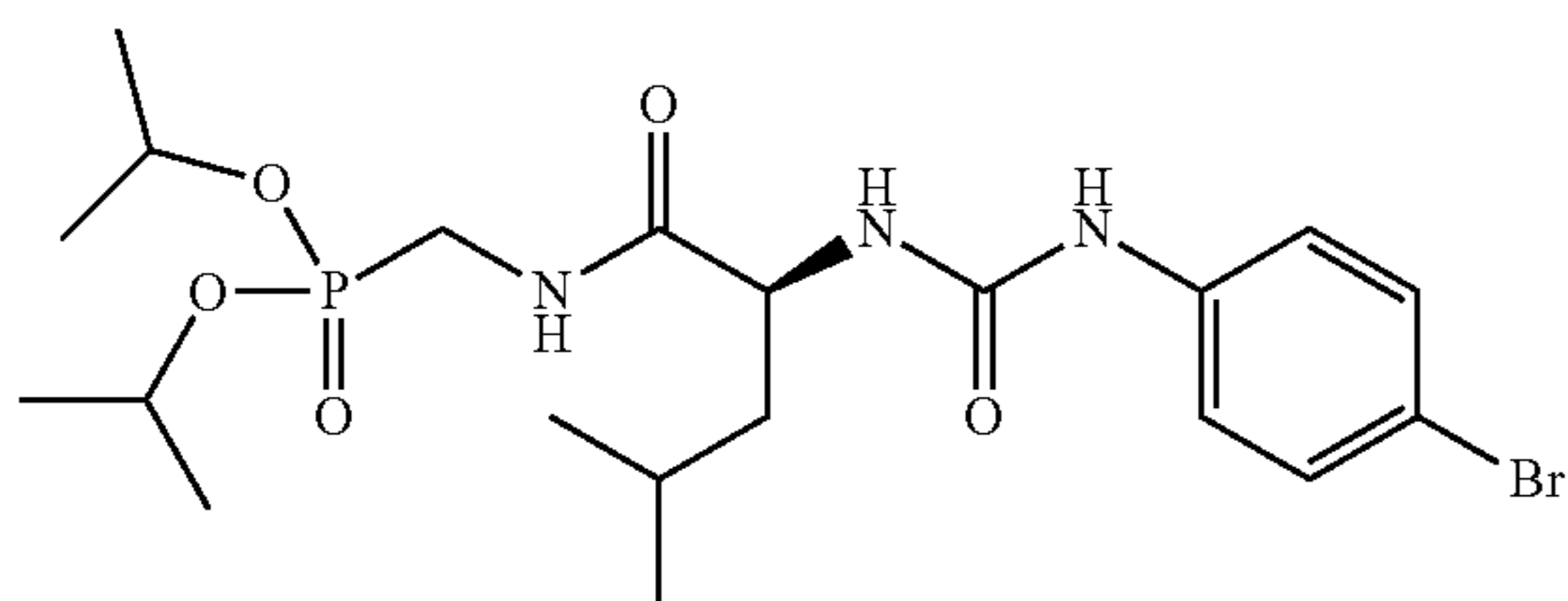
dipropan-2-yl ((2S)-2-((4-bromophenyl)carbamoyl)amino)-4-methylpentanoate methyl phosphonate
