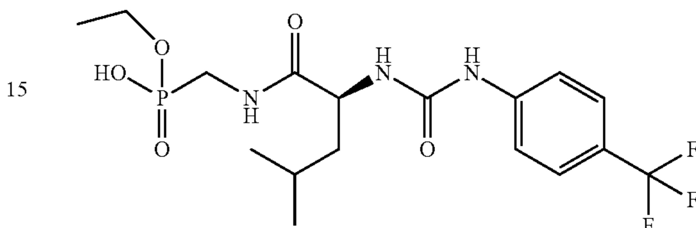
ethyl hydrogen ((2S)-4-methyl-2-((4-(trifluoromethyl)phenyl)carbamoyl)amino)pentanoate
