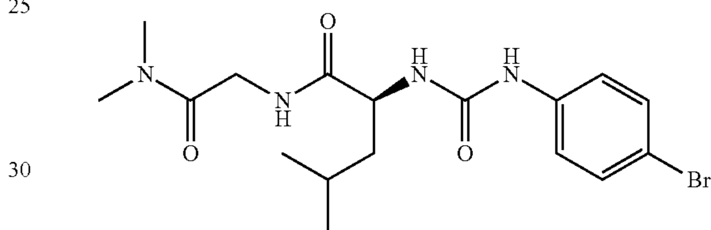
(2S)-2-((4-bromophenyl)carbamoyl)amino)-N-[2-(dimethylamino)-2-oxoethyl]-4-methylpentanamide
