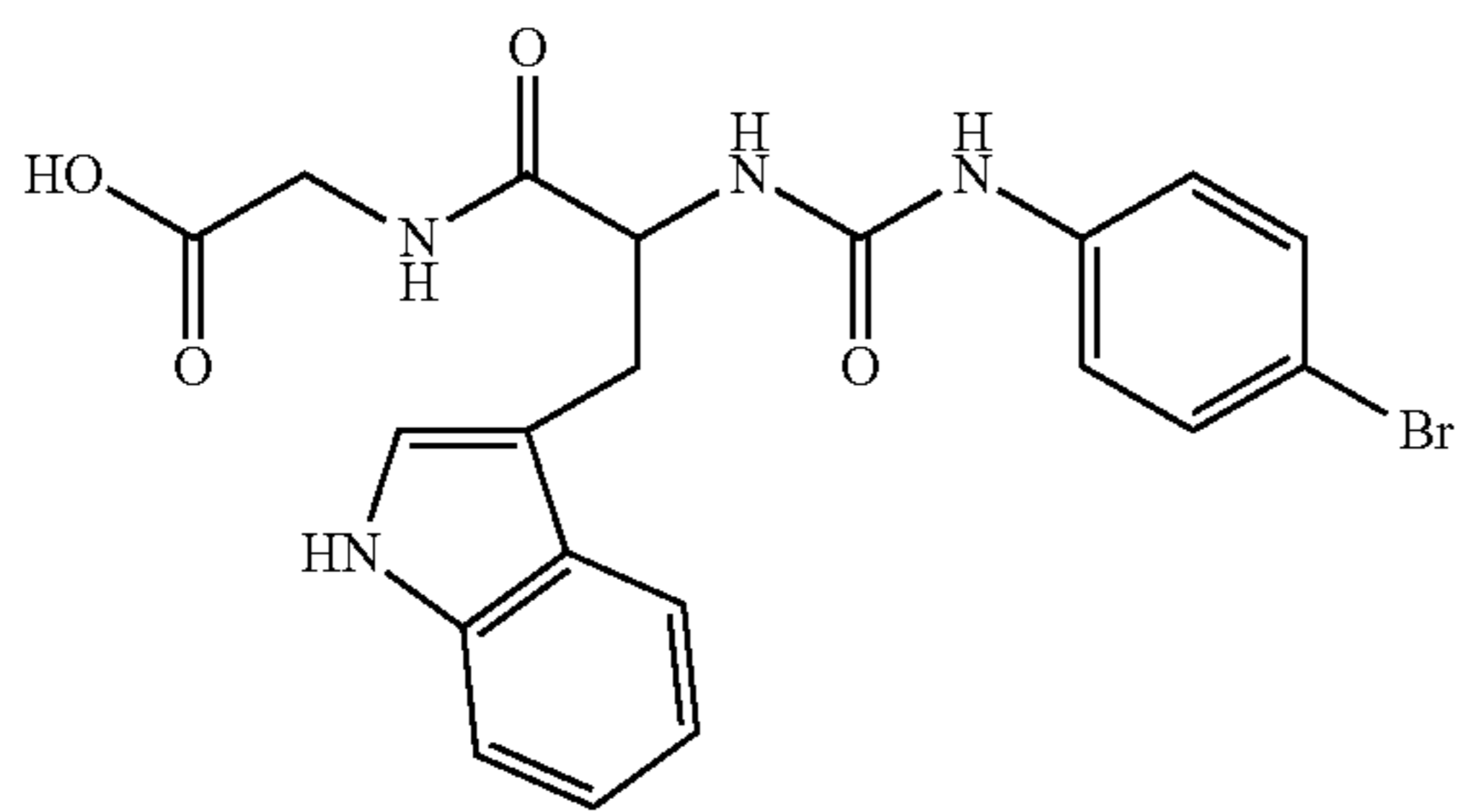
{[(2S)-2-({[4-bromophenyl]carbamoyl}amino)-3-(1H-indol-3-yl)propanoyl]amino}acetic acid
