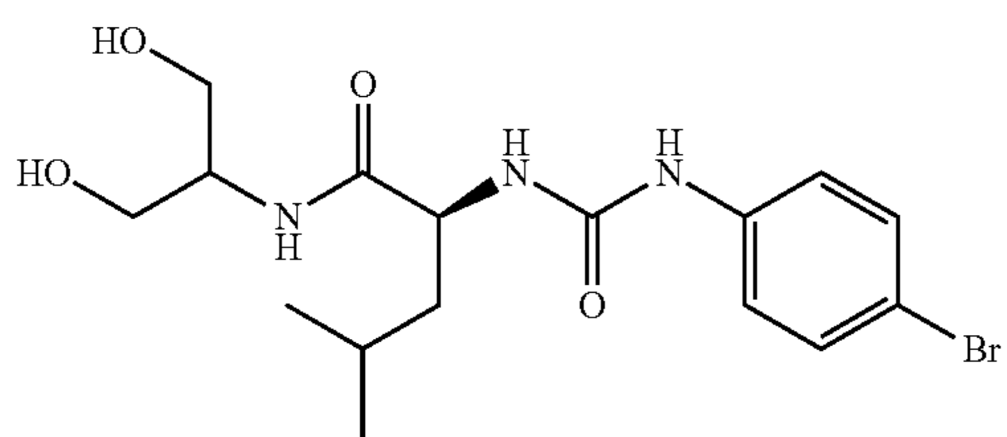
(2S)-2-([(4-bromophenyl)carbamoyl]amino)-N-(1,3-dihydroxypropan-2-yl)-4-methylpentanamide
