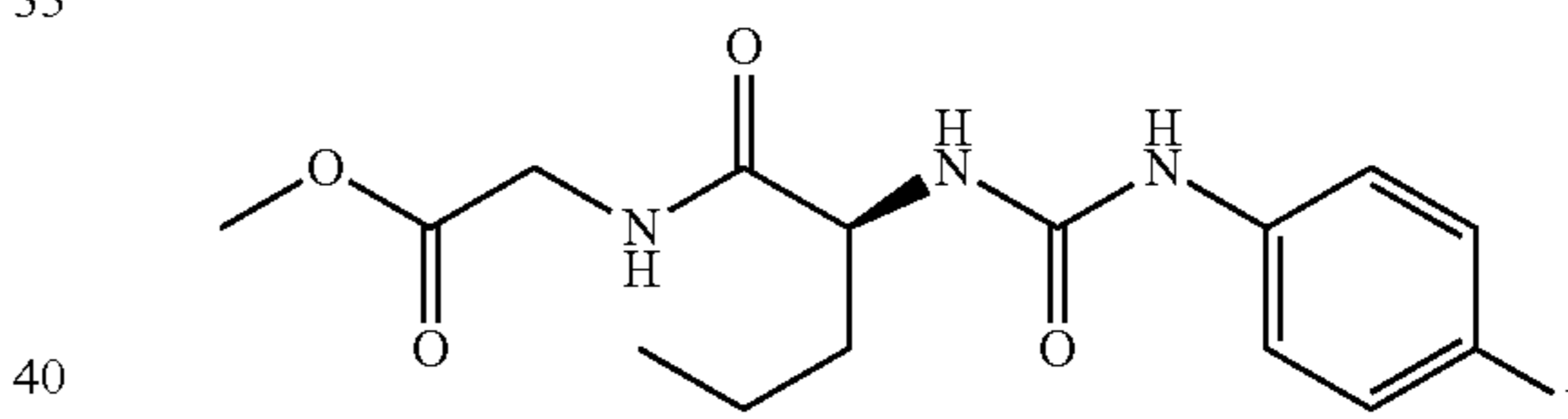
methyl{{(2S)-2-{{(4-bromophenyl)carbamoyl}amino}pentanoyl amino}acetate
