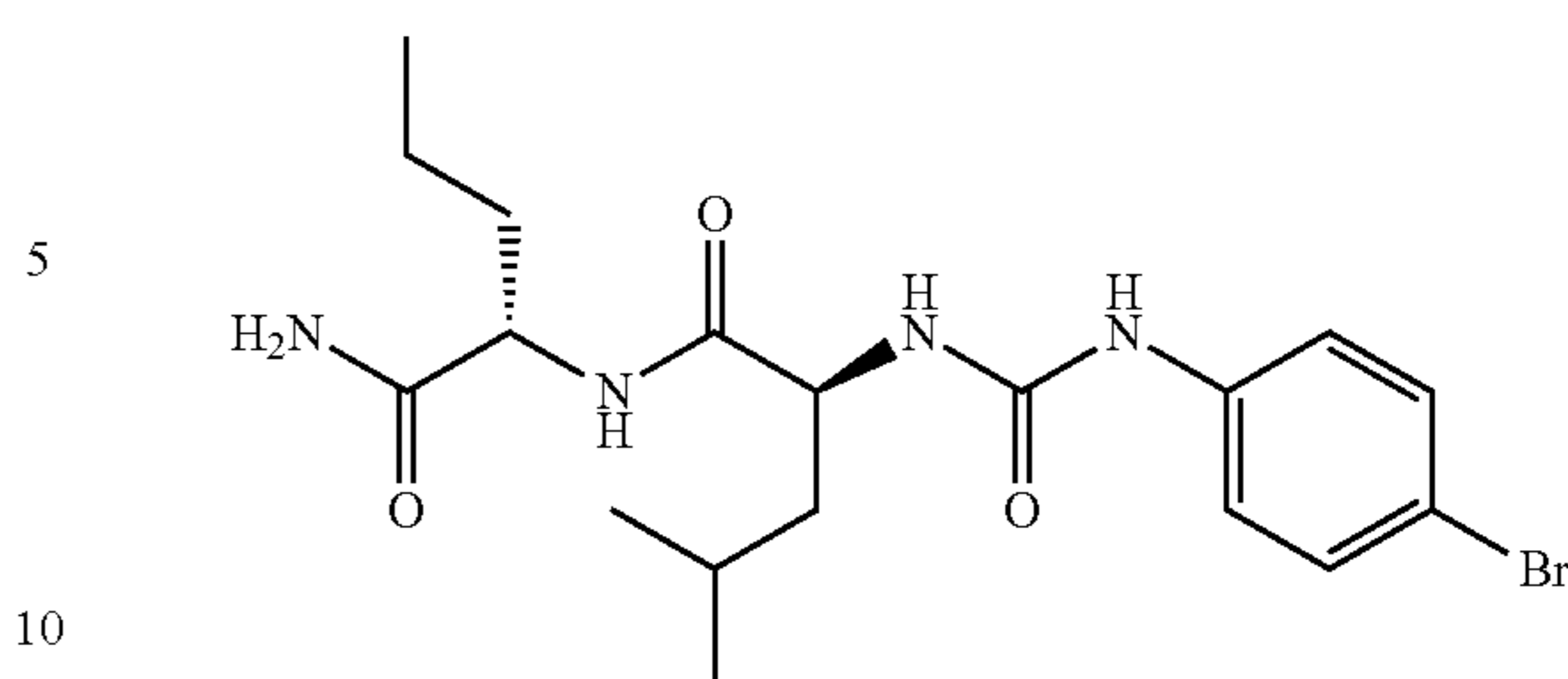
(2S)-N-[(2S)-1-amino-1-oxopentan-2-yl]-2-([(4-bromophenyl)carbamoyl]amino)-4-methylpentanamide
