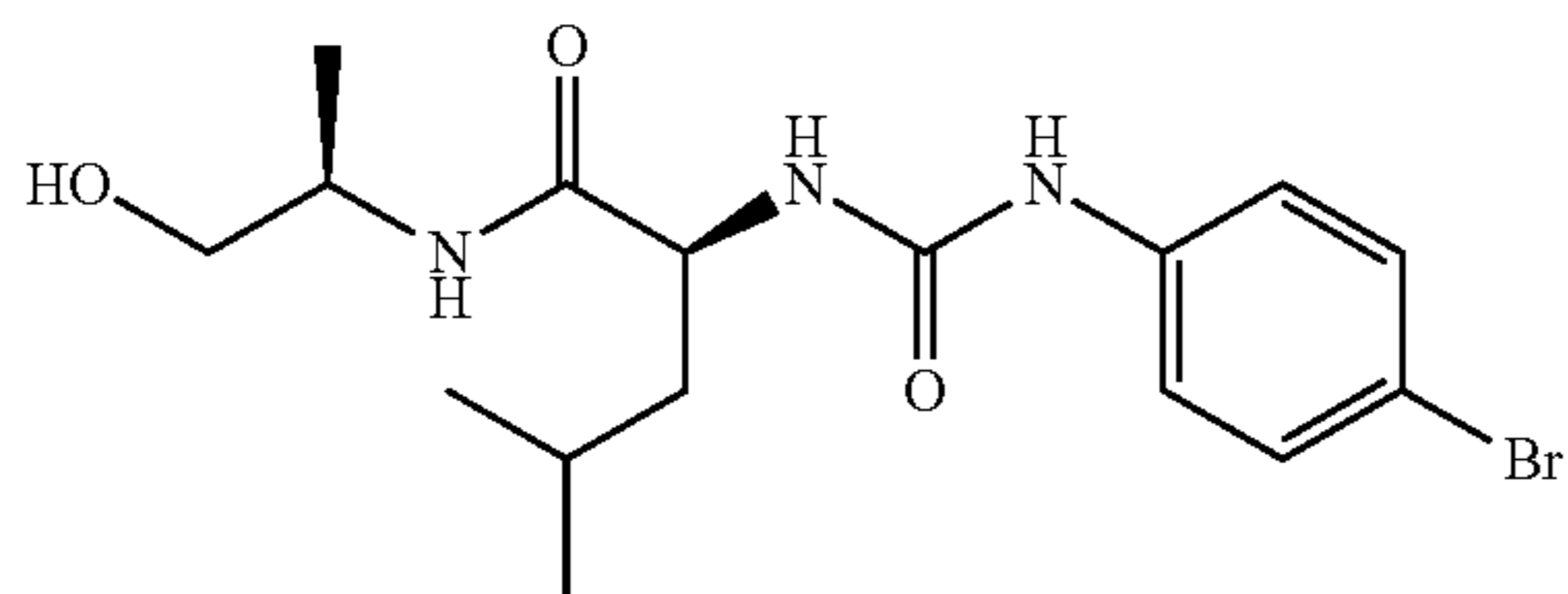
(2S)-2-([(4-bromophenyl)carbamoyl]amino)-N-[(2R)-1-hydroxypropan-2-yl]-4-methylpentanamide
