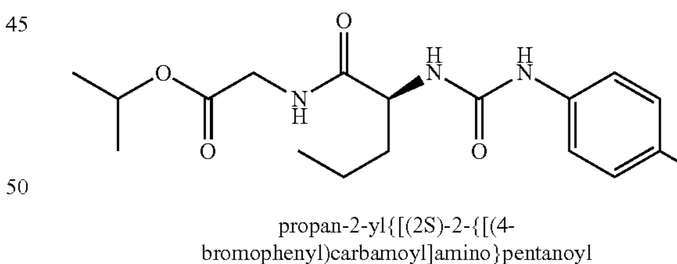
methyl{{(2S)-2-{{(4-bromophenyl)carbamoyl}amino}pentanoyl amino}acetate
