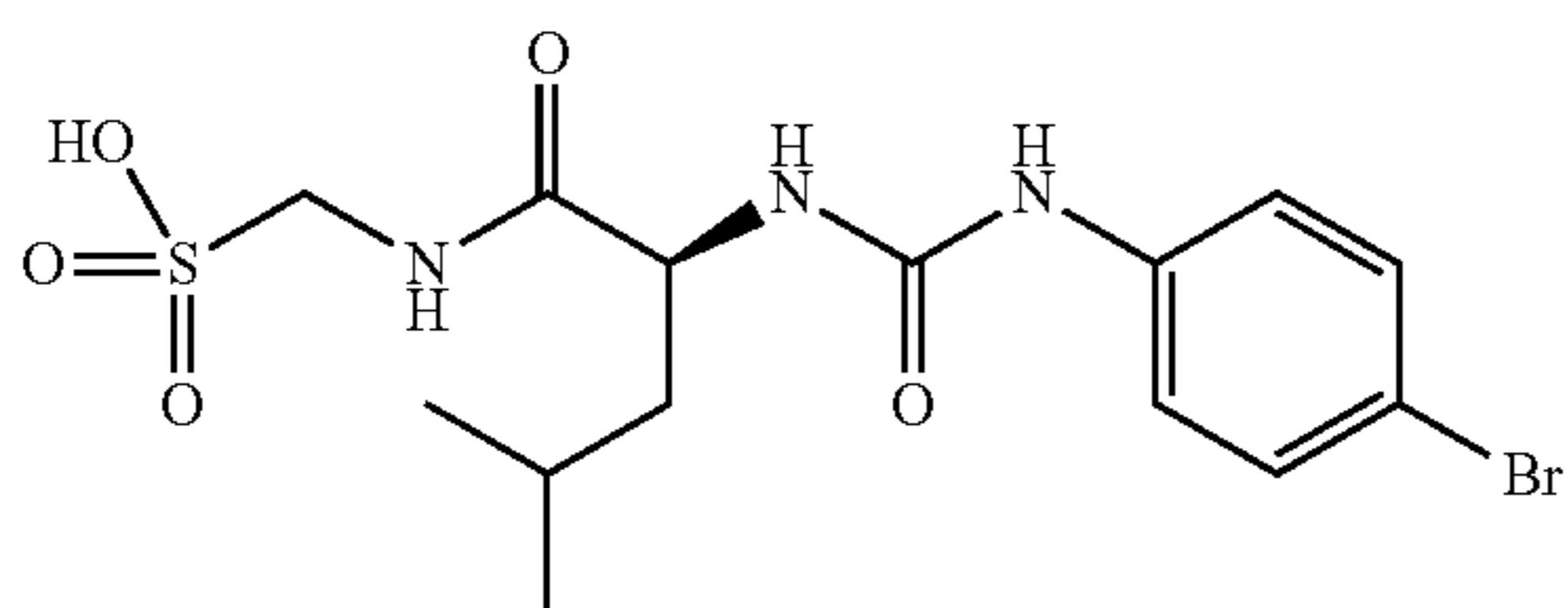
((2S)-2-((4-bromophenyl)carbamoyl)amino)-4-methylpentanoate methanesulfonic acid
