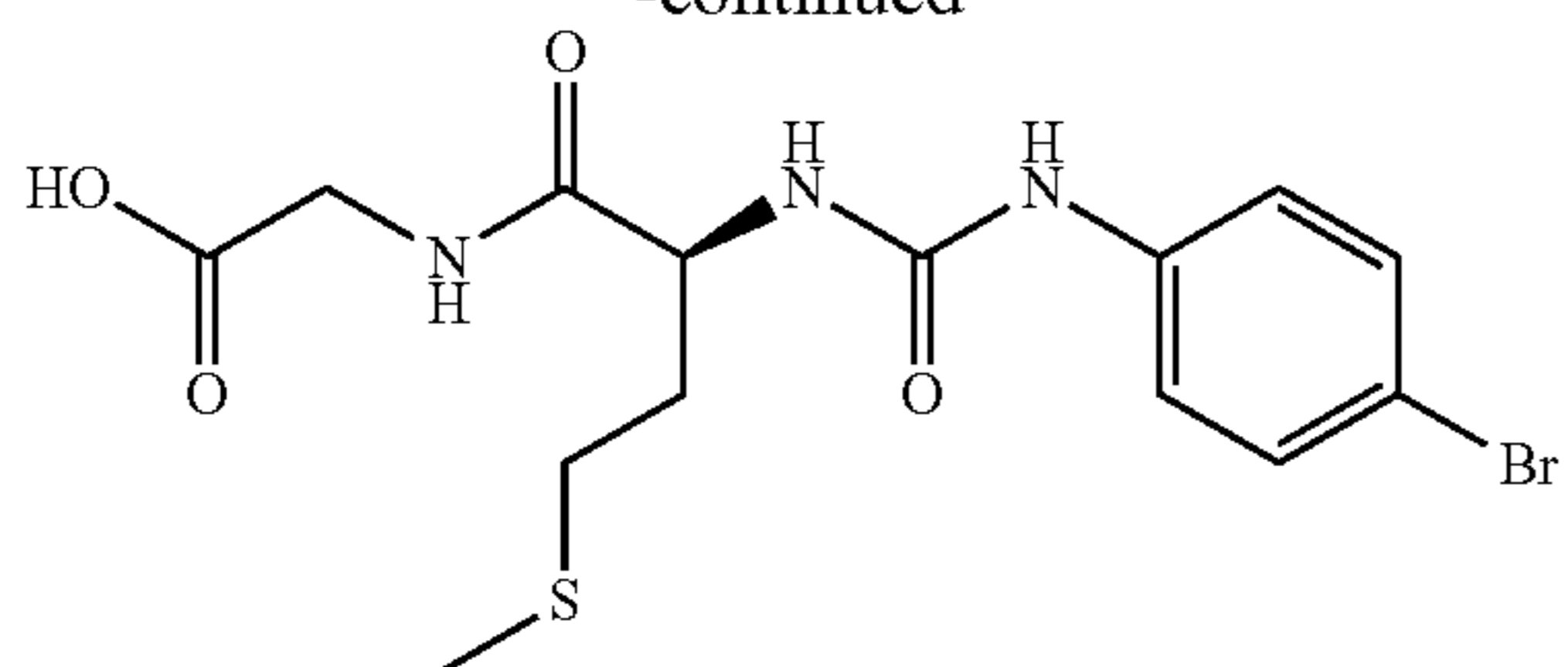
{[(2S)-2-({[4-bromophenyl]carbamoyl}amino)-4-(methylsulfanyl)butanoyl]amino}acetic acid
