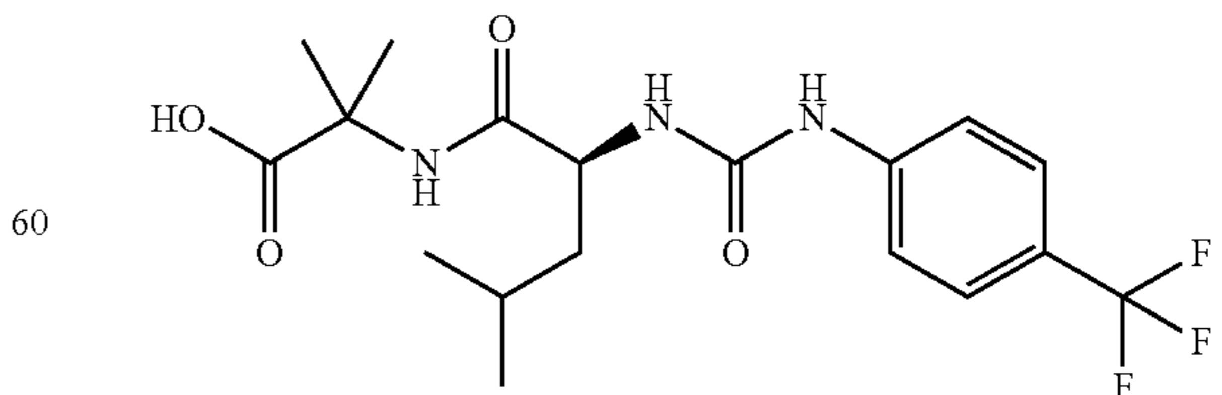
2-methyl-2-{{(2S)-4-methyl-2-{{(4-(trifluoromethyl)phenyl}carbamoyl}amino)pentanoyl]amino}propanoic acid
