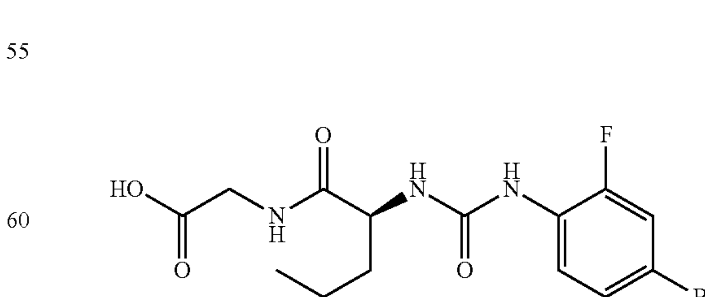
{{(2S)-2-{{(4-bromo-2-fluorophenyl)carbamoyl}amino}pentanoyl amino}acetate acid
