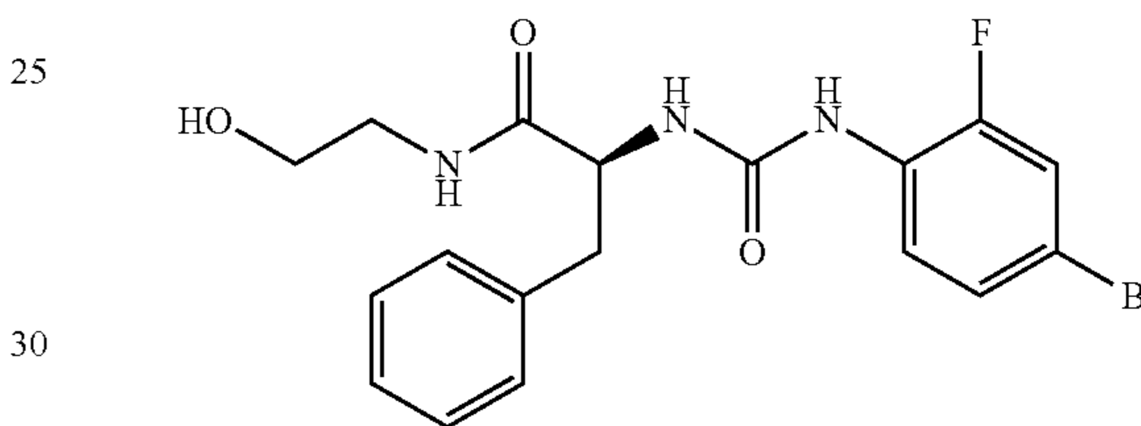
(2S)-2-{{(4-bromo-2-fluorophenyl)carbamoyl}amino}-N-(2-hydroxyethyl)-3-phenylpropanamide
