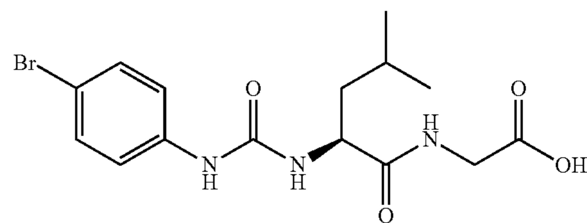
{{(2S)-2-{{(4-bromophenyl)carbamoyl}amino}-4-methylpentanoyl]amino}acetic acid
