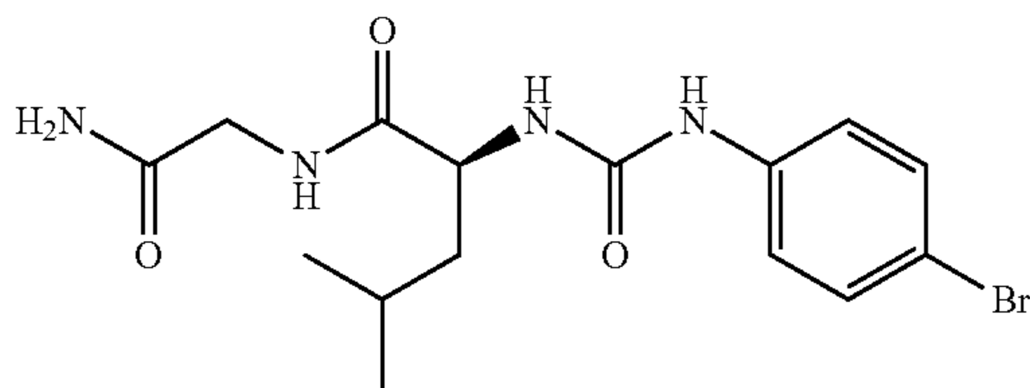
(2S)-N-(2-amino-2-oxoethyl)-2-[[4-bromophenyl]carbamoyl]amino-4-methylpentanamide
