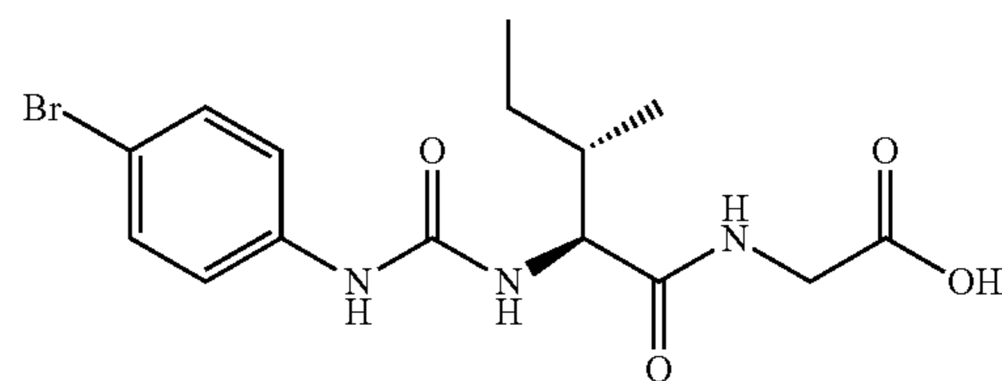
{{(2S,3S)-2-{{(4-bromophenyl)carbamoyl}amino}-3-methylpentanoyl]amino}acetic acid
