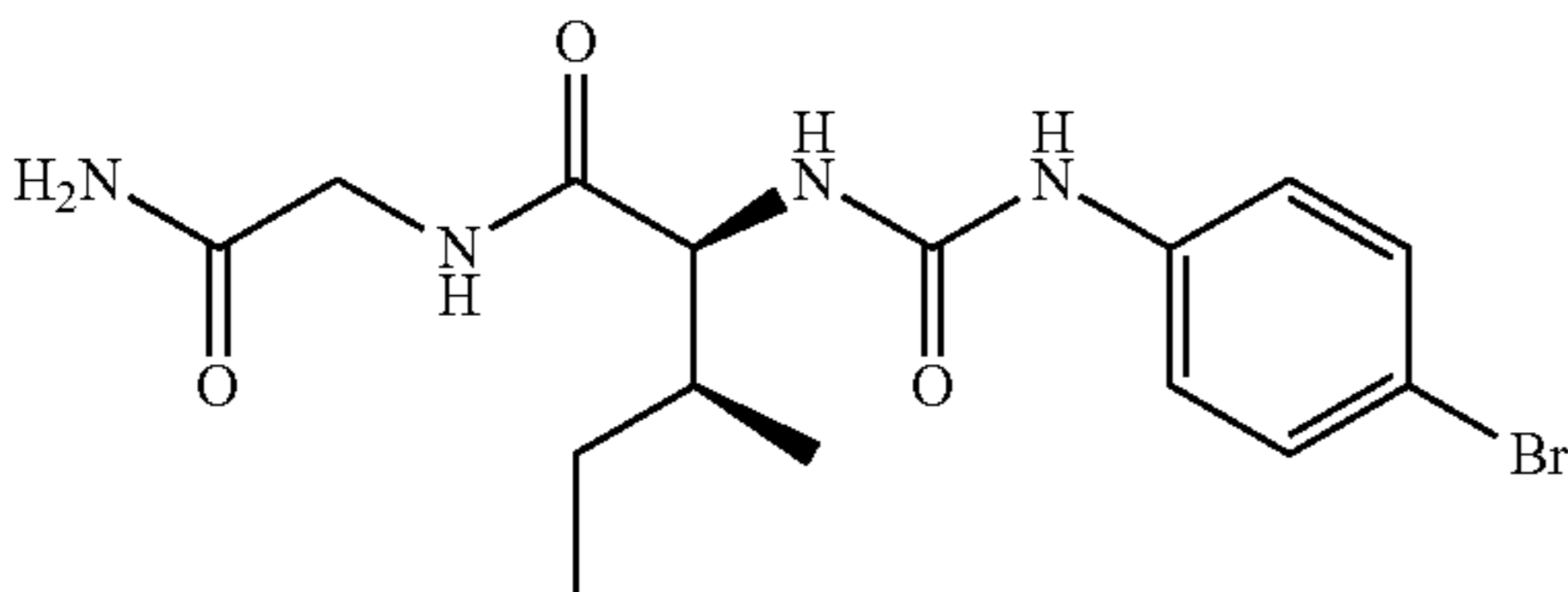
(2S,3S)-N-(2-amino-2-oxoethyl)-2-{{(4-bromophenyl)carbamoyl}amino}-3-methylpentanamide
