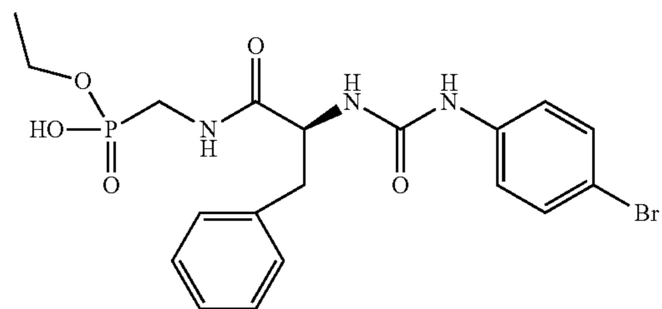
ethyl hydrogen (2-((4-bromophenyl)carbamoyl)amino)-3-phenylpropanoate methyl phosphonate
