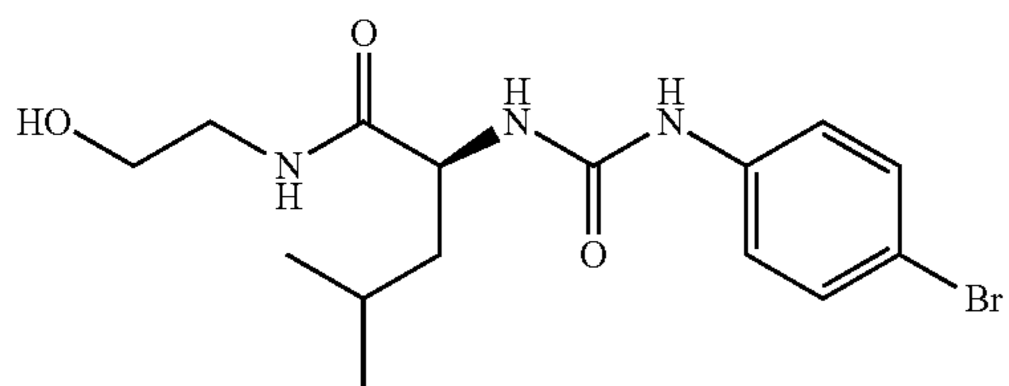
(2S)-2-[[4-bromophenyl]carbamoyl]amino-N-(2-hydroxyethyl)-4-methylpentanamide
