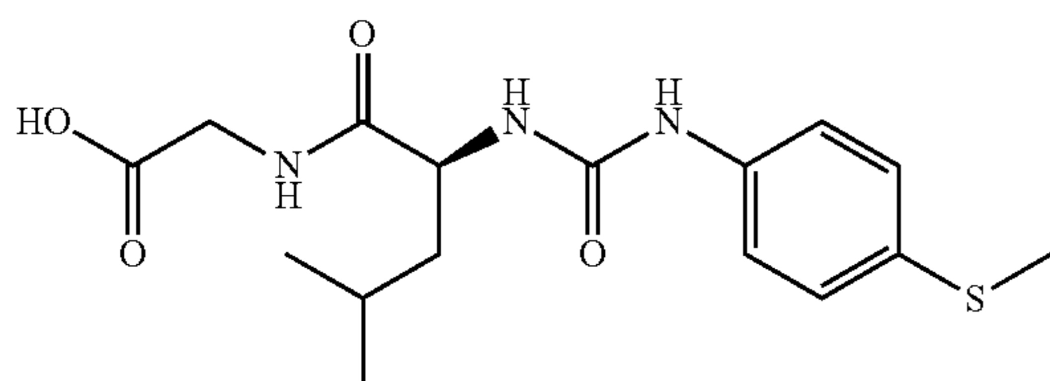
((2S)-4-methyl-2-((4-methylsulfanyl)phenyl)carbamoyl)amino)pentanoate acetic acid
