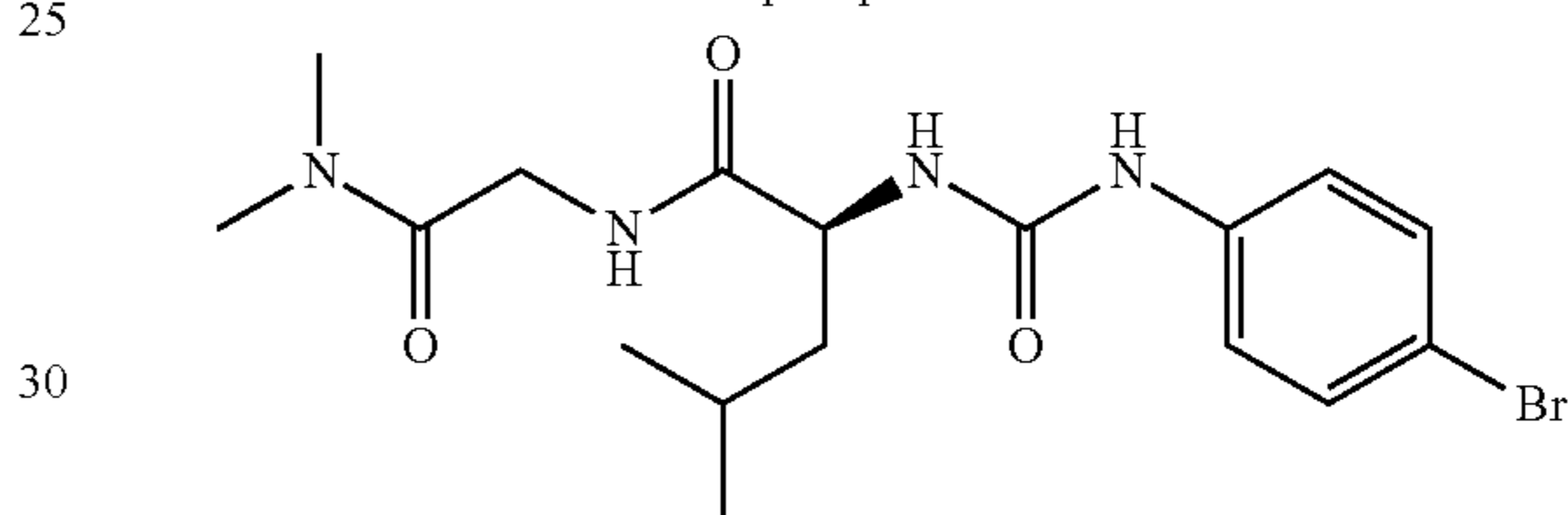
(2S)-2-((4-bromophenyl)carbamoyl)amino)-N-[2-(dimethylamino)-2-oxoethyl]-4-methylpentanamide
