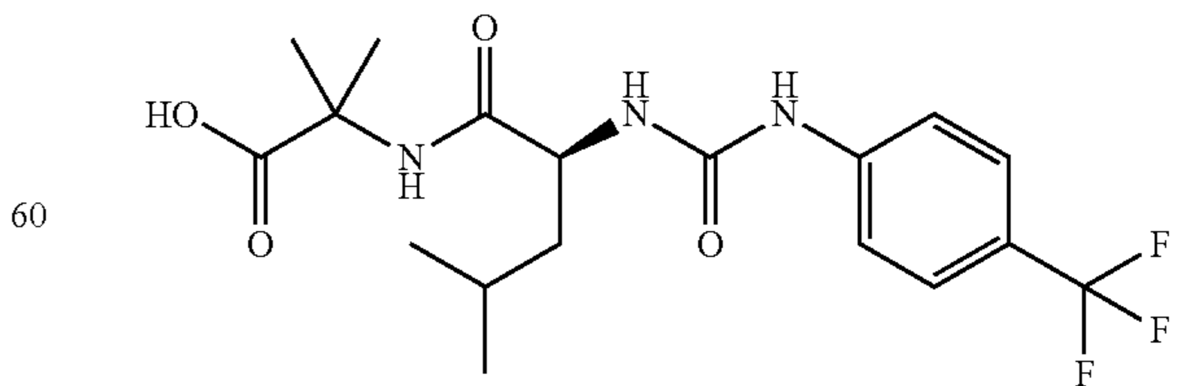
2-methyl-2-((2S)-4-methyl-2-((4-(trifluoromethyl)phenyl)carbamoyl)amino)pentanoate propanoic acid
