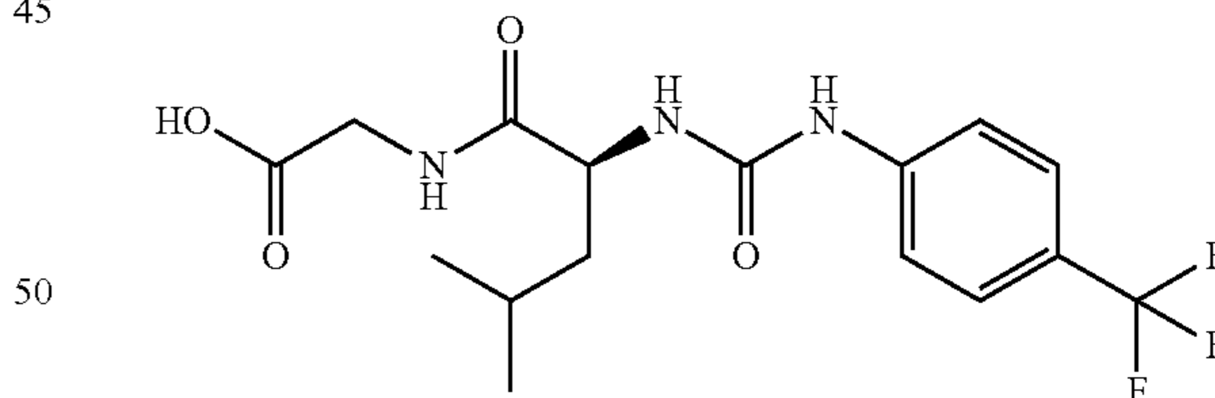
((2S)-4-methyl-2-((4-(trifluoromethyl)phenyl)carbamoyl)amino)pentanoyl]amino)acetic acid
