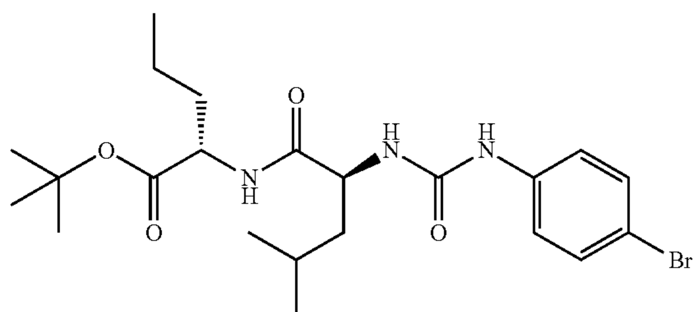
tert-butyl (2S)-2-([(2S)-2-([(4-bromophenyl)carbamoyl]amino)-4-methylpentanoyl]amino)pentanoate
