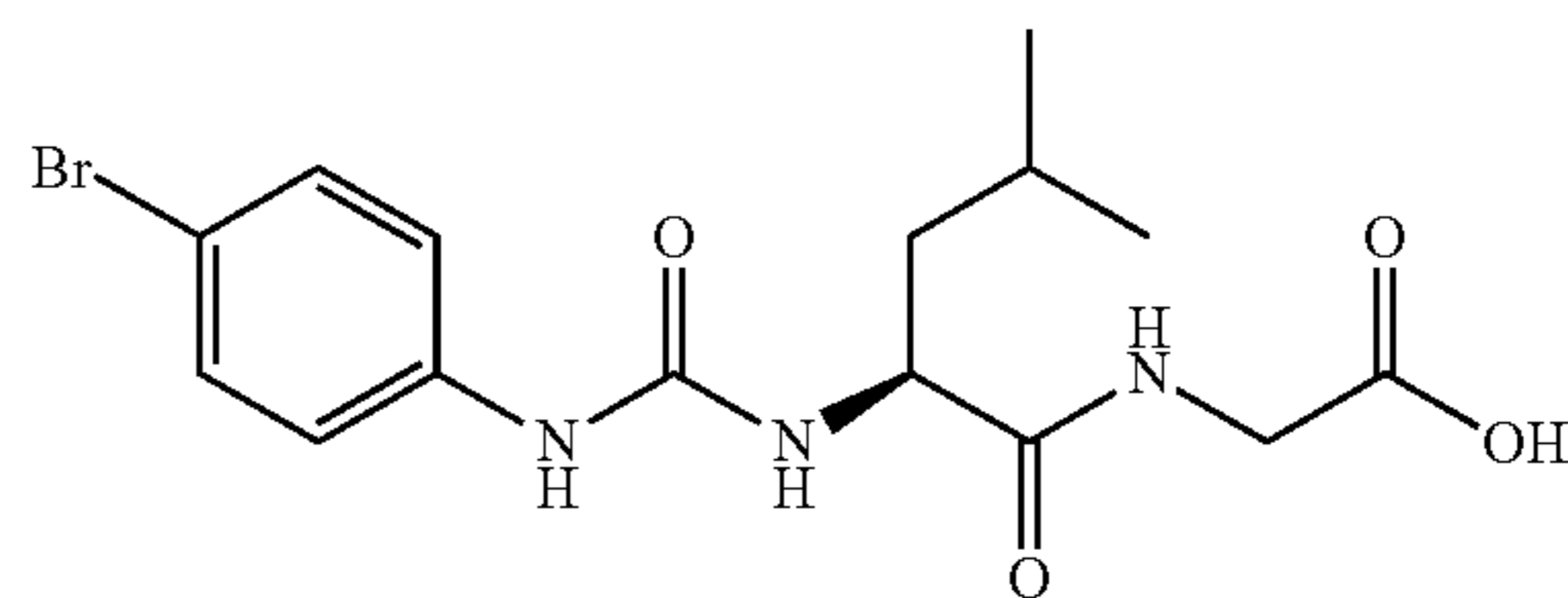
{{(2S)-2-{{(4-bromophenyl)carbamoyl}amino}-4-methylpentanoyl]amino}acetic acid
