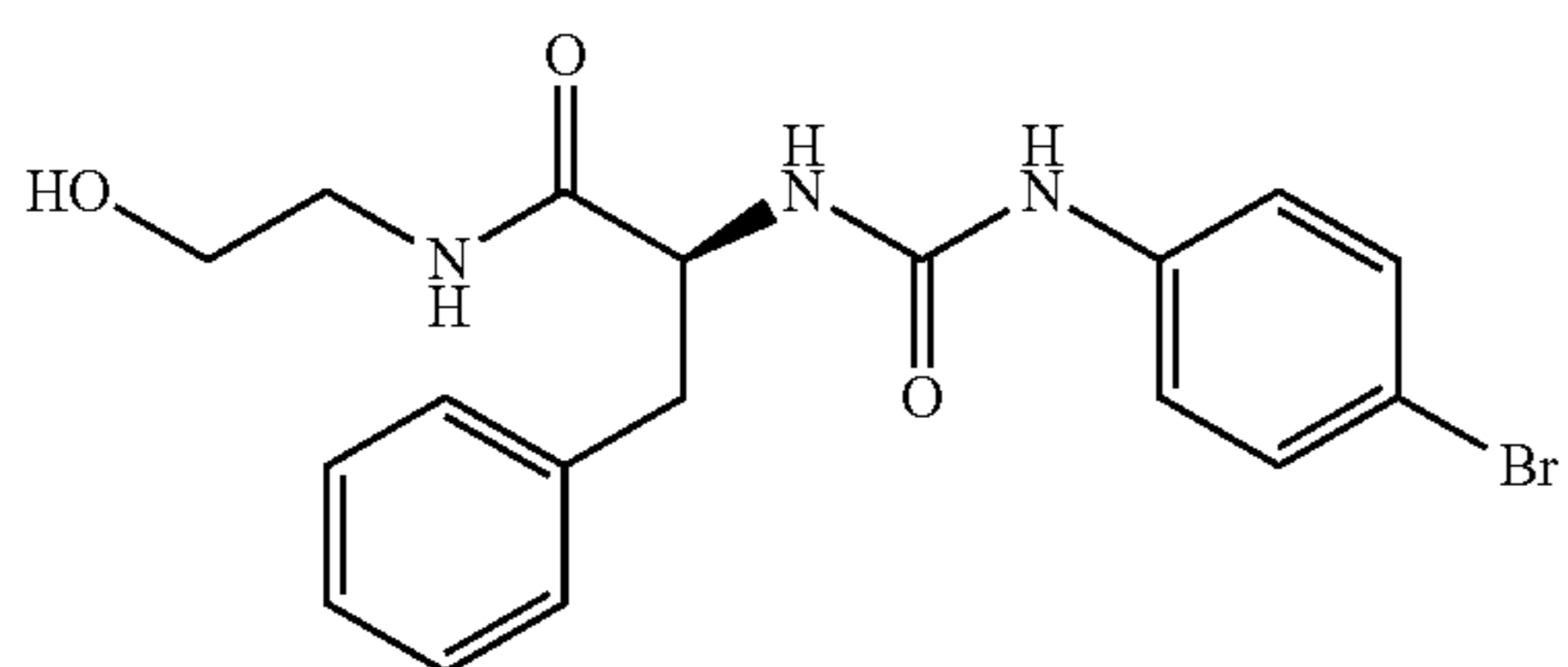
(2S)-2-{{(4-bromophenyl)carbamoyl}amino}-N-(2-hydroxyethyl)-3-phenylpropanamide
