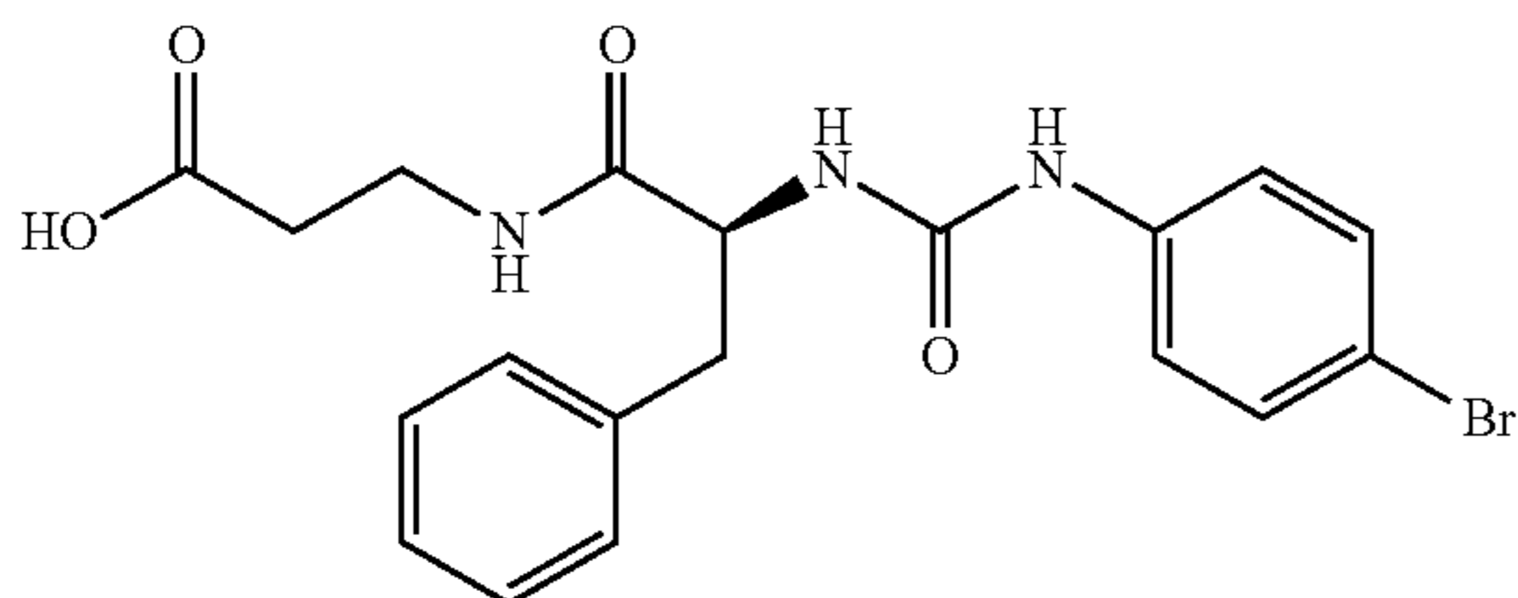
3-{{(2S)-2-{{(4-bromophenyl)carbamoyl}amino}-3-phenylpentanoyl]amino}propanoic acid
