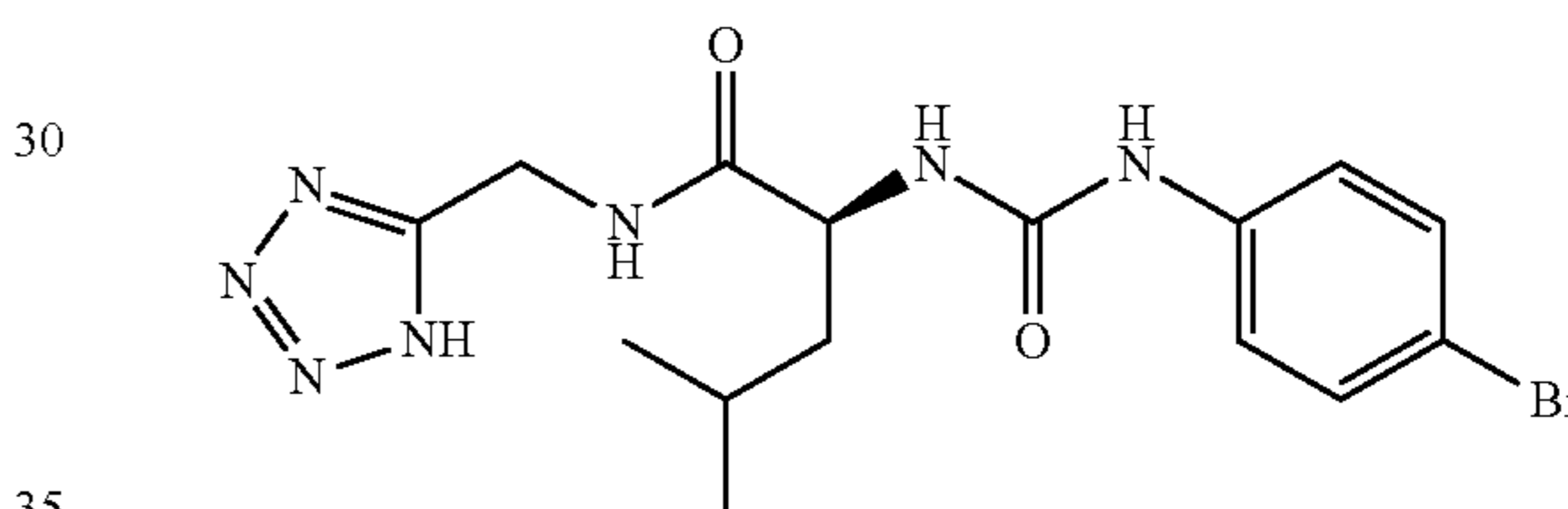
(2S)-2-([(4-bromophenyl)carbamoyl]amino)-4-methyl-N-(1H-tetrazol-5-ylmethyl)pentanamide
