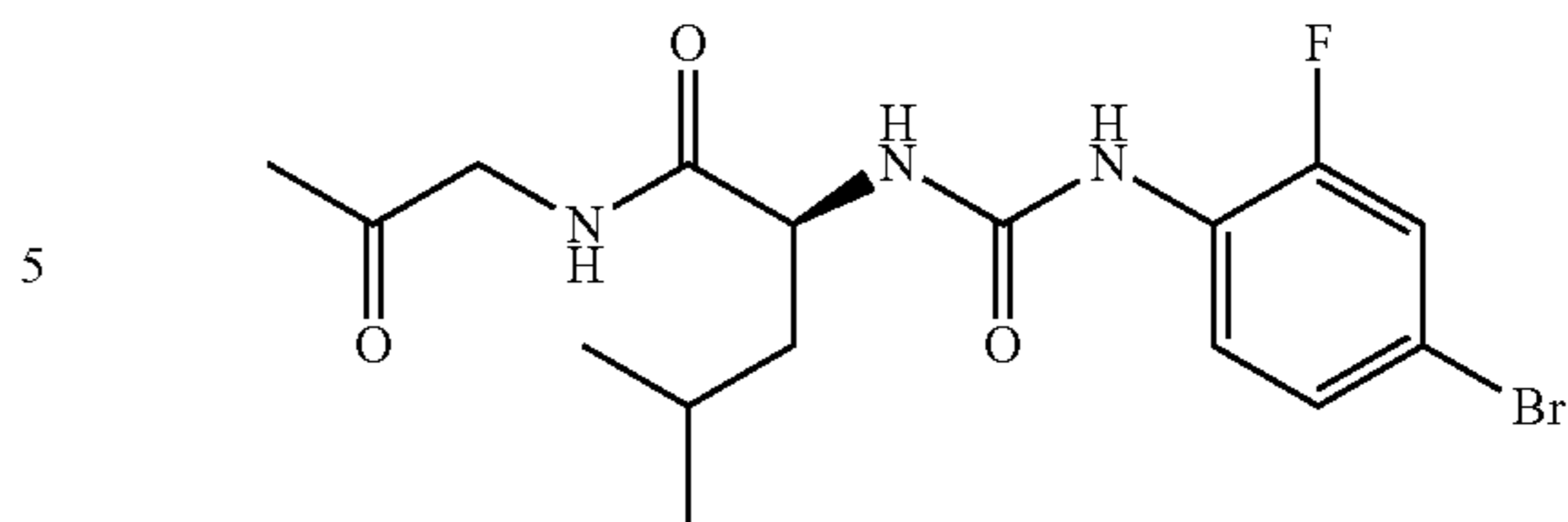
(2S)-2-[[4-bromo-2-fluorophenyl]carbamoyl]amino-N-(2-oxopropyl)pentanamide
