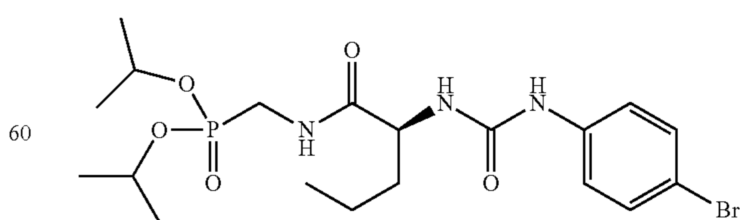
dipropan-2-yl(((2S)-2-((4-bromophenyl)carbamoyl)amino)pentanoyl]amino)methyl phosphonate
