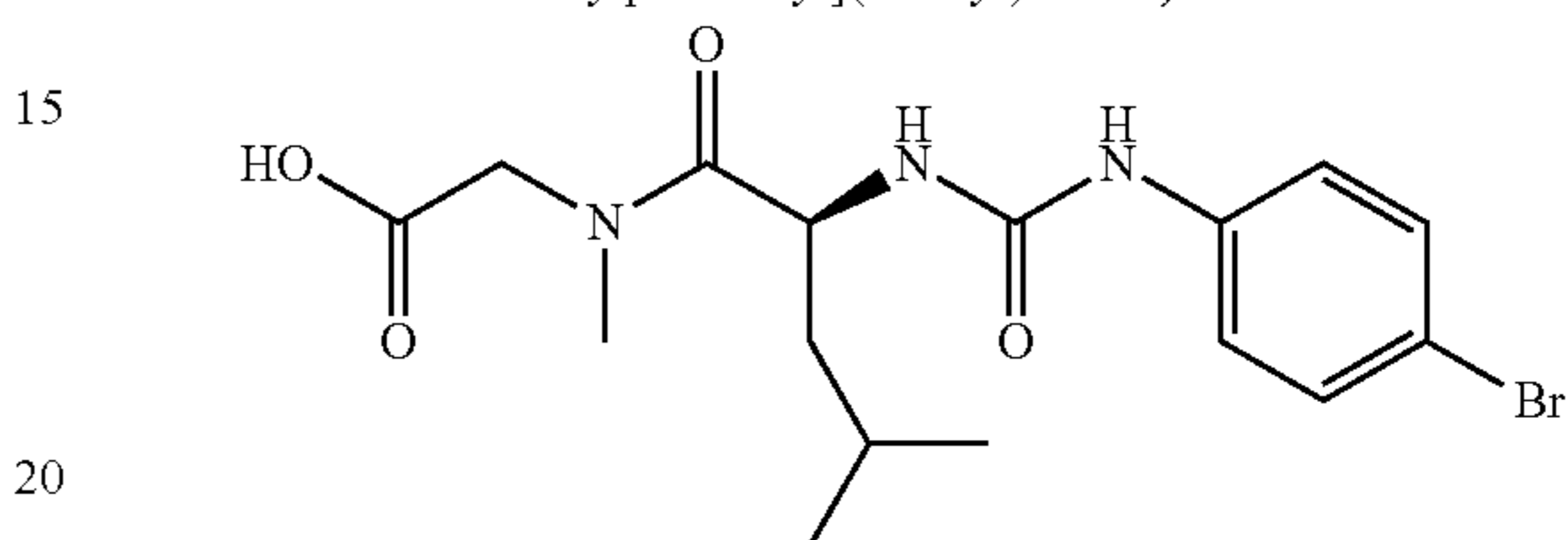
20 25 {[(2S)-2-({[4-bromophenyl]carbamoyl}amino)-4-methylpentanoyl](methyl)amino}acetic acid
