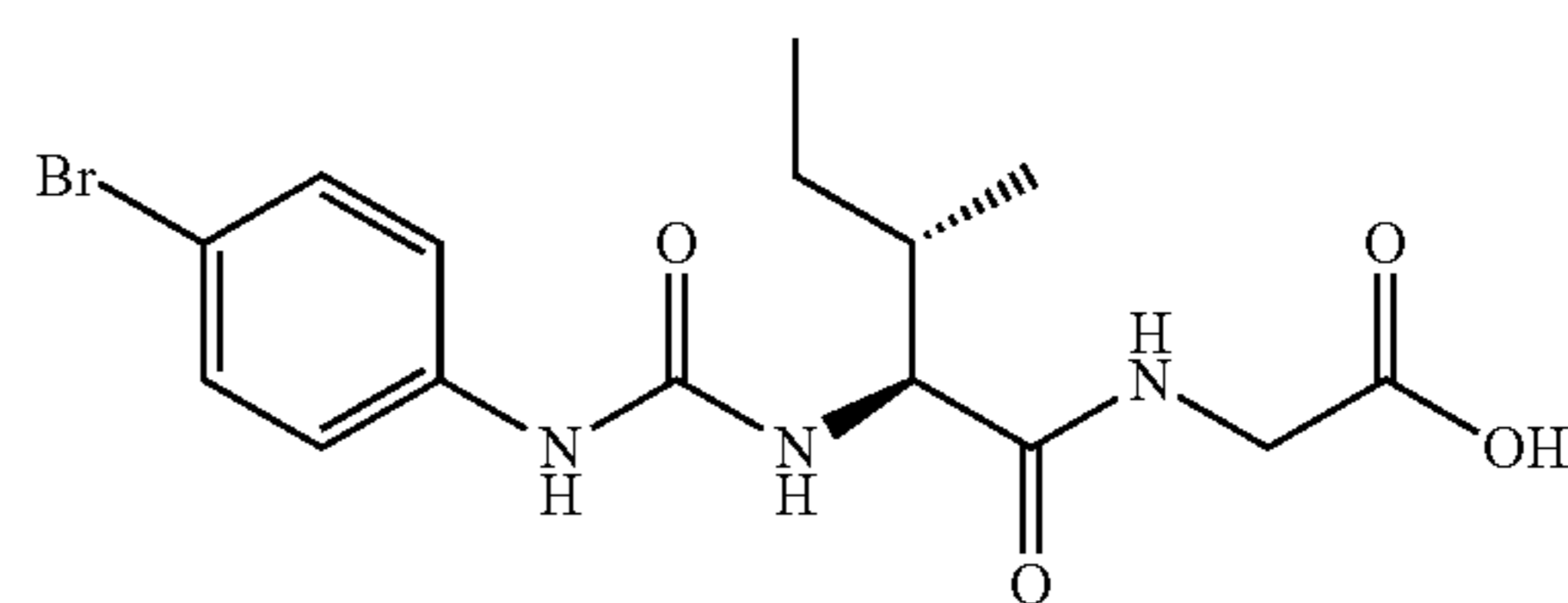
{{(2S,3S)-2-{{(4-bromophenyl)carbamoyl}amino}-3-methylpentanoyl]amino}acetic acid
