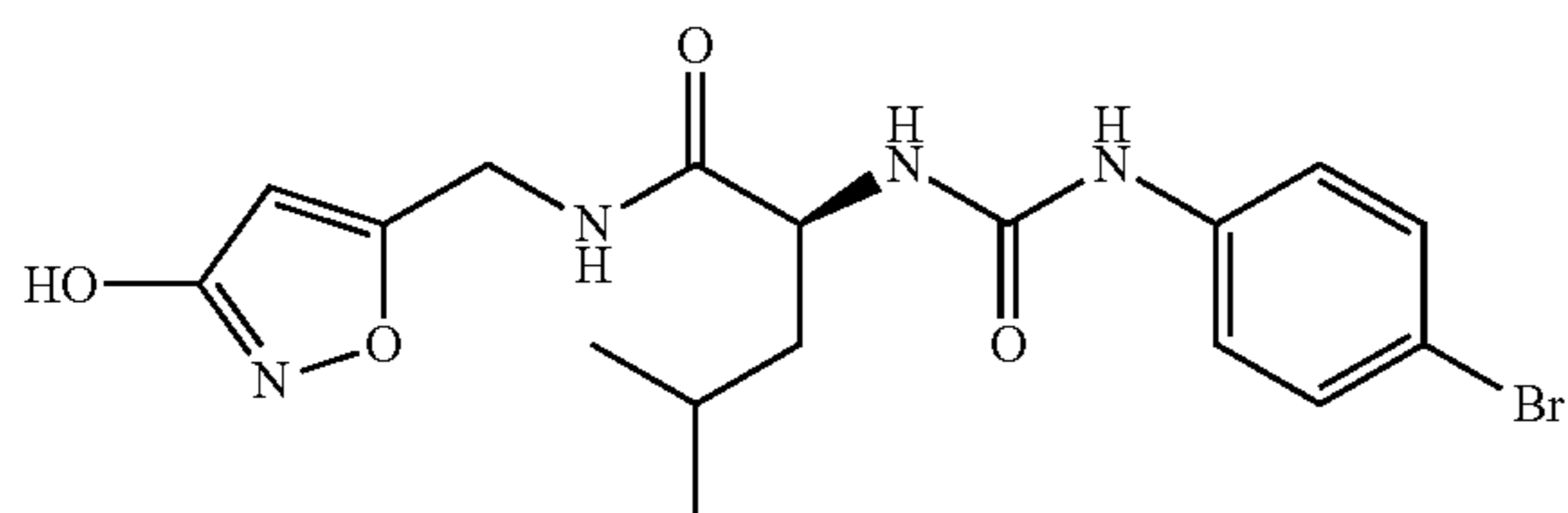
(2S)-2-((4-bromophenyl)carbamoyl)amino)-N-[(3-hydroxy-1,2-oxazol-5-yl)methyl]-4-methylpentanamide
