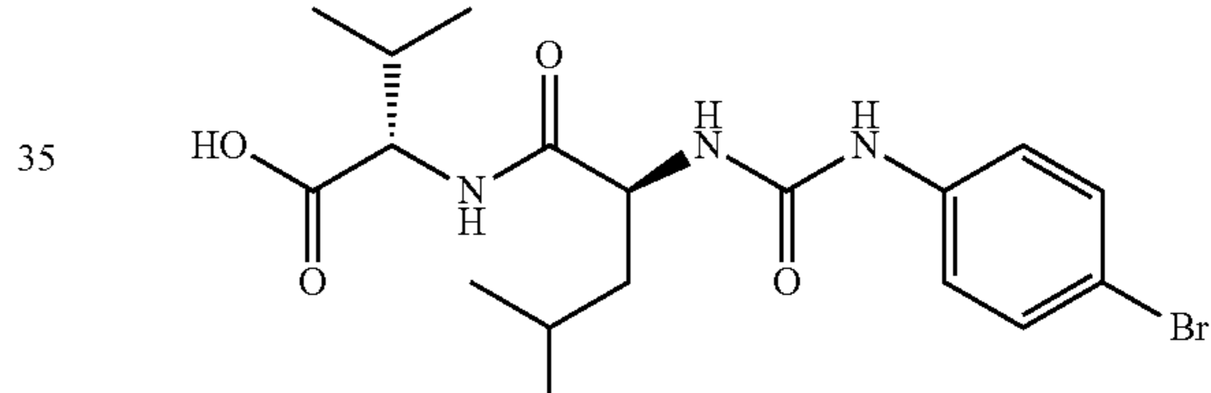
(2S)-2-[[2S)-2-[[4-bromophenyl]carbamoyl]amino]-4-methylpentanoyl]amino}-3-methylbutanoic acid
