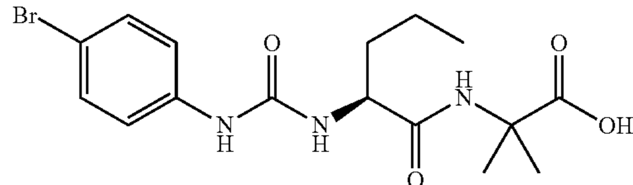
2-{{(2S)-2-{{(4-bromophenyl)carbamoyl}amino}-4-methylpentanoyl]amino}-2-methylpropanoic acid
