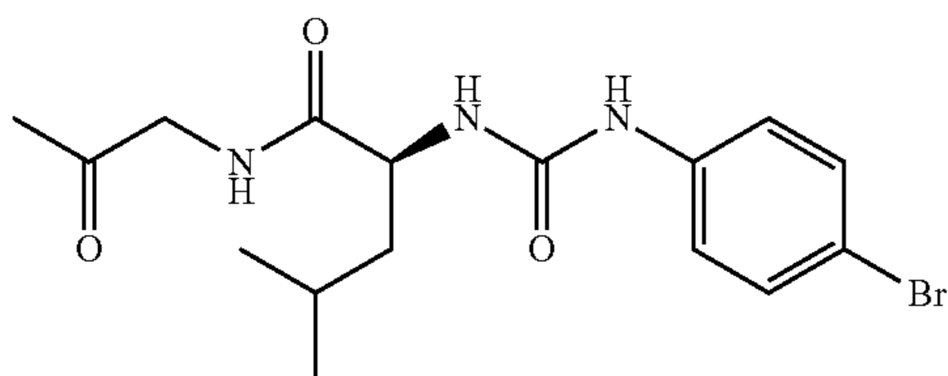
(2S)-2-[[4-bromophenyl]carbamoyl]amino-N-(2-oxopropyl)pentanamide
