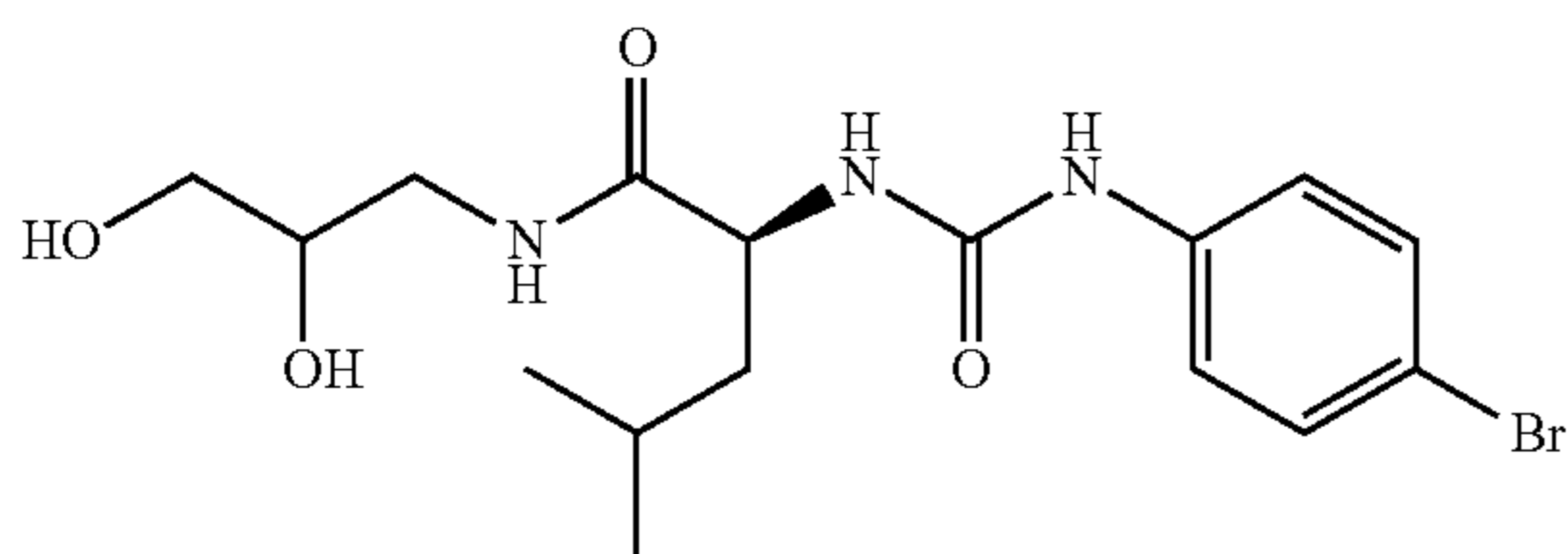
(2S)-2-([(4-bromophenyl)carbamoyl]amino)-N-(2,3-dihydroxypropyl)-4-methylpentanamide
