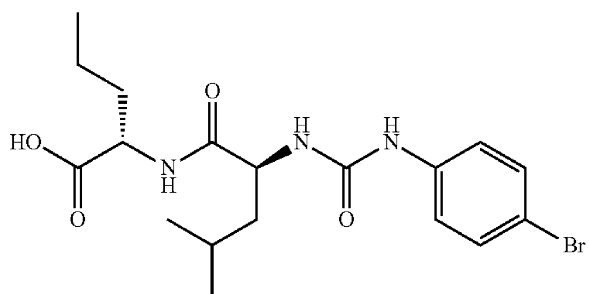
(2S)-2-({[4-bromophenyl]carbamoyl}amino)-4-methylpentanoic acid
