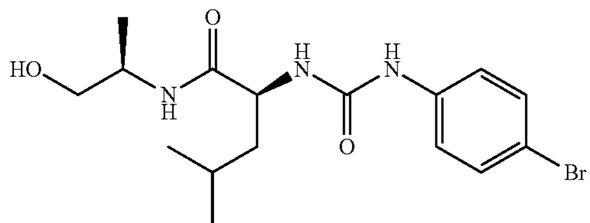
(2S)-2-([(4-bromophenyl)carbamoyl]amino)-N-[(2R)-1-hydroxypropan-2-yl]-4-methylpentanamide
