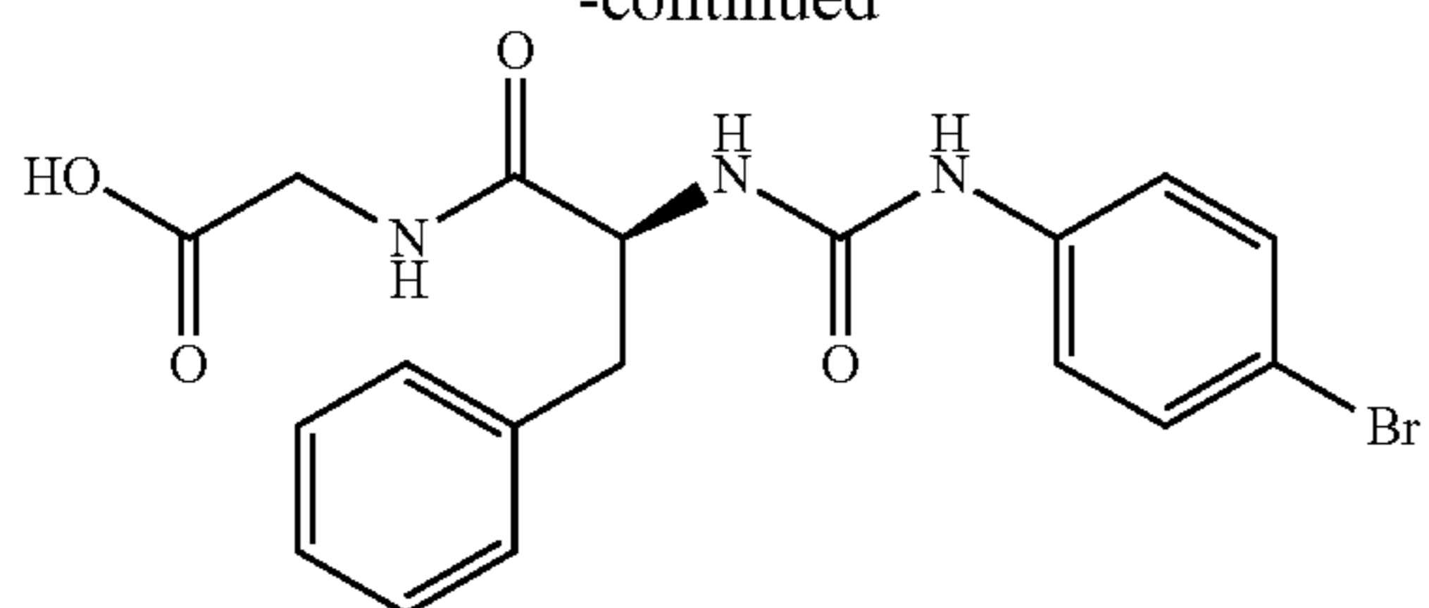
{[(2S)-2-{{(4-bromophenyl)carbamoyl}amino}-3-phenylpentanoyl]amino}acetic acid
