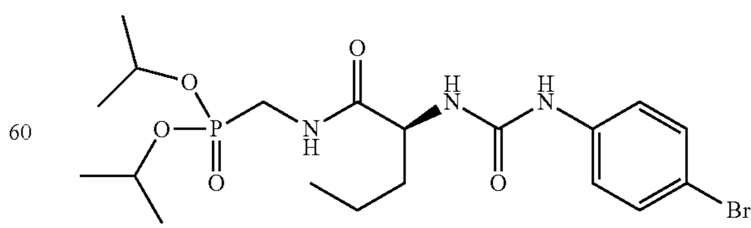
dipropan-2-yl(((2S)-2-((4-bromophenyl)carbamoyl)amino)pentanoyl]amino)methyl phosphonate
