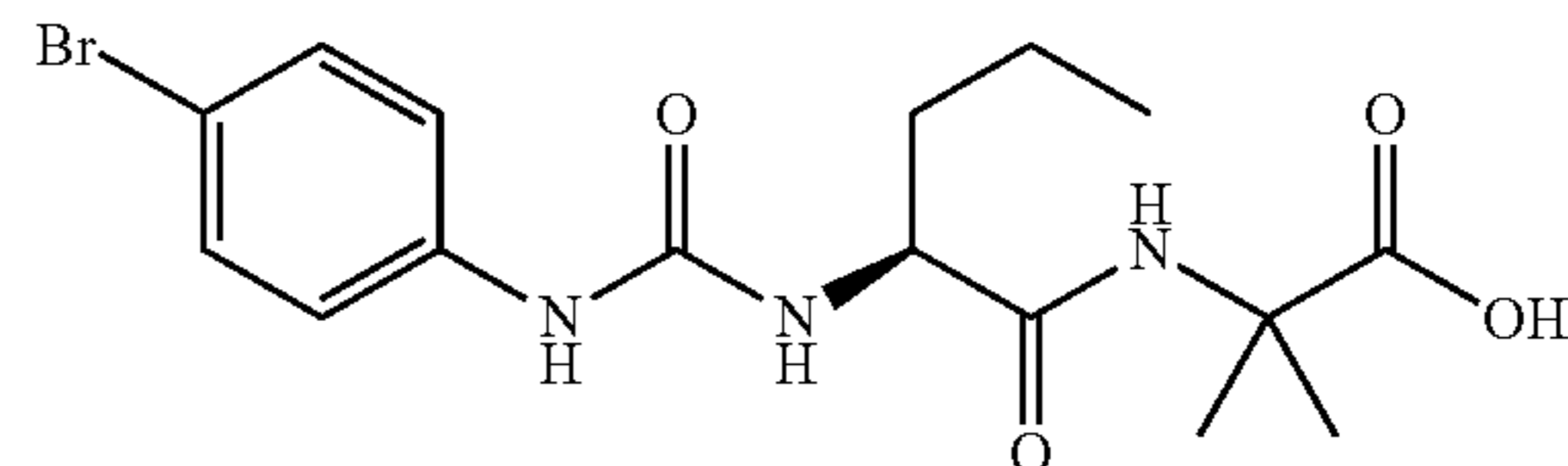
2-{{(2S)-2-{{(4-bromophenyl)carbamoyl}amino}-4-methylpentanoyl]amino}-2-methylpropanoic acid
