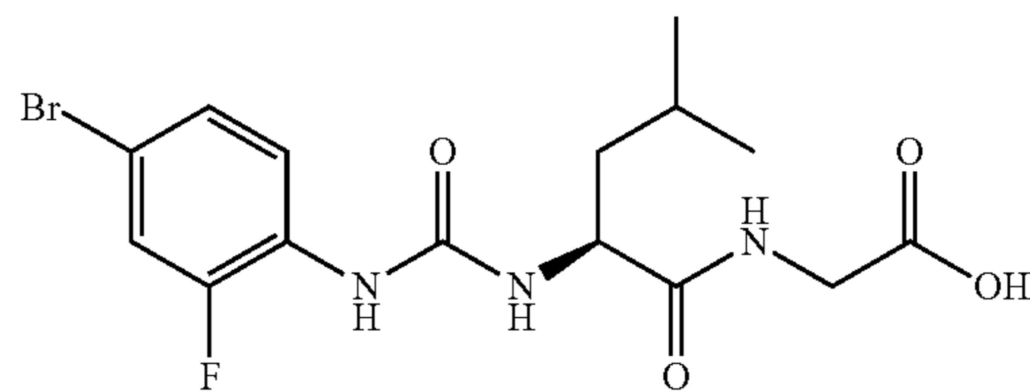
{{(2S)-2-{{(4-bromo-2-fluorophenyl)carbamoyl}amino}-4-methylpentanoyl]amino}acetic acid
