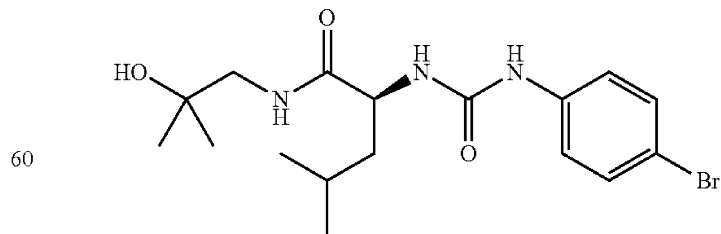
(2S)-2-[[4-bromophenyl]carbamoyl]amino-N-(2-hydroxy-2-methylpropyl)-4-methylpentanamide
