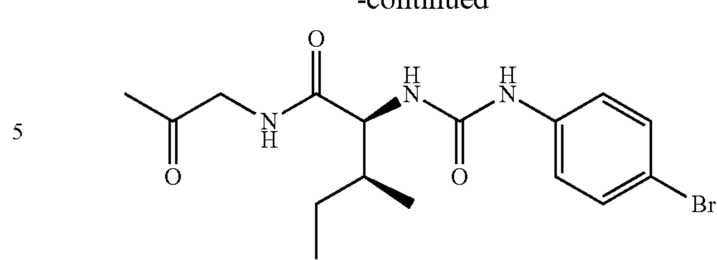
(2S,3S)-2-{{(4-bromophenyl)carbamoyl}amino}-3-methyl-N-(2-oxopropyl)pentanamide
