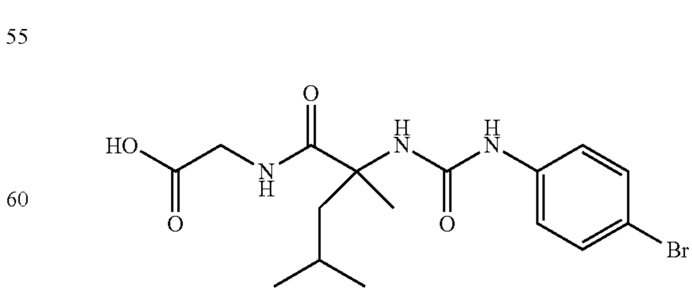
[(2-([(4-bromophenyl)carbamoyl]amino)-2,4-dimethylpentanoyl]amino)acetic acid
