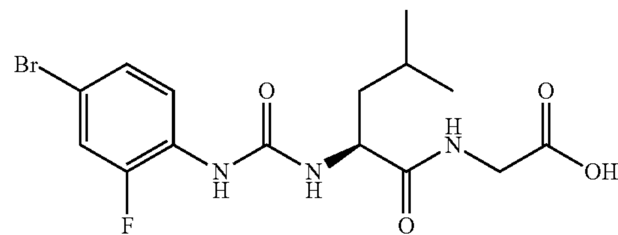
{{(2S)-2-{{(4-bromo-2-fluorophenyl)carbamoyl}amino}-4-methylpentanoyl]amino}acetic acid
