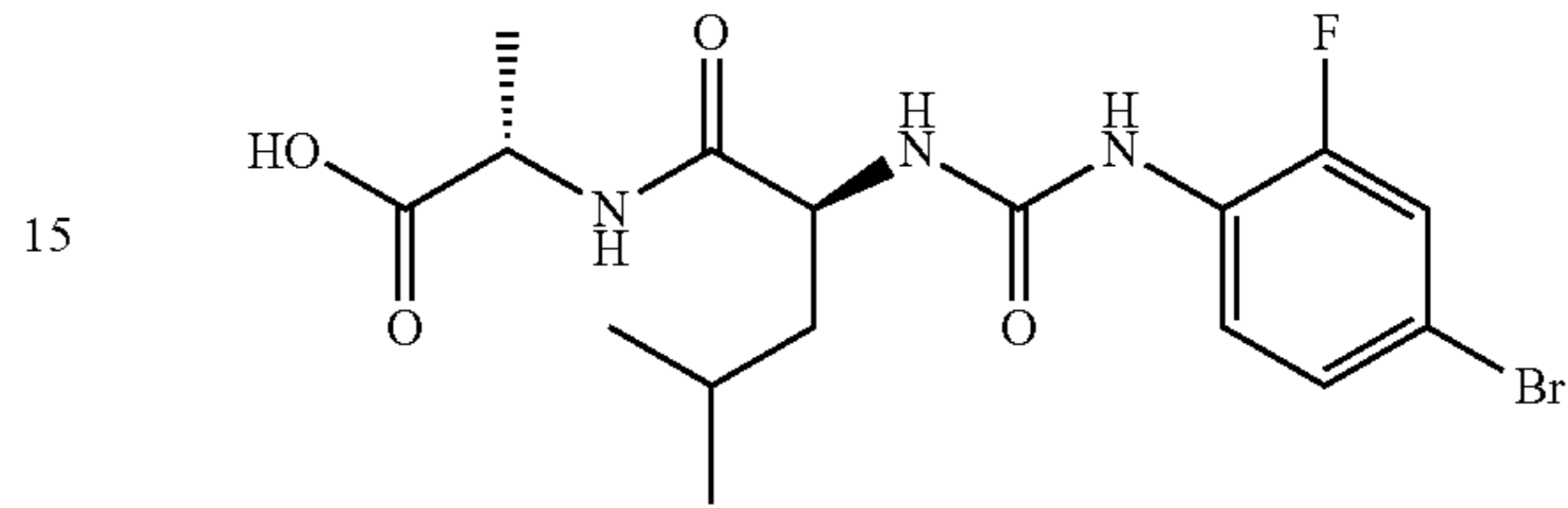
(2S)-2-[[2S)-2-[[4-bromo-2-fluorophenyl]carbamoyl]amino]-4-methylpentanoyl]amino}propanoic acid
