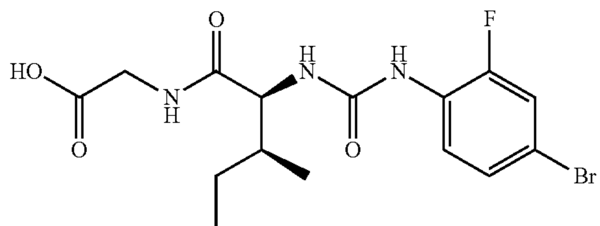
{{(2S,3S)-2-{{(4-bromo-2-fluorophenyl)carbamoyl}amino}-3-methylpentanoyl]amino}acetic acid
