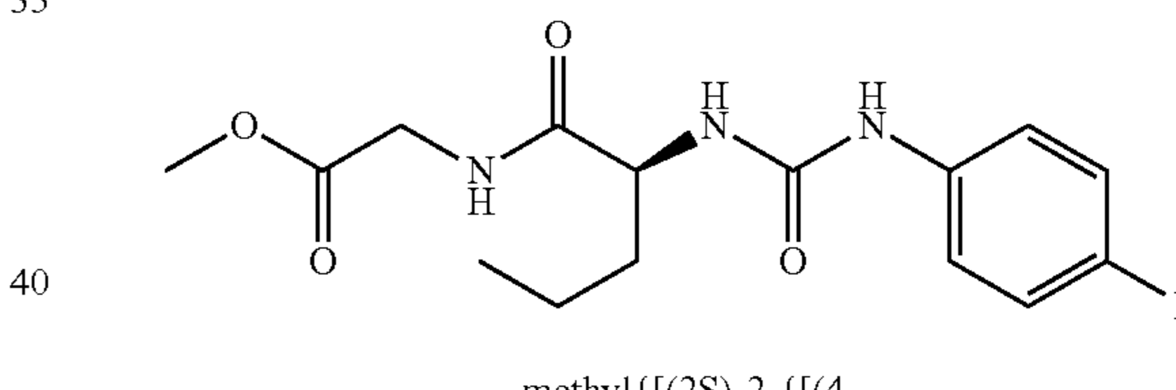
methyl{{(2S)-2-{{(4-bromophenyl)carbamoyl}amino}pentanoyl amino}acetate
