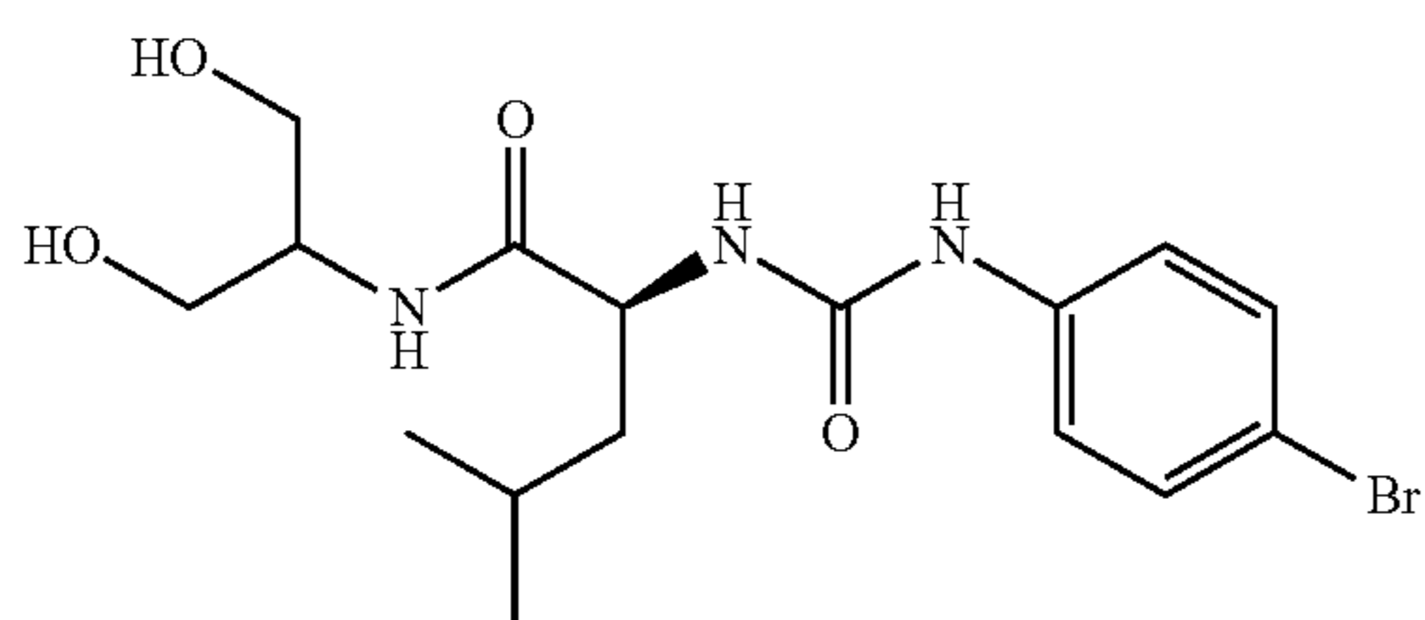
(2S)-2-([(4-bromophenyl)carbamoyl]amino)-N-(1,3-dihydroxypropan-2-yl)-4-methylpentanamide
