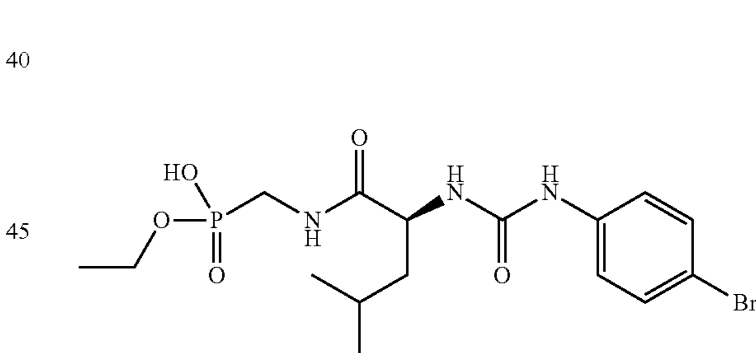
ethyl hydrogen (([(2S)-2-([(4-bromophenyl)carbamoyl]amino)-4-methylpentanoyl]amino)methyl)phosphonate
