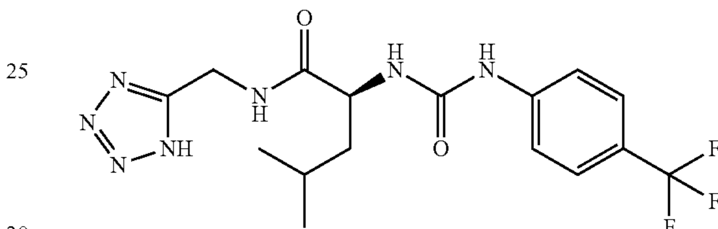
(2S)-4-methyl-N-(1H-tetrazol-5-ylmethyl)-2-{{(4-(trifluoromethyl)phenyl}carbamoyl}amino)pentanamide
