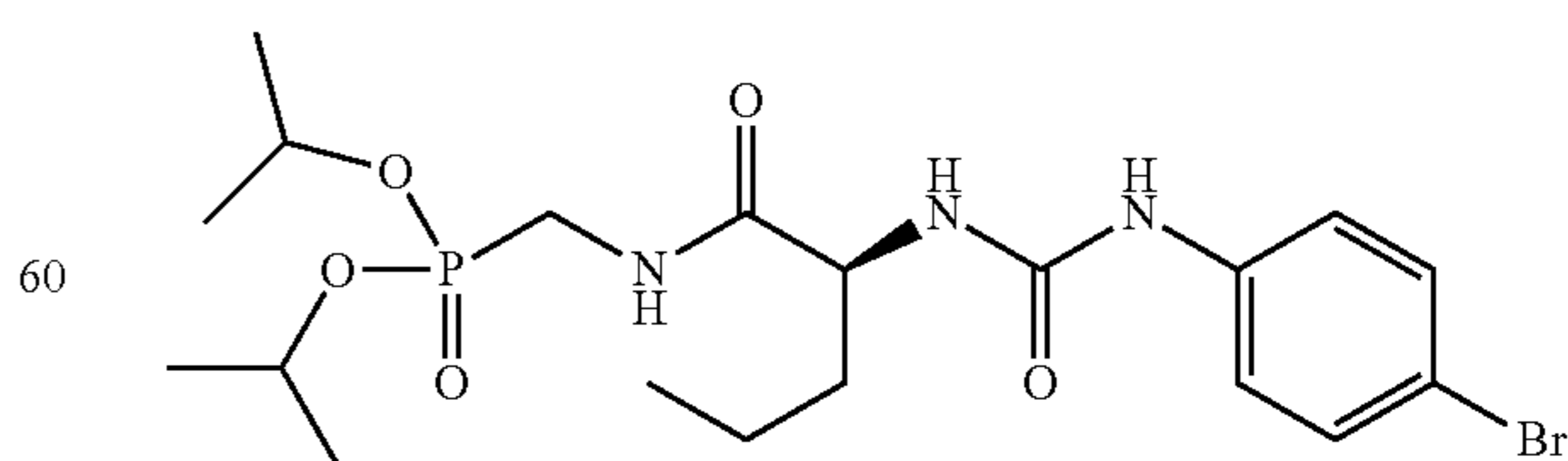
dipropan-2-yl(((2S)-2-((4-bromophenyl)carbamoyl)amino)pentanoyl]amino)methyl phosphonate
