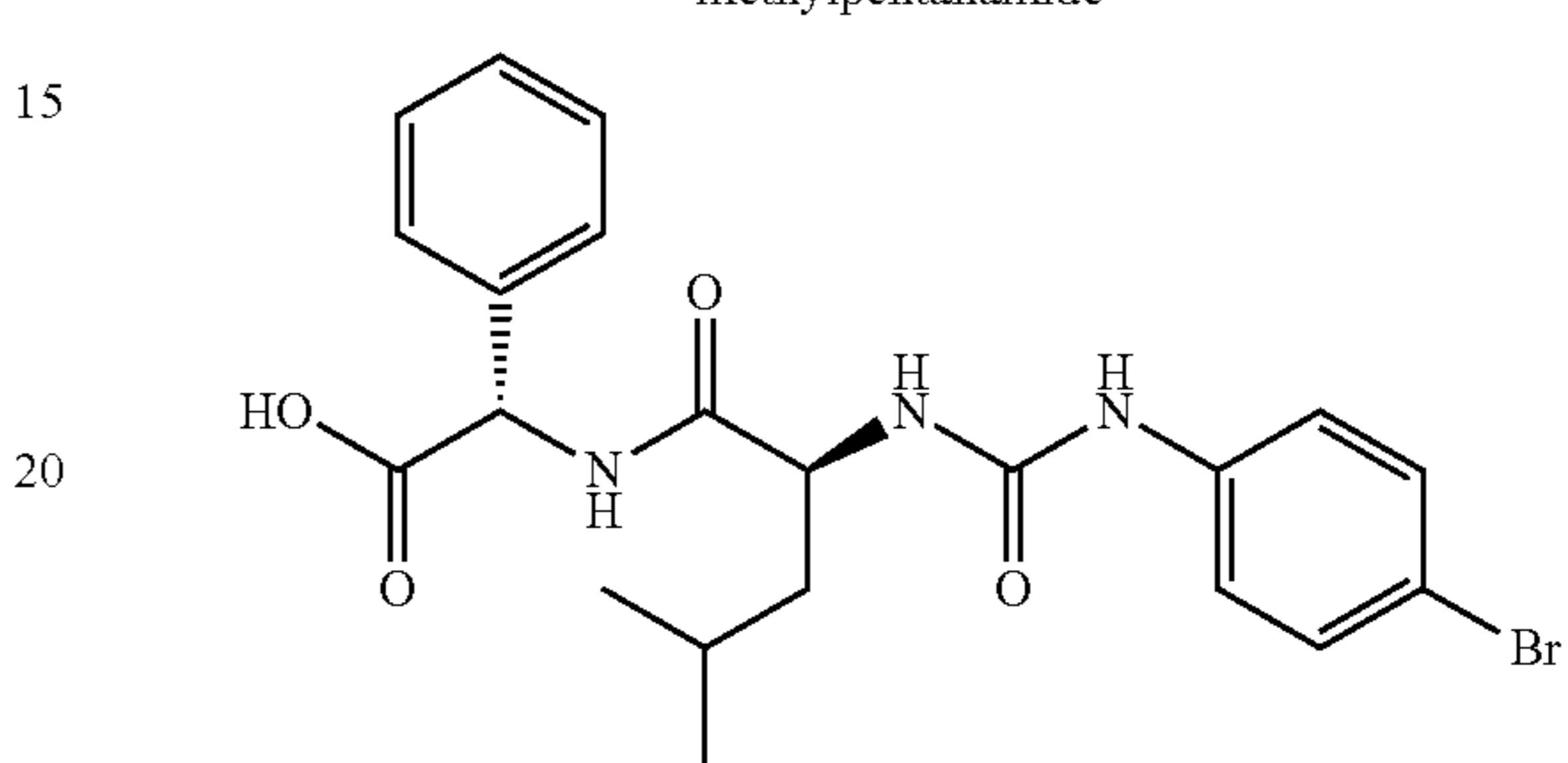
(2S)-({[4-bromophenyl]carbamoyl}amino)-4-methylpentanoyl(phenyl)ethanoic acid
