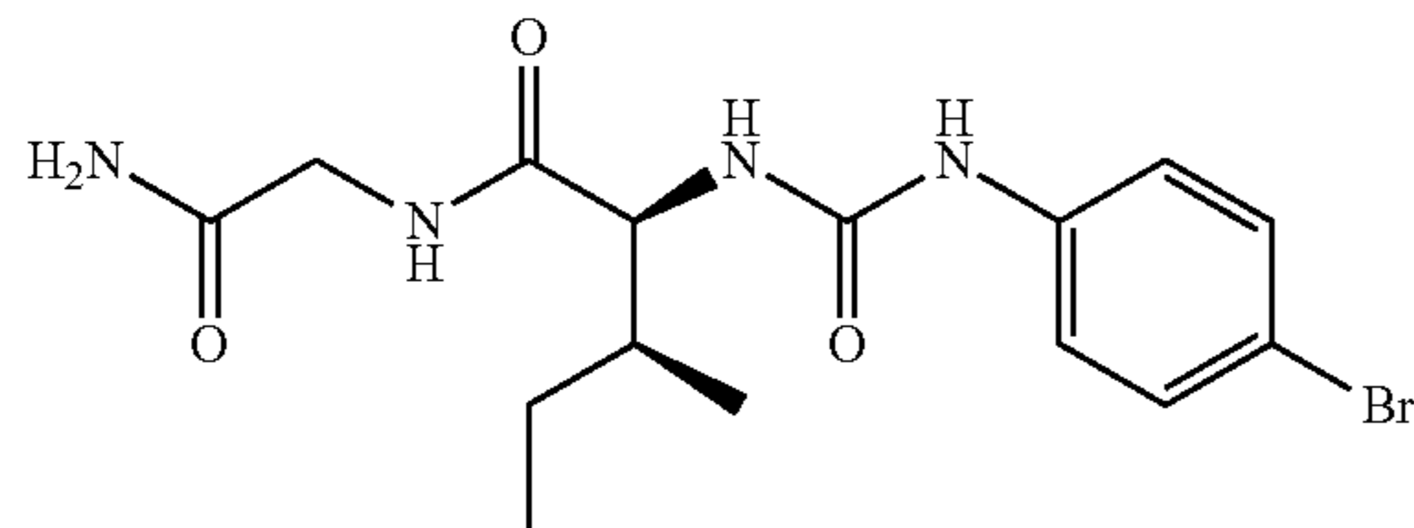
(2S,3S)-N-(2-amino-2-oxoethyl)-2-{{(4-bromophenyl)carbamoyl}amino}-3-methylpentanamide
