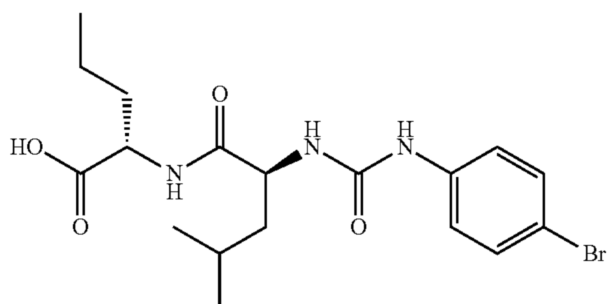
(2S)-2-([(2S)-2-([(4-bromophenyl)carbamoyl]amino)-4-methylpentanoyl]amino)pentanoic acid
