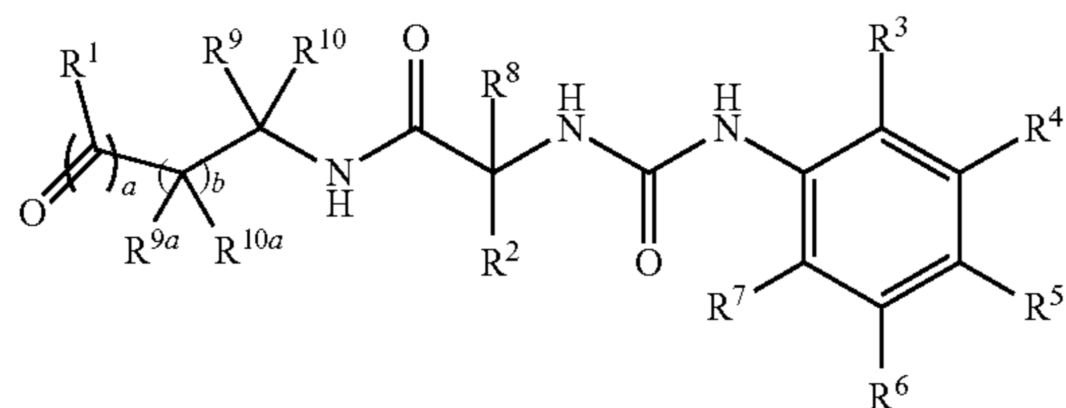
Formula II
