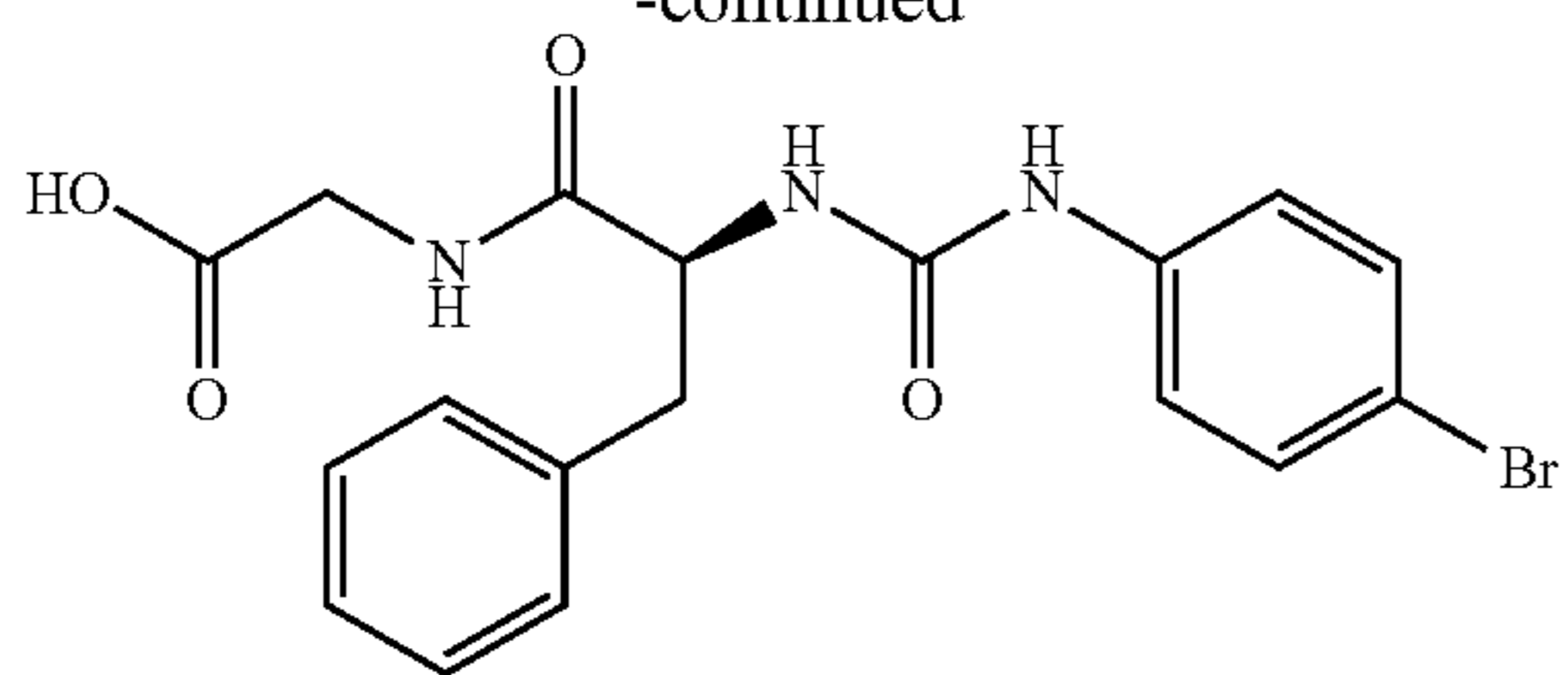
{[(2S)-2-{{(4-bromophenyl)carbamoyl}amino}-3-phenylpentanoyl]amino}acetic acid
