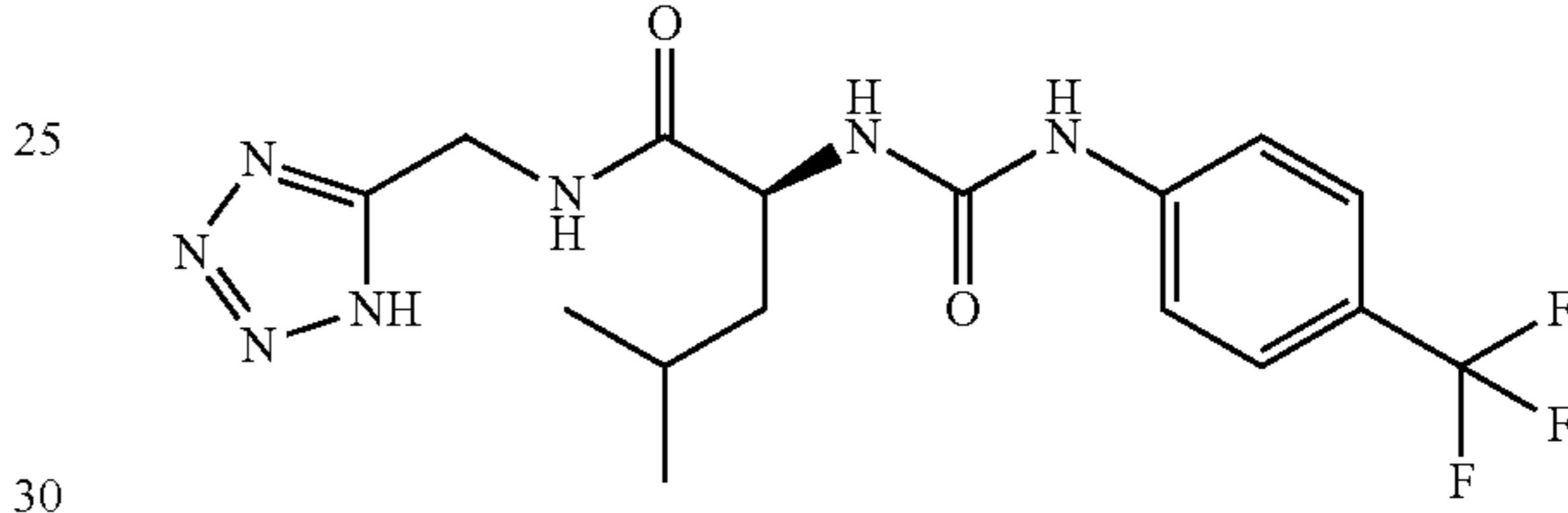
25 (2S)-4-methyl-N-(1H-tetrazol-5-ylmethyl)-2-((4-(trifluoromethyl)phenyl)carbamoyl)amino-5-pentanamide
