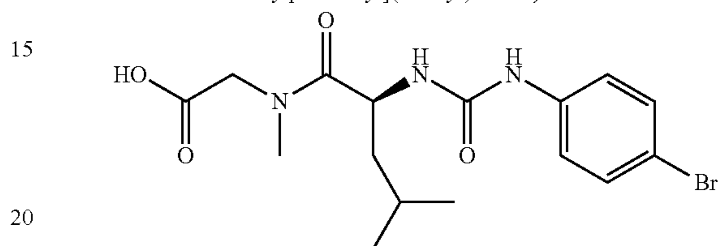
{[(2S)-2-({[4-bromophenyl]carbamoyl}amino)-4-methylpentanoyl](methyl)amino}acetic acid
