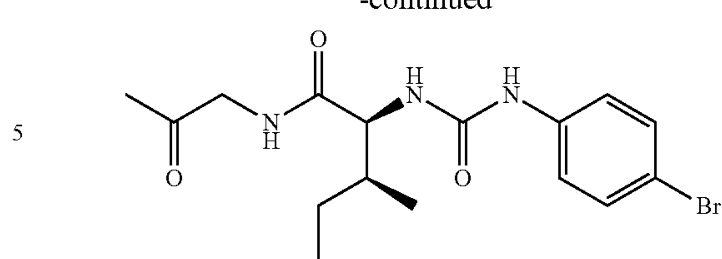
(2S,3S)-2-{{(4-bromophenyl)carbamoyl}amino}-3-methyl-N-(2-oxopropyl)pentanamide
