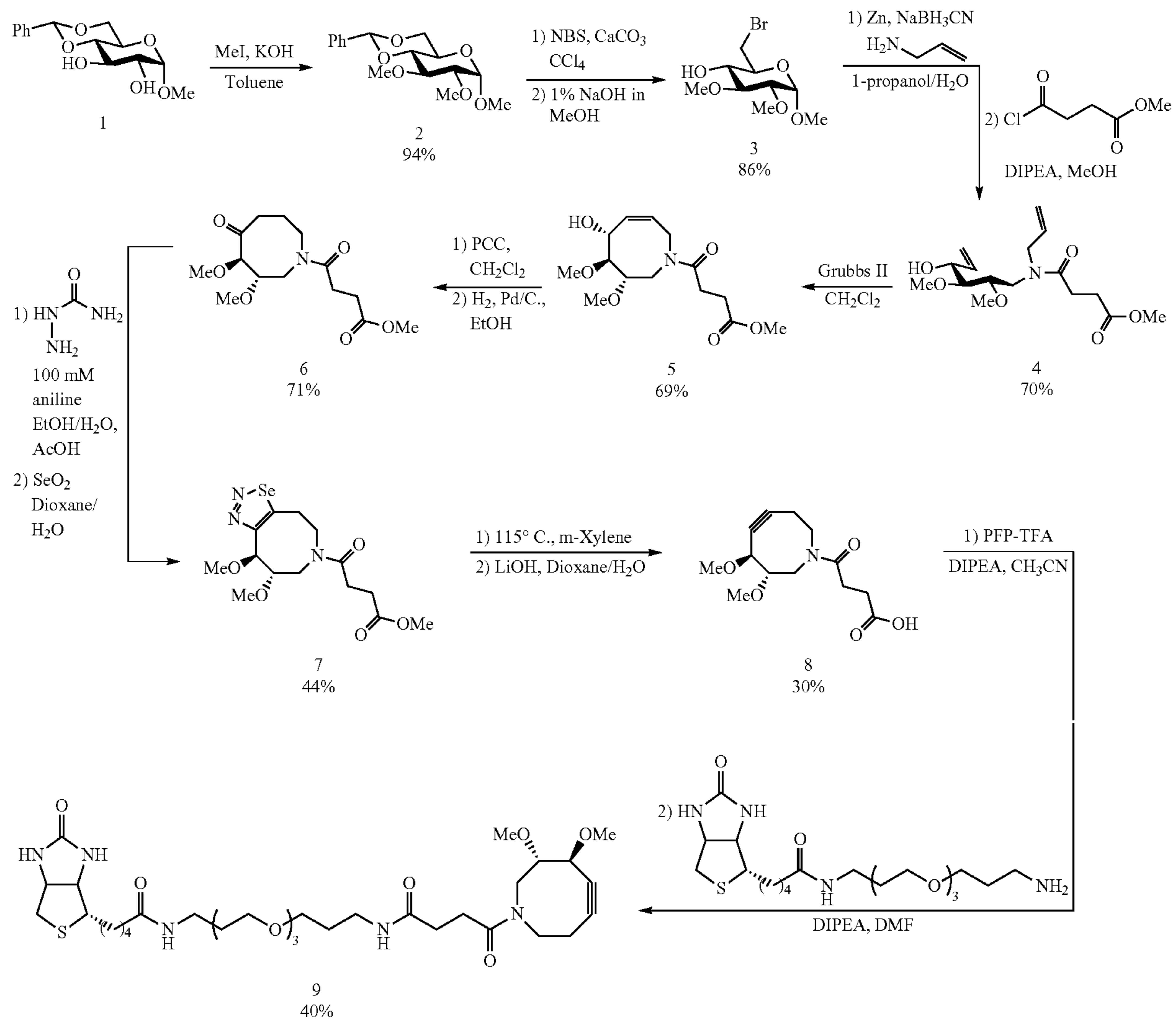
Scheme 3
