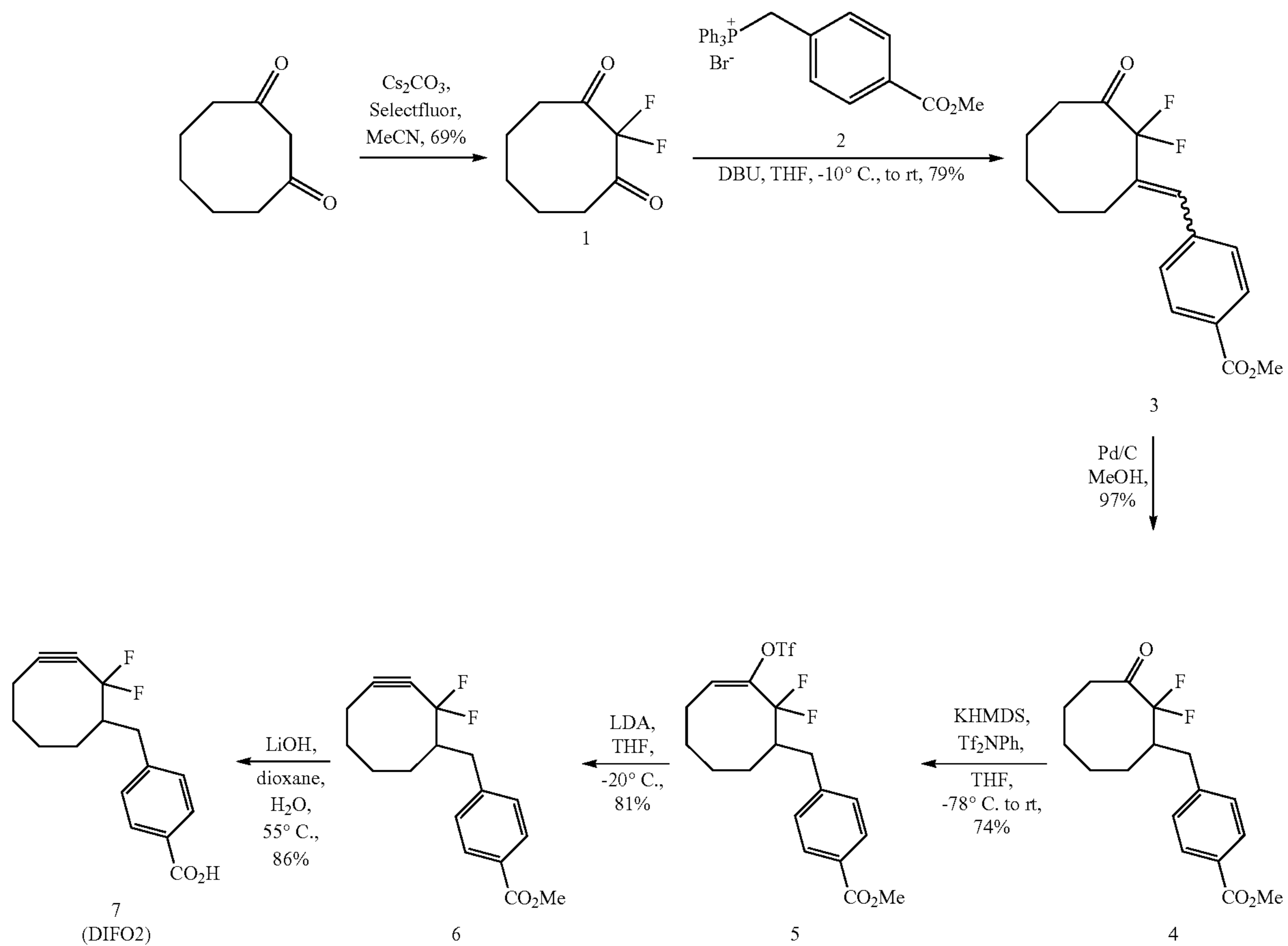
Scheme 8. Synthesis of DIFO2 (7).
