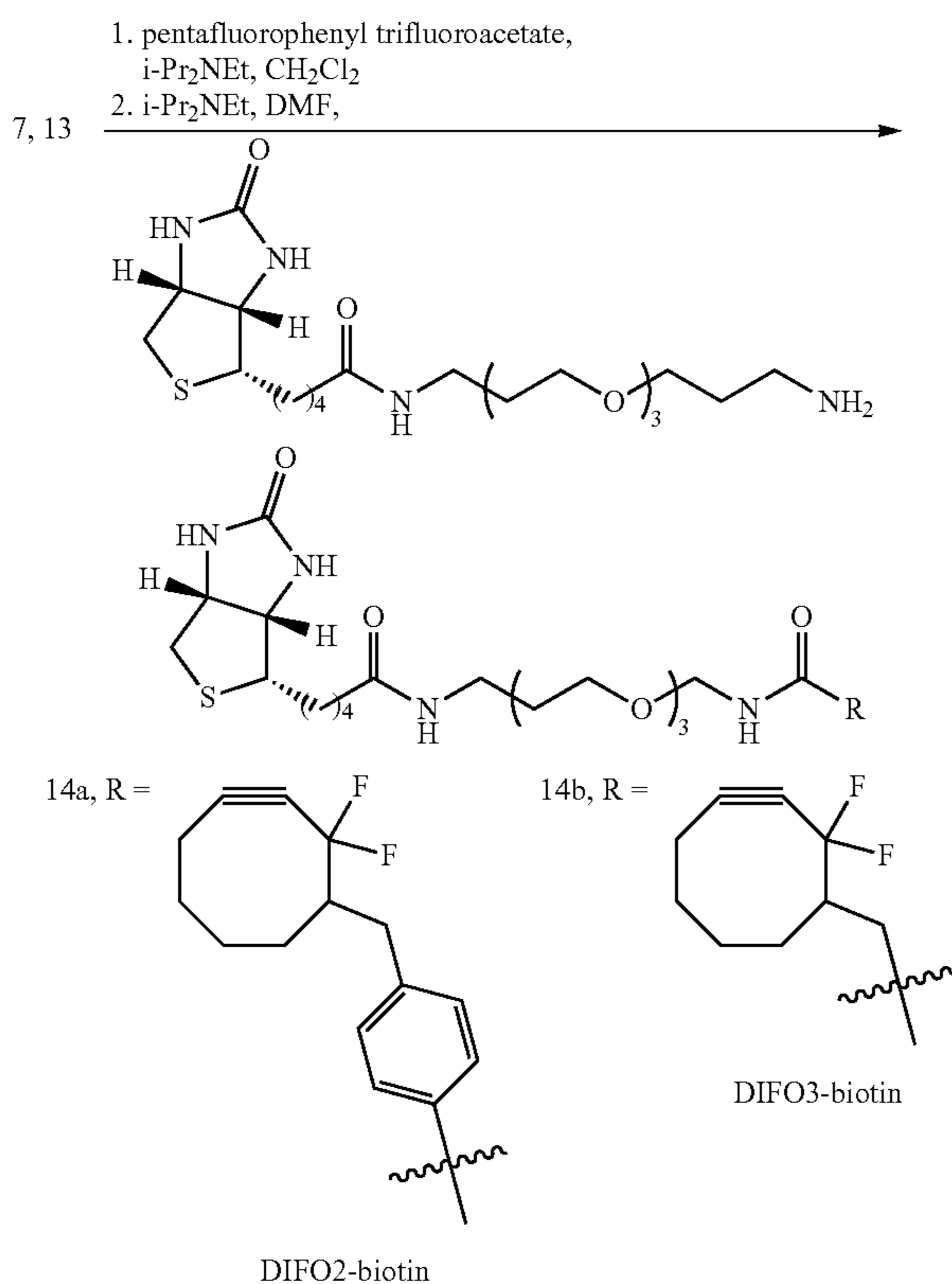
Scheme 10. Synthesis of biotin conjugates of DIFO2 and DIFO3.
