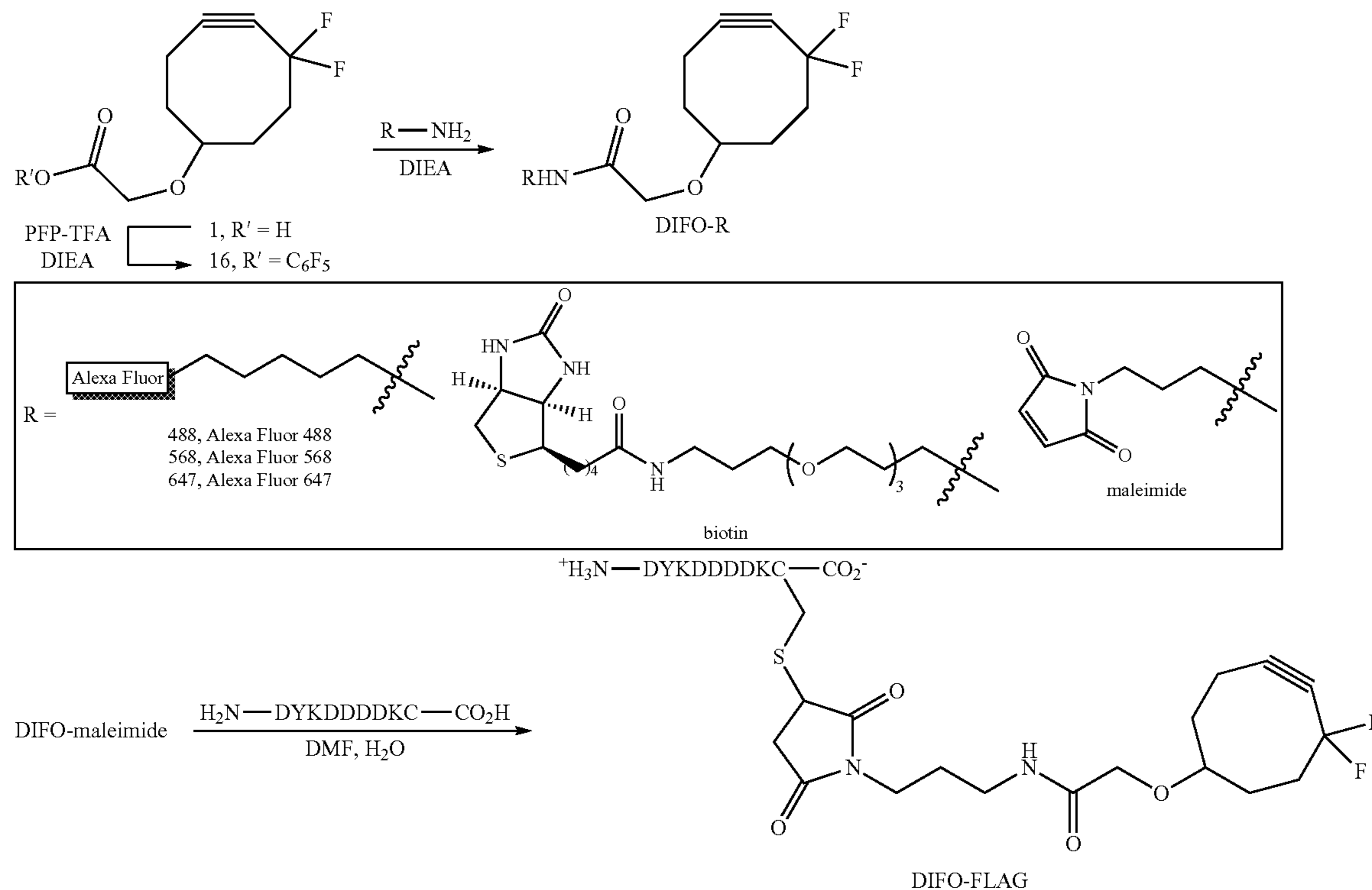
Scheme 7. Synthesis of conjugates of DIFO (biotin, Alexa Fluor 488, 568, and 647, and FLAG peptide)
