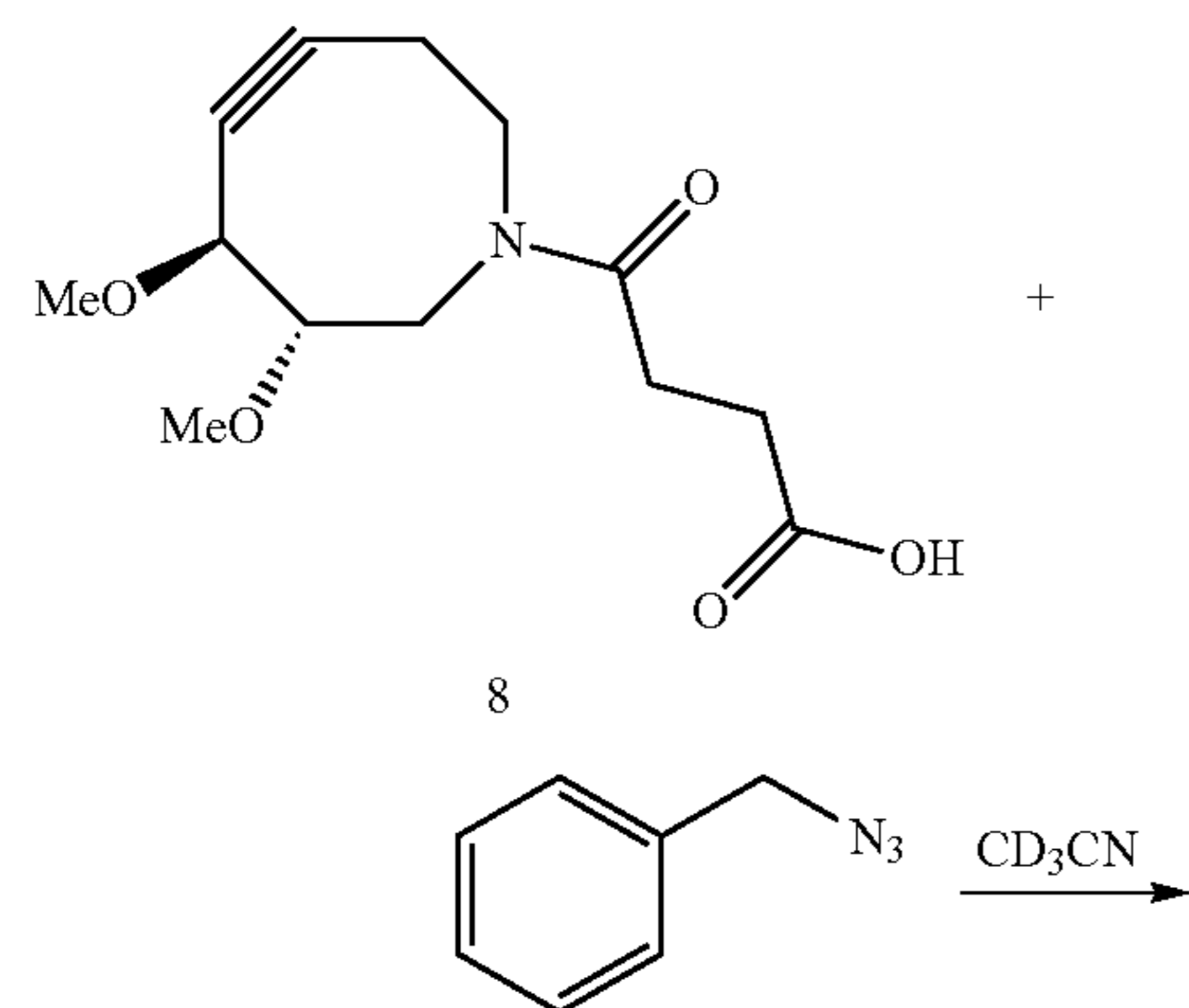
Scheme 4
