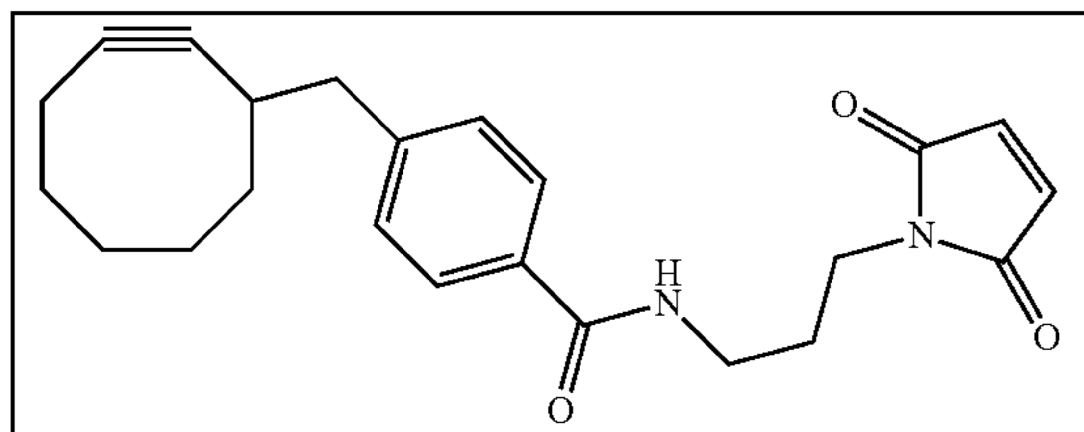
Compound 12a
