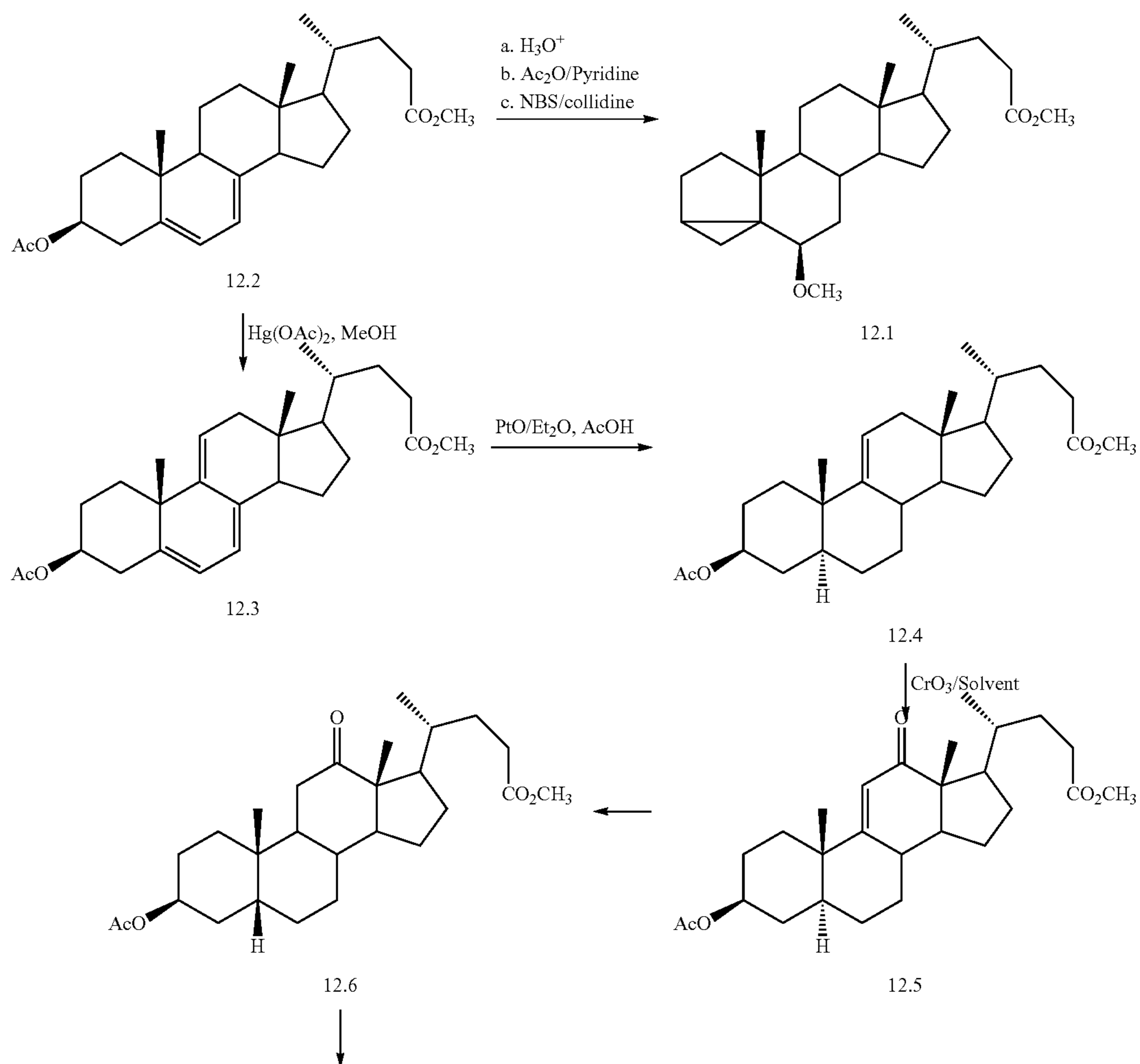
Scheme 12. Triene formation and allylic oxidation
