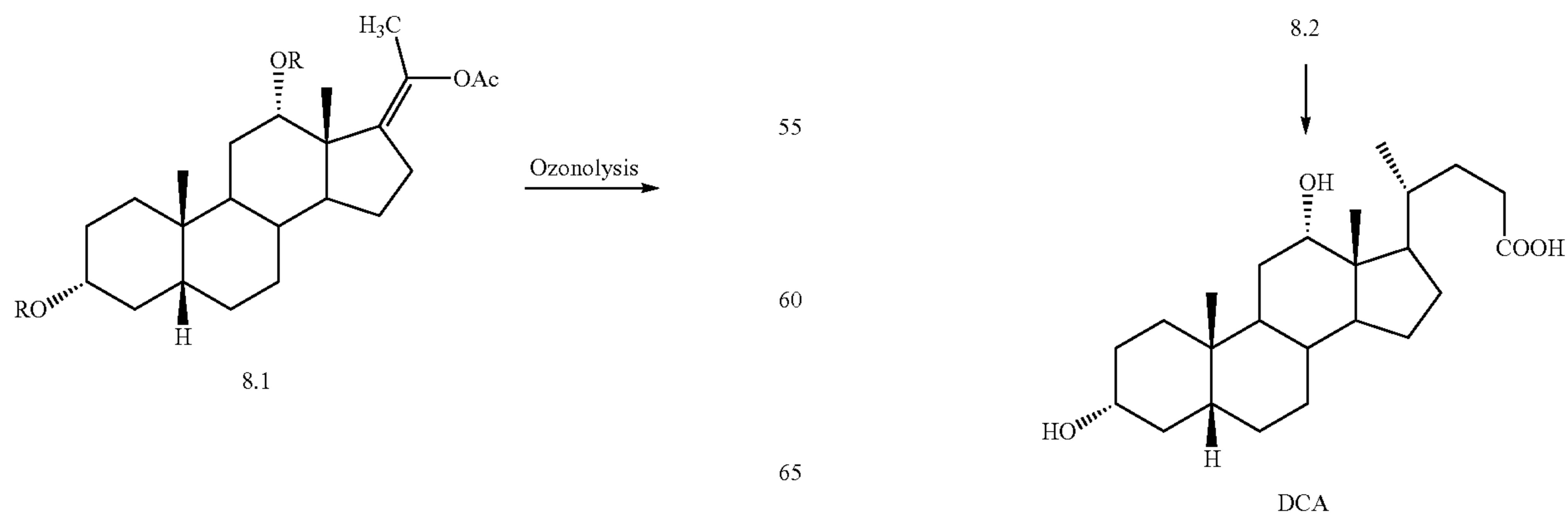
Scheme 8. Side-chain introduction
