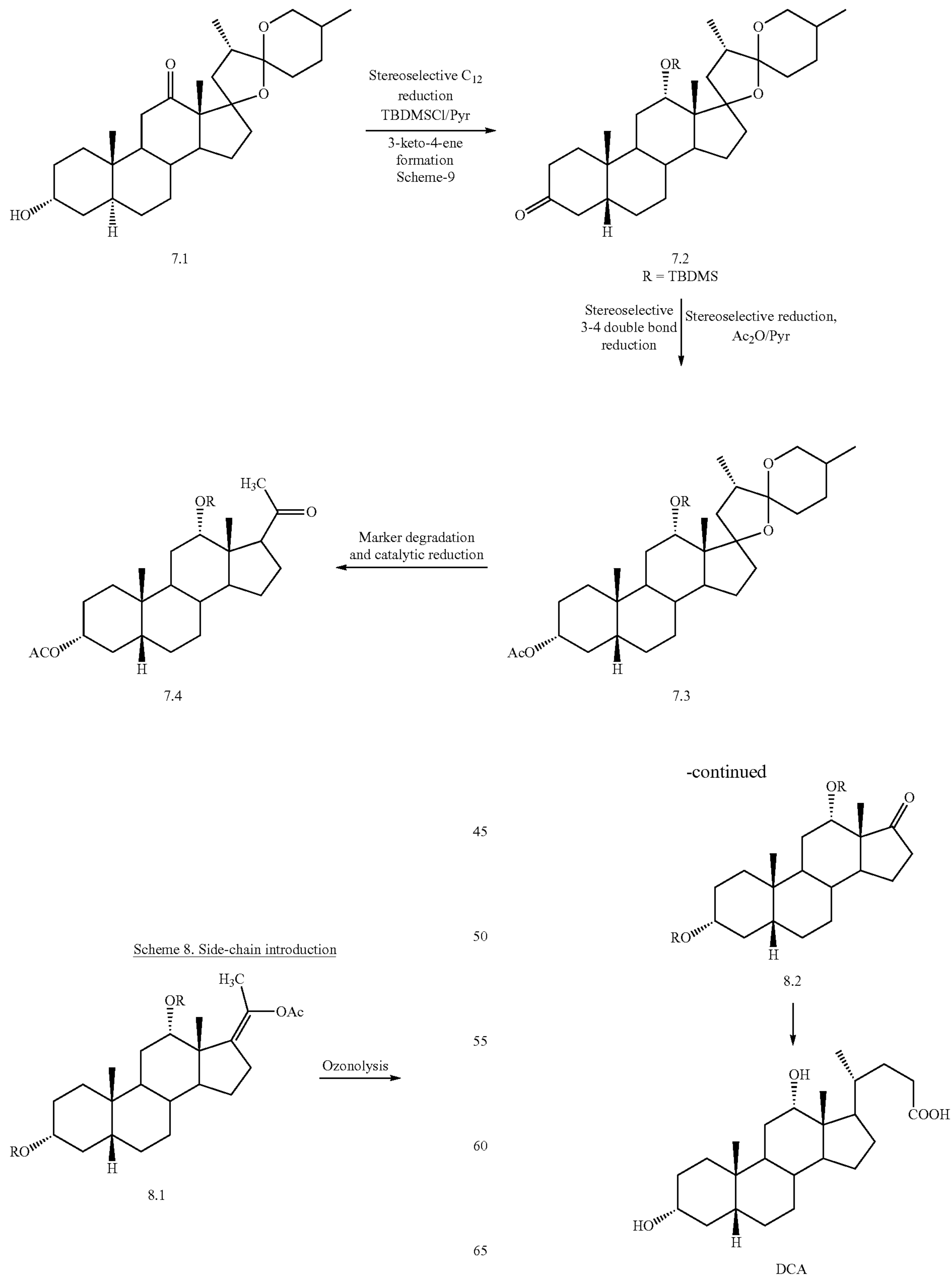
Scheme 7. C 12 -hydroxyl group introduction, AB ring modification and side chain cleavage
