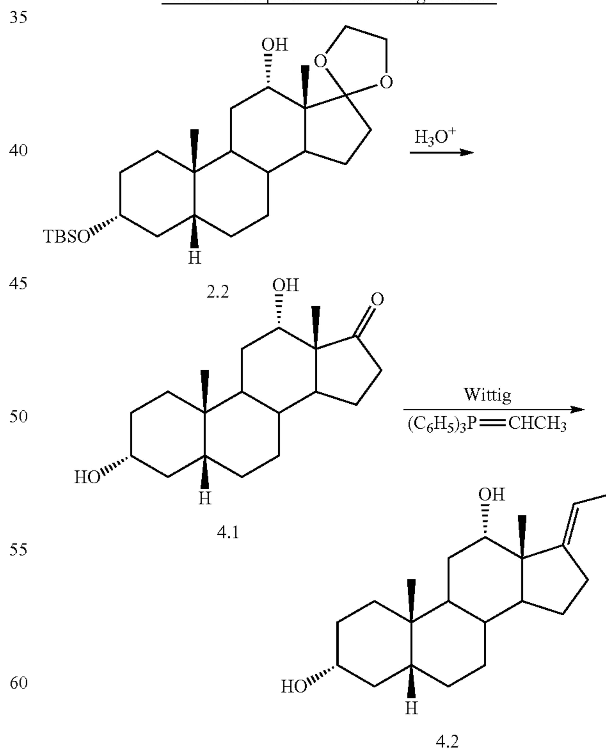
Scheme 4. Deprotection and Wittig Reaction
