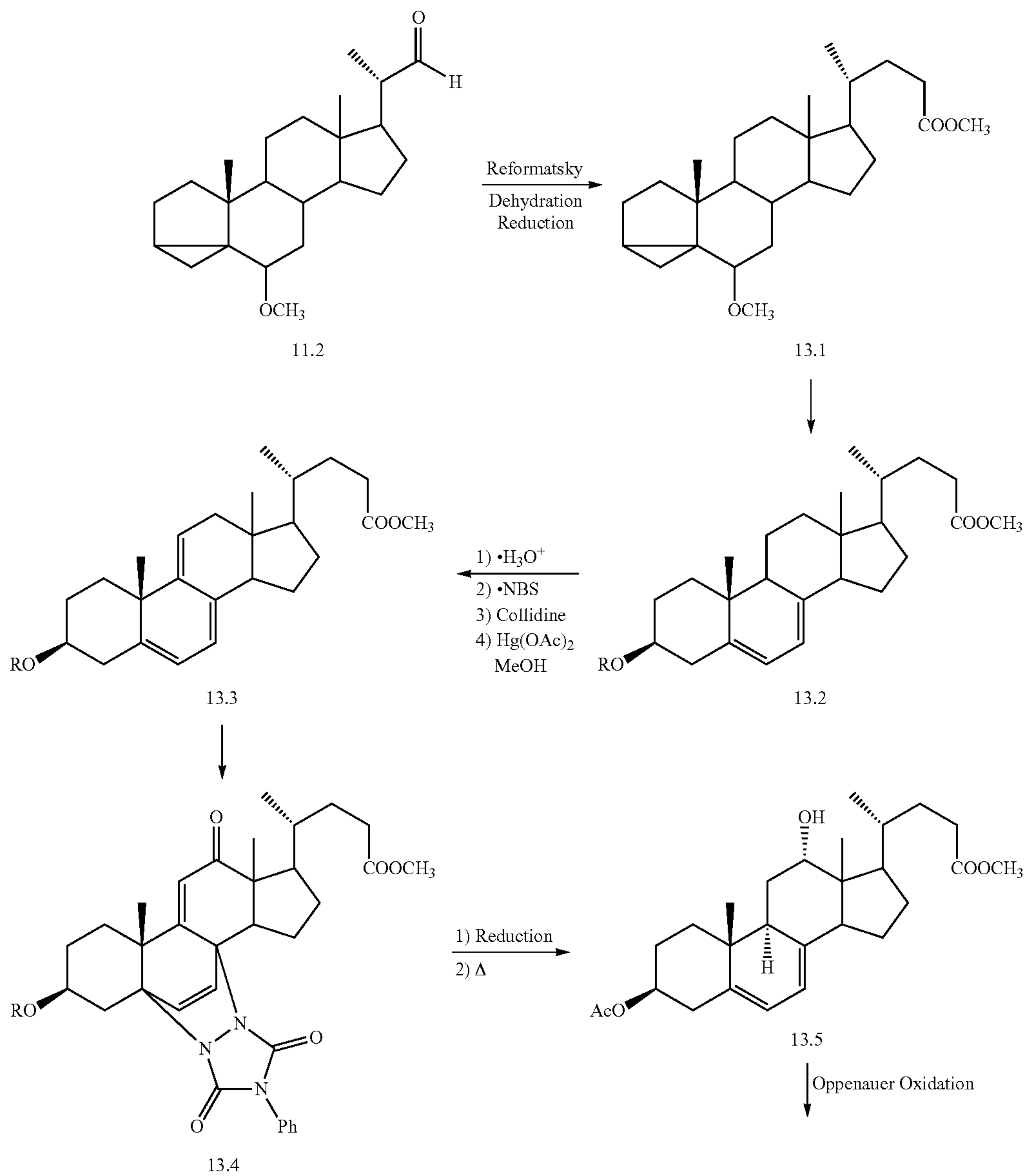
Scheme 13. Triene Formation and Diels-Alder Protection of the Ring B Diene.
