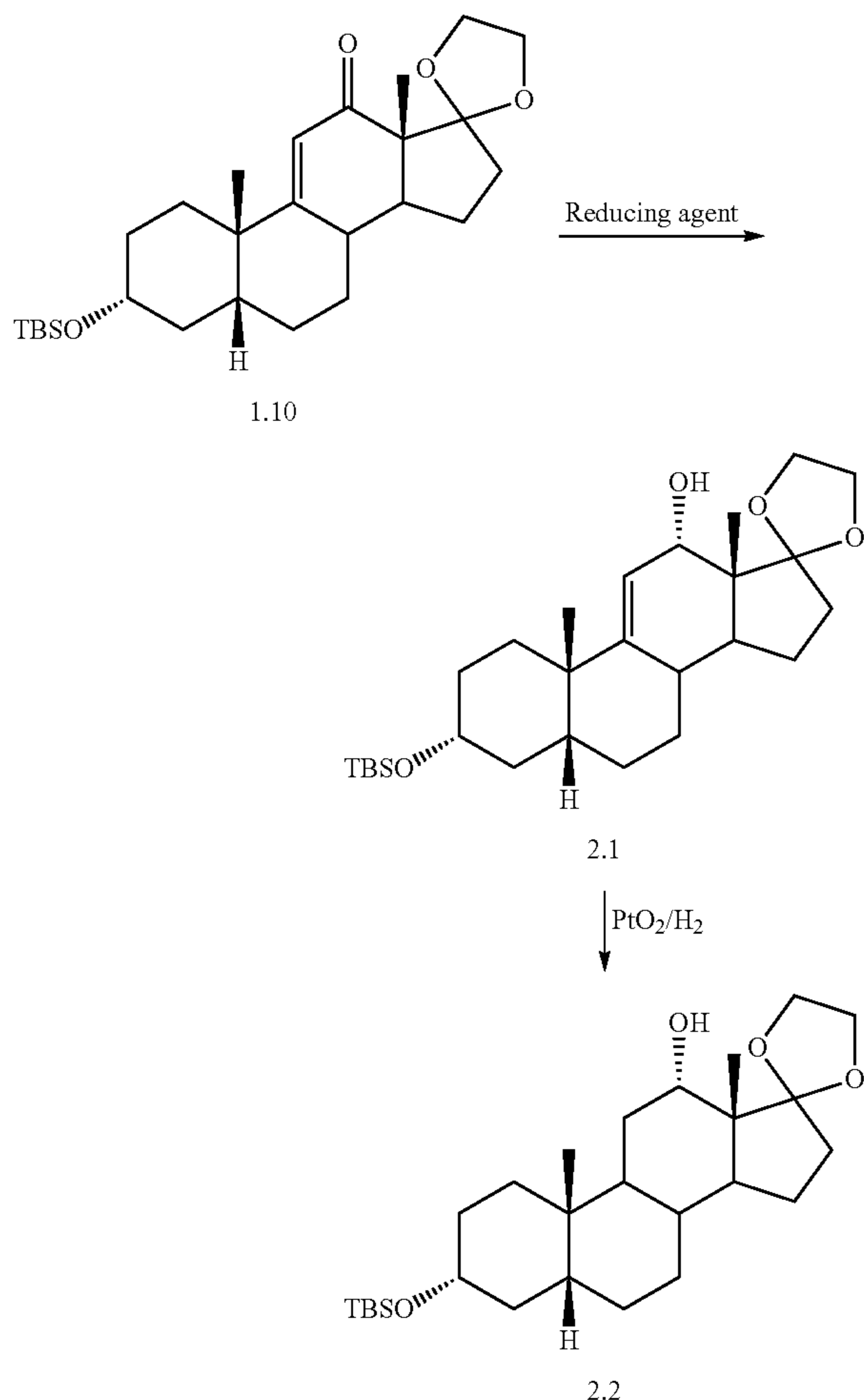
Scheme 2. Introduction of C 12 a hydroxyl group using the allylic oxidation route
