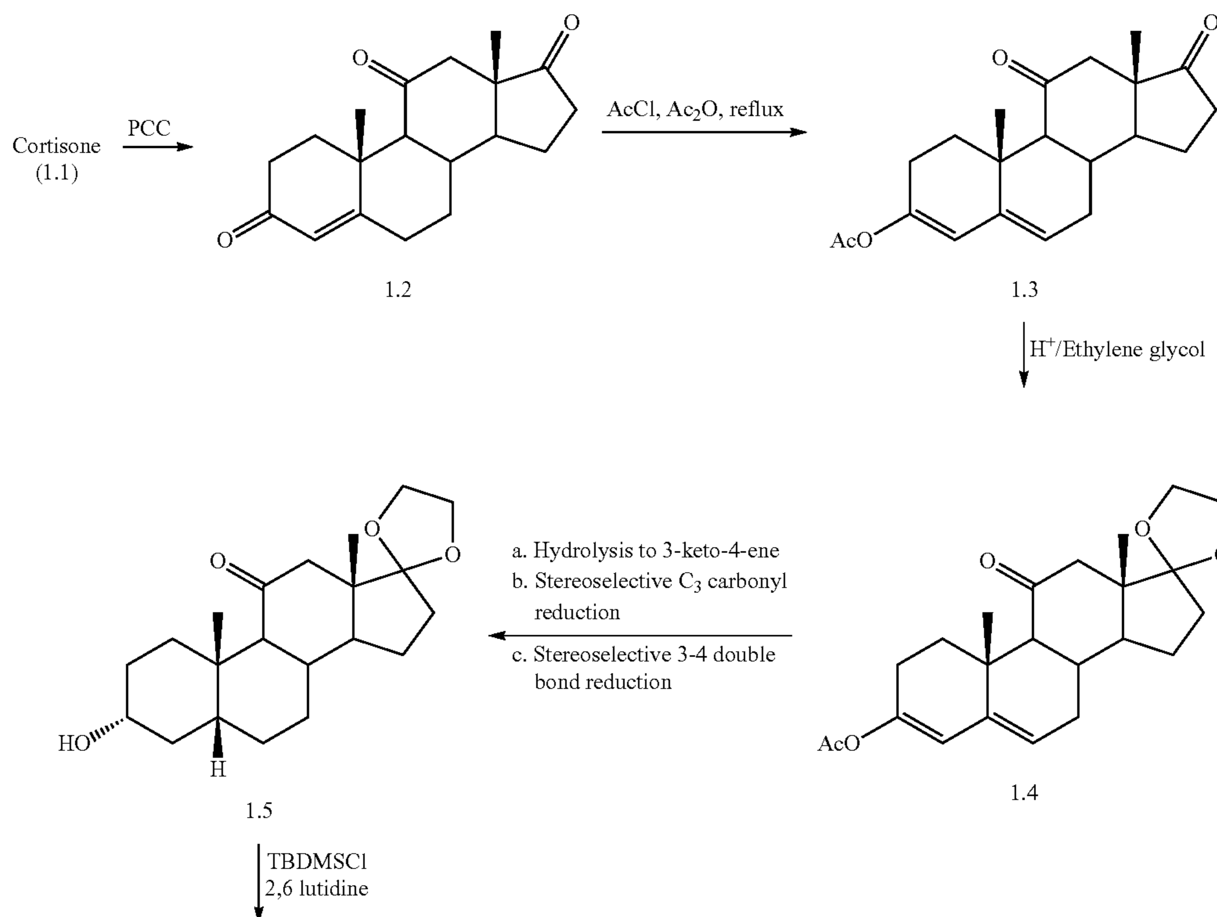
Scheme 1A. Synthesis of the two C-ring precursors of the C 12 hydroxyl group of DCA
