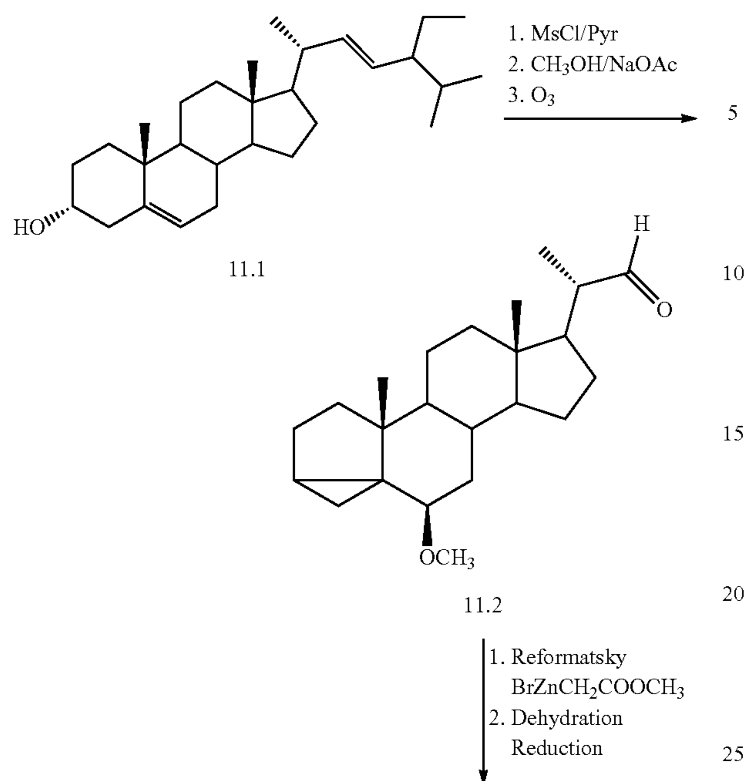
Scheme 11. Ozonolysis of i -steroid and side chain reduction
