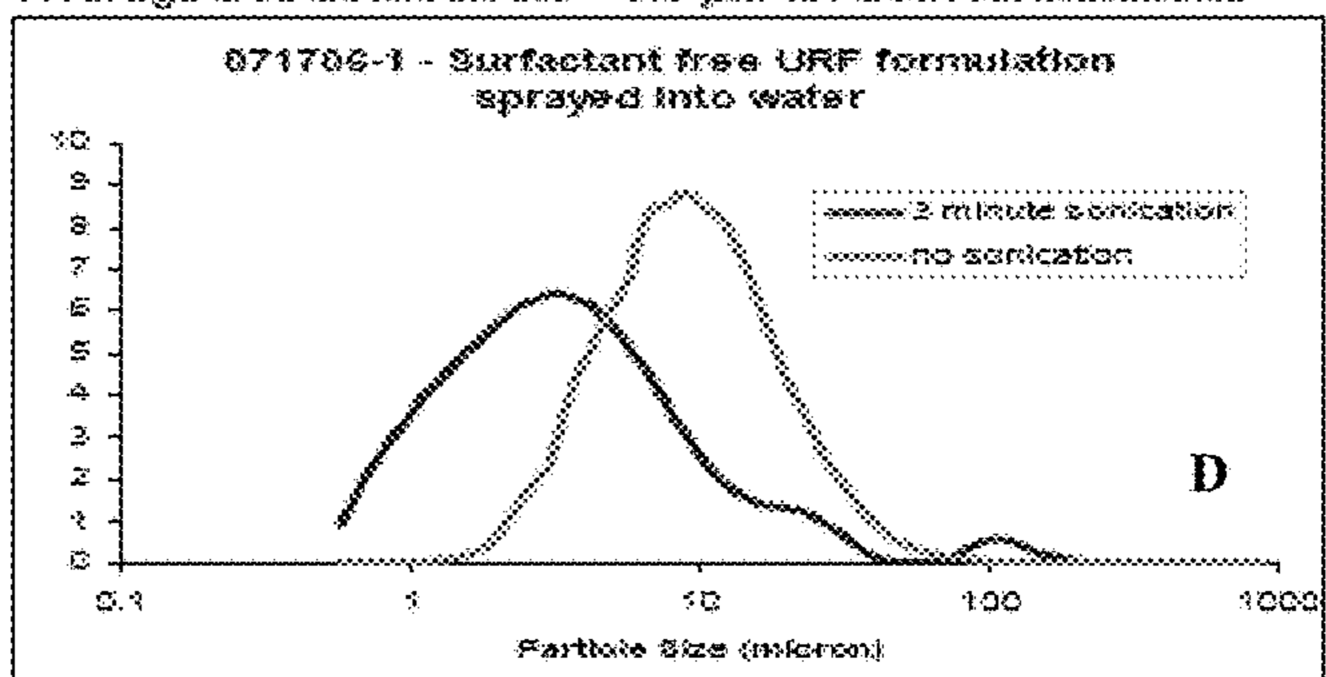
Average D50 ~ 8.4 \mu m for particles without sonication and 3.0 \mu m for particles with sonication
