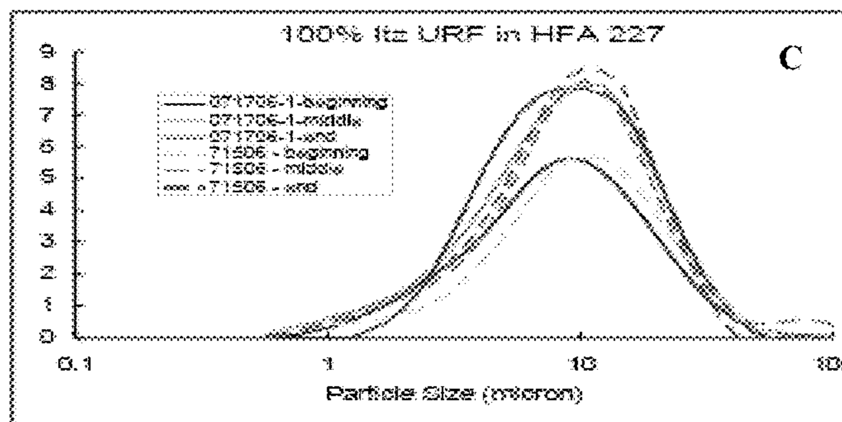
PSD not significantly affected by drug loading in HFA 227 Average D50 between 8.0 – 9.5 \mu m for both formulations
