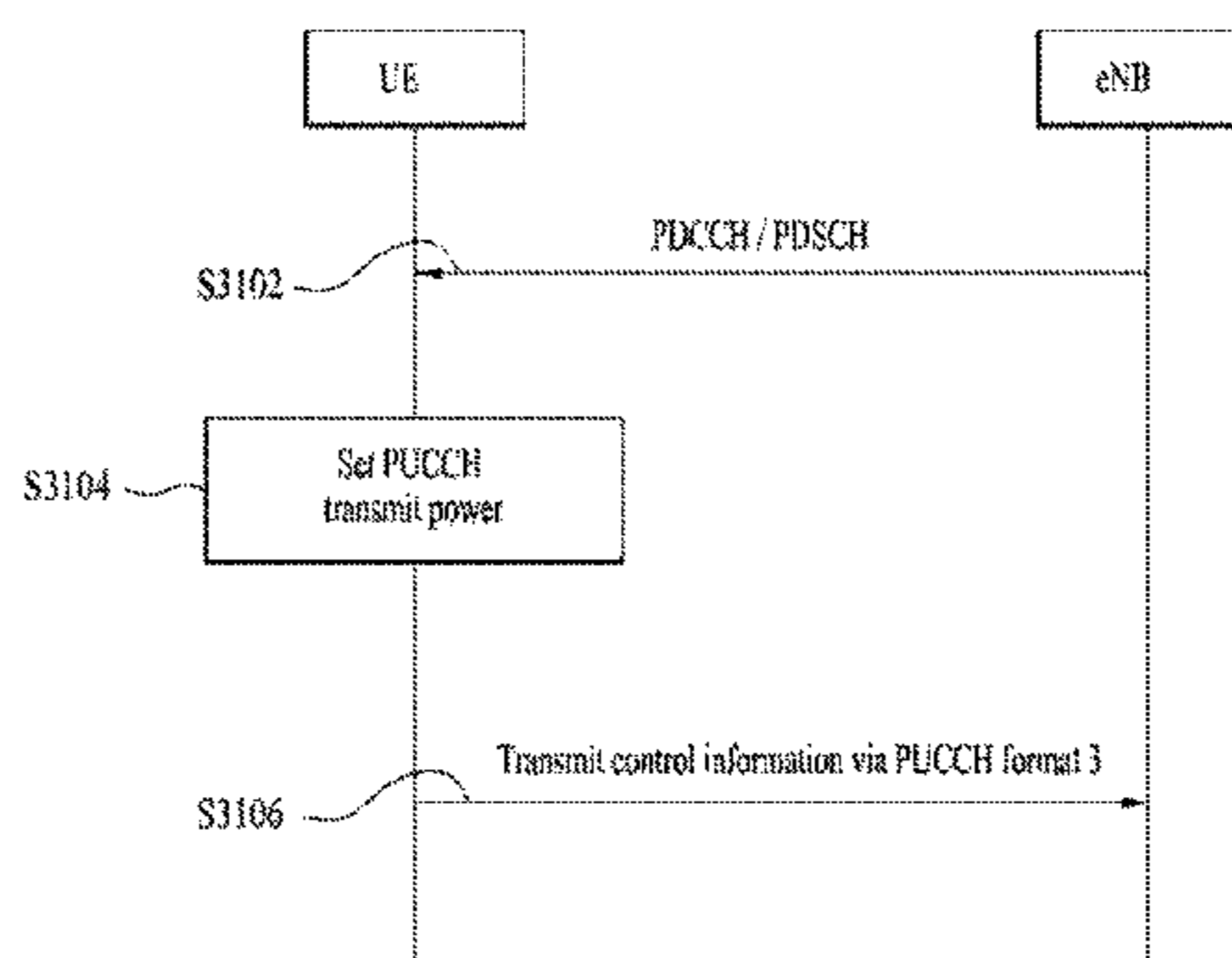
PUCCH transmit power is set in consideration of presence/absence of UL-SCH transport block associated with the SR subframe
