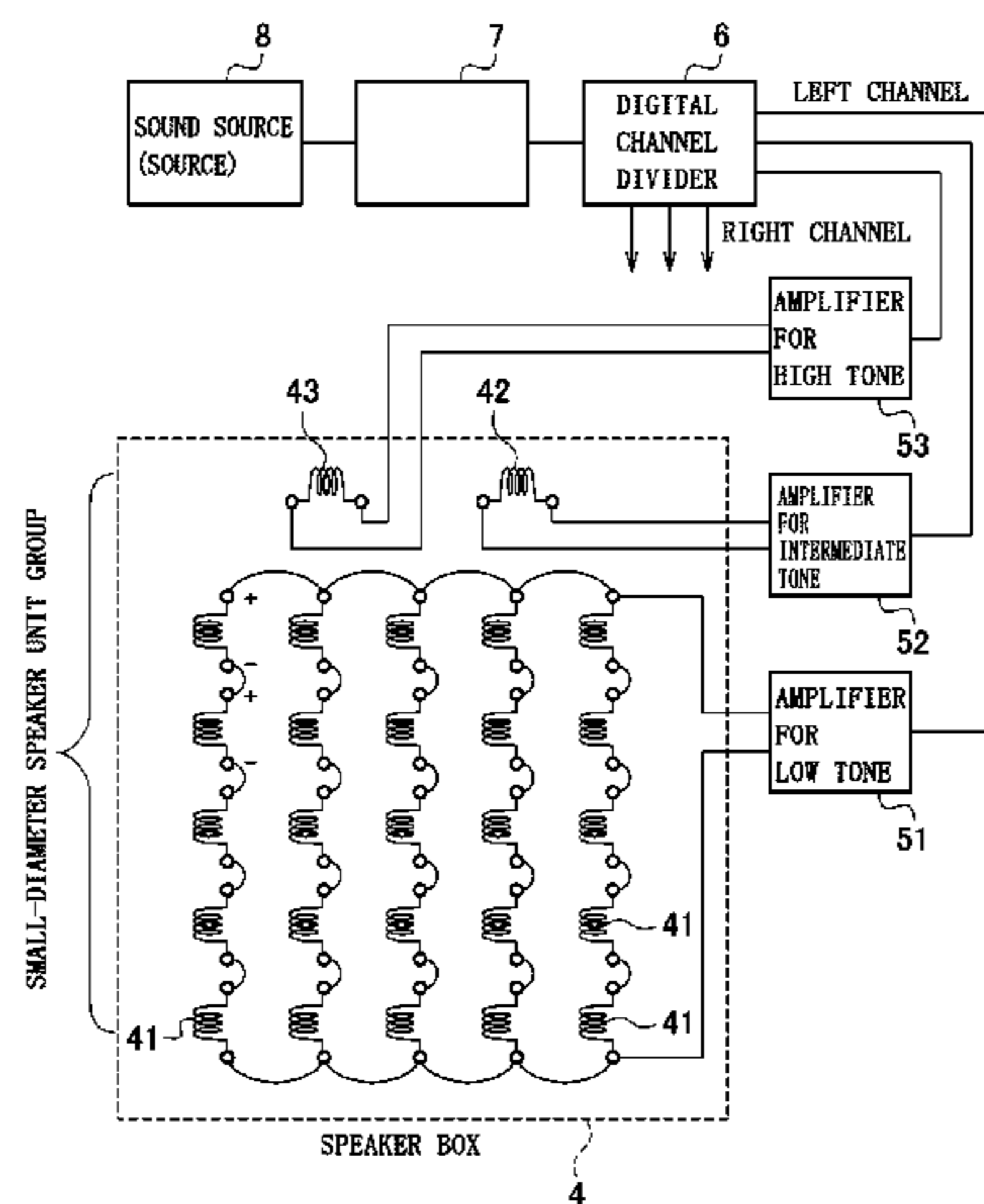
7 = PREAMPLIFIER WITH SOUND FIELD CORRECTION FUNCTION
