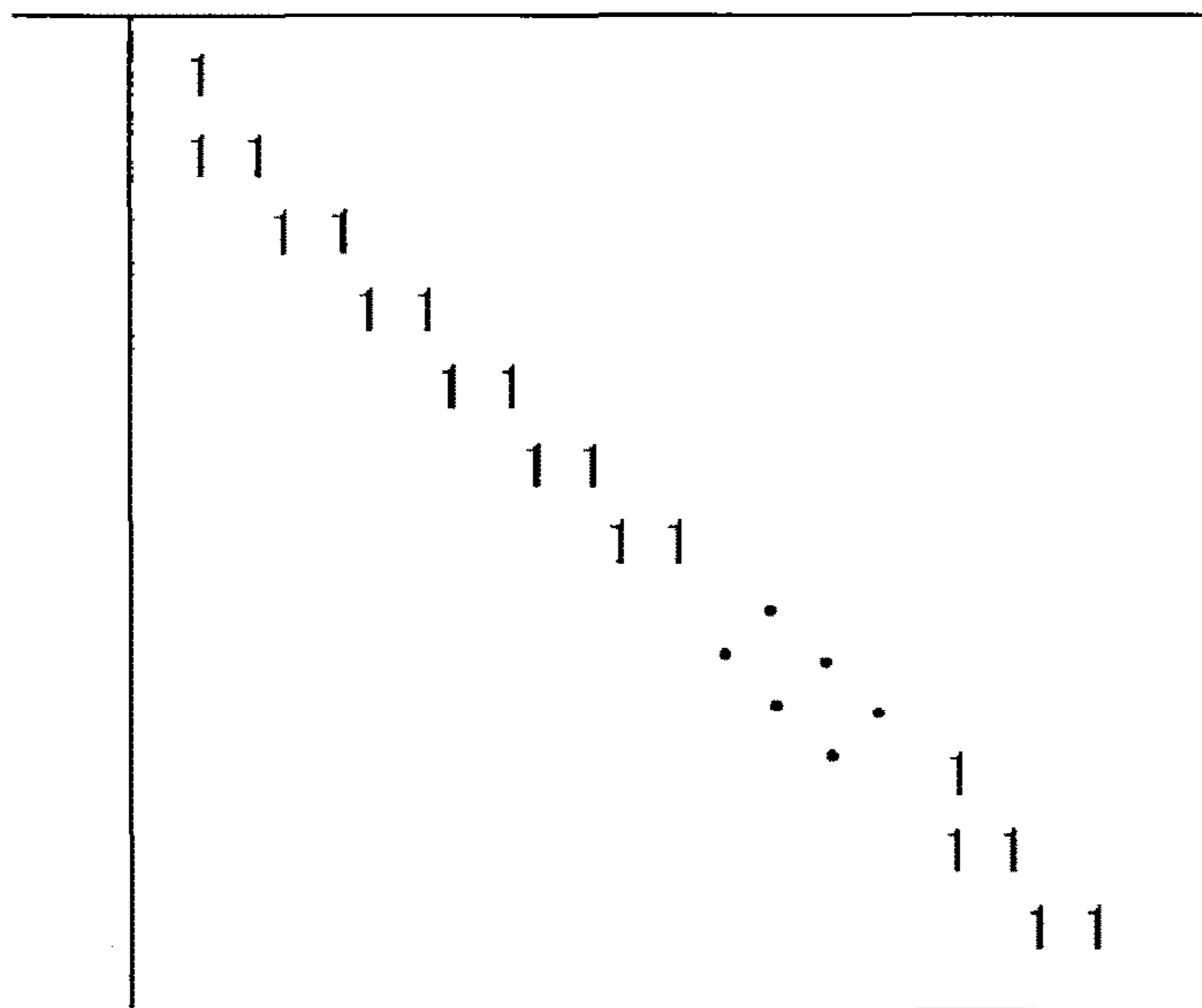
STAIRCASE STRUCTURE OF PARITY MATRIX A
