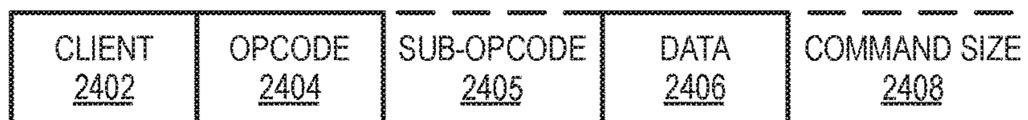
FIG. 17A GRAPHICS PROCESSOR COMMAND FORMAT 2400
