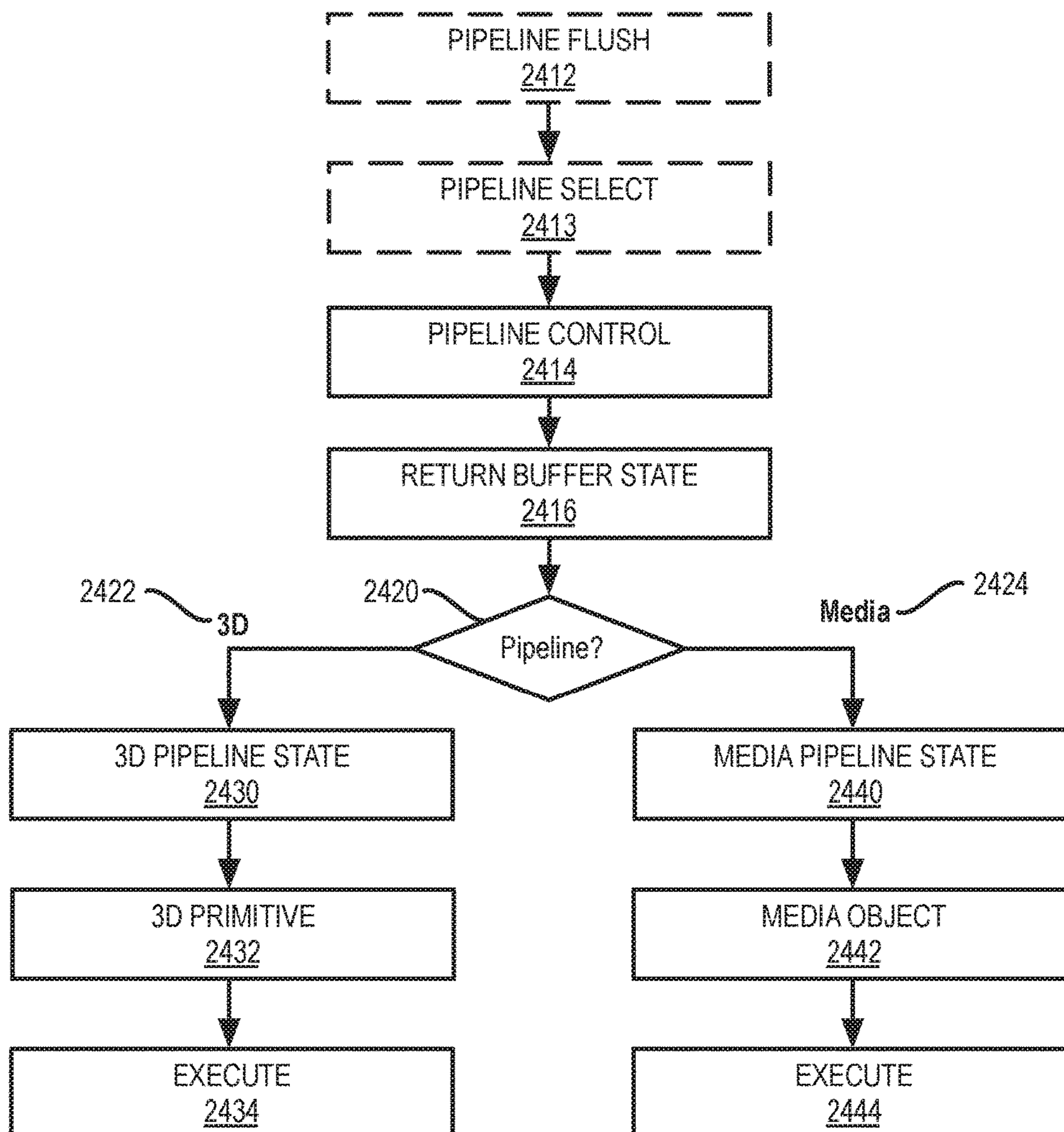
FIG. 17B GRAPHICS PROCESSOR COMMAND SEQUENCE 2410
