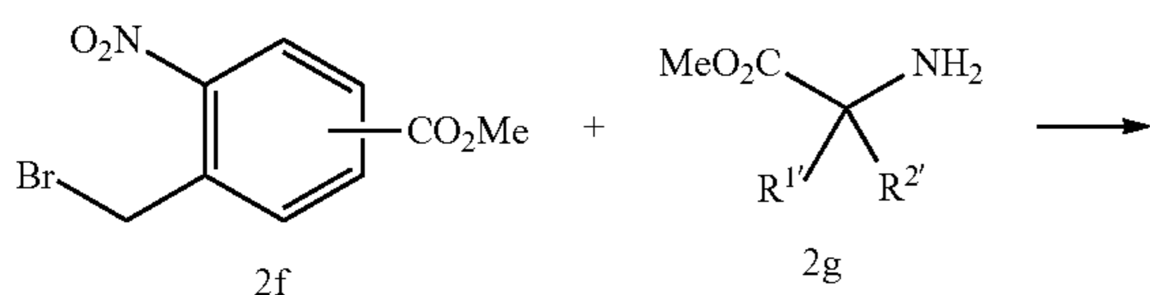
Scheme 2. General synthesis of amides described in the disclosure.
