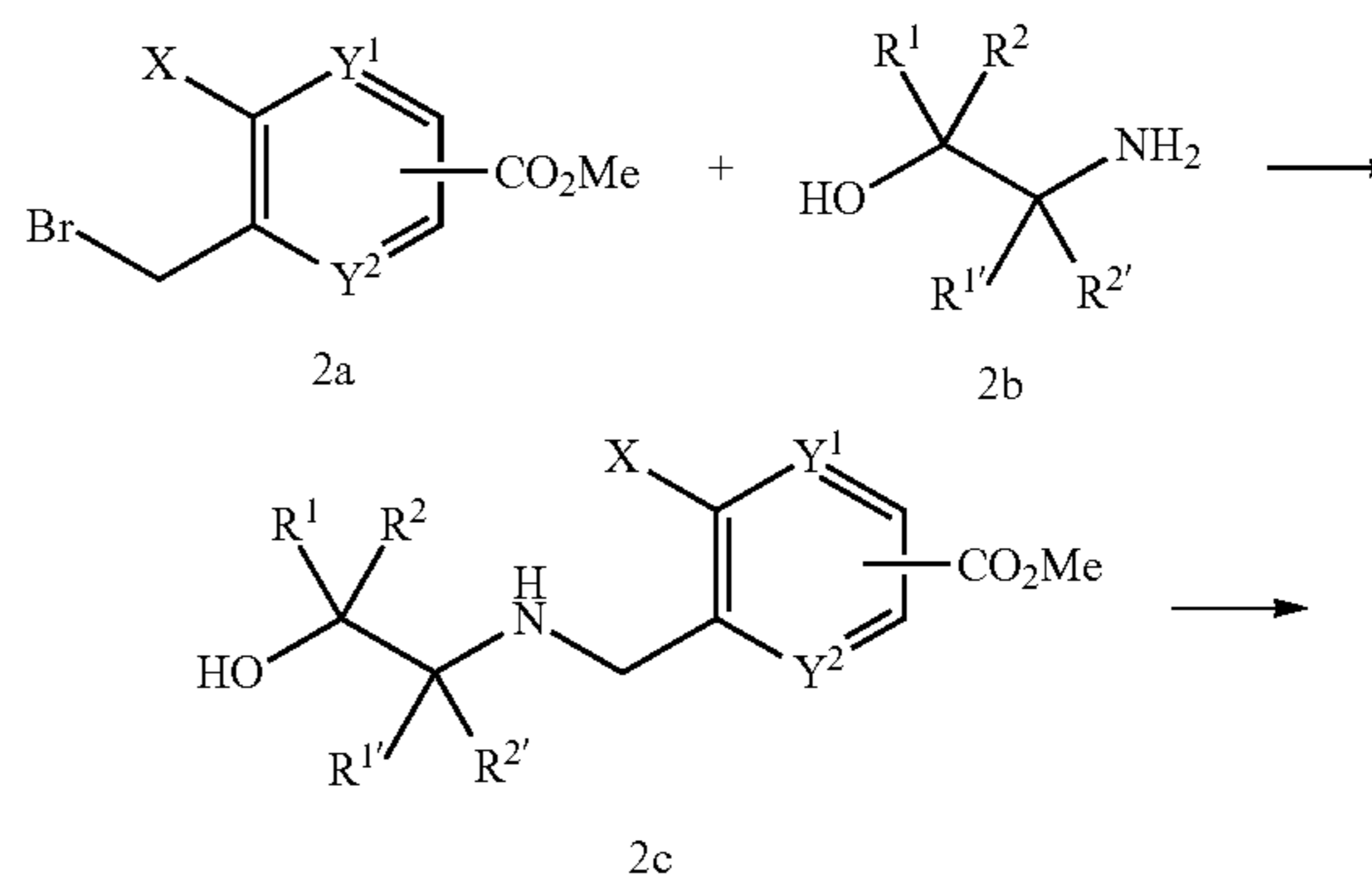
Scheme 1. General synthesis of ethers, thioethers, or sulfones described in the disclosure.
